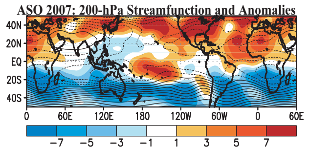
Fig. 14. August–October 2007: 200-hpa streamfunction (contours, 10 \times 10^6 \text{ m}^2 \text{ s}^{-1} ) and anomalies (shaded). Anomalous ridges are indicated by positive values (red) in the NH and negative values (blue) in the SH. Anomalous troughs are indicated by negative values in the NH and positive values in the SH. Anomalies are departures from the 1971-2000 period monthly means.
