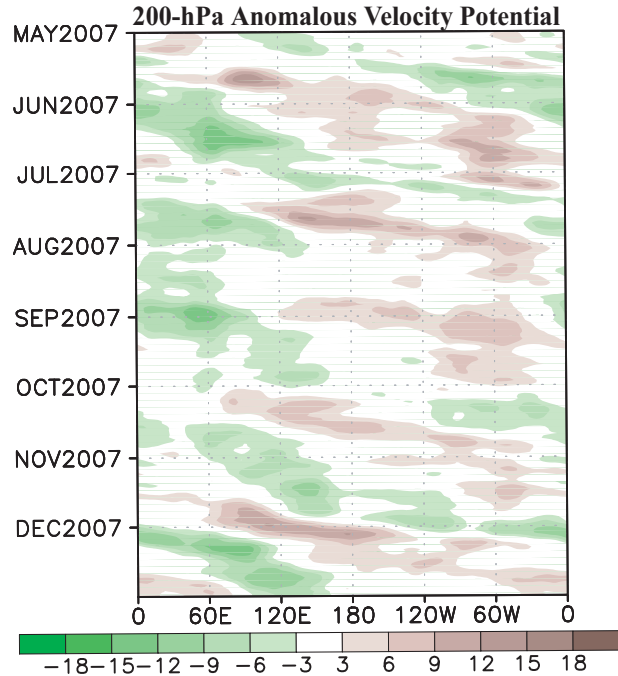
Fig. 13. Time-longitude section of 5-day running mean 200-hpa velocity potential anomalies ( \times 10^6 \text{ m}^2 \text{ s}^{-1} ) averaged over the region 5^\circ\text{N} - 5^\circ\text{S} . Green shading indicate enhanced convection and anomalous upper-level divergence, and brown shading indicate suppressed convection and anomalous upper-level convergence. Anomalies are departures from the 1971-2000 period daily means.
