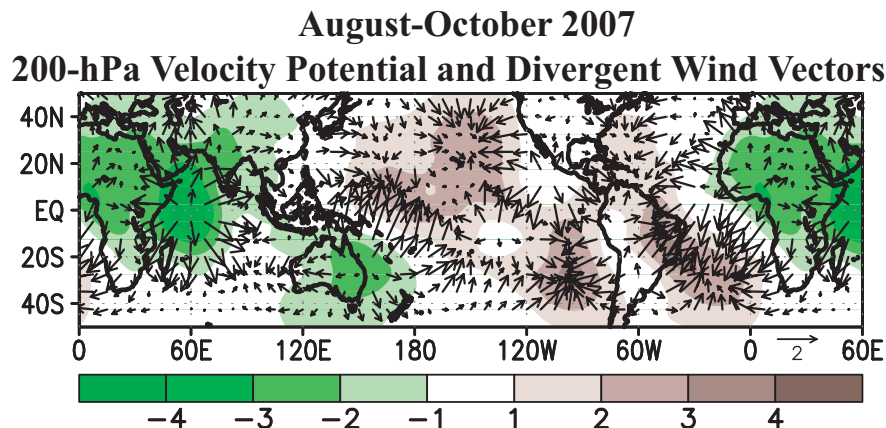
Fig. 17. August-October 2007: Anomalous 200-hPa velocity potential ( \times 10^6 \text{ m}^2 \text{ s}^{-1} ) and divergent wind vectors ( \text{m s}^{-1} ). Vector scale is shown at bottom right. Anomalies are departures from the 1971-2000 period daily means.
