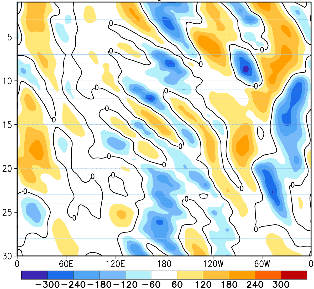
FIGURE E12. Northern Hemisphere: Daily 500-hPa height anomalies for APR 2016 averaged over the 5° latitude band centered on 40°N. Positive values are indicated by solid contours and dark shading. Negative values are indicated by dashed contours and light shading. Contour interval is 60 m. Anomalies are departures from the 1981-2010 base period daily means.
