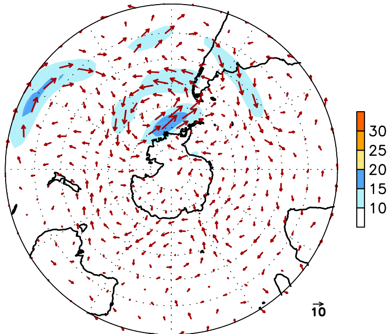
FIGURE E16. Southern Hemisphere mean (left) and anomalous (right) 300-hPa vector wind (CDAS/Reanalysis) for APR 2016. Mean (anomaly) isotach contour interval is 10 (5) ms -1 . Values greater than 30 ms -1 (left) and 10 ms -1 (rights) are shaded. Anomalies are departures from the 1981-2010 base period monthly means.
