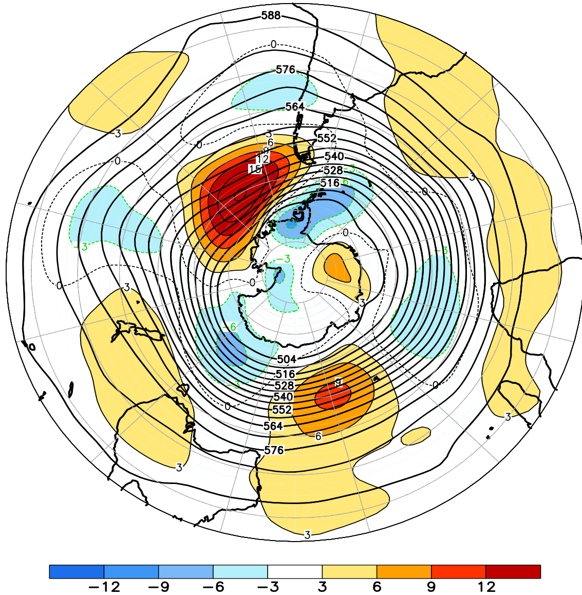
FIGURE E15. Southern Hemisphere mean and anomalous 500-hPa geopotential height (CDAS/Reanalysis) for APR 2016. Mean heights are denoted by solid contours drawn at an interval of 6 dam. Anomaly contour interval is 3 dam with values less (greater) than -3 dam (3 dam) indicated by dark (light) shading. Anomalies are calculated as departures from the 1981-2010 base period monthly means.
