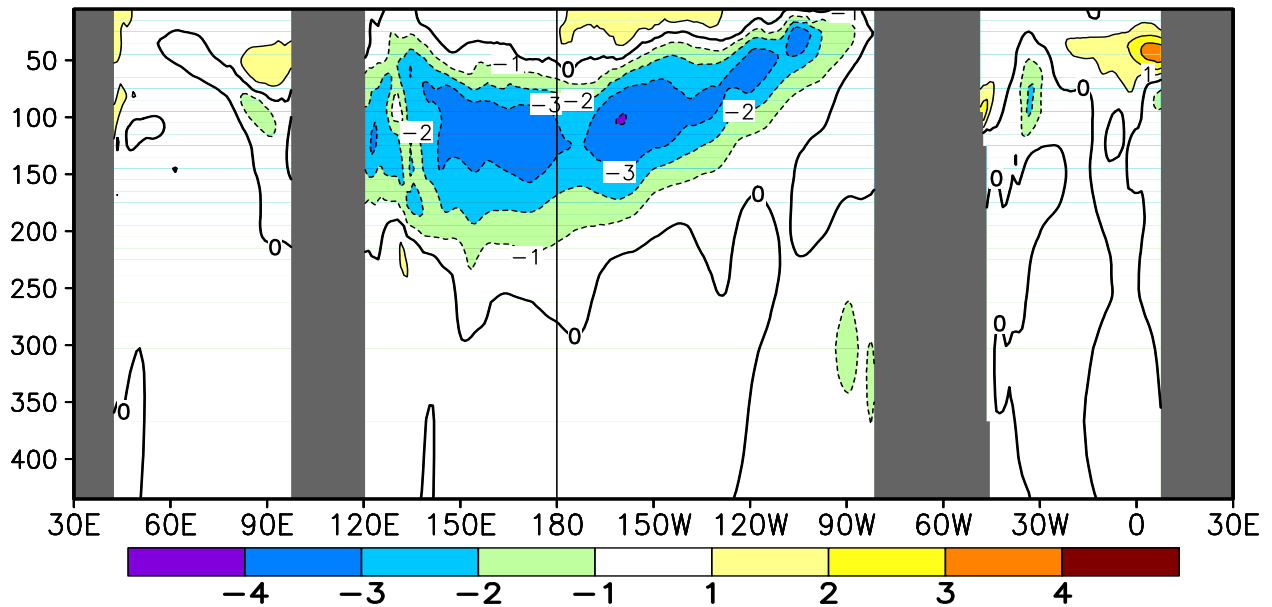
FIGURE T17. Equatorial depth–longitude section of ocean temperature (top) and ocean temperature anomalies (bottom) for APR 2016. Contour interval is 1°C. Dashed contours in bottom panel indicate negative anomalies. Data are derived from the NCEP’s global ocean data assimilation system version 2 which assimilates oceanic observations into an oceanic GCM (Xue, Y. and Behringer, D.W., 2006: Operational global ocean data assimilation system at NCEP, to be submitted to BAMS). Anomalies are departures from the 1981–2010 base period means.
