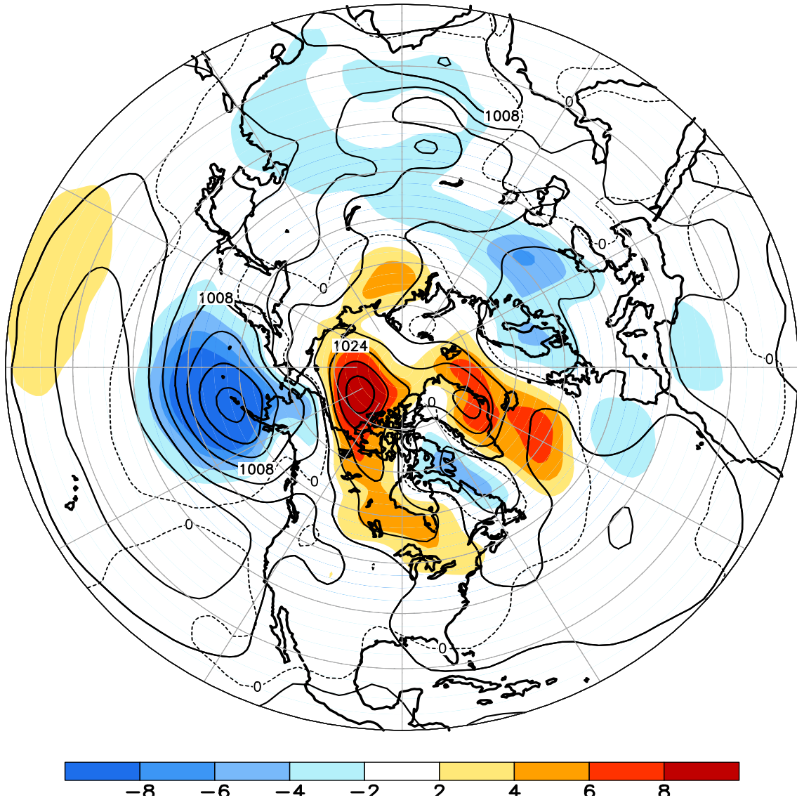
FIGURE E8. Northern Hemisphere mean and anomalous sea level pressure (CDAS/Reanalysis) for APR 2016. Mean values are denoted by solid contours drawn at an interval of 4 hPa. Anomaly contour interval is 2 hPa with values less (greater) than -2 hPa (2 hPa) indicated by dark (light) shading. Anomalies are calculated as departures from the 1981-2010 base period monthly means.
