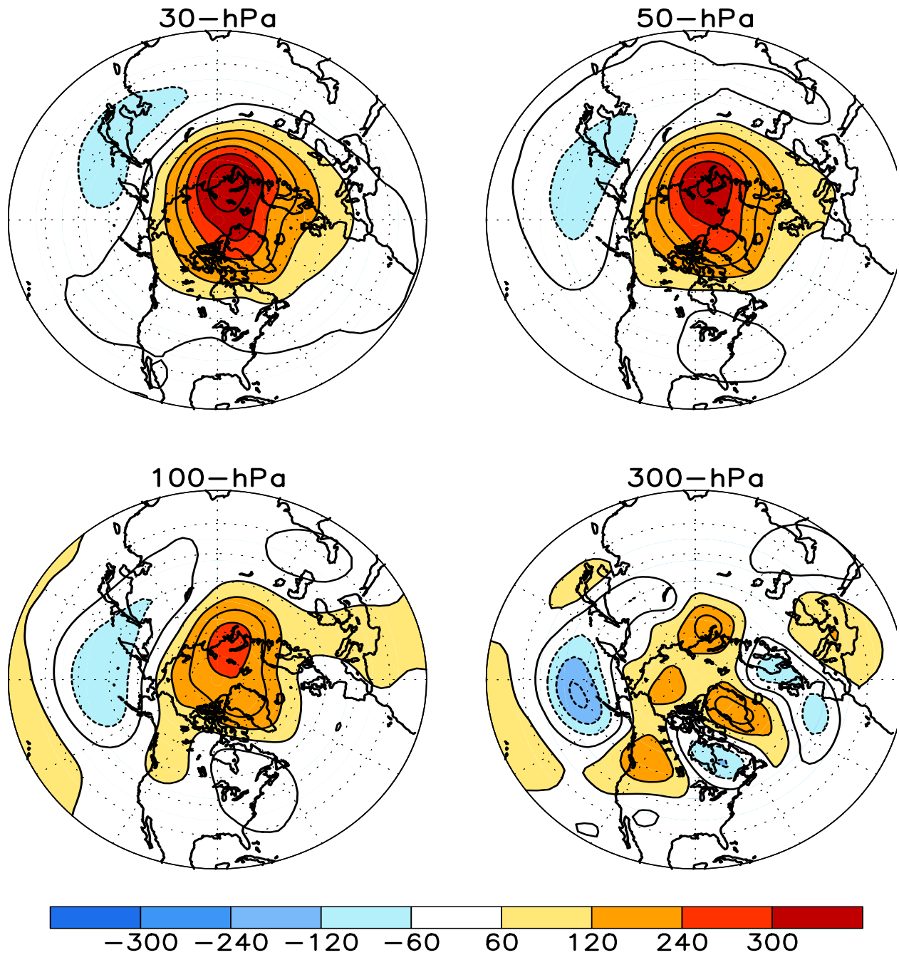
FIGURE S1. Stratospheric height anomalies (m) at selected levels for APR 2016. Positive values are indicated by solid contours and dark shading. Negative values are indicated by dashed contours and light shading. Contour interval is 60 m. Anomalies are calculated from the 1981-2010 base period means. Winter Hemisphere is shown.
