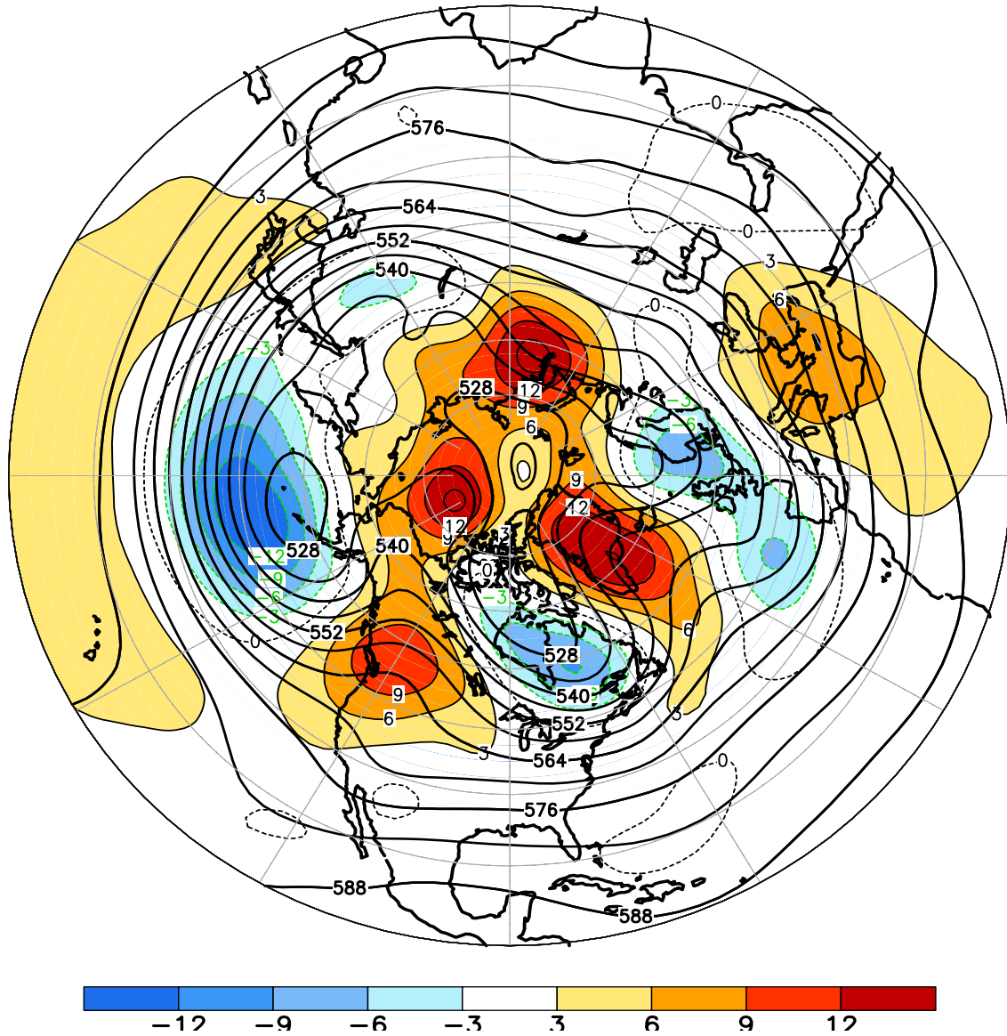
FIGURE E9. Northern Hemisphere mean and anomalous 500-hPa geopotential height (CDAS/Reanalysis) for APR 2016. Mean heights are denoted by solid contours drawn at an interval of 6 dam. Anomaly contour interval is 3 dam with values less (greater) than -3 dam (3 dam) indicated by dark (light) shading. Anomalies are calculated as departures from the 1981-2010 base period monthly means.
