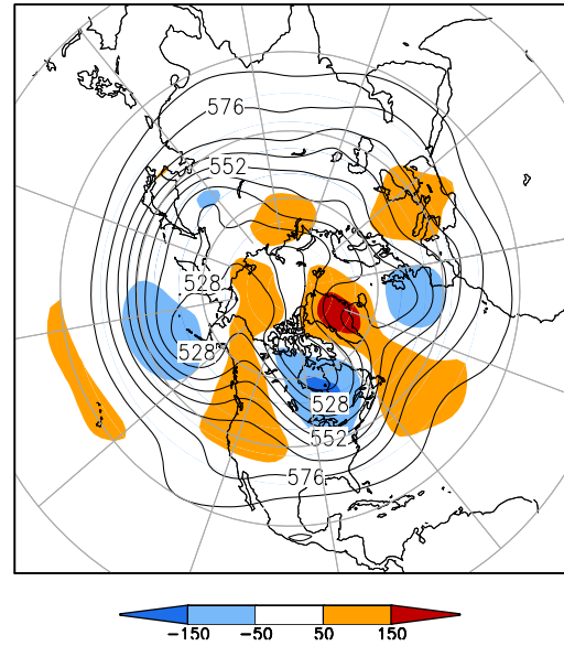
500-hPa Height (dm) & Anomalies (m) (Apr 1–15, 2016)
