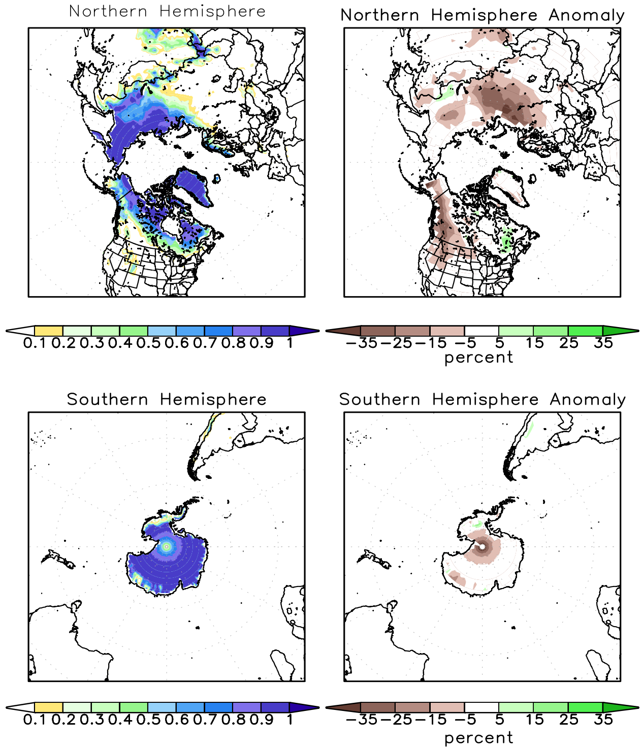
FIGURE A2.2. SSM/I derived snow cover frequency (%) (left) and snow cover anomaly (%) (right) for the month of APR 2016 based on 1987 - 2010 base period for the Northern Hemisphere (top) and Southern Hemisphere (bottom). It is generated using the algorithm described by Ferraro et. al, 1996, Bull. Amer. Meteor. Soc., vol 77, 891-905.
