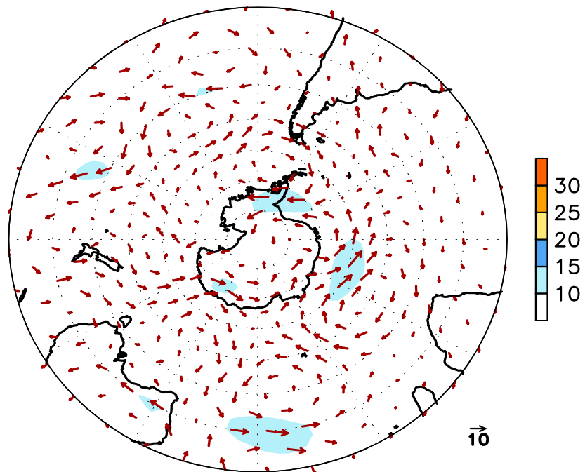
FIGURE E16. Southern Hemisphere mean (left) and anomalous (right) 300-hPa vector wind (CDAS/Reanalysis) for APR 2023. Mean (anomaly) isotach contour interval is 10 (5) \text{ms}^{-1} . Values greater than 30 \text{ms}^{-1} (left) and 10 \text{ms}^{-1} (rights) are shaded. Anomalies are departures from the 1991-2020 base period monthly means.
