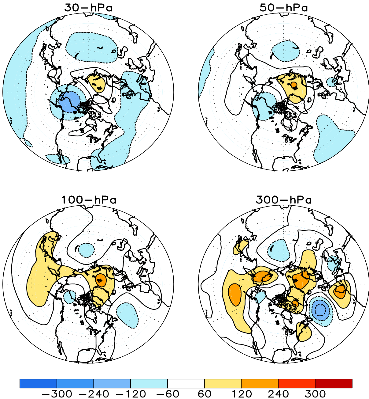
FIGURE S1. Stratospheric height anomalies (m) at selected levels for APR 2023. Positive values are indicated by solid contours and dark shading. Negative values are indicated by dashed contours and light shading. Contour interval is 60 m. Anomalies are calculated from the 1991-2020 base period means. Winter Hemisphere is shown.
