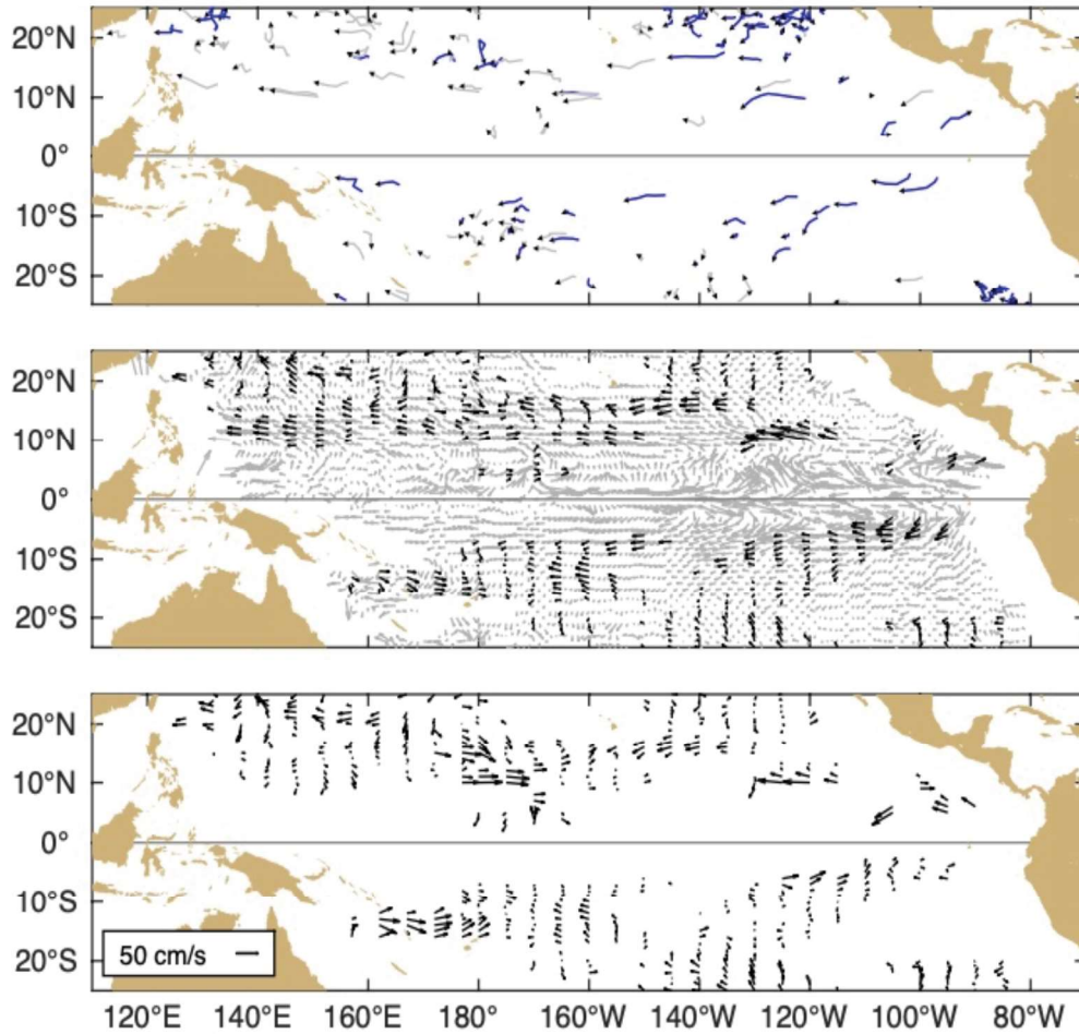
Figure A1.1 Top: Movements of drifting buoys in the tropical Pacific Ocean during April 2023. The linear segments of each trajectory represent a one week displacement. Trajectories of buoys which have lost their subsurface drogues are gray; those with drogues are black.
