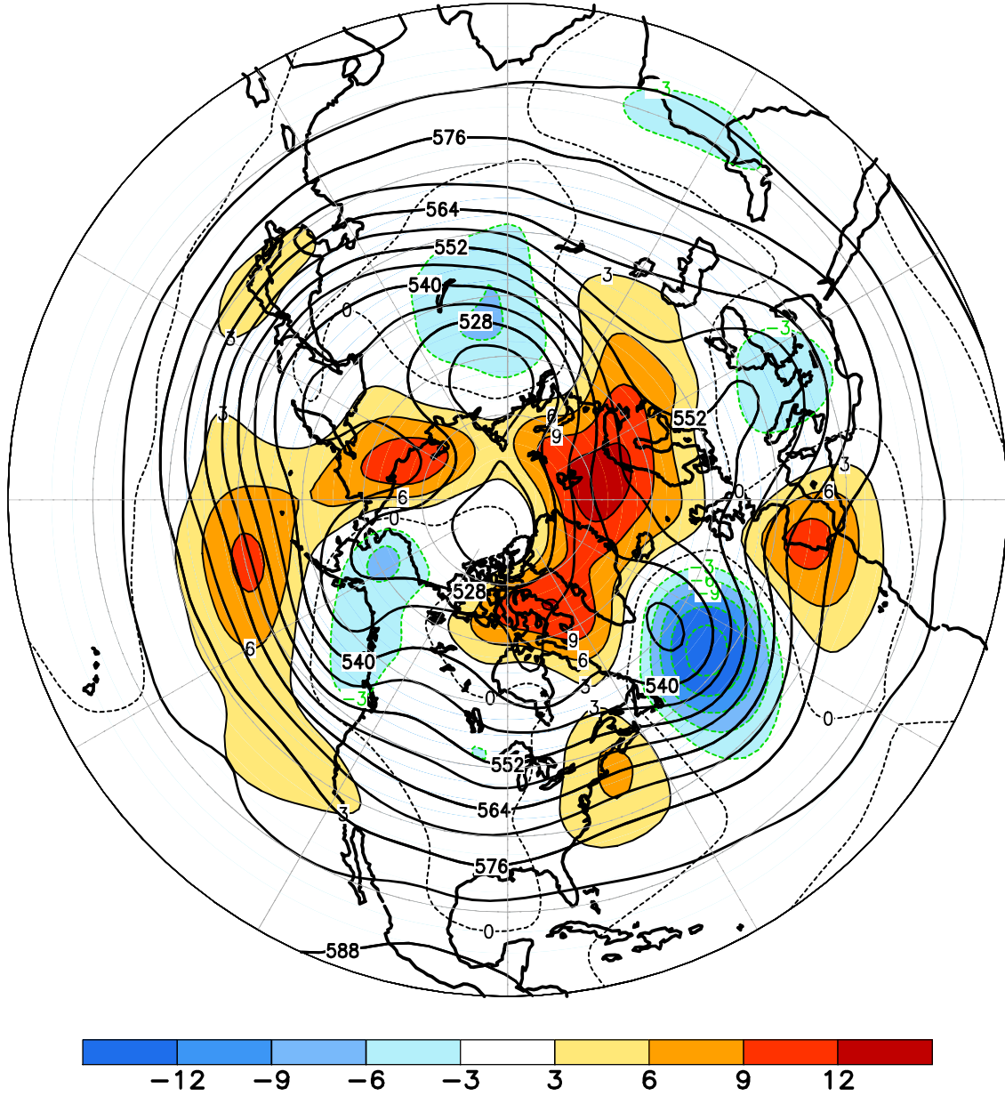
FIGURE E9. Northern Hemisphere mean and anomalous 500-hPa geopotential height (CDAS/Reanalysis) for APR 2023. Mean heights are denoted by solid contours drawn at an interval of 6 dam. Anomaly contour interval is 3 dam with values less (greater) than -3 dam (3 dam) indicated by dark (light) shading. Anomalies are calculated as departures from the 1991-2020 base period monthly means.
