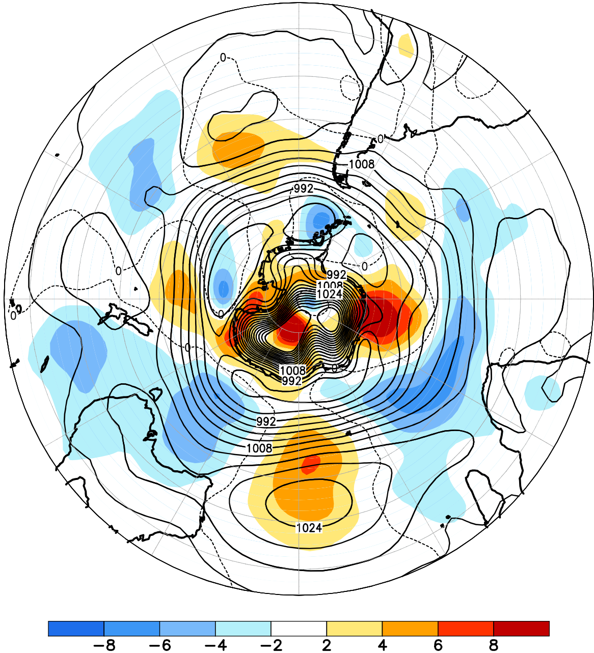
FIGURE E14. Southern Hemisphere mean and anomalous sea level pressure(CDAS/Reanalysis) for APR 2023. Mean values are denoted by solid contours drawn at an interval of 4 hPa. Anomaly contour interval is 2 hPa with values less (greater) than -2 hPa (2 hPa) indicated by dark (light) shading. Anomalies are calculated as departures from the 1991-2020 base period monthly means.
