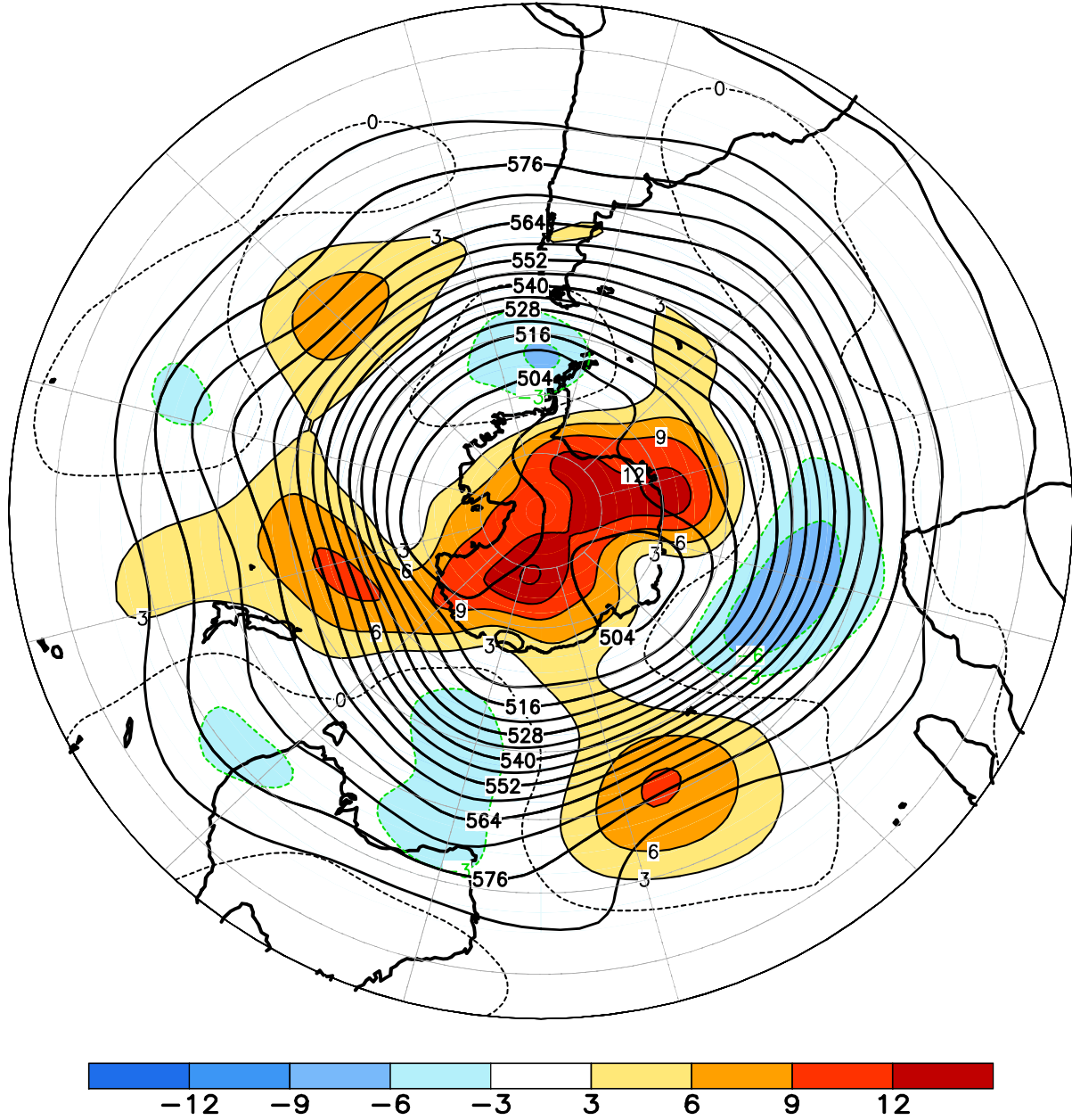
FIGURE E15. Southern Hemisphere mean and anomalous 500-hPa geopotential height (CDAS/Reanalysis) for APR 2023. Mean heights are denoted by solid contours drawn at an interval of 6 dam. Anomaly contour interval is 3 dam with values less (greater) than -3 dam (3 dam) indicated by dark (light) shading. Anomalies are calculated as departures from the 1991-2020 base period monthly means.
