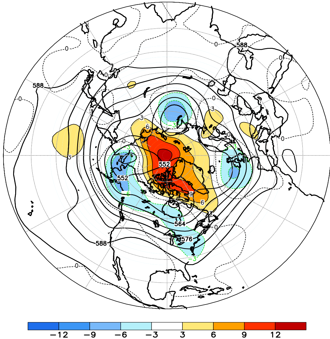
FIGURE E9. Northern Hemisphere mean and anomalous 500-hPa geopotential height (CDAS/Reanalysis) for AUG 2011. Mean heights are denoted by solid contours drawn at an interval of 6 dam. Anomaly contour interval is 3 dam with values less (greater) than -3 dam (3 dam) indicated by dark (light) shading. Anomalies are calculated as departures from the 1981-2010 base period monthly means.
