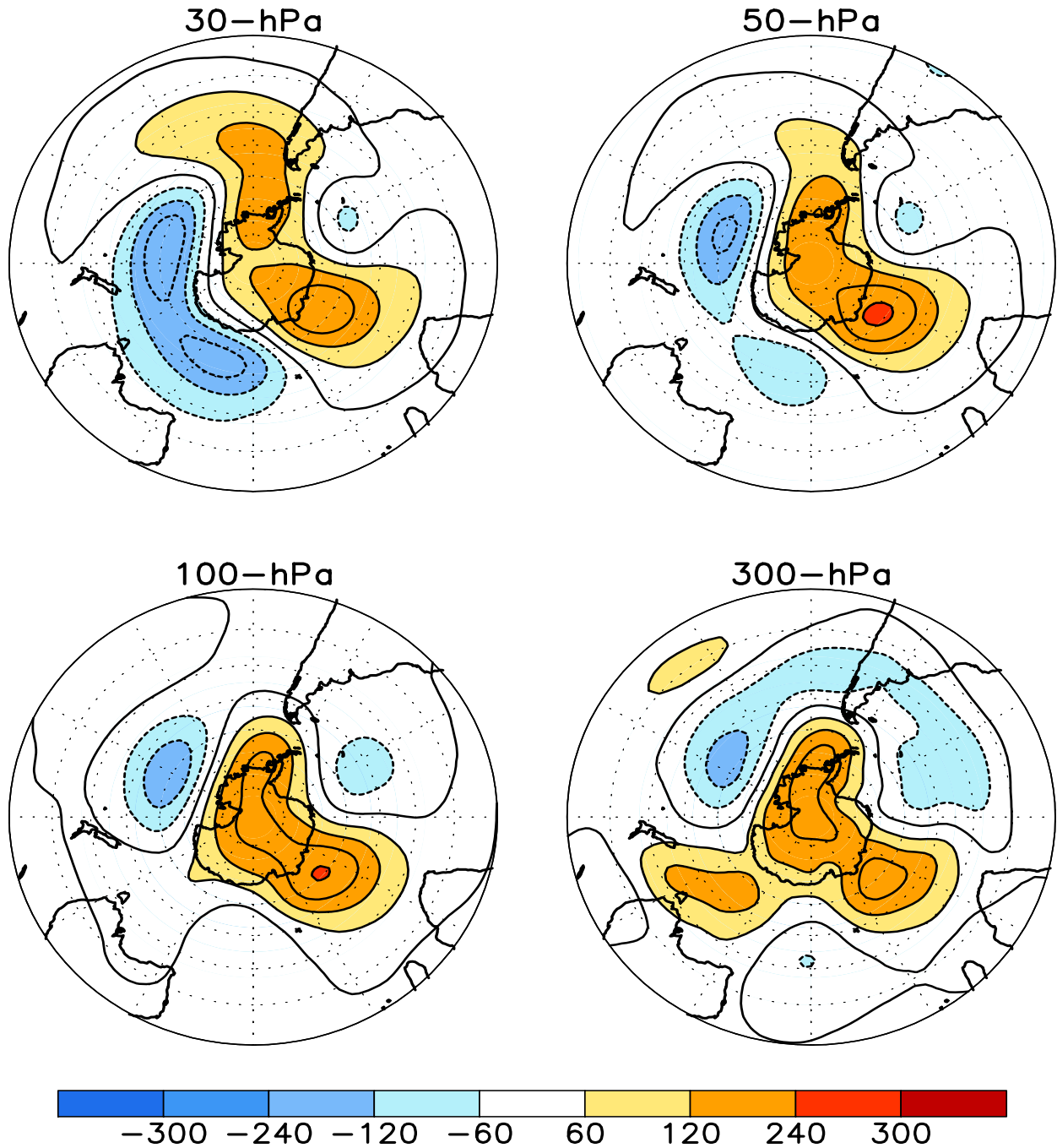
FIGURE S1. Stratospheric height anomalies (m) at selected levels for AUG 2011. Positive values are indicated by solid contours and dark shading. Negative values are indicated by dashed contours and light shading. Contour interval is 60 m. Anomalies are calculated from the 1981-2010 base period means. Winter Hemisphere is shown.
