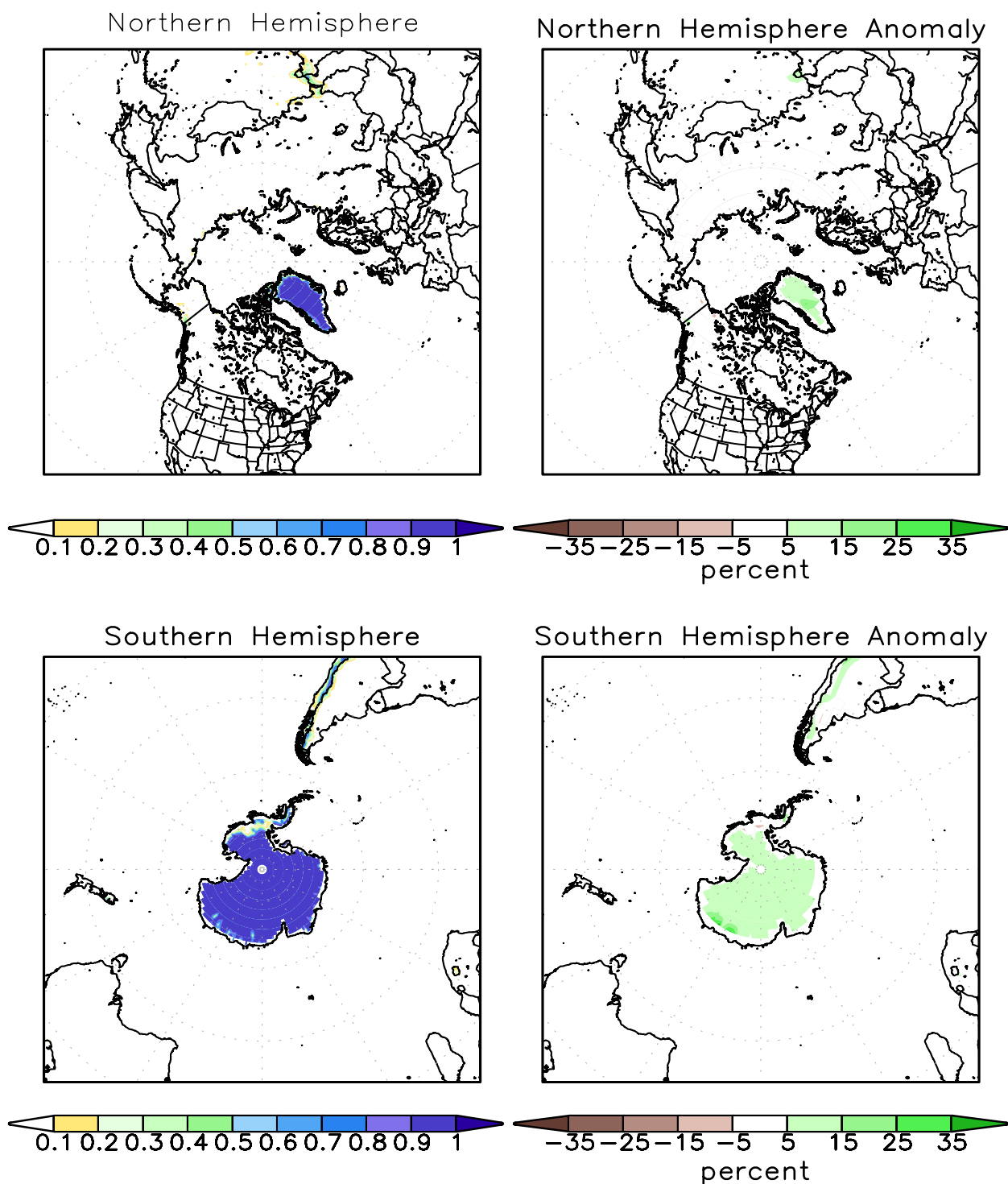
FIGURE A2.2. SSM/I derived snow cover frequency (%) (left) and snow cover anomaly (%) (right) for the month of AUG 2011 based on 1987 - 2010 base period for the Northern Hemisphere (top) and Southern Hemisphere (bottom). It is generated using the algorithm described by Ferraro et. al, 1996, Bull. Amer. Meteor. Soc., vol 77, 891-905.
