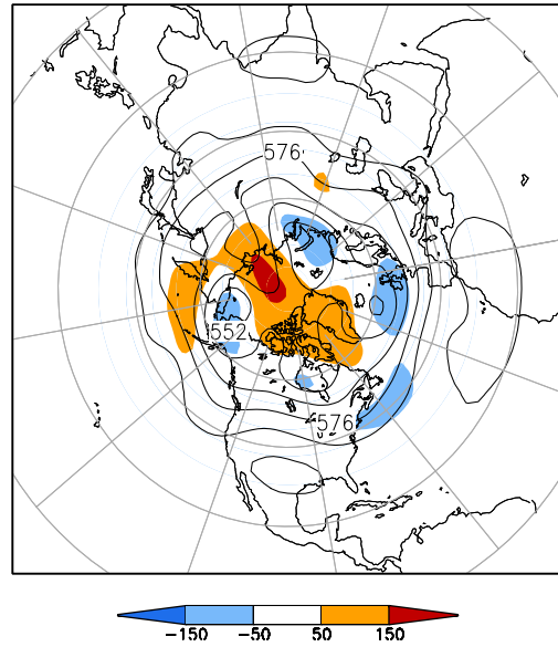
500-hPa Height (dm) & Anomalies (m) (Aug 1–15, 2011)
