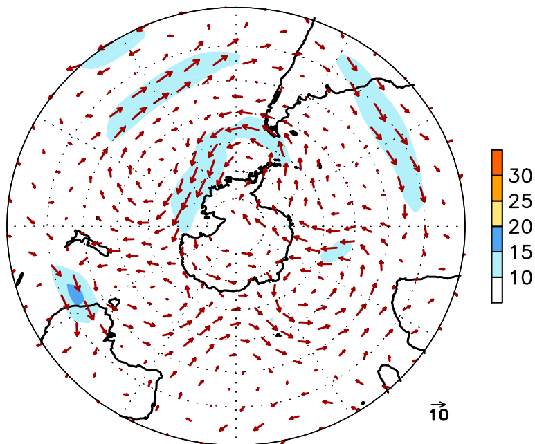
FIGURE E16. Southern Hemisphere mean (left) and anomalous (right) 300-hPa vector wind (CDAS/Reanalysis) for AUG 2011. Mean (anomaly) isotach contour interval is 10 (5) \text{ms}^{-1} . Values greater than 30 \text{ms}^{-1} (left) and 10 \text{ms}^{-1} (rights) are shaded. Anomalies are departures from the 1981-2010 base period monthly means.
