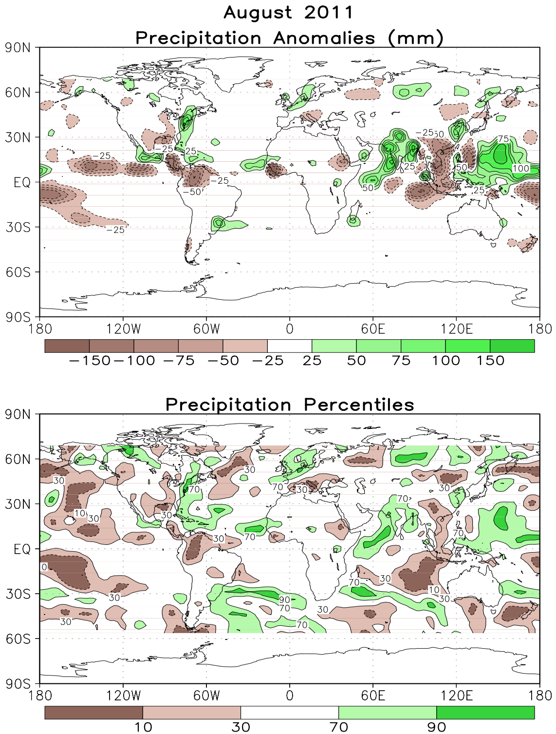
FIGURE E3. Anomalous precipitation (mm, top) and precipitation percentiles based on a Gamma distribution fit to the 1981–2010 base period data (bottom) for AUG 2011. Data are obtained from a merge of raingauge observations and satellite-derived precipitation estimates (Janowiak and Xie 1999, J. Climate , 12 , 3335–3342). Contours are drawn at 200, 100, 50, 25, -25, -50, -100, and -200 mm in top panel. Percentiles are not plotted in regions where mean monthly precipitation is <5mm/month.
