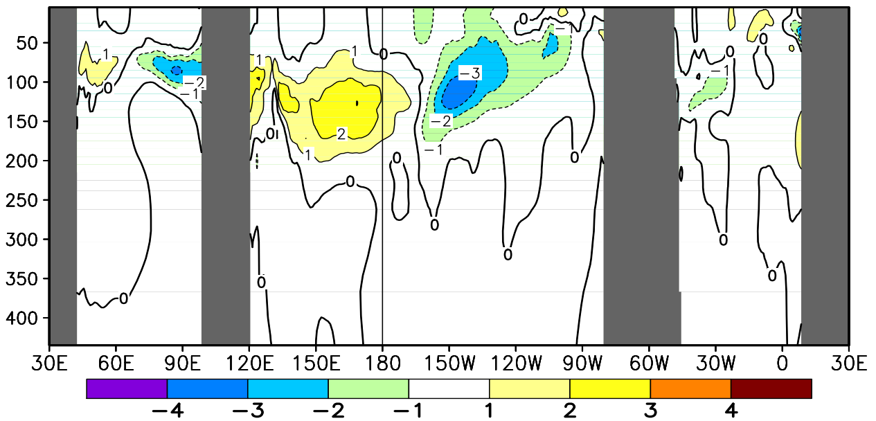
FIGURE T17. Equatorial depth–longitude section of ocean temperature (top) and ocean temperature anomalies (bottom) for AUG 2011. Contour interval is 1°C. Dashed contours in bottom panel indicate negative anomalies. Data are derived from the NCEP’s global ocean data assimilation system version 2 which assimilates oceanic observations into an oceanic GCM (Xue, Y. and Behringer, D.W., 2006: Operational global ocean data assimilation system at NCEP, to be submitted to BAMS). Anomalies are departures from the 1981–2010 base period means.
