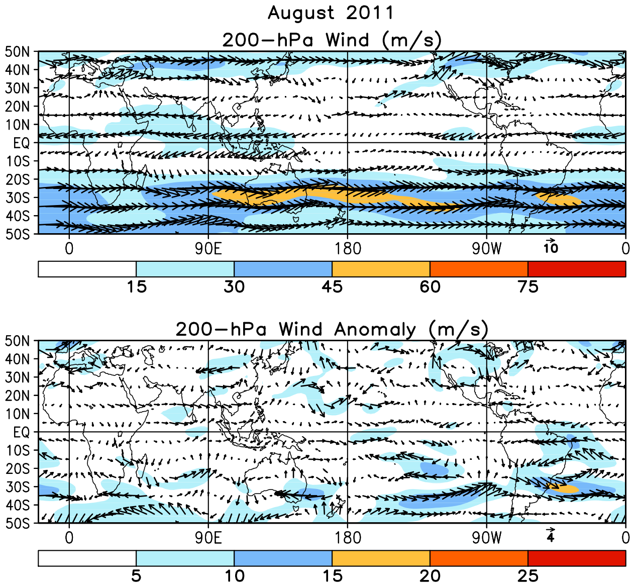
FIGURE T21. Mean (top) and anomalous (bottom) 200-hPa vector wind (CDAS/Reanalysis) for AUG 2011. Contour interval for isotachs is 15 \text{ ms}^{-1} (top) and 5 \text{ ms}^{-1} (bottom). Anomalies are departures from 1981-2010 base period monthly means.
