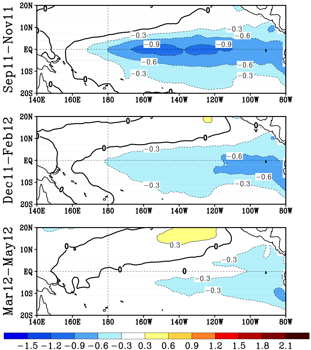
FIGURE F5. Predicted 3-month average sea surface temperature anomalies from the NCEP/CPC Markov model (Xue et al. 2000, J. Climate , 13 , 849-871). The forecast is initiated in AUG 2011 . Contour interval is 0.3C and negative anomalies are indicated by dashed contours. Anomalies are calculated relative to the 1971-2000 climatology.
