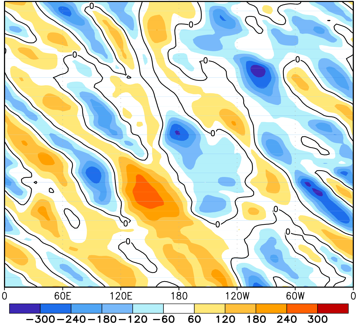
FIGURE E18. Southern Hemisphere: Daily 500-hPa height anomalies for AUG 2011 averaged over the 5° latitude band centered on 40°S. Positive values are indicated by solid contours and dark shading. Negative values are indicated by dashed contours and light shading. Contour interval is 60 m. Anomalies are departures from the 1981-2010 base period daily means.
