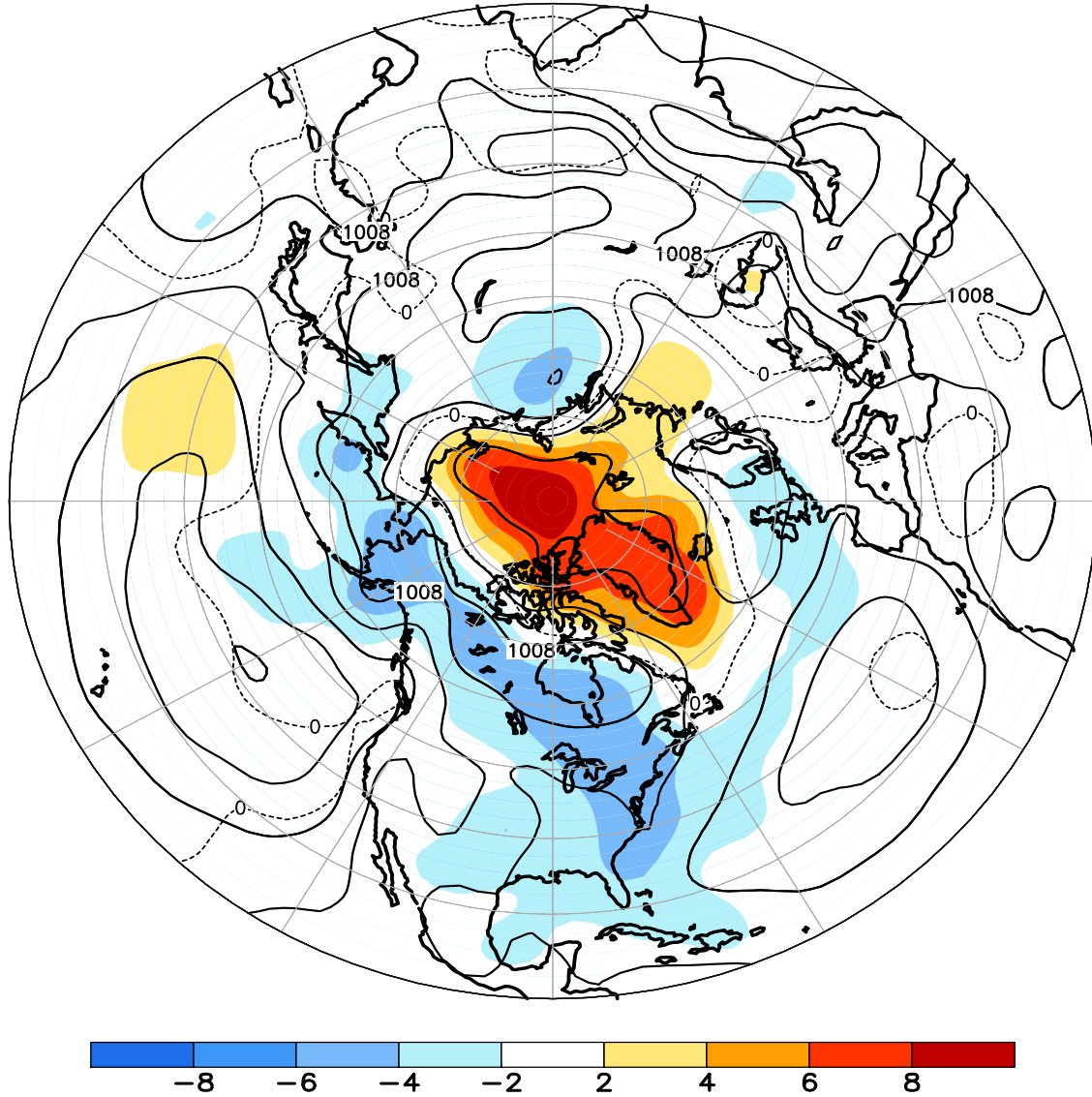
FIGURE E8. Northern Hemisphere mean and anomalous sea level pressure (CDAS/Reanalysis) for AUG 2011. Mean values are denoted by solid contours drawn at an interval of 4 hPa. Anomaly contour interval is 2 hPa with values less (greater) than -2 hPa (2 hPa) indicated by dark (light) shading. Anomalies are calculated as departures from the 1981-2010 base period monthly means.
