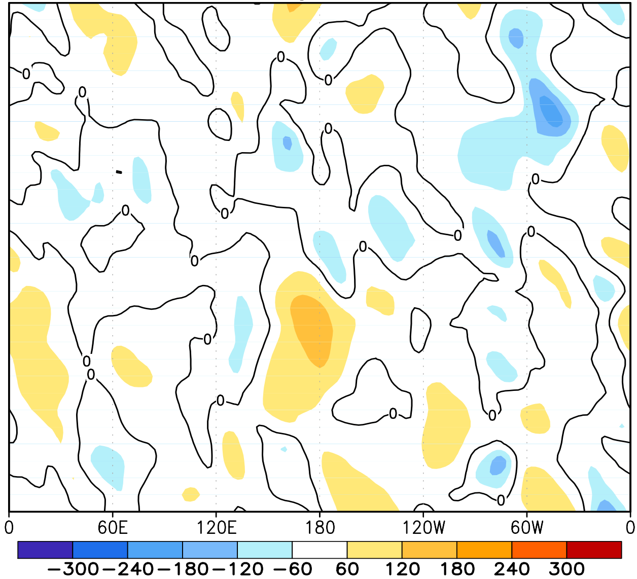
FIGURE E12. Northern Hemisphere: Daily 500-hPa height anomalies for AUG 2011 averaged over the 5° latitude band centered on 40°N. Positive values are indicated by solid contours and dark shading. Negative values are indicated by dashed contours and light shading. Contour interval is 60 m. Anomalies are departures from the 1981-2010 base period daily means.
