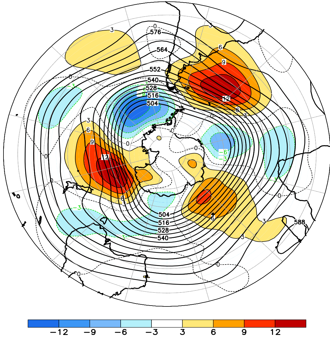
FIGURE E15. Southern Hemisphere mean and anomalous 500-hPa geopotential height (CDAS/Reanalysis) for AUG 2012. Mean heights are denoted by solid contours drawn at an interval of 6 dam. Anomaly contour interval is 3 dam with values less (greater) than -3 dam (3 dam) indicated by dark (light) shading. Anomalies are calculated as departures from the 1981-2010 base period monthly means.
