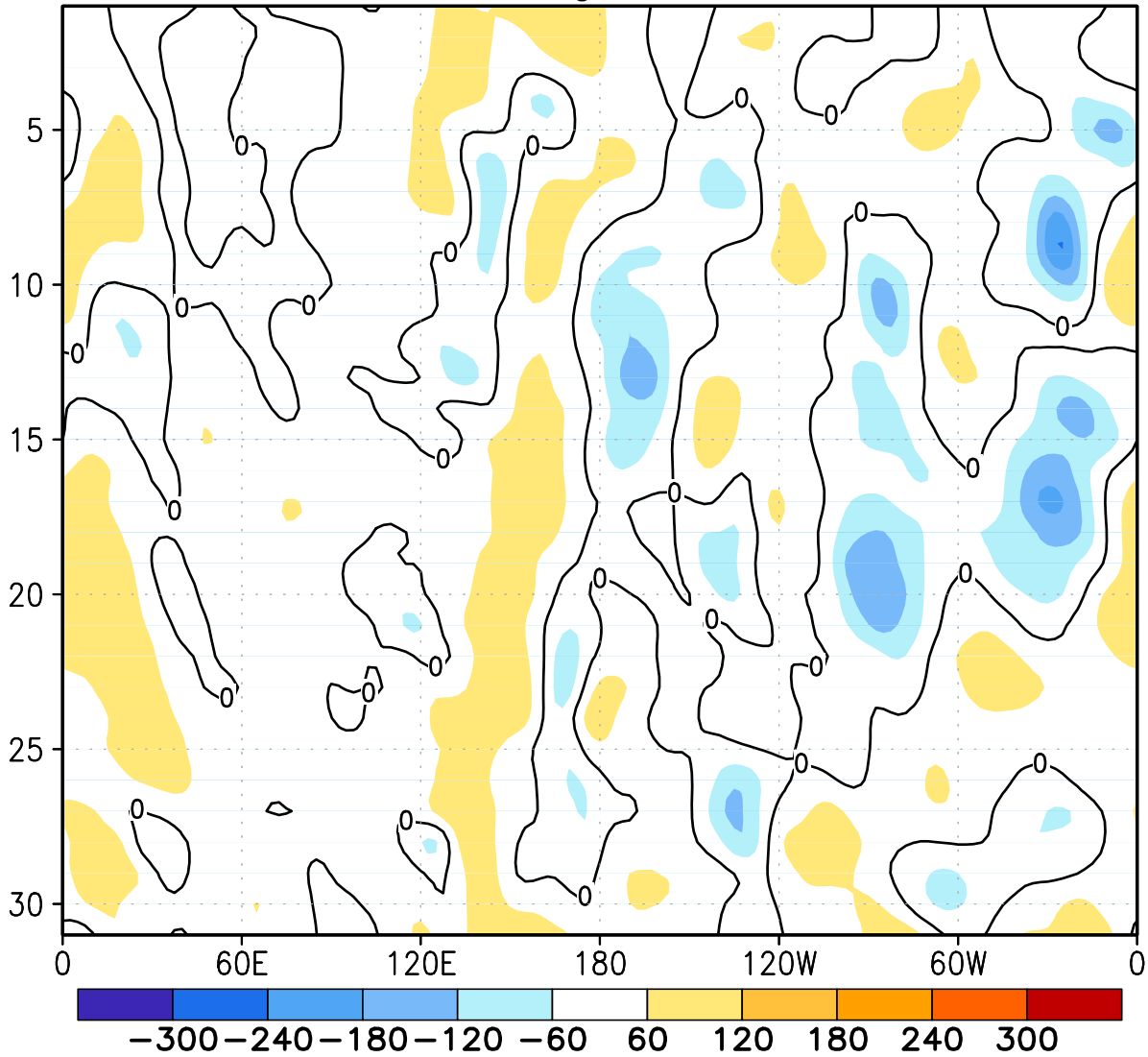
FIGURE E12. Northern Hemisphere: Daily 500-hPa height anomalies for AUG 2012 averaged over the 5° latitude band centered on 40°N. Positive values are indicated by solid contours and dark shading. Negative values are indicated by dashed contours and light shading. Contour interval is 60 m. Anomalies are departures from the 1981-2010 base period daily means.
