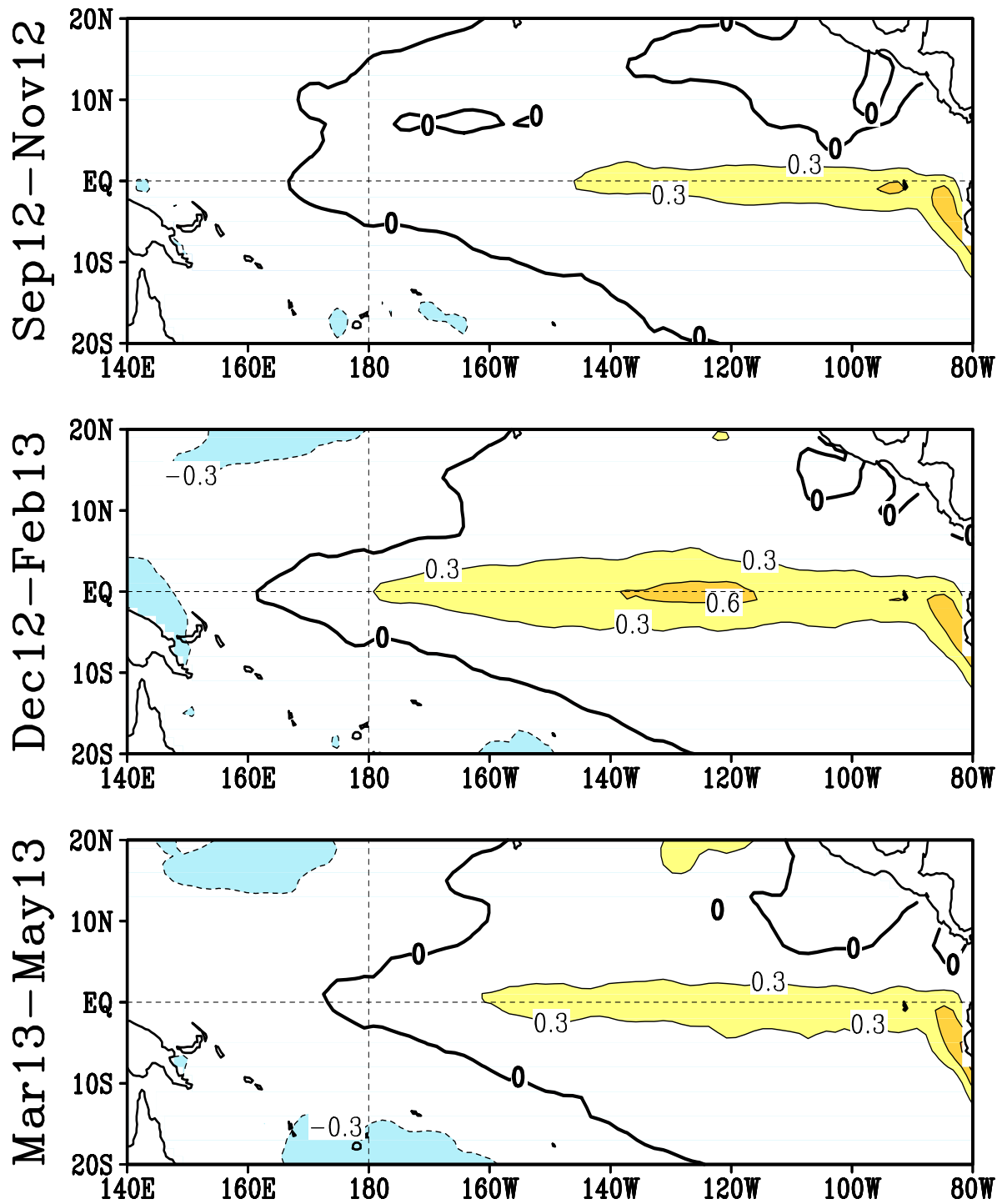
FIGURE F5. Predicted 3-month average sea surface temperature anomalies from the NCEP/CPC Markov model (Xue et al. 2000, J. Climate , 13 , 849-871). The forecast is initiated in AUG 2012. Contour interval is 0.3C and negative anomalies are indicated by dashed contours. Anomalies are calculated relative to the 1971-2000 climatology.
