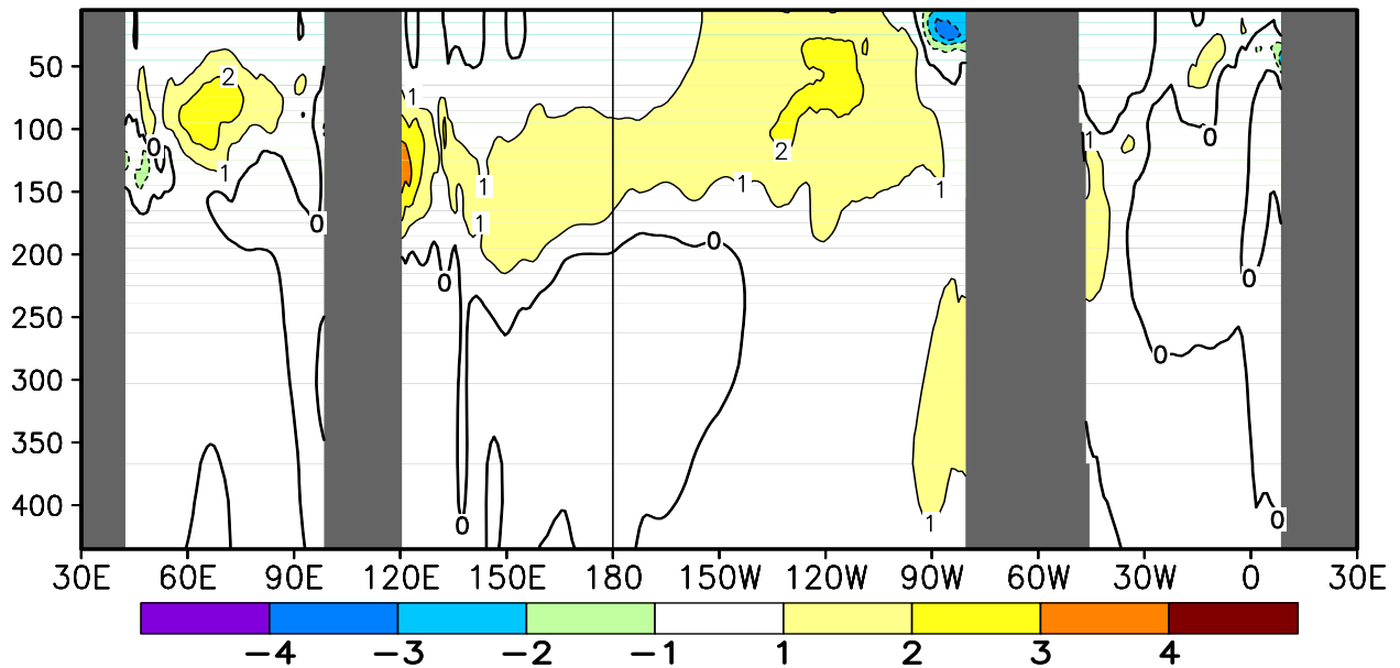
FIGURE T17. Equatorial depth–longitude section of ocean temperature (top) and ocean temperature anomalies (bottom) for AUG 2012. Contour interval is 1°C. Dashed contours in bottom panel indicate negative anomalies. Data are derived from the NCEP’s global ocean data assimilation system version 2 which assimilates oceanic observations into an oceanic GCM (Xue, Y. and Behringer, D.W., 2006: Operational global ocean data assimilation system at NCEP, to be submitted to BAMS). Anomalies are departures from the 1981–2010 base period means.
