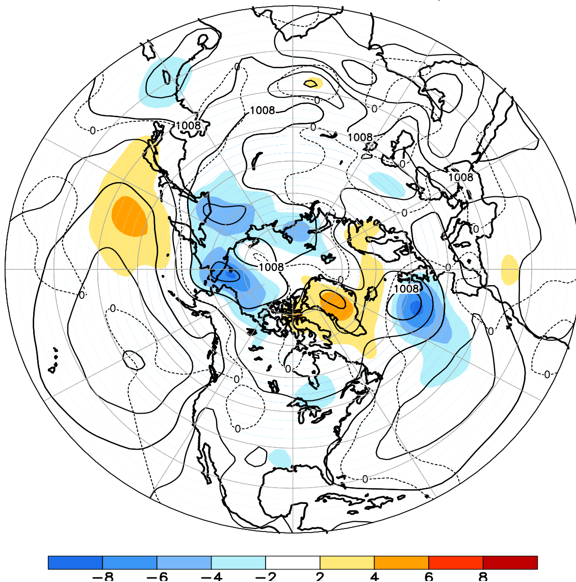
FIGURE E8. Northern Hemisphere mean and anomalous sea level pressure (CDAS/Reanalysis) for AUG 2012. Mean values are denoted by solid contours drawn at an interval of 4 hPa. Anomaly contour interval is 2 hPa with values less (greater) than -2 hPa (2 hPa) indicated by dark (light) shading. Anomalies are calculated as departures from the 1981-2010 base period monthly means.
