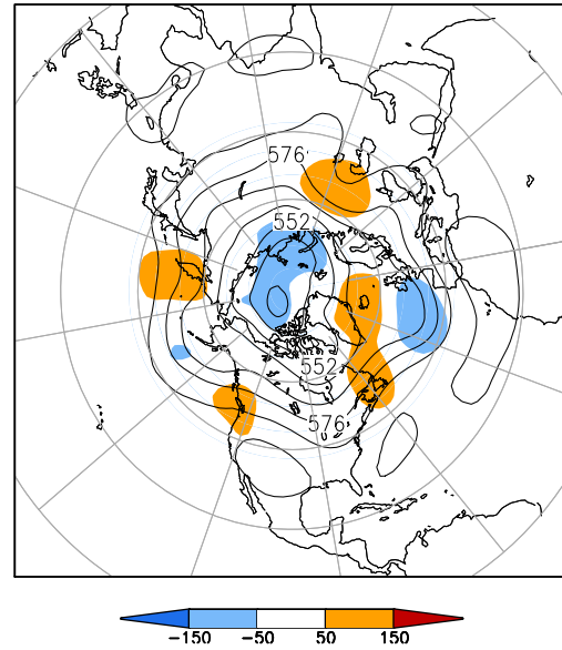
500-hPa Height (dm) & Anomalies (m) (Aug 1–15, 2012)
