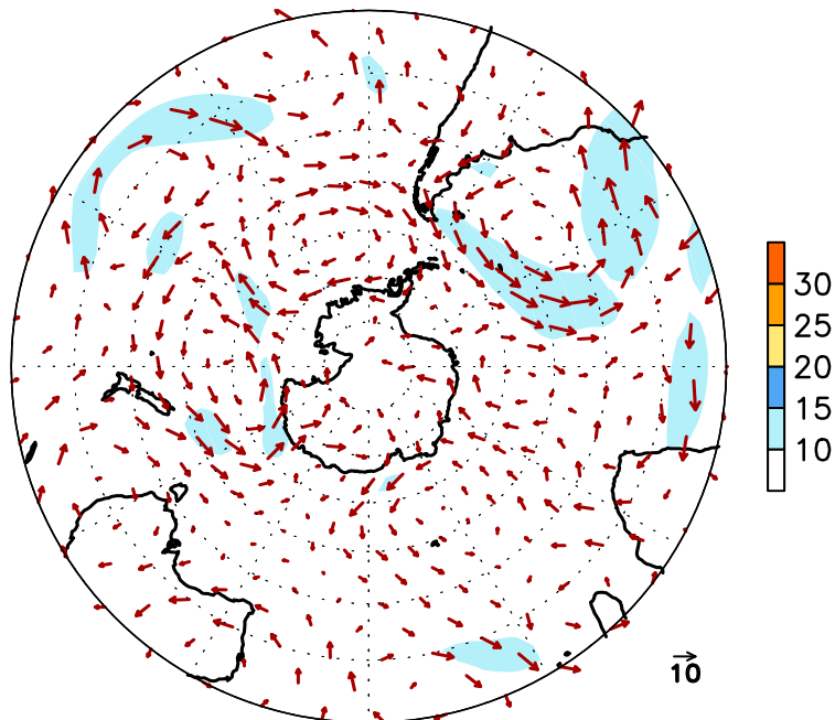
FIGURE E16. Southern Hemisphere mean (left) and anomalous (right) 300-hPa vector wind (CDAS/Reanalysis) for AUG 2012. Mean (anomaly) isotach contour interval is 10 (5) \text{ms}^{-1} . Values greater than 30 \text{ms}^{-1} (left) and 10 \text{ms}^{-1} (rights) are shaded. Anomalies are departures from the 1981-2010 base period monthly means.
