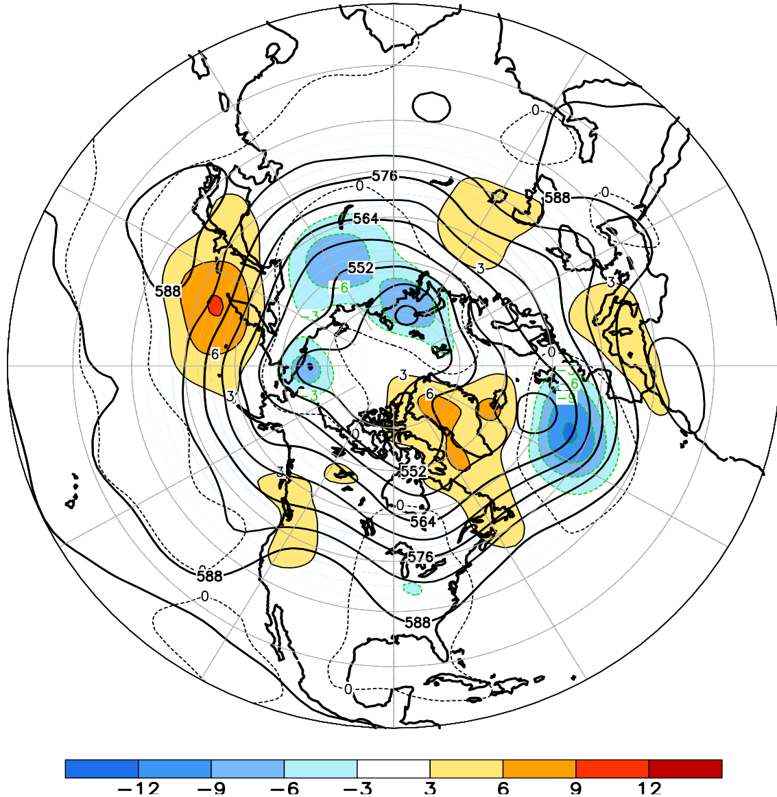
FIGURE E9. Northern Hemisphere mean and anomalous 500-hPa geopotential height (CDAS/Reanalysis) for AUG 2012. Mean heights are denoted by solid contours drawn at an interval of 6 dam. Anomaly contour interval is 3 dam with values less (greater) than -3 dam (3 dam) indicated by dark (light) shading. Anomalies are calculated as departures from the 1981-2010 base period monthly means.
