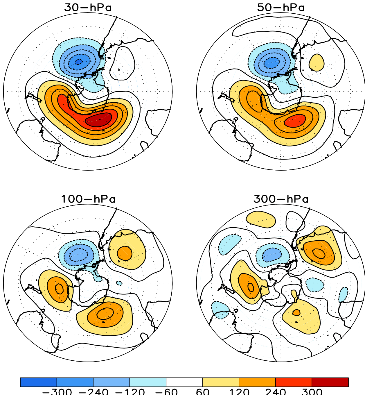
FIGURE S1. Stratospheric height anomalies (m) at selected levels for AUG 2012. Positive values are indicated by solid contours and dark shading. Negative values are indicated by dashed contours and light shading. Contour interval is 60 m. Anomalies are calculated from the 1981-2010 base period means. Winter Hemisphere is shown.
