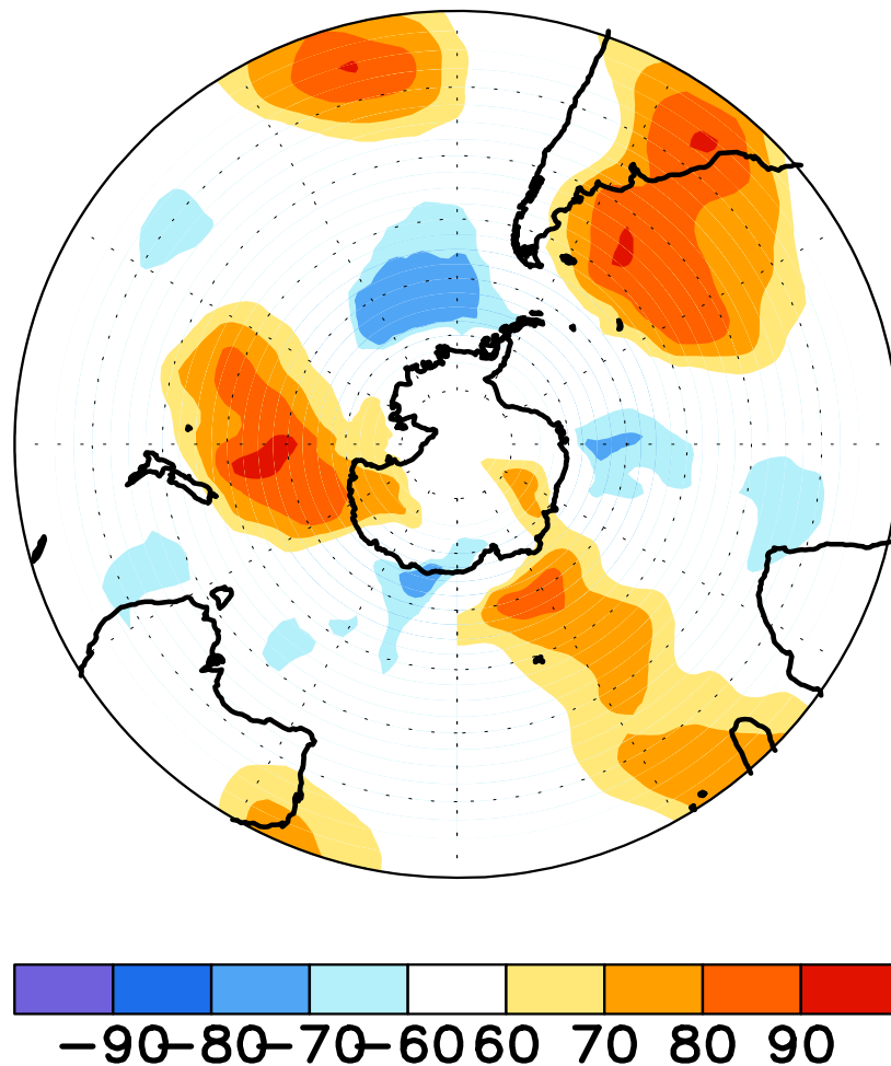
FIGURE E17. Southern Hemisphere percentage of days during AUG 2012 in which 500-hPa height anomalies greater than 15 m (red) and less than -15 m (blue) were observed. Values greater than 70% are shaded and contour in-
