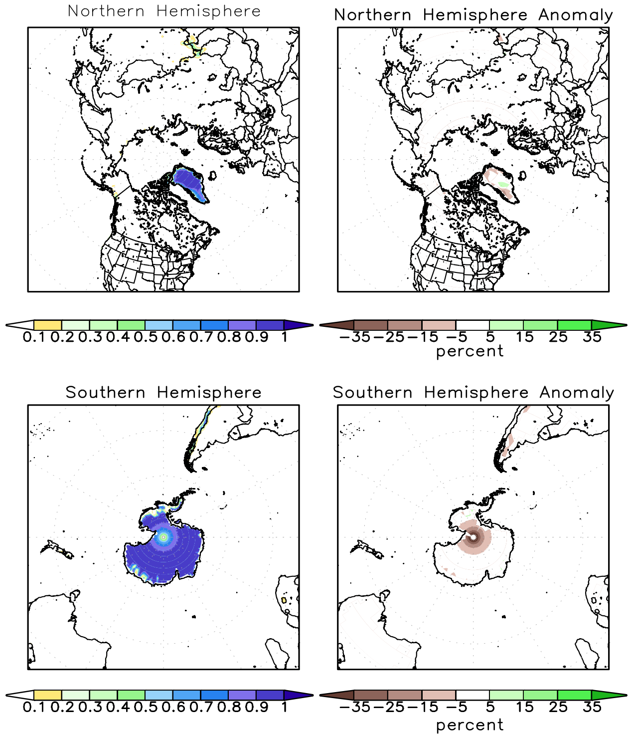
FIGURE A2.2. SSM/I derived snow cover frequency (%) (left) and snow cover anomaly (%) (right) for the month of AUG 2012 based on 1987 - 2010 base period for the Northern Hemisphere (top) and Southern Hemisphere (bottom). It is generated using the algorithm described by Ferraro et. al, 1996, Bull. Amer. Meteor. Soc., vol 77, 891-905.
