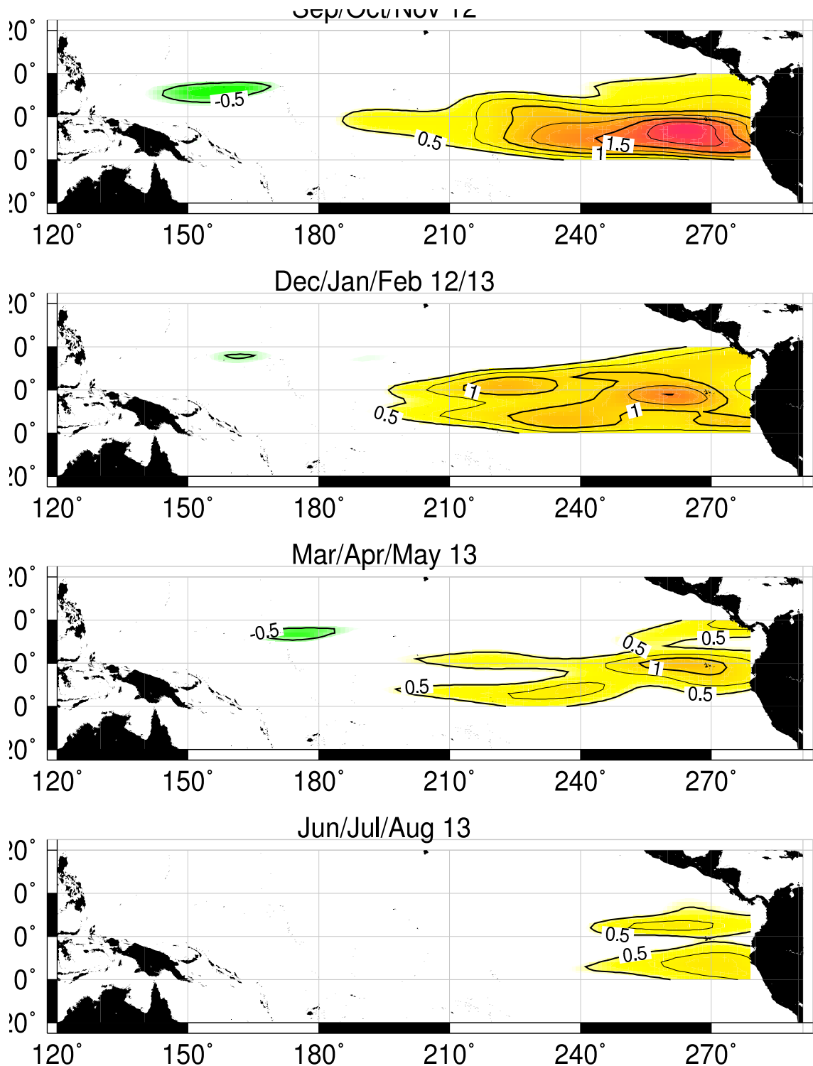
FIGURE F11. SST anomaly forecast for the equatorial Pacific from the Hybrid Coupled Model (HCM) developed by the Scripps Institution of Oceanography and the Max-Plank Institut fuer Meteorologie.
