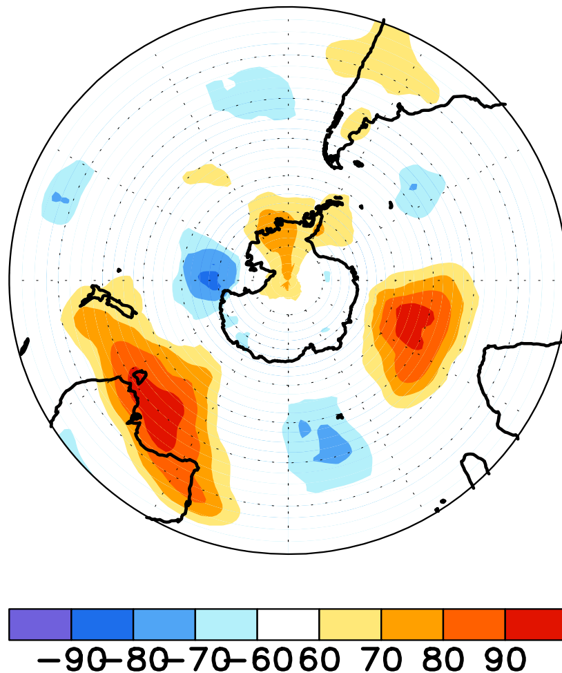
FIGURE E17. Southern Hemisphere percentage of days during AUG 2014 in which 500-hPa height anomalies greater than 15 m (red) and less than -15 m (blue) were observed. Values greater than 70% are shaded and contour in-
