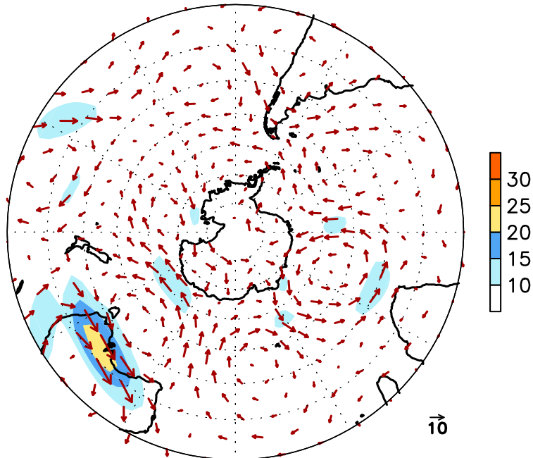
FIGURE E16. Southern Hemisphere mean (left) and anomalous (right) 300-hPa vector wind (CDAS/Reanalysis) for AUG 2014. Mean (anomaly) isotach contour interval is 10 (5) \text{ms}^{-1} . Values greater than 30 \text{ ms}^{-1} (left) and 10 \text{ ms}^{-1} (rights) are shaded. Anomalies are departures from the 1981-2010 base period monthly means.
