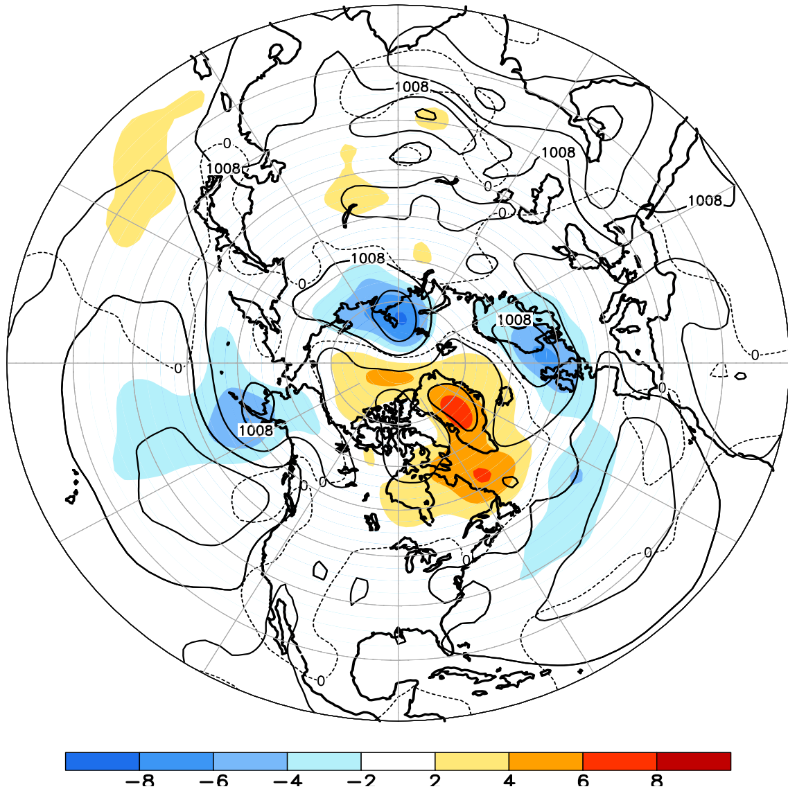
FIGURE E8. Northern Hemisphere mean and anomalous sea level pressure (CDAS/Reanalysis) for AUG 2014. Mean values are denoted by solid contours drawn at an interval of 4 hPa. Anomaly contour interval is 2 hPa with values less (greater) than -2 hPa (2 hPa) indicated by dark (light) shading. Anomalies are calculated as departures from the 1981-2010 base period monthly means.
