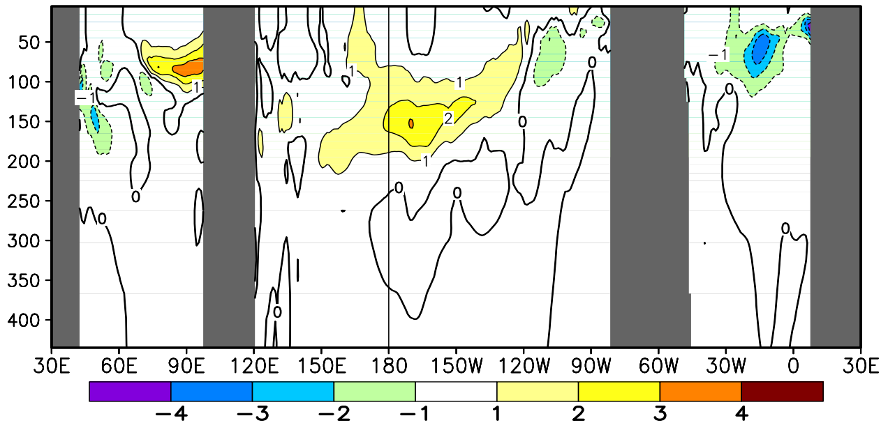
FIGURE T17. Equatorial depth–longitude section of ocean temperature (top) and ocean temperature anomalies (bottom) for AUG 2014. Contour interval is 1°C. Dashed contours in bottom panel indicate negative anomalies. Data are derived from the NCEP’s global ocean data assimilation system version 2 which assimilates oceanic observations into an oceanic GCM (Xue, Y. and Behringer, D.W., 2006: Operational global ocean data assimilation system at NCEP, to be submitted to BAMS). Anomalies are departures from the 1981–2010 base period means.
