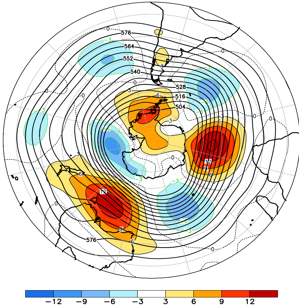
FIGURE E15. Southern Hemisphere mean and anomalous 500-hPa geopotential height (CDAS/Reanalysis) for AUG 2014. Mean heights are denoted by solid contours drawn at an interval of 6 dam. Anomaly contour interval is 3 dam with values less (greater) than -3 dam (3 dam) indicated by dark (light) shading. Anomalies are calculated as departures from the 1981-2010 base period monthly means.
