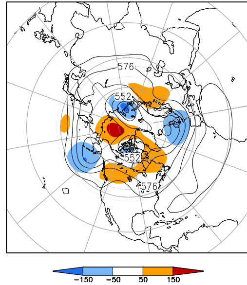
500-hPa Height (dm) & Anomalies (m) (Aug 1–15, 2014)
