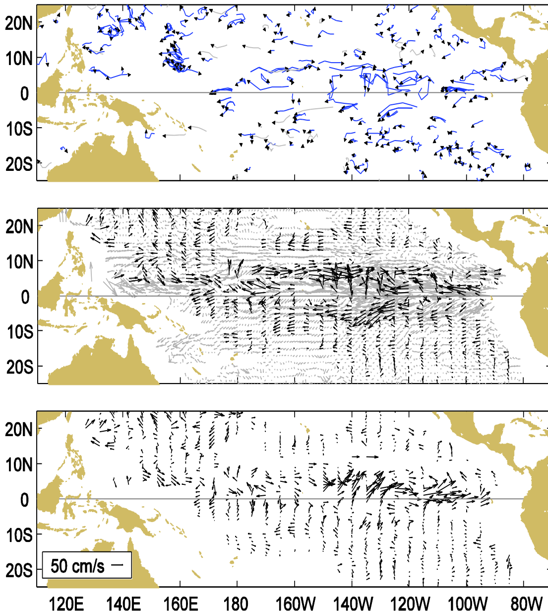
Figure A1.1 Top: Movements of drifting buoys in the tropical Pacific Ocean during August 2014. The linear segments of each trajectory represent a one week displacement. Trajectories of buoys which have lost their subsurface drogues are gray; those with drogues are black.
