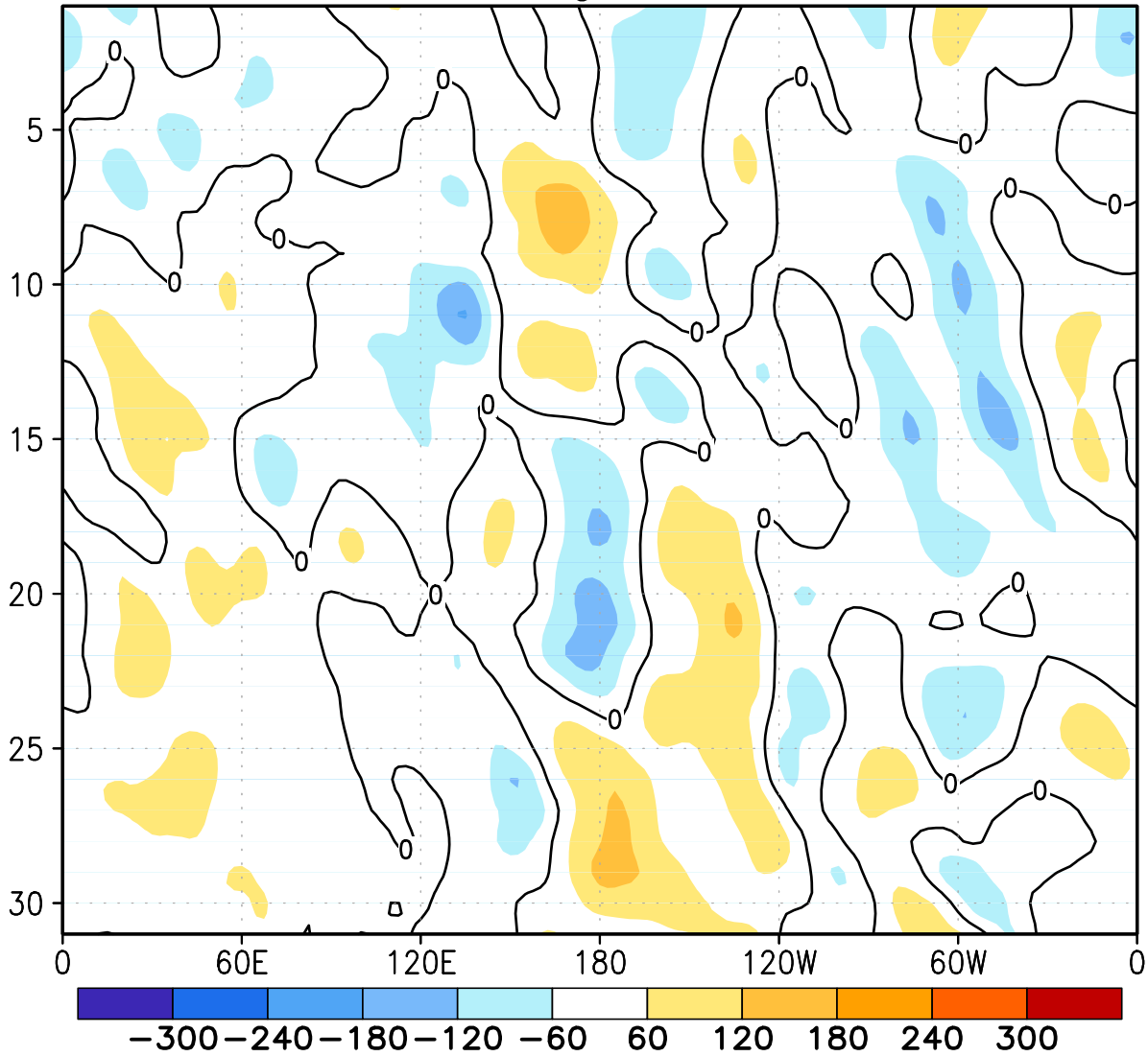
FIGURE E12. Northern Hemisphere: Daily 500-hPa height anomalies for AUG 2014 averaged over the 5° latitude band centered on 40°N. Positive values are indicated by solid contours and dark shading. Negative values are indicated by dashed contours and light shading. Contour interval is 60 m. Anomalies are departures from the 1981-2010 base period daily means.
