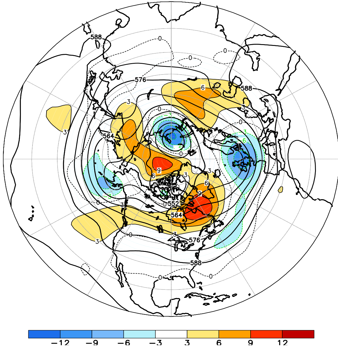
FIGURE E9. Northern Hemisphere mean and anomalous 500-hPa geopotential height (CDAS/Reanalysis) for AUG 2014. Mean heights are denoted by solid contours drawn at an interval of 6 dam. Anomaly contour interval is 3 dam with values less (greater) than -3 dam (3 dam) indicated by dark (light) shading. Anomalies are calculated as departures from the 1981-2010 base period monthly means.
