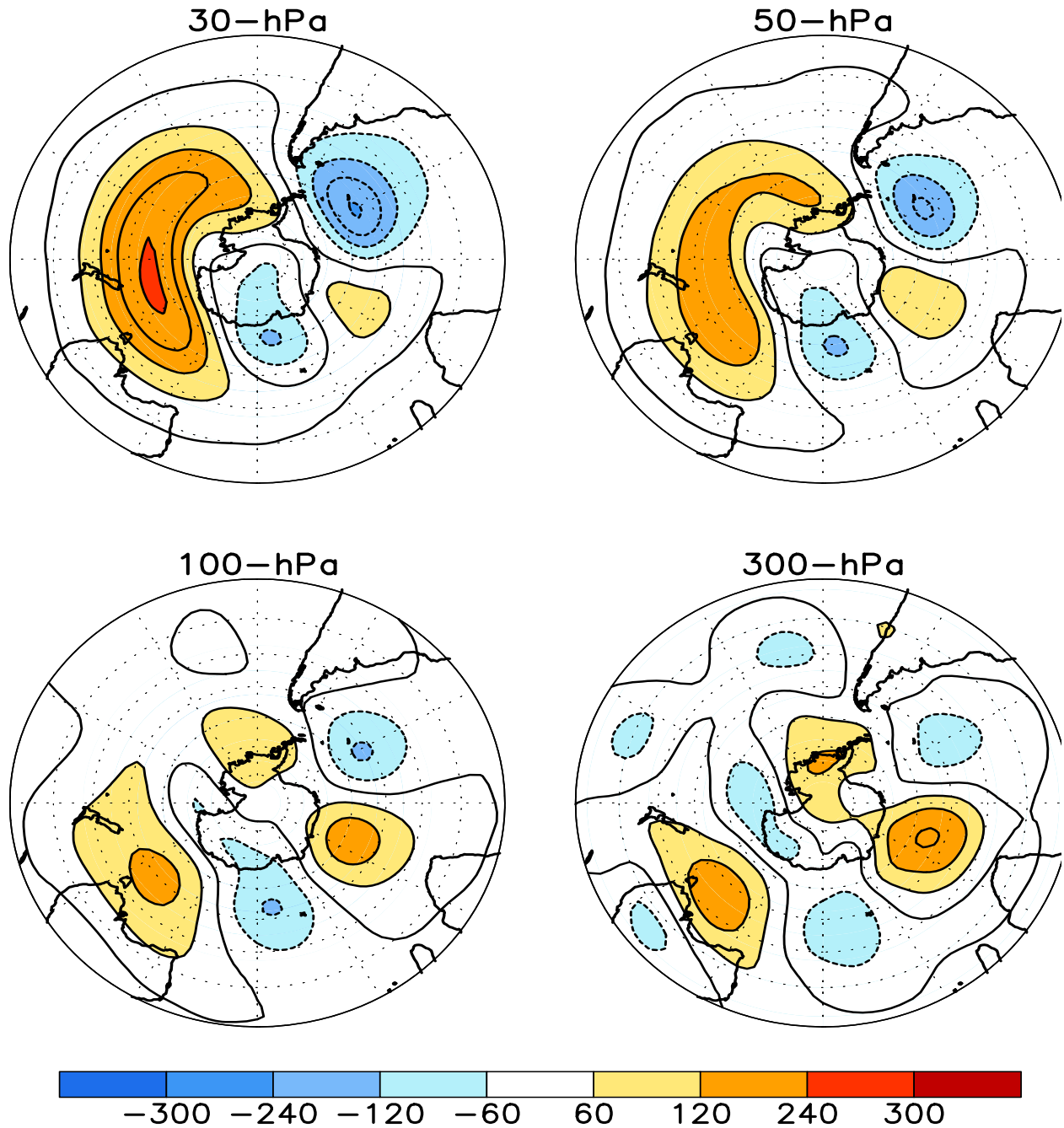
FIGURE S1. Stratospheric height anomalies (m) at selected levels for AUG 2014. Positive values are indicated by solid contours and dark shading. Negative values are indicated by dashed contours and light shading. Contour interval is 60 m. Anomalies are calculated from the 1981-2010 base period means. Winter Hemisphere is shown.
