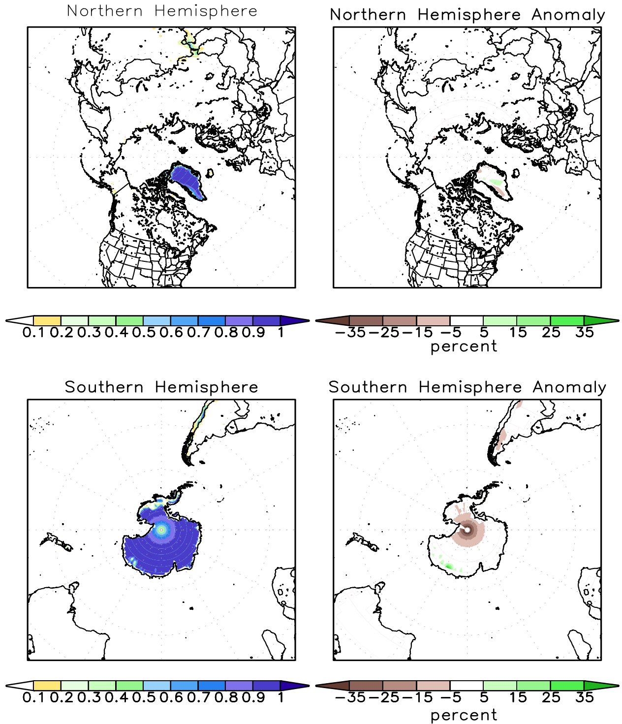
FIGURE A2.2. SSM/I derived snow cover frequency (%) (left) and snow cover anomaly (%) (right) for the month of AUG 2014 based on 1987 - 2010 base period for the Northern Hemisphere (top) and Southern Hemisphere (bottom). It is generated using the algorithm described by Ferraro et. al, 1996, Bull. Amer. Meteor. Soc., vol 77, 891-905.
