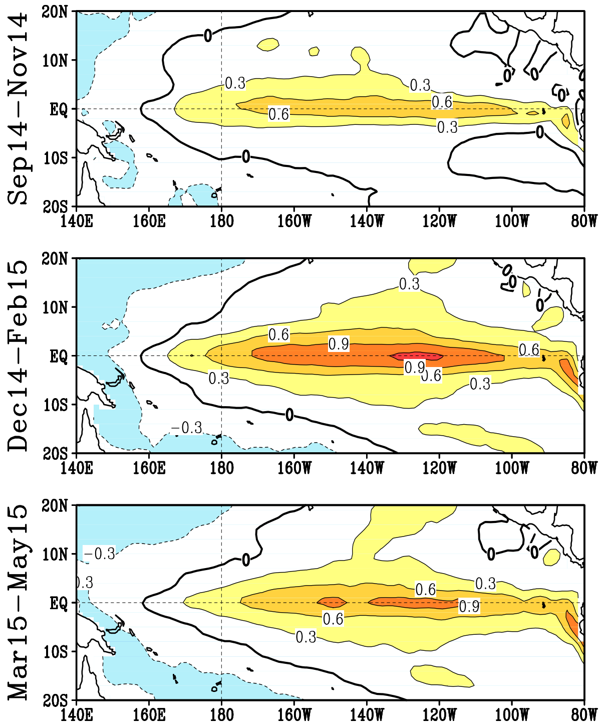
FIGURE F5. Predicted 3-month average sea surface temperature anomalies from the NCEP/CPC Markov model (Xue et al. 2000, J. Climate , 13 , 849-871). The forecast is initiated in AUG 2014 . Contour interval is 0.3C and negative anomalies are indicated by dashed contours. Anomalies are calculated relative to the 1971-2000 climatology.
