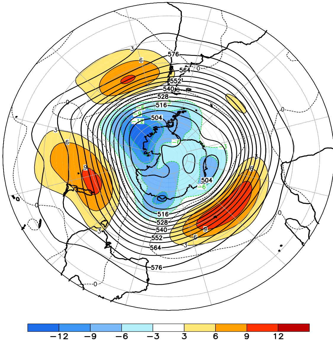
FIGURE E15. Southern Hemisphere mean and anomalous 500-hPa geopotential height (CDAS/Reanalysis) for DEC 2007. Mean heights are denoted by solid contours drawn at an interval of 8 dam. Anomaly contour interval is 3 dam with values less (greater) than -3 dam (3 dam) indicated by dark (light) shading. Anomalies are calculated as departures from the 1979-95 base period monthly means.
