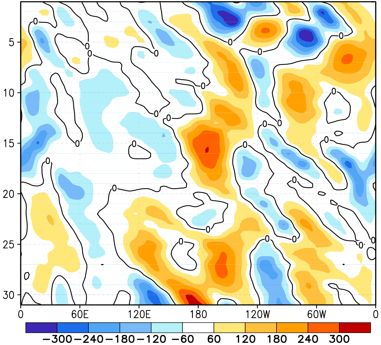
FIGURE E12. Northern Hemisphere: Daily 500-hPa height anomalies for DEC 2007 averaged over the 5° latitude band centered on 40°N. Positive values are indicated by solid contours and dark shading. Negative values are indicated by dashed contours and light shading. Contour interval is 60 m. Anomalies are departures from the 1979-95 base period daily means.
