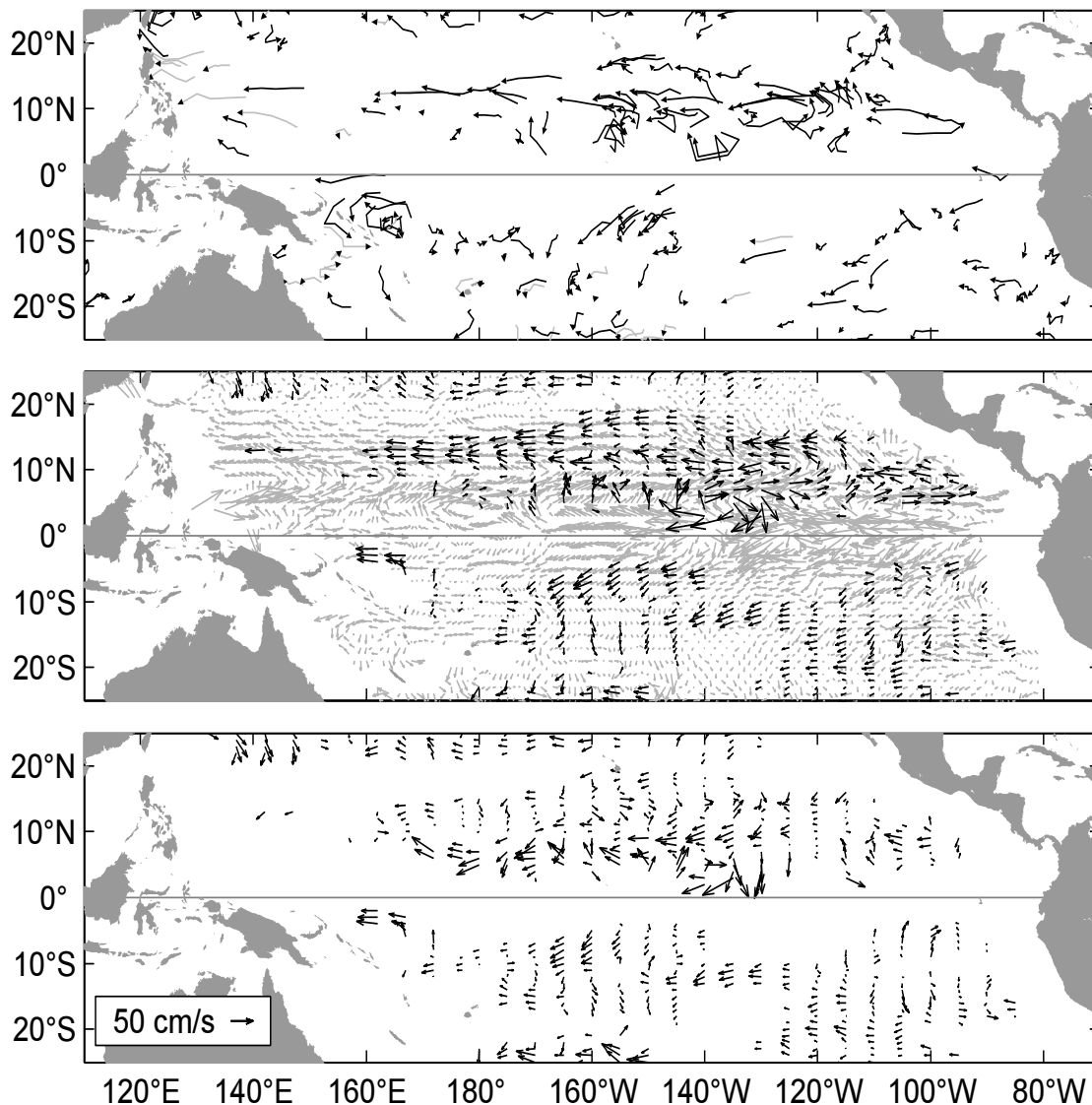
Figure A1.1 Top: Movements of drifting buoys in the tropical Pacific Ocean during December 2007. The linear segments of each trajectory represent a one week displacement. Trajectories of buoys which have lost their subsurface drogues are gray; those with drogues are black. Middle: Monthly mean currents calculated from all buoys 1993-2002 (gray), and currents measured by the drogued buoys this month (black) smoothed by an optimal filter. Bottom: Anomalies from the climatological monthly mean currents for this month.
