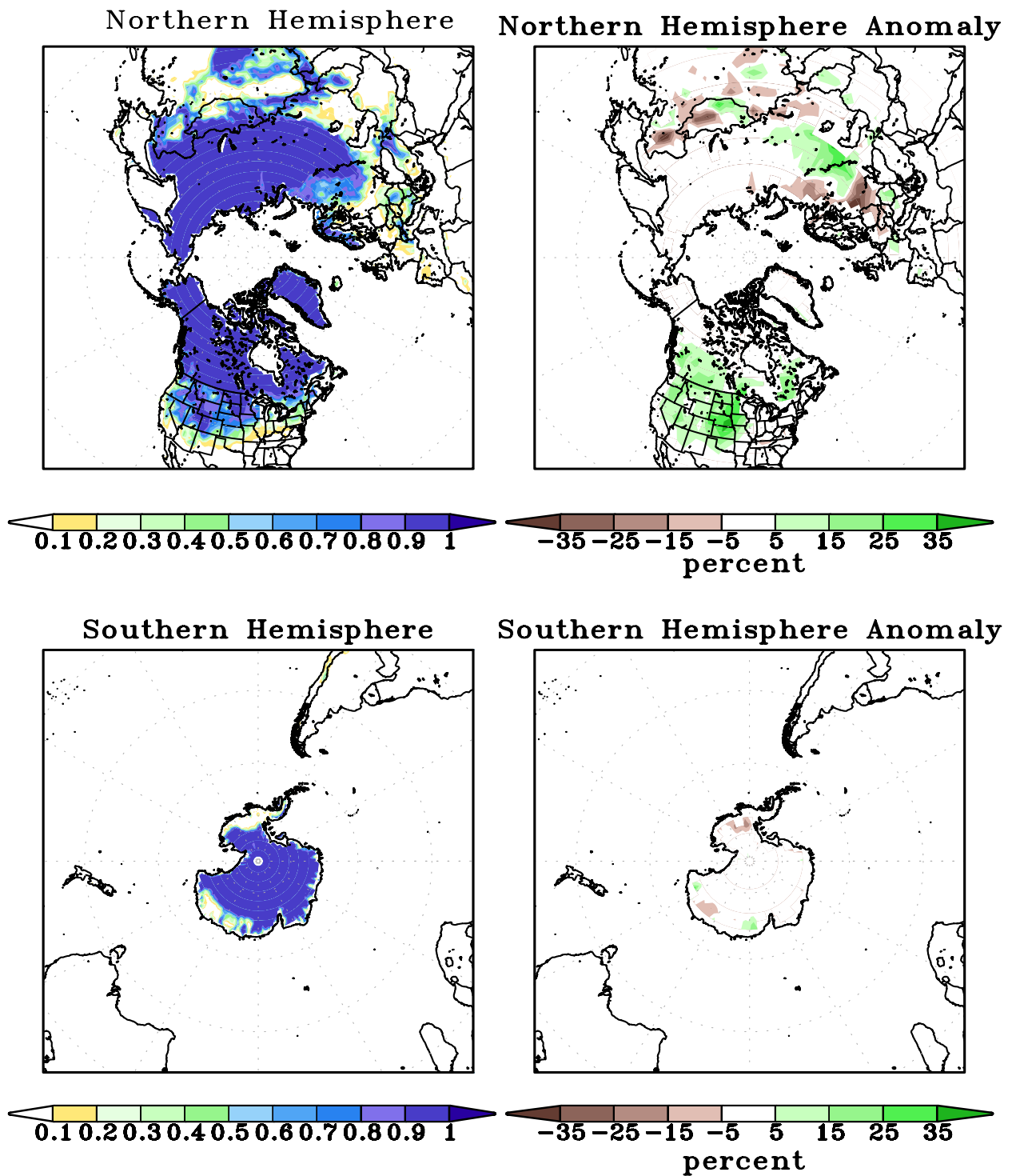
FIGURE A2.2. SSM/I derived snow cover frequency (%) (left) and snow cover anomaly (%) (right) for the month of DEC 2007 based on 1987 - 2006 base period for the Northern Hemisphere (top) and Southern Hemisphere (bottom). It is generated using the algorithm described by Ferraro et. al, 1996, Bull. Amer. Meteor. Soc., vol 77, 891-905.
