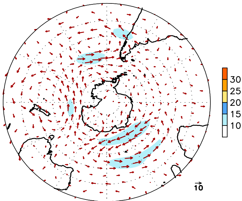
FIGURE E16. Southern Hemisphere mean (left) and anomalous (right) 300-hPa vector wind (CDAS/Reanalysis) for DEC 2007. Mean (anomaly) isotach contour interval is 10 (5) \text{ms}^{-1} . Values greater than 30 \text{ms}^{-1} (left) and 10 \text{ms}^{-1} (rights) are shaded. Anomalies are departures from the 1979-95 base period monthly means.
