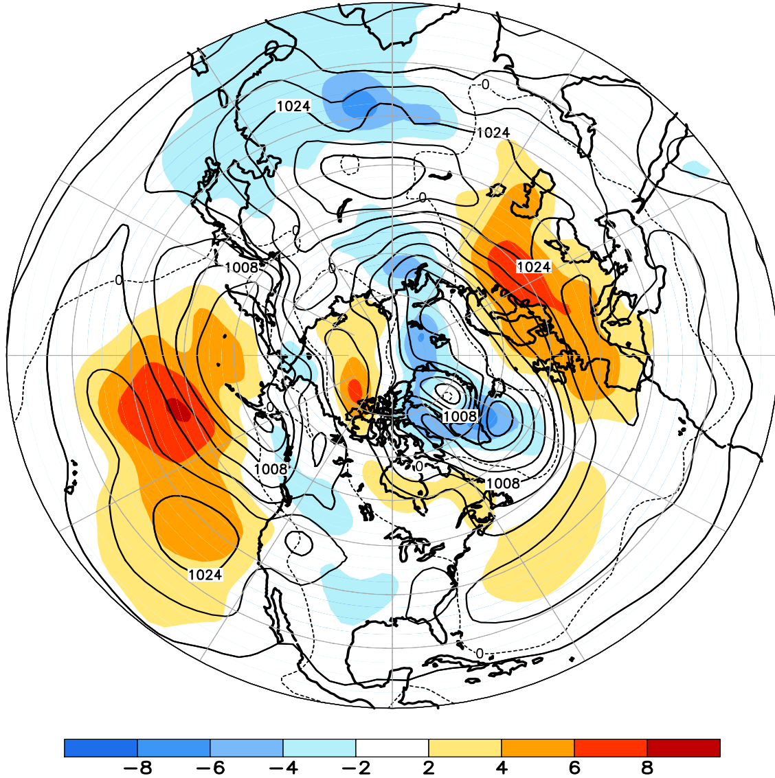
FIGURE E8. Northern Hemisphere mean and anomalous sea level pressure (CDAS/Reanalysis) for DEC 2007. Mean values are denoted by solid contours drawn at an interval of 4 hPa. Anomaly contour interval is 2 hPa with values less (greater) than -2 hPa (2 hPa) indicated by dark (light) shading. Anomalies are calculated as departures from the 1979-95 base period monthly means.
