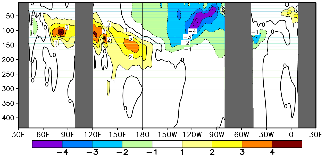
FIGURE T17. Equatorial depth–longitude section of ocean temperature (top) and ocean temperature anomalies (bottom) for DEC 2007. Contour interval is 1°C. Dashed contours in bottom panel indicate negative anomalies. Data are derived from the NCEP’s global ocean data assimilation system version 2 which assimilates oceanic observations into an oceanic GCM (Xue, Y. and Behringer, D.W., 2006: Operational global ocean data assimilation system at NCEP, to be submitted to BAMS). Anomalies are departures from the 1982–2004 base period means.
