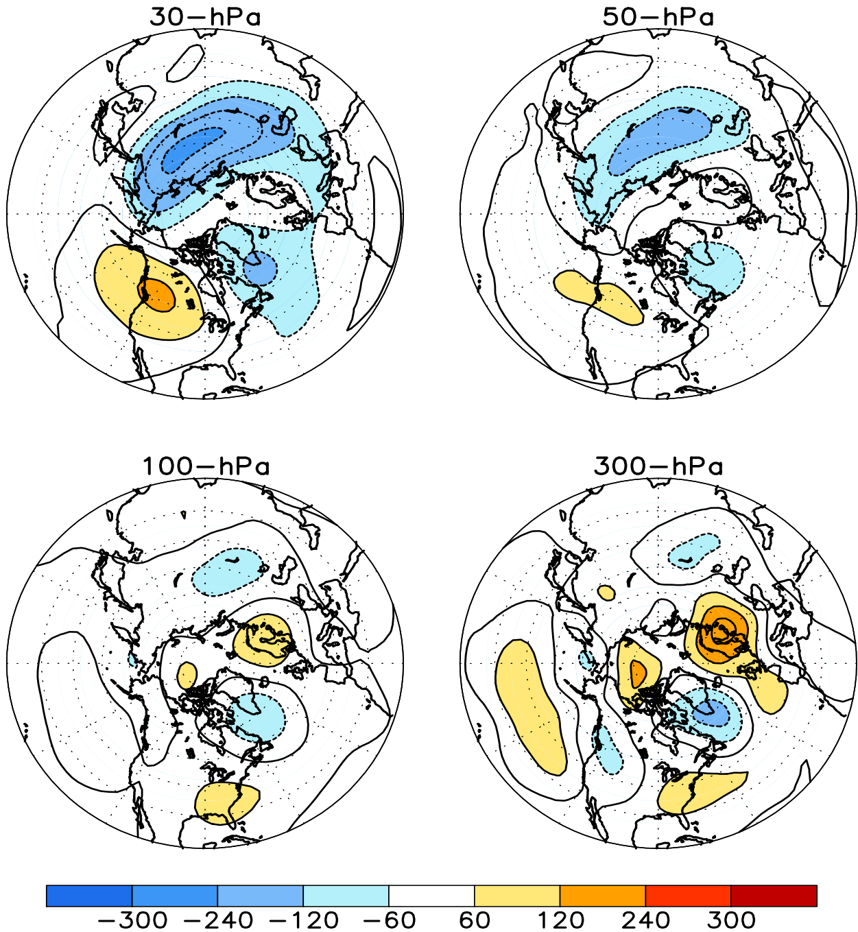
FIGURE S1. Stratospheric height anomalies (m) at selected levels for DEC 2007. Positive values are indicated by solid contours and dark shading. Negative values are indicated by dashed contours and light shading. Contour interval is 60 m. Anomalies are calculated from the 1979–95 base period means. Winter Hemisphere is shown.
