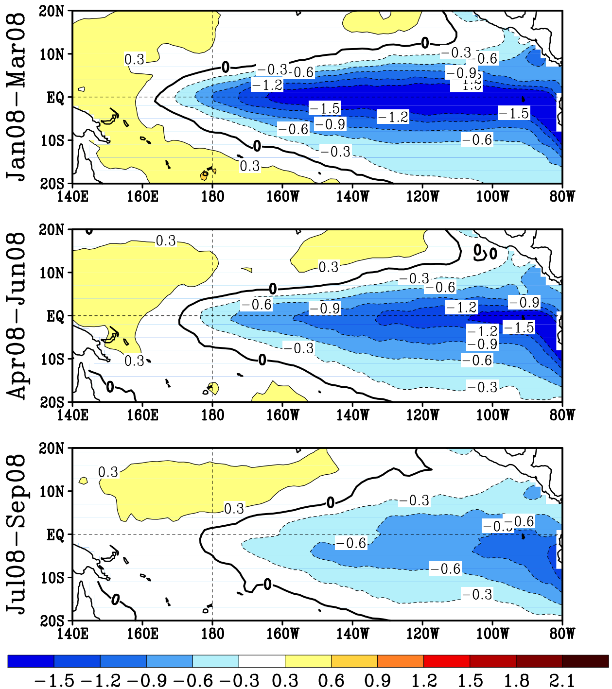
FIGURE F5. Predicted 3-month average sea surface temperature anomalies from the NCEP/CPC Markov model (Xue et al. 2000, J. Climate , 13 , 849-871). The forecast is initiated in DEC 2007 . Contour interval is 0.3C and negative anomalies are indicated by dashed contours. Anomalies are calculated relative to the 1971-2000 climatology.
