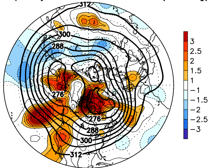
FIGURE E13. Northern Hemisphere: 700-hPa heights for DEC 2007 overlaid with standard deviation of high-pass filtered height (left) and normalized anomalous variance of high-pass filtered height (right). Heights are indicated by thick solid contours in both panels (interval is 60 m). High-pass filtered fields reflect fluctuations having periods less than 10 days, and are indicated by thin contours and shading. Contour interval for standard deviation is 15 m with values > 45 m shaded. Contour interval for normalized variance is 1 standard deviation, with positive values shown by solid contours and dark shading and negative values shown by dashed contours and light shading. Anomalies are departures from the 1964-93 base period monthly means.
