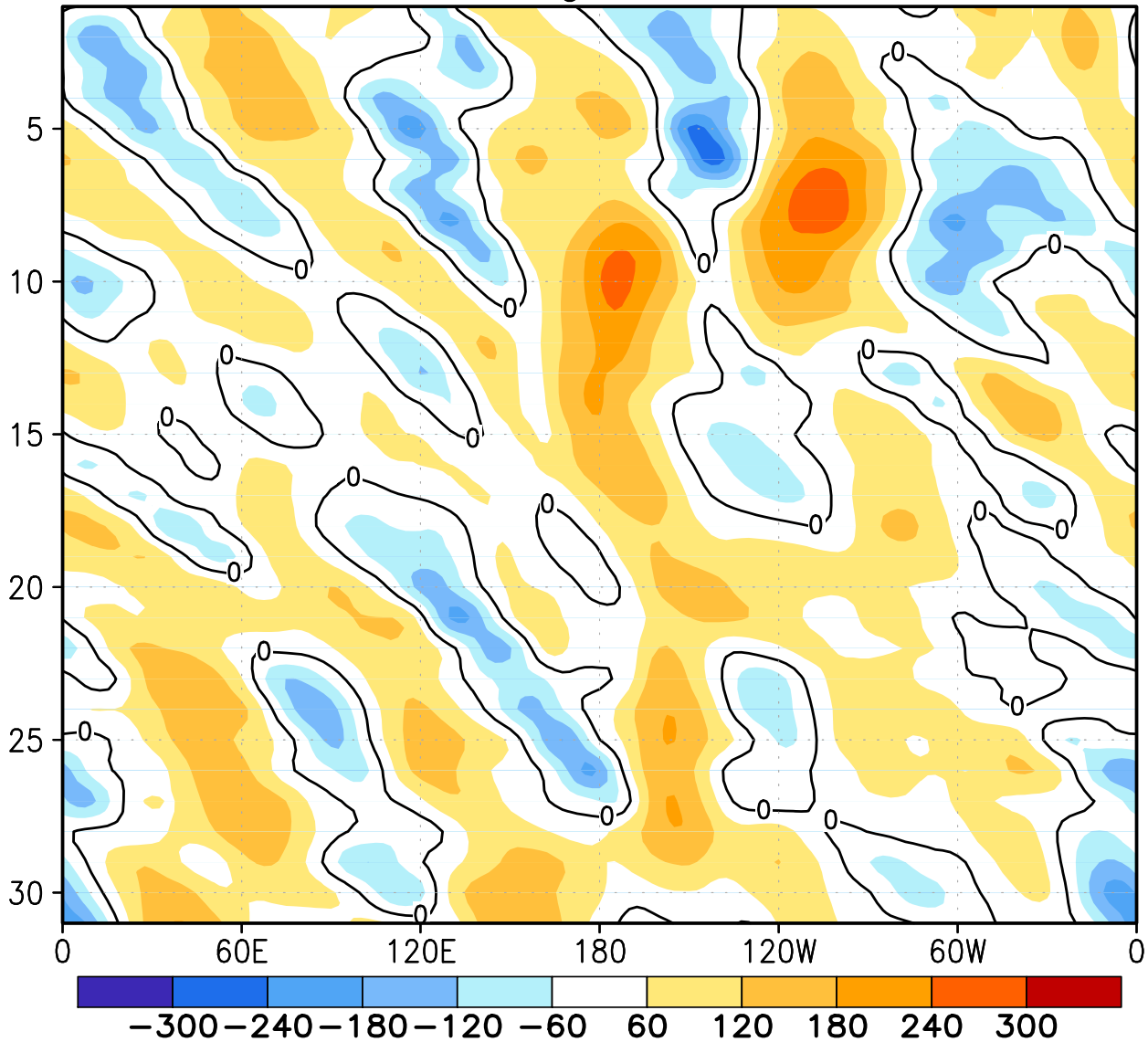
FIGURE E18. Southern Hemisphere: Daily 500-hPa height anomalies for DEC 2007 averaged over the 5° latitude band centered on 40°S. Positive values are indicated by solid contours and dark shading. Negative values are indicated by dashed contours and light shading. Contour interval is 60 m. Anomalies are departures from the 1979-95 base period daily means.
