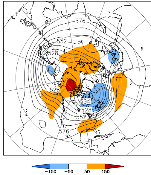
500-hPa Height (dm) & Anomalies (m) (Dec 1–15, 2007)
