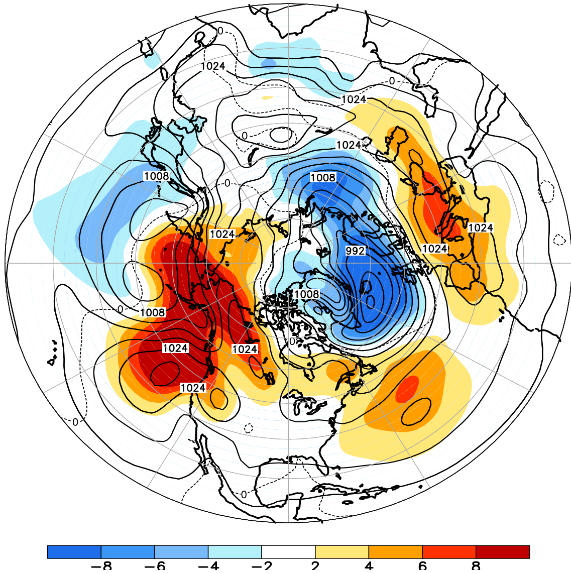
FIGURE E8. Northern Hemisphere mean and anomalous sea level pressure (CDAS/Reanalysis) for DEC 2013. Mean values are denoted by solid contours drawn at an interval of 4 hPa. Anomaly contour interval is 2 hPa with values less (greater) than -2 hPa (2 hPa) indicated by dark (light) shading. Anomalies are calculated as departures from the 1981-2010 base period monthly means.
