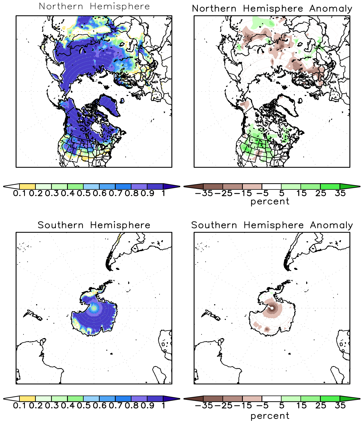
FIGURE A2.2. SSM/I derived snow cover frequency (%) (left) and snow cover anomaly (%) (right) for the month of DEC 2013 based on 1987 - 2010 base period for the Northern Hemisphere (top) and Southern Hemisphere (bottom). It is generated using the algorithm described by Ferraro et. al, 1996, Bull. Amer. Meteor. Soc., vol 77, 891-905.
