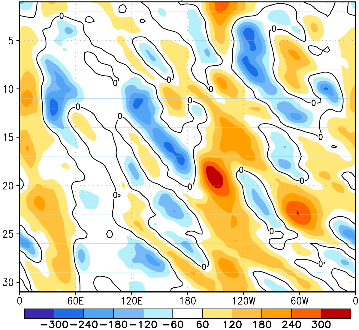
FIGURE E12. Northern Hemisphere: Daily 500-hPa height anomalies for DEC 2013 averaged over the 5° latitude band centered on 40°N. Positive values are indicated by solid contours and dark shading. Negative values are indicated by dashed contours and light shading. Contour interval is 60 m. Anomalies are departures from the 1981-2010 base period daily means.
