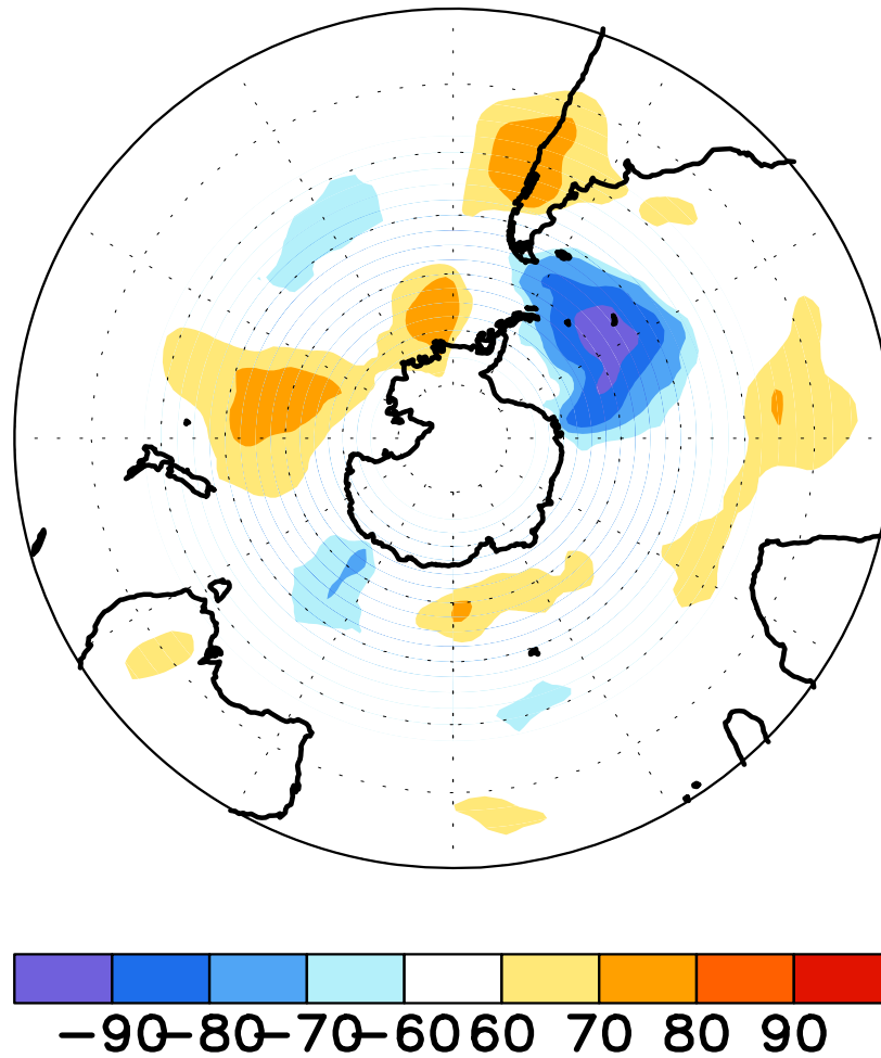
FIGURE E17. Southern Hemisphere percentage of days during DEC 2013 in which 500-hPa height anomalies greater than 15 m (red) and less than -15 m (blue) were observed. Values greater than 70% are shaded and contour in-
