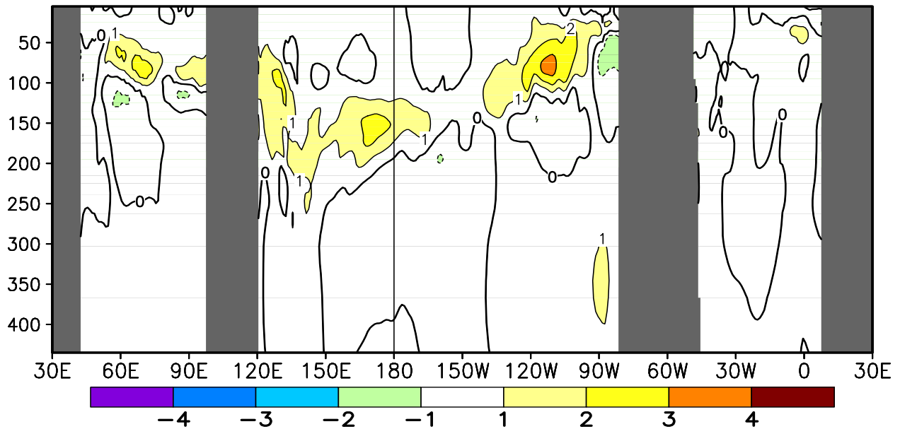
FIGURE T17. Equatorial depth–longitude section of ocean temperature (top) and ocean temperature anomalies (bottom) for DEC 2013. Contour interval is 1°C. Dashed contours in bottom panel indicate negative anomalies. Data are derived from the NCEP’s global ocean data assimilation system version 2 which assimilates oceanic observations into an oceanic GCM (Xue, Y. and Behringer, D.W., 2006: Operational global ocean data assimilation system at NCEP, to be submitted to BAMS). Anomalies are departures from the 1981–2010 base period means.
