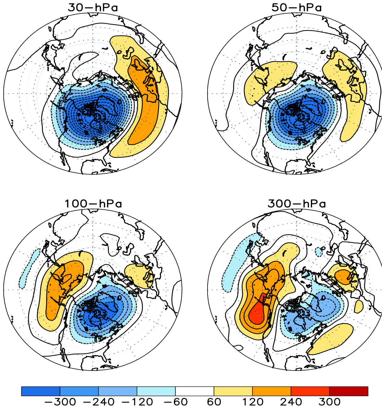
FIGURE S1. Stratospheric height anomalies (m) at selected levels for DEC 2013. Positive values are indicated by solid contours and dark shading. Negative values are indicated by dashed contours and light shading. Contour interval is 60 m. Anomalies are calculated from the 1981-2010 base period means. Winter Hemisphere is shown.
