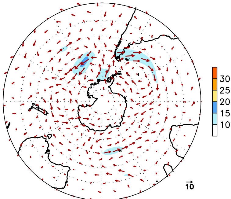
FIGURE E16. Southern Hemisphere mean (left) and anomalous (right) 300-hPa vector wind (CDAS/Reanalysis) for DEC 2013. Mean (anomaly) isotach contour interval is 10 (5) \text{ms}^{-1} . Values greater than 30 \text{ms}^{-1} (left) and 10 \text{ms}^{-1} (rights) are shaded. Anomalies are departures from the 1981-2010 base period monthly means.
