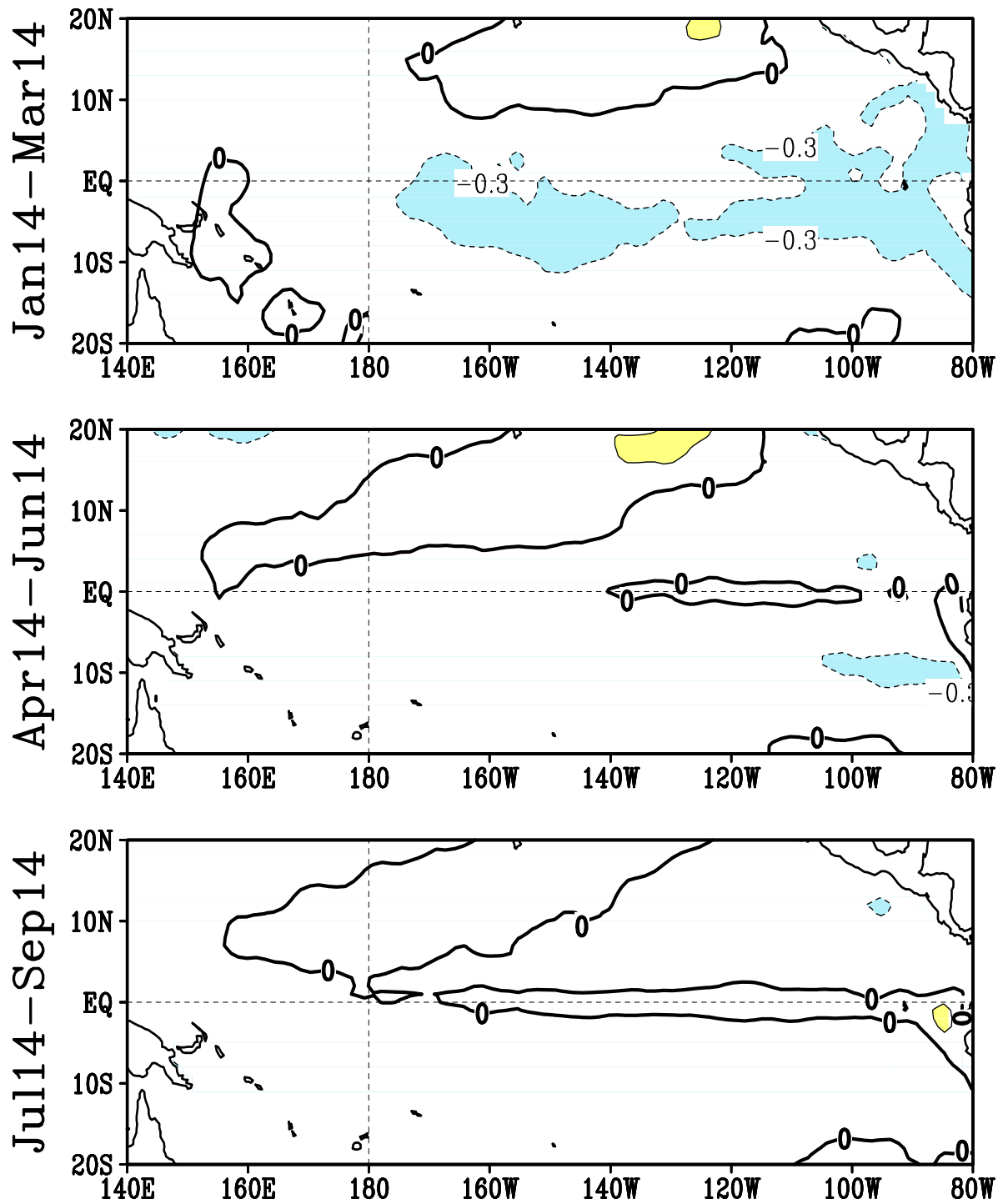
FIGURE F5. Predicted 3-month average sea surface temperature anomalies from the NCEP/CPC Markov model (Xue et al. 2000, J. Climate , 13 , 849-871). The forecast is initiated in DEC 2013 . Contour interval is 0.3C and negative anomalies are indicated by dashed contours. Anomalies are calculated relative to the 1971-2000 climatology.
