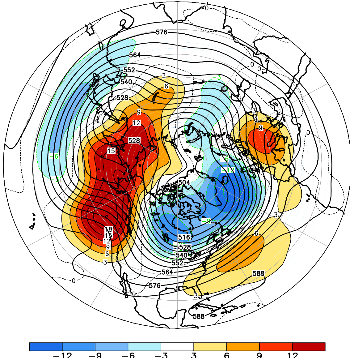
FIGURE E9. Northern Hemisphere mean and anomalous 500-hPa geopotential height (CDAS/Reanalysis) for DEC 2013. Mean heights are denoted by solid contours drawn at an interval of 6 dam. Anomaly contour interval is 3 dam with values less (greater) than -3 dam (3 dam) indicated by dark (light) shading. Anomalies are calculated as departures from the 1981-2010 base period monthly means.
