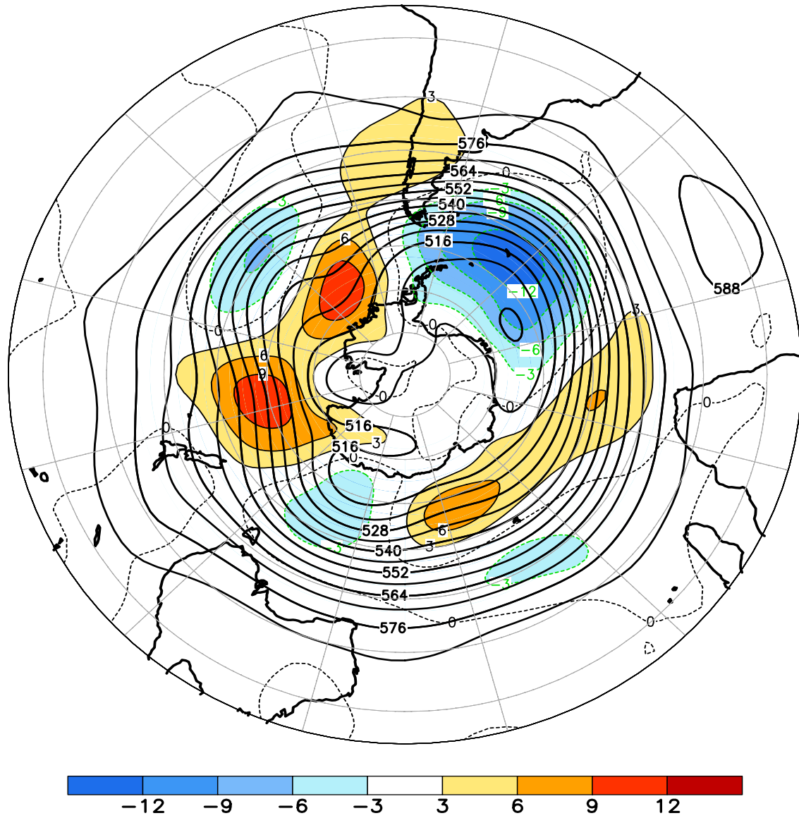
FIGURE E15. Southern Hemisphere mean and anomalous 500-hPa geopotential height (CDAS/Reanalysis) for DEC 2013. Mean heights are denoted by solid contours drawn at an interval of 6 dam. Anomaly contour interval is 3 dam with values less (greater) than -3 dam (3 dam) indicated by dark (light) shading. Anomalies are calculated as departures from the 1981-2010 base period monthly means.
