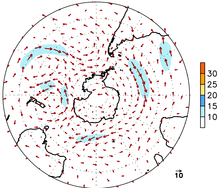
FIGURE E16. Southern Hemisphere mean (left) and anomalous (right) 300-hPa vector wind (CDAS/Reanalysis) for DEC 2014. Mean (anomaly) isotach contour interval is 10 (5) ms -1 . Values greater than 30 ms -1 (left) and 10 ms -1 (rights) are shaded. Anomalies are departures from the 1981-2010 base period monthly means.
