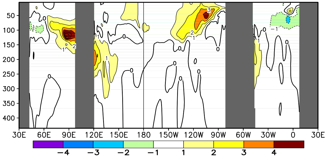
FIGURE T17. Equatorial depth–longitude section of ocean temperature (top) and ocean temperature anomalies (bottom) for DEC 2014. Contour interval is 1°C. Dashed contours in bottom panel indicate negative anomalies. Data are derived from the NCEP’s global ocean data assimilation system version 2 which assimilates oceanic observations into an oceanic GCM (Xue, Y. and Behringer, D.W., 2006: Operational global ocean data assimilation system at NCEP, to be submitted to BAMS). Anomalies are departures from the 1981–2010 base period means.
