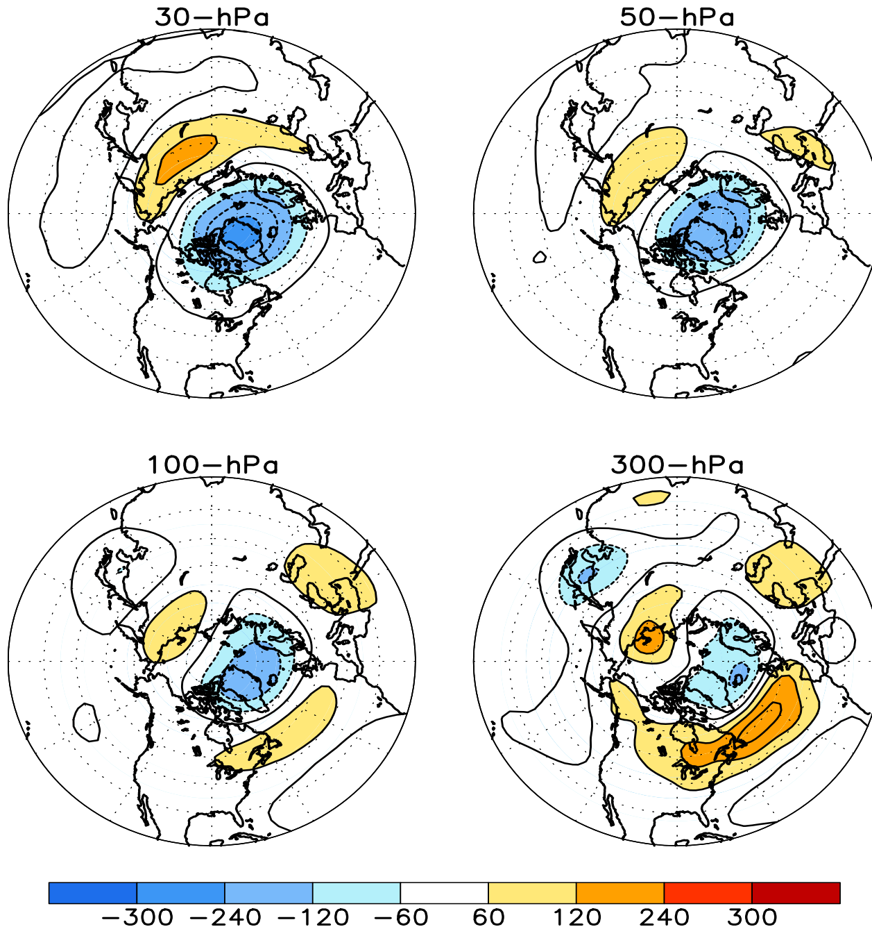
FIGURE S1. Stratospheric height anomalies (m) at selected levels for DEC 2014. Positive values are indicated by solid contours and dark shading. Negative values are indicated by dashed contours and light shading. Contour interval is 60 m. Anomalies are calculated from the 1981-2010 base period means. Winter Hemisphere is shown.
