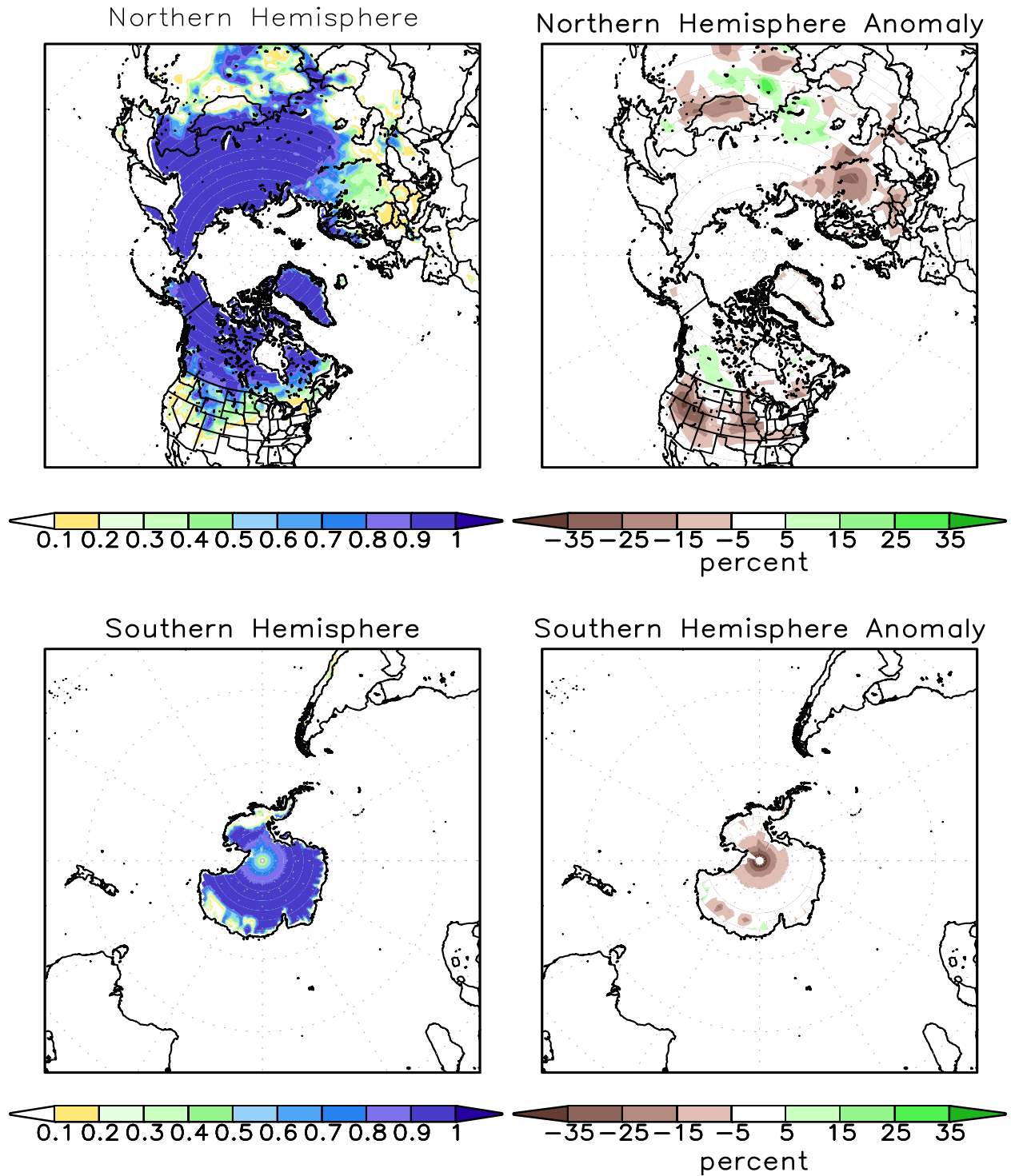
FIGURE A2.2. SSM/I derived snow cover frequency (%) (left) and snow cover anomaly (%) (right) for the month of DEC 2014 based on 1987 - 2010 base period for the Northern Hemisphere (top) and Southern Hemisphere (bottom). It is generated using the algorithm described by Ferraro et. al, 1996, Bull. Amer. Meteor. Soc., vol 77, 891-905.
