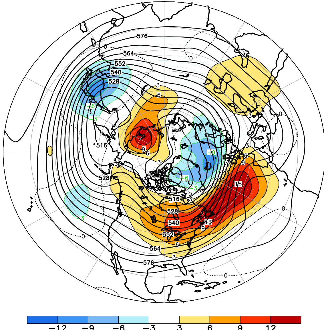
FIGURE E9. Northern Hemisphere mean and anomalous 500-hPa geopotential height (CDAS/Reanalysis) for DEC 2014. Mean heights are denoted by solid contours drawn at an interval of 6 dam. Anomaly contour interval is 3 dam with values less (greater) than -3 dam (3 dam) indicated by dark (light) shading. Anomalies are calculated as departures from the 1981-2010 base period monthly means.
