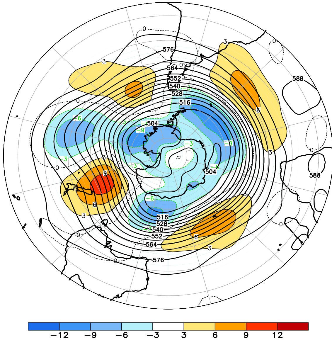
FIGURE E15. Southern Hemisphere mean and anomalous 500-hPa geopotential height (CDAS/Reanalysis) for DEC 2014. Mean heights are denoted by solid contours drawn at an interval of 6 dam. Anomaly contour interval is 3 dam with values less (greater) than -3 dam (3 dam) indicated by dark (light) shading. Anomalies are calculated as departures from the 1981-2010 base period monthly means.
