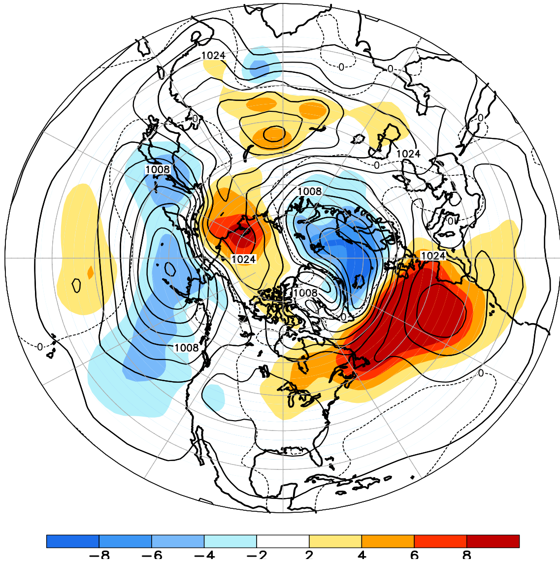
FIGURE E8. Northern Hemisphere mean and anomalous sea level pressure (CDAS/Reanalysis) for DEC 2014. Mean values are denoted by solid contours drawn at an interval of 4 hPa. Anomaly contour interval is 2 hPa with values less (greater) than -2 hPa (2 hPa) indicated by dark (light) shading. Anomalies are calculated as departures from the 1981-2010 base period monthly means.
