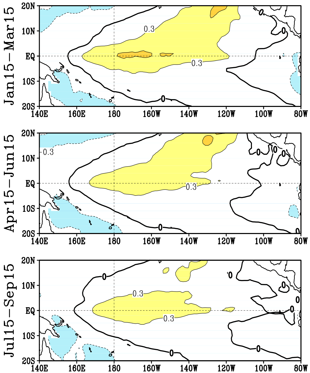
FIGURE F5. Predicted 3-month average sea surface temperature anomalies from the NCEP/CPC Markov model (Xue et al. 2000, J. Climate , 13 , 849-871). The forecast is initiated in DEC 2014 . Contour interval is 0.3C and negative anomalies are indicated by dashed contours. Anomalies are calculated relative to the 1971-2000 climatology.
