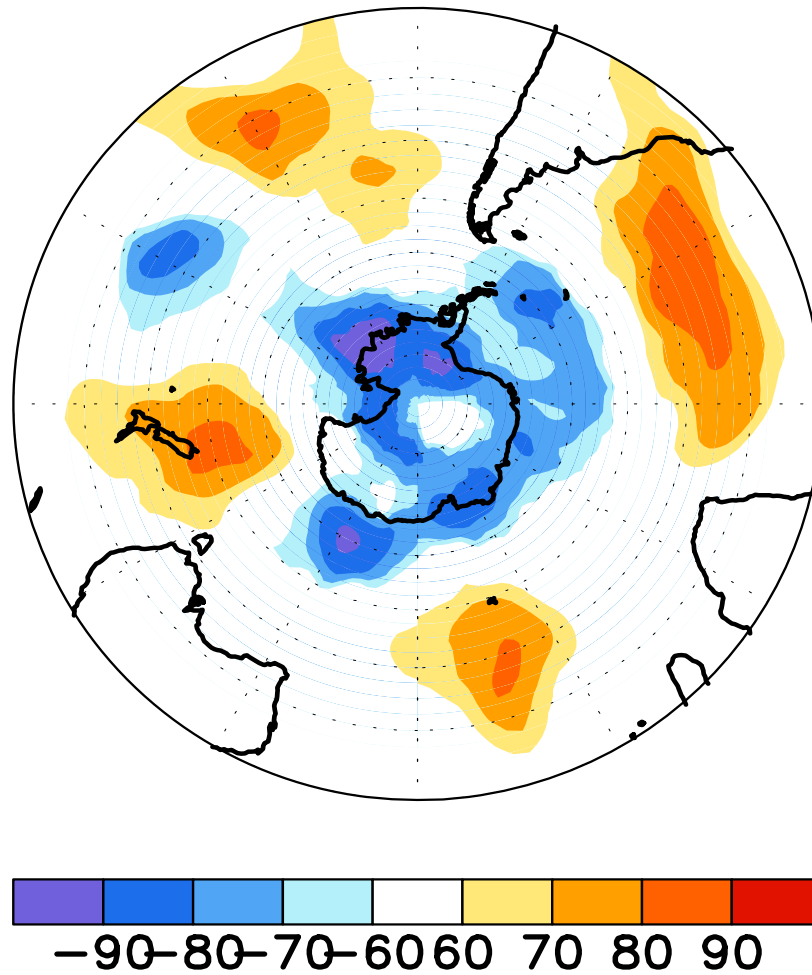
FIGURE E17. Southern Hemisphere percentage of days during DEC 2014 in which 500-hPa height anomalies greater than 15 m (red) and less than -15 m (blue) were observed. Values greater than 70% are shaded and contour in-
