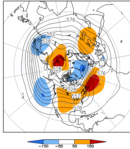
500-hPa Height (dm) & Anomalies (m) (Dec 1–15, 2014)
