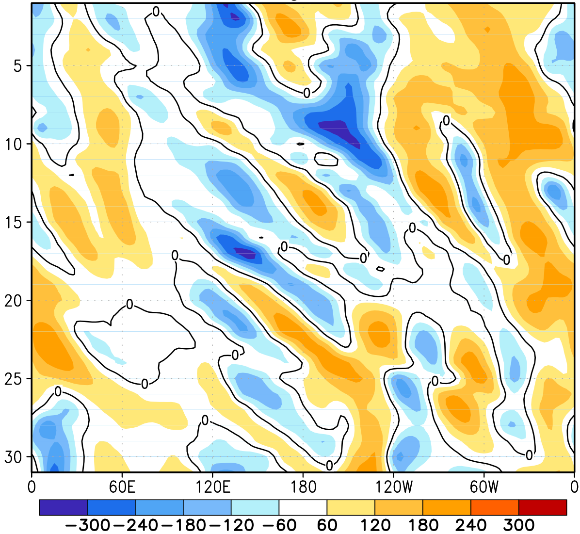
FIGURE E12. Northern Hemisphere: Daily 500-hPa height anomalies for DEC 2014 averaged over the 5° latitude band centered on 40°N. Positive values are indicated by solid contours and dark shading. Negative values are indicated by dashed contours and light shading. Contour interval is 60 m. Anomalies are departures from the 1981-2010 base period daily means.
