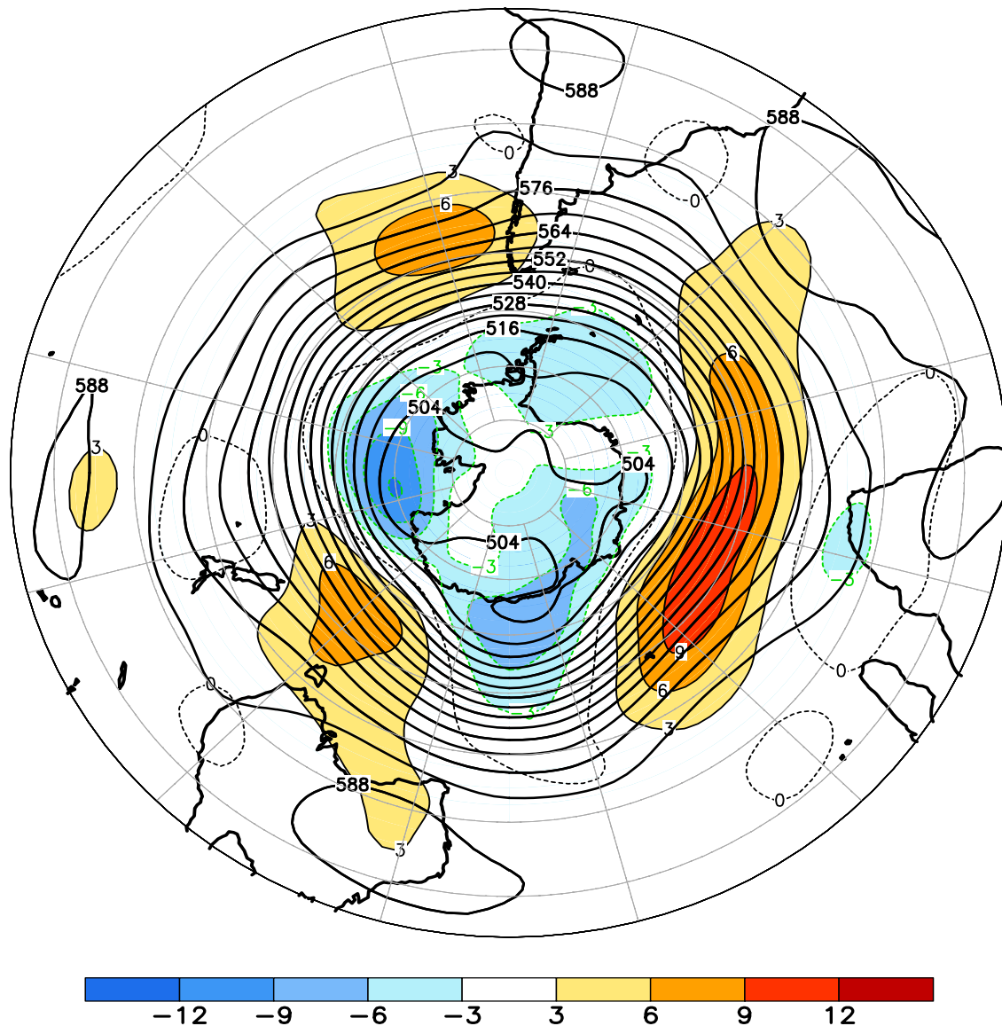
FIGURE E15. Southern Hemisphere mean and anomalous 500-hPa geopotential height (CDAS/Reanalysis) for FEB 2015. Mean heights are denoted by solid contours drawn at an interval of 6 dam. Anomaly contour interval is 3 dam with values less (greater) than -3 dam (3 dam) indicated by dark (light) shading. Anomalies are calculated as departures from the 1981-2010 base period monthly means.
