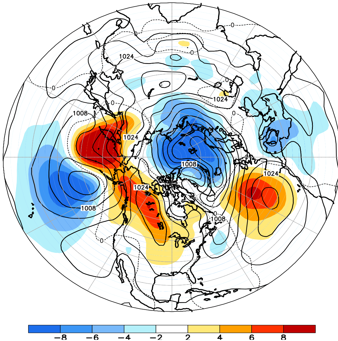
FIGURE E8. Northern Hemisphere mean and anomalous sea level pressure (CDAS/Reanalysis) for FEB 2015. Mean values are denoted by solid contours drawn at an interval of 4 hPa. Anomaly contour interval is 2 hPa with values less (greater) than -2 hPa (2 hPa) indicated by dark (light) shading. Anomalies are calculated as departures from the 1981-2010 base period monthly means.
