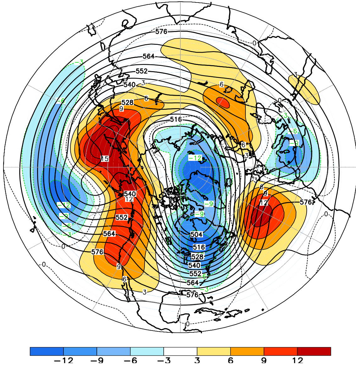
FIGURE E9. Northern Hemisphere mean and anomalous 500-hPa geopotential height (CDAS/Reanalysis) for FEB 2015. Mean heights are denoted by solid contours drawn at an interval of 6 dam. Anomaly contour interval is 3 dam with values less (greater) than -3 dam (3 dam) indicated by dark (light) shading. Anomalies are calculated as departures from the 1981-2010 base period monthly means.
