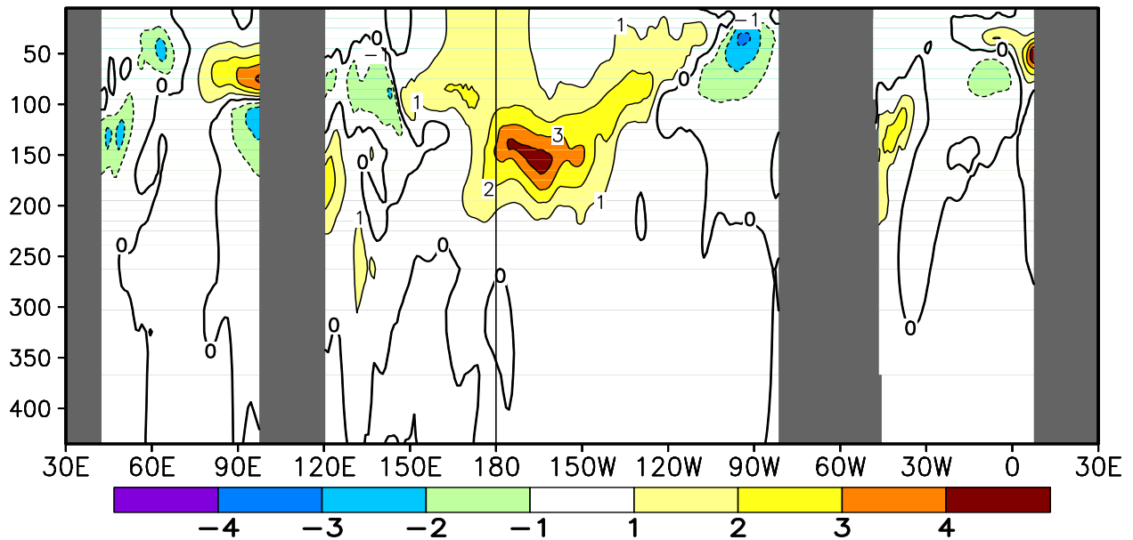
FIGURE T17. Equatorial depth–longitude section of ocean temperature (top) and ocean temperature anomalies (bottom) for FEB 2015. Contour interval is 1°C. Dashed contours in bottom panel indicate negative anomalies. Data are derived from the NCEP’s global ocean data assimilation system version 2 which assimilates oceanic observations into an oceanic GCM (Xue, Y. and Behringer, D.W., 2006: Operational global ocean data assimilation system at NCEP, to be submitted to BAMS). Anomalies are departures from the 1981–2010 base period means.
