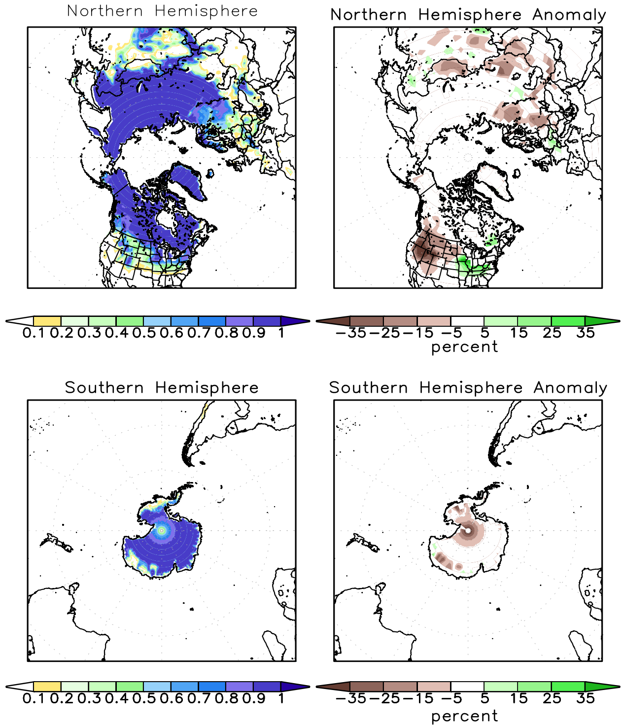
FIGURE A2.2. SSM/I derived snow cover frequency (%) (left) and snow cover anomaly (%) (right) for the month of FEB 2015 based on 1987 - 2010 base period for the Northern Hemisphere (top) and Southern Hemisphere (bottom). It is generated using the algorithm described by Ferraro et. al, 1996, Bull. Amer. Meteor. Soc., vol 77, 891-905.
