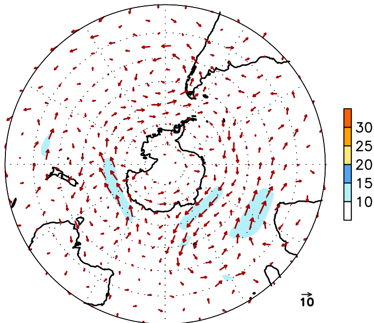
FIGURE E16. Southern Hemisphere mean (left) and anomalous (right) 300-hPa vector wind (CDAS/Reanalysis) for FEB 2015. Mean (anomaly) isotach contour interval is 10 (5) \text{ms}^{-1} . Values greater than 30 \text{ms}^{-1} (left) and 10 \text{ms}^{-1} (rights) are shaded. Anomalies are departures from the 1981-2010 base period monthly means.
