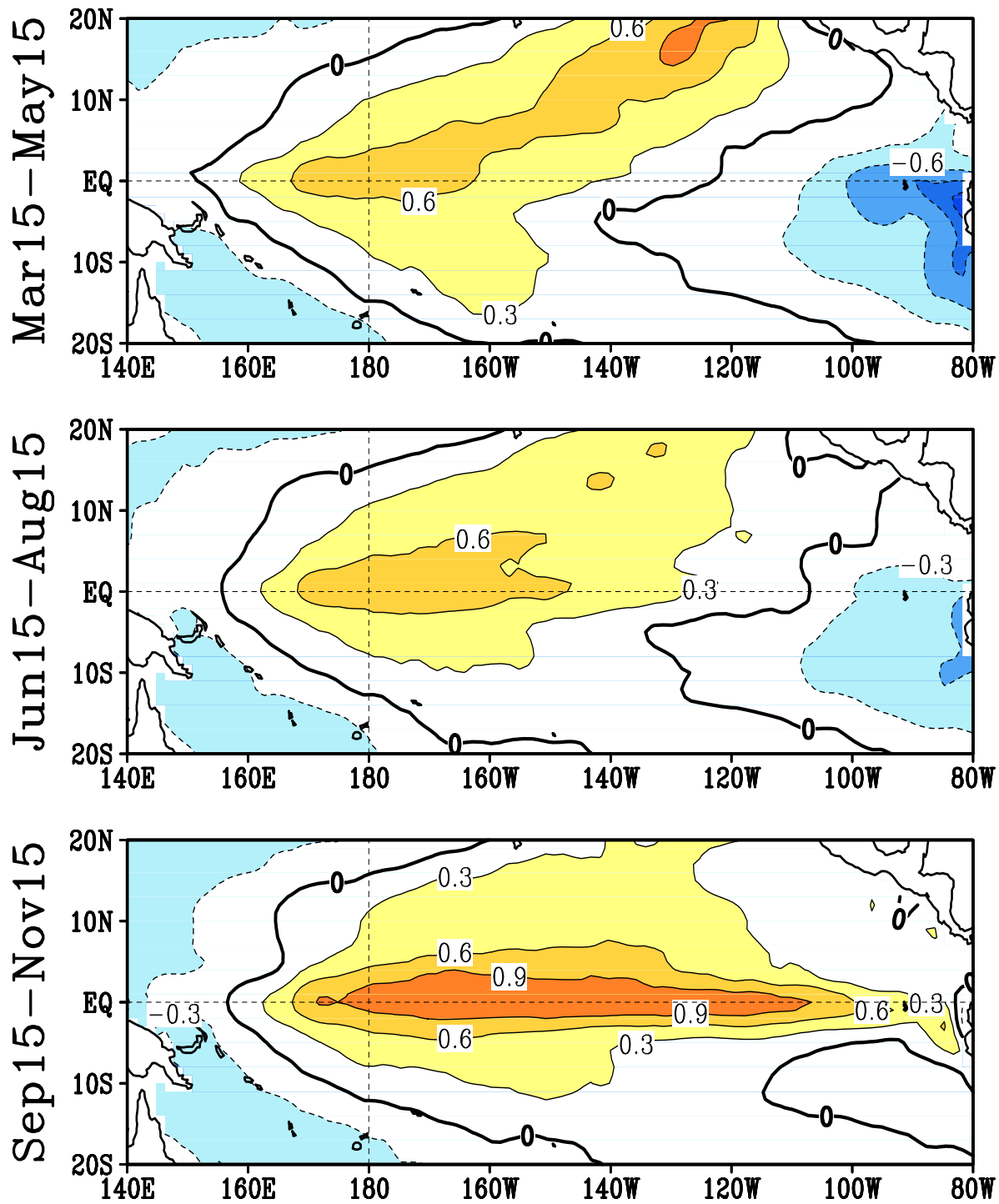
FIGURE F5. Predicted 3-month average sea surface temperature anomalies from the NCEP/CPC Markov model (Xue et al. 2000, J. Climate , 13 , 849-871). The forecast is initiated in FEB 2015 . Contour interval is 0.3C and negative anomalies are indicated by dashed contours. Anomalies are calculated relative to the 1971-2000 climatology.
