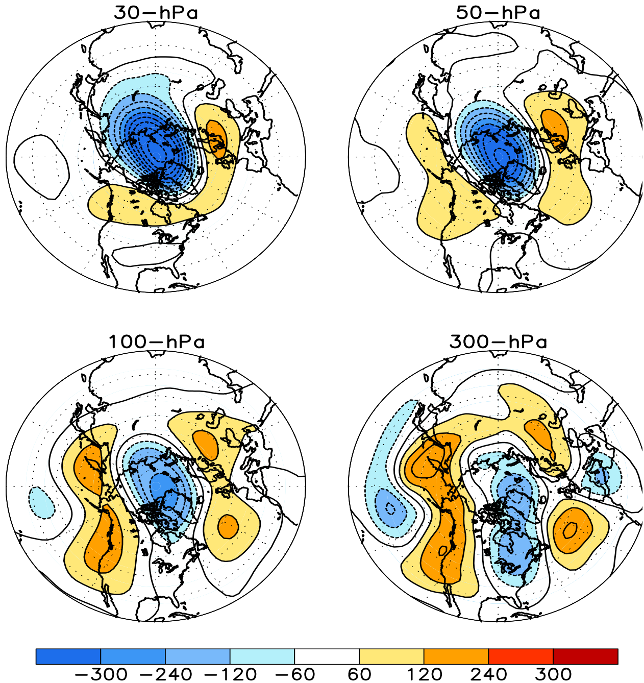
FIGURE S1. Stratospheric height anomalies (m) at selected levels for FEB 2015. Positive values are indicated by solid contours and dark shading. Negative values are indicated by dashed contours and light shading. Contour interval is 60 m. Anomalies are calculated from the 1981-2010 base period means. Winter Hemisphere is shown.
