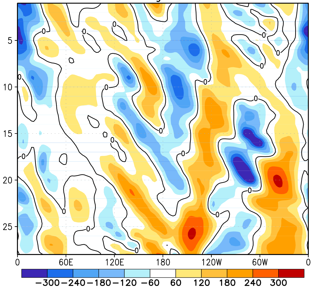
FIGURE E12. Northern Hemisphere: Daily 500-hPa height anomalies for FEB 2015 averaged over the 5° latitude band centered on 40°N. Positive values are indicated by solid contours and dark shading. Negative values are indicated by dashed contours and light shading. Contour interval is 60 m. Anomalies are departures from the 1981-2010 base period daily means.
