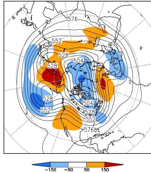
500-hPa Height (dm) & Anomalies (m) (Feb 1–15, 2015)
