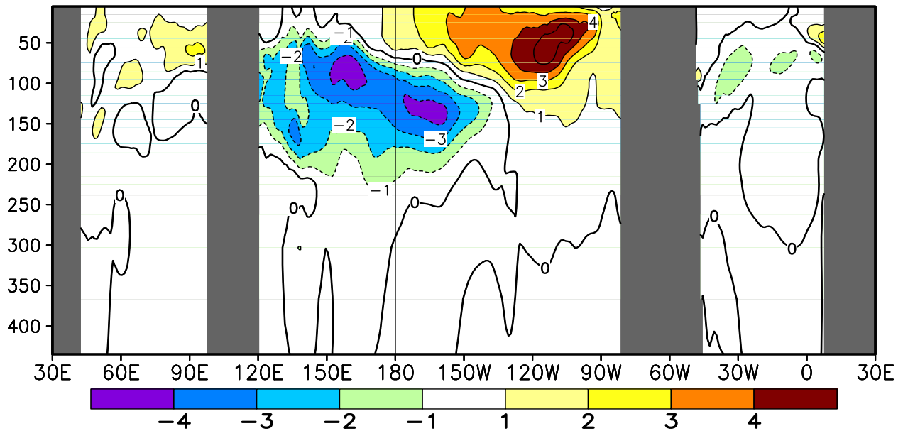
FIGURE T17. Equatorial depth–longitude section of ocean temperature (top) and ocean temperature anomalies (bottom) for FEB 2016. Contour interval is 1°C. Dashed contours in bottom panel indicate negative anomalies. Data are derived from the NCEP’s global ocean data assimilation system version 2 which assimilates oceanic observations into an oceanic GCM (Xue, Y. and Behringer, D.W., 2006: Operational global ocean data assimilation system at NCEP, to be submitted to BAMS). Anomalies are departures from the 1981–2010 base period means.
