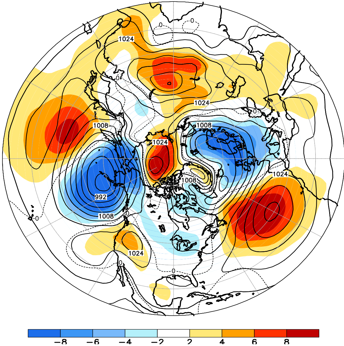
FIGURE E8. Northern Hemisphere mean and anomalous sea level pressure (CDAS/Reanalysis) for FEB 2016. Mean values are denoted by solid contours drawn at an interval of 4 hPa. Anomaly contour interval is 2 hPa with values less (greater) than -2 hPa (2 hPa) indicated by dark (light) shading. Anomalies are calculated as departures from the 1981-2010 base period monthly means.
