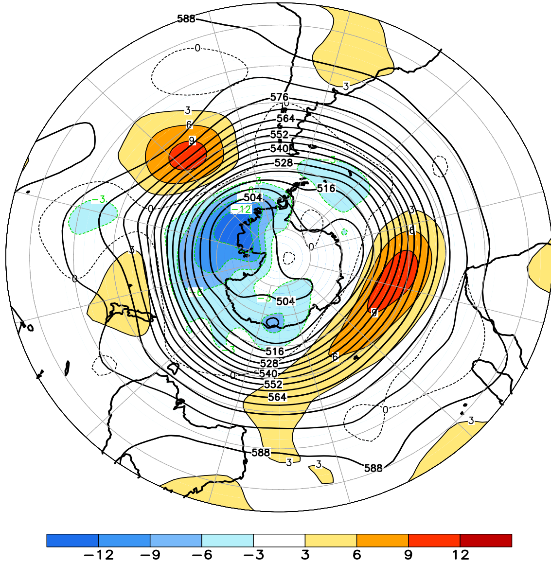
FIGURE E15. Southern Hemisphere mean and anomalous 500-hPa geopotential height (CDAS/Reanalysis) for FEB 2016. Mean heights are denoted by solid contours drawn at an interval of 6 dam. Anomaly contour interval is 3 dam with values less (greater) than -3 dam (3 dam) indicated by dark (light) shading. Anomalies are calculated as departures from the 1981-2010 base period monthly means.
