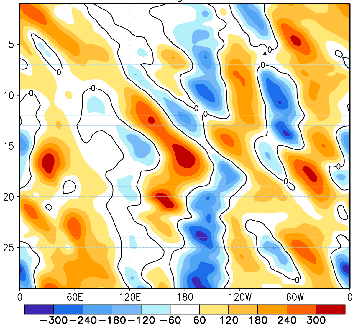
FIGURE E12. Northern Hemisphere: Daily 500-hPa height anomalies for FEB 2016 averaged over the 5° latitude band centered on 40°N. Positive values are indicated by solid contours and dark shading. Negative values are indicated by dashed contours and light shading. Contour interval is 60 m. Anomalies are departures from the 1981-2010 base period daily means.
