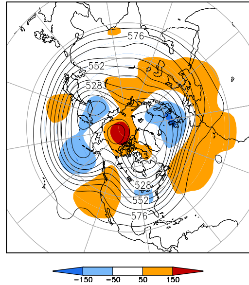
500-hPa Height (dm) & Anomalies (m) (Feb 1–15, 2016)
