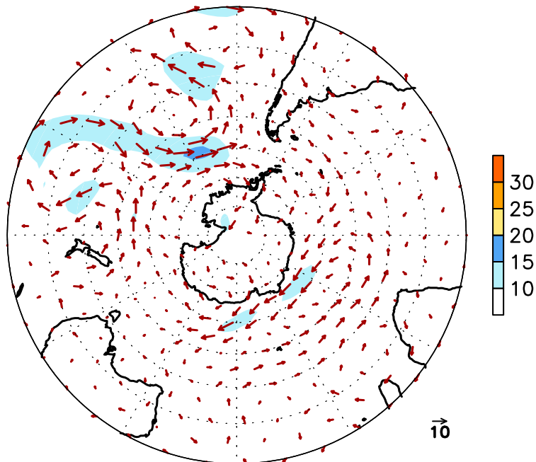
FIGURE E16. Southern Hemisphere mean (left) and anomalous (right) 300-hPa vector wind (CDAS/Reanalysis) for FEB 2016. Mean (anomaly) isotach contour interval is 10 (5) \text{ms}^{-1} . Values greater than 30 \text{ms}^{-1} (left) and 10 \text{ms}^{-1} (rights) are shaded. Anomalies are departures from the 1981-2010 base period monthly means.
