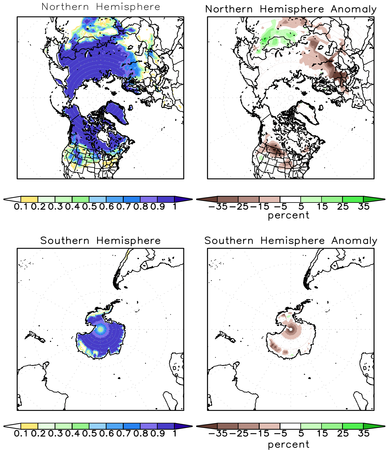
FIGURE A2.2. SSM/I derived snow cover frequency (%) (left) and snow cover anomaly (%) (right) for the month of FEB 2016 based on 1987 - 2010 base period for the Northern Hemisphere (top) and Southern Hemisphere (bottom). It is generated using the algorithm described by Ferraro et. al, 1996, Bull. Amer. Meteor. Soc., vol 77, 891-905.
