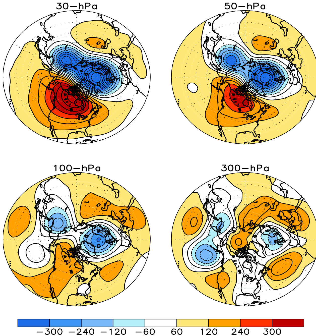
FIGURE S1. Stratospheric height anomalies (m) at selected levels for FEB 2016. Positive values are indicated by solid contours and dark shading. Negative values are indicated by dashed contours and light shading. Contour interval is 60 m. Anomalies are calculated from the 1981-2010 base period means. Winter Hemisphere is shown.
