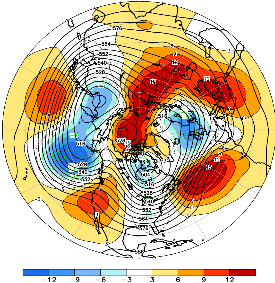
FIGURE E9. Northern Hemisphere mean and anomalous 500-hPa geopotential height (CDAS/Reanalysis) for FEB 2016. Mean heights are denoted by solid contours drawn at an interval of 6 dam. Anomaly contour interval is 3 dam with values less (greater) than -3 dam (3 dam) indicated by dark (light) shading. Anomalies are calculated as departures from the 1981-2010 base period monthly means.
