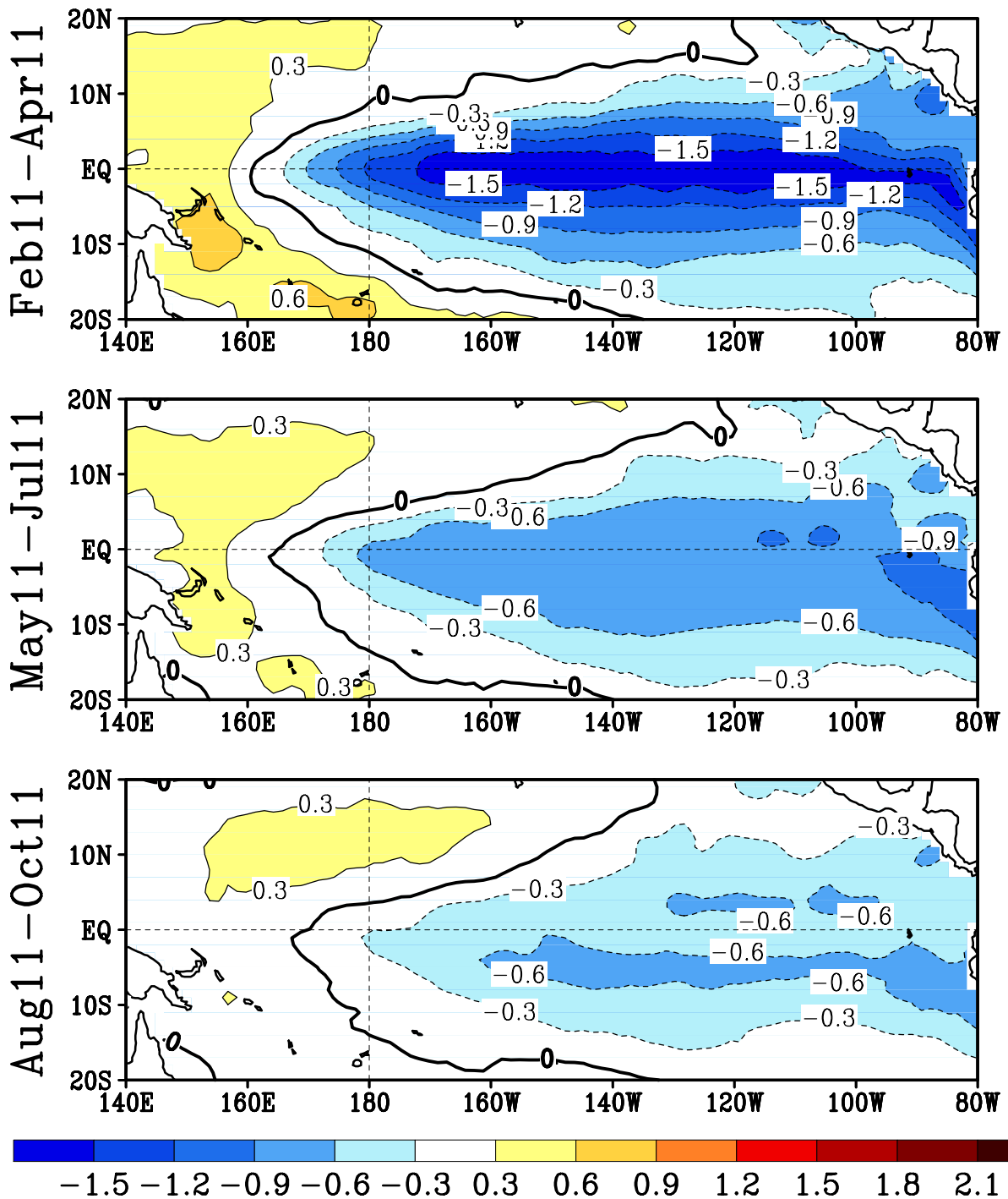
FIGURE F5. Predicted 3-month average sea surface temperature anomalies from the NCEP/CPC Markov model (Xue et al. 2000, J. Climate , 13 , 849-871). The forecast is initiated in JAN 2011. Contour interval is 0.3C and negative anomalies are indicated by dashed contours. Anomalies are calculated relative to the 1971-2000 climatology.
