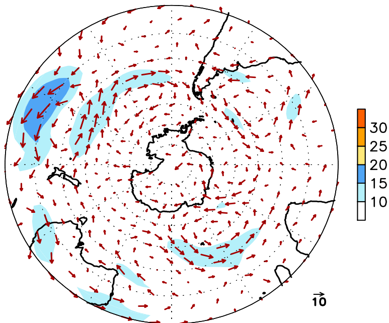
FIGURE E16. Southern Hemisphere mean (left) and anomalous (right) 300-hPa vector wind (CDAS/Reanalysis) for JAN 2011. Mean (anomaly) isotach contour interval is 10 (5) \text{ms}^{-1} . Values greater than 30 \text{ms}^{-1} (left) and 10 \text{ms}^{-1} (rights) are shaded. Anomalies are departures from the 1981-2010 base period monthly means.
