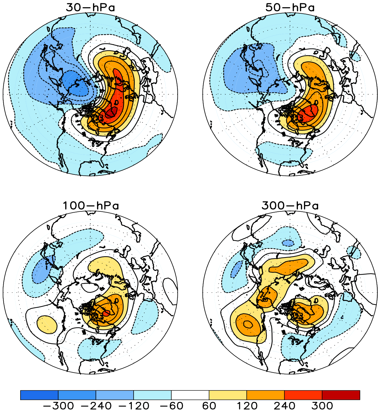
FIGURE S1. Stratospheric height anomalies (m) at selected levels for JAN 2011. Positive values are indicated by solid contours and dark shading. Negative values are indicated by dashed contours and light shading. Contour interval is 60 m. Anomalies are calculated from the 1981-2010 base period means. Winter Hemisphere is shown.
