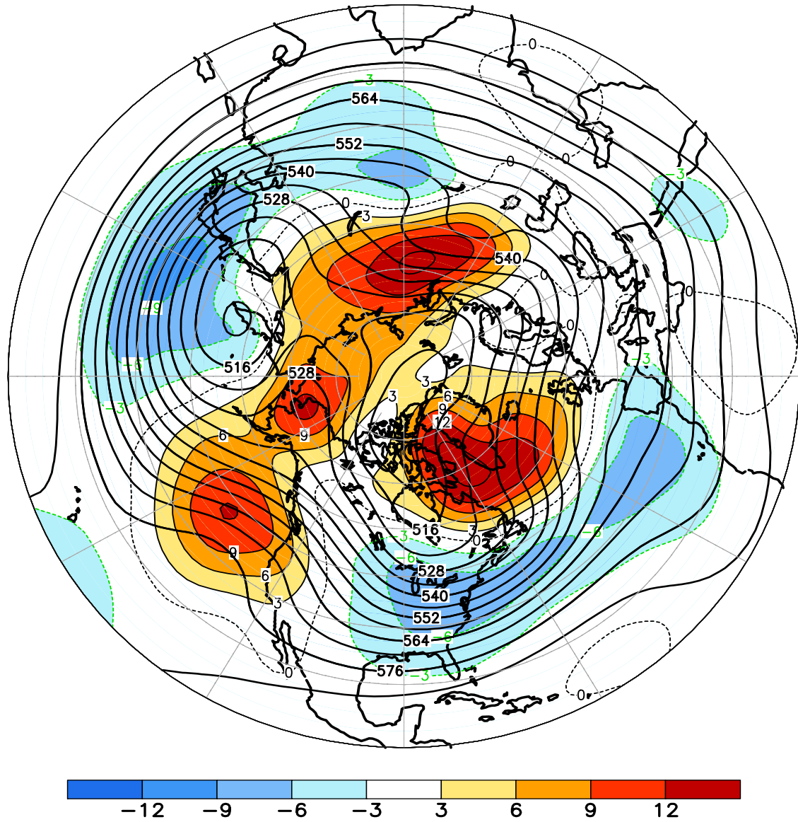
FIGURE E9. Northern Hemisphere mean and anomalous 500-hPa geopotential height (CDAS/Reanalysis) for JAN 2011. Mean heights are denoted by solid contours drawn at an interval of 6 dam. Anomaly contour interval is 3 dam with values less (greater) than -3 dam (3 dam) indicated by dark (light) shading. Anomalies are calculated as departures from the 1981-2010 base period monthly means.
