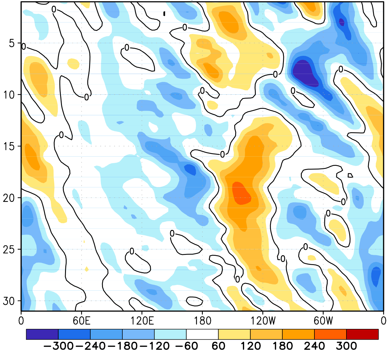
FIGURE E12. Northern Hemisphere: Daily 500-hPa height anomalies for JAN 2011 averaged over the 5° latitude band centered on 40°N. Positive values are indicated by solid contours and dark shading. Negative values are indicated by dashed contours and light shading. Contour interval is 60 m. Anomalies are departures from the 1981-2010 base period daily means.
