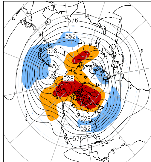
500-hPa Height (dm) & Anomalies (m) (Jan 1–15, 2011)
