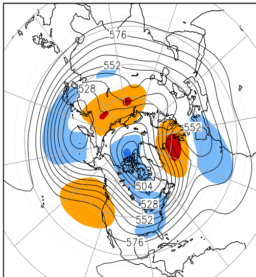
500-hPa Height (dm) & Anomalies (m) (Jan 16–31, 2011)
