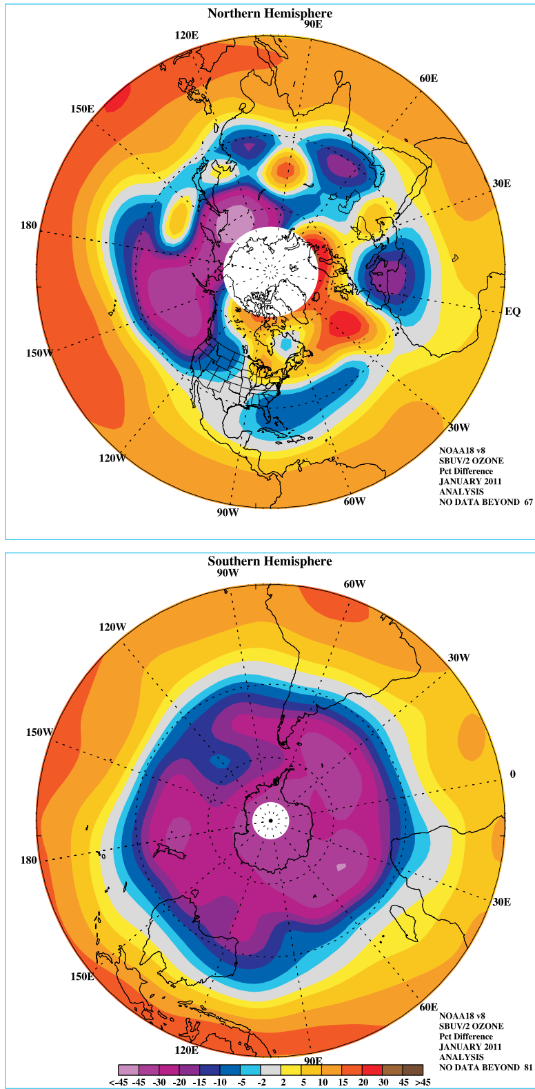
FIGURE S6. Northern (top) and Southern (bottom) Hemisphere total ozone anomaly (percent difference from monthly mean for the period 1981-2010). The region near the winter pole has no SBUV/2 data.
