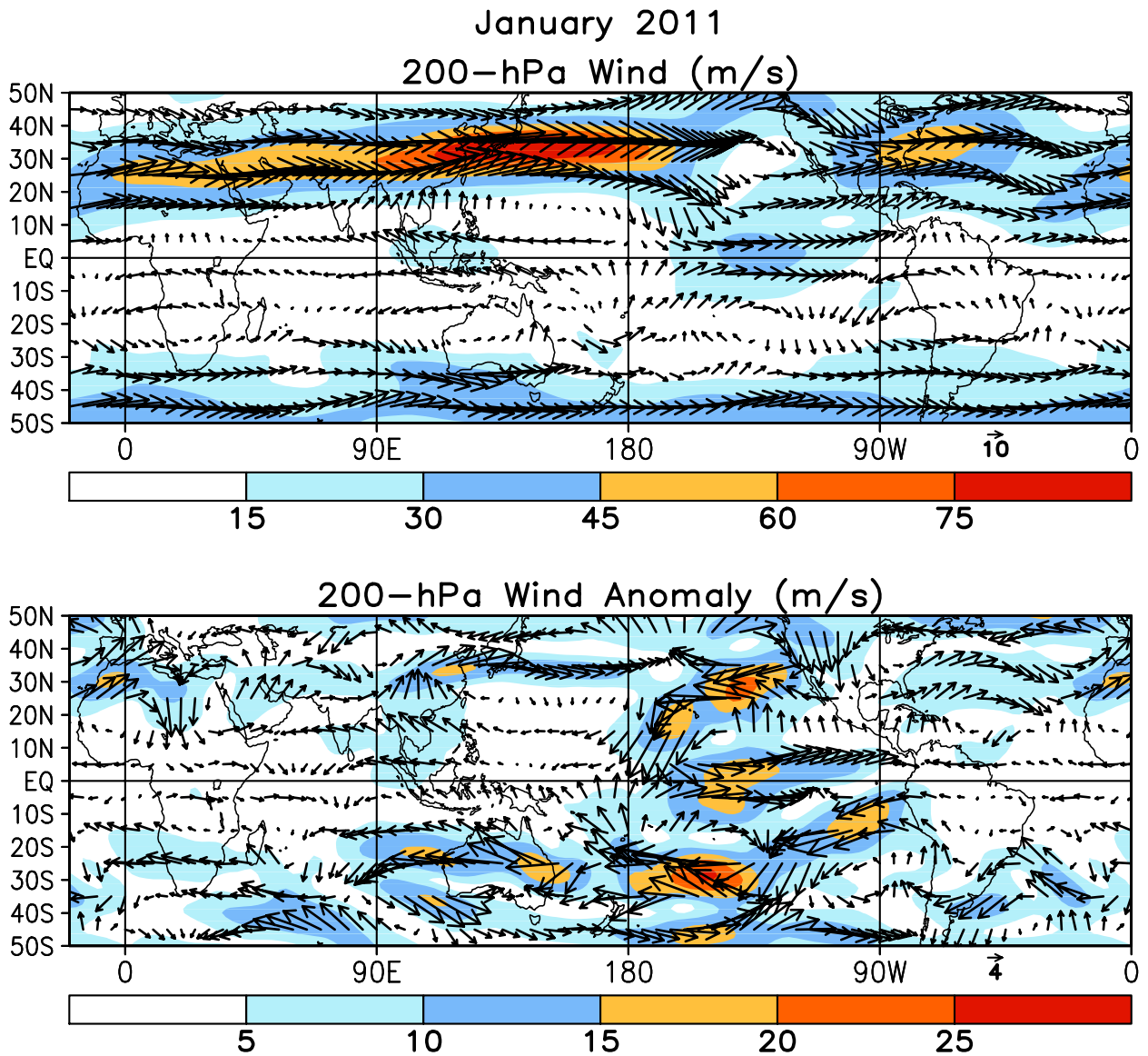
FIGURE T21. Mean (top) and anomalous (bottom) 200-hPa vector wind (CDAS/Reanalysis) for JAN 2011. Contour interval for isotachs is 15 \text{ ms}^{-1} (top) and 5 \text{ ms}^{-1} (bottom). Anomalies are departures from 1981-2010 base period monthly means.
