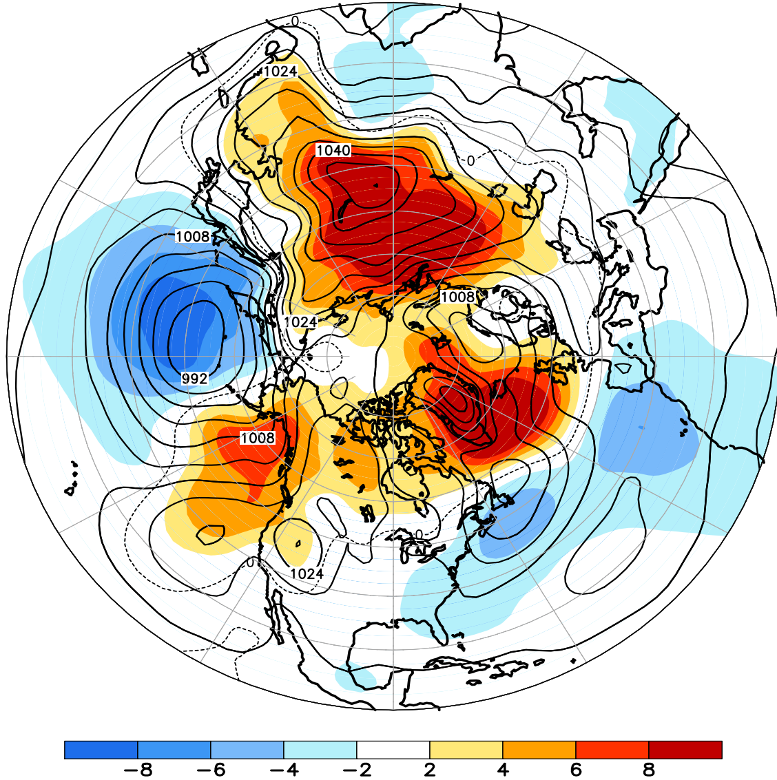
FIGURE E8. Northern Hemisphere mean and anomalous sea level pressure (CDAS/Reanalysis) for JAN 2011. Mean values are denoted by solid contours drawn at an interval of 4 hPa. Anomaly contour interval is 2 hPa with values less (greater) than -2 hPa (2 hPa) indicated by dark (light) shading. Anomalies are calculated as departures from the 1981-2010 base period monthly means.
