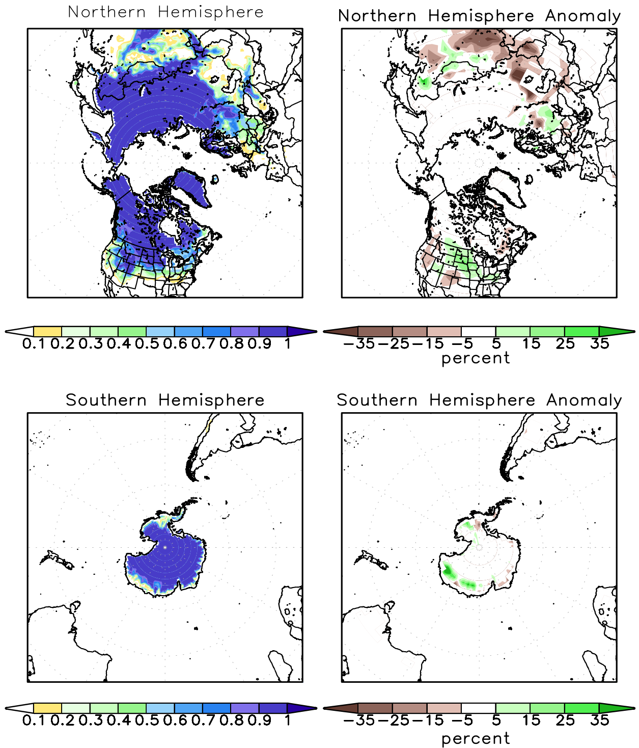
FIGURE A2.2. SSM/I derived snow cover frequency (%) (left) and snow cover anomaly (%) (right) for the month of JAN 2011 based on 1987 - 2010 base period for the Northern Hemisphere (top) and Southern Hemisphere (bottom). It is generated using the algorithm described by Ferraro et. al, 1996, Bull. Amer. Meteor. Soc., vol 77, 891-905.
