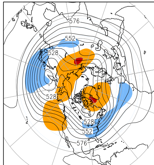
500-hPa Height (dm) & Anomalies (m) (Jan 1–31, 2011)
