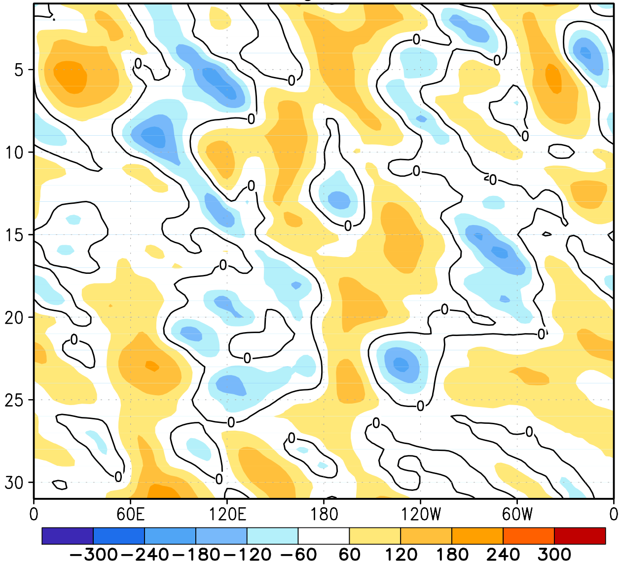
FIGURE E18. Southern Hemisphere: Daily 500-hPa height anomalies for JAN 2011 averaged over the 5° latitude band centered on 40°S. Positive values are indicated by solid contours and dark shading. Negative values are indicated by dashed contours and light shading. Contour interval is 60 m. Anomalies are departures from the 1981-2010 base period daily means.
