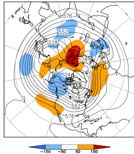
500-hPa Height (dm) & Anomalies (m) (Jan 1–31, 2012)
