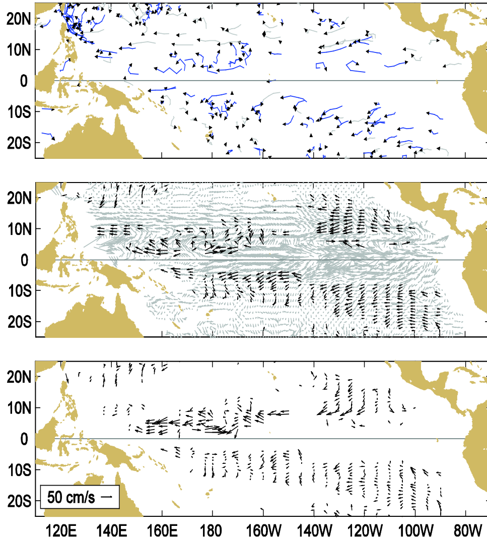
Figure A1.1 Top: Movements of drifting buoys in the tropical Pacific Ocean during January 2012. The linear segments of each trajectory represent a one week displacement. Trajectories of buoys which have lost their subsurface drogues are gray; those with drogues are black.
