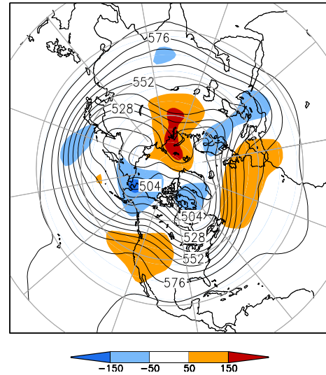
500-hPa Height (dm) & Anomalies (m) (Jan 1–15, 2012)
