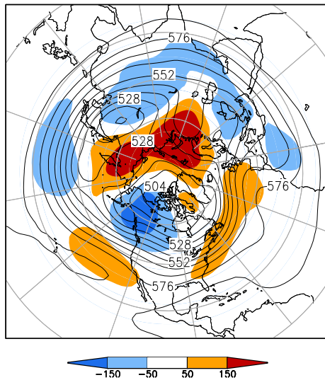
500-hPa Height (dm) & Anomalies (m) (Jan 16–31, 2012)
