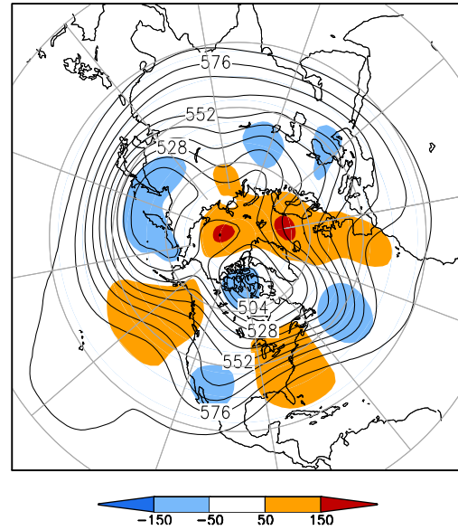
500-hPa Height (dm) & Anomalies (m) (Jan 1–15, 2013)
