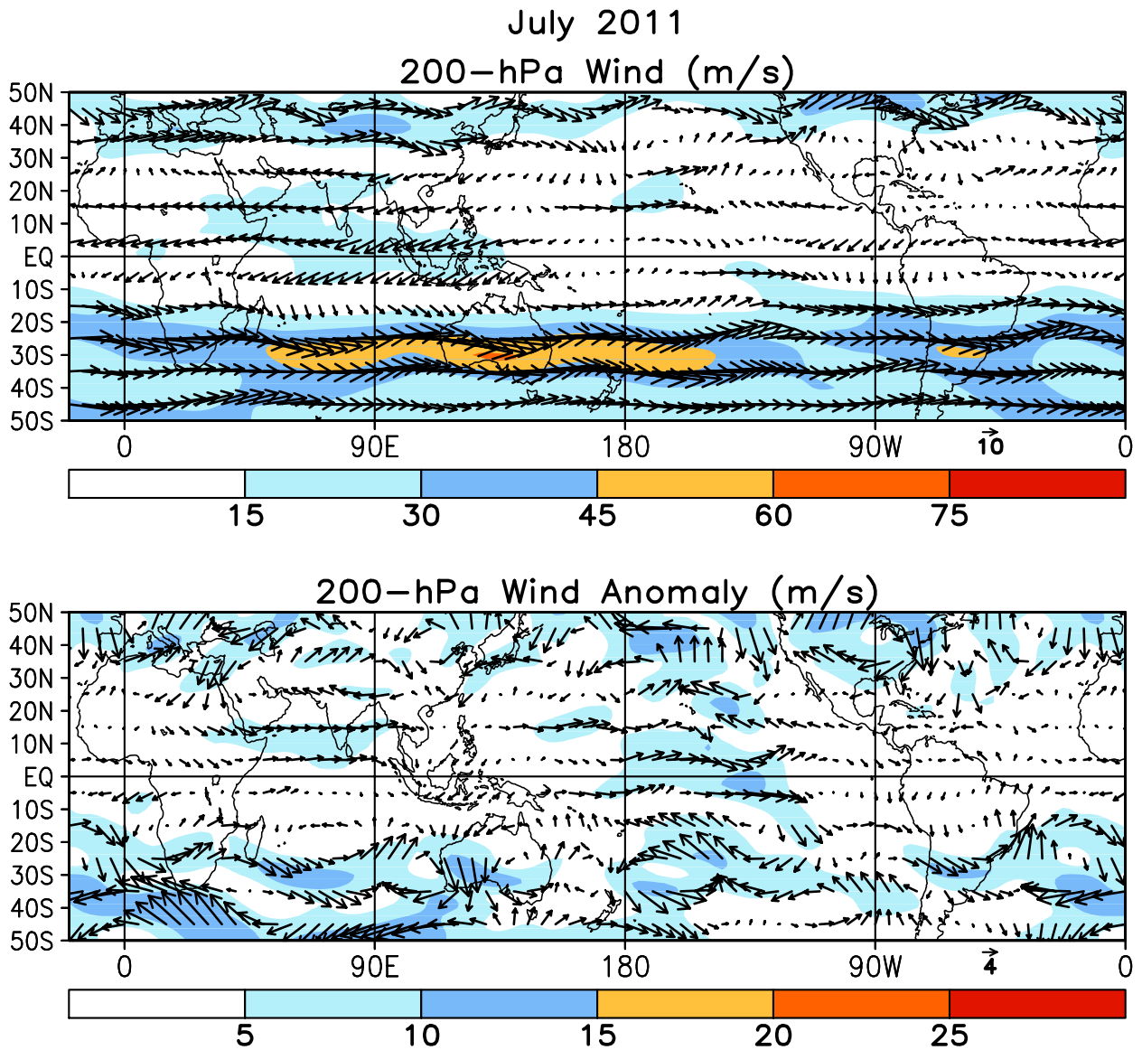
FIGURE T21. Mean (top) and anomalous (bottom) 200-hPa vector wind (CDAS/Reanalysis) for JUL 2011. Contour interval for isotachs is 15 \text{ ms}^{-1} (top) and 5 \text{ ms}^{-1} (bottom). Anomalies are departures from 1981-2010 base period monthly means.
