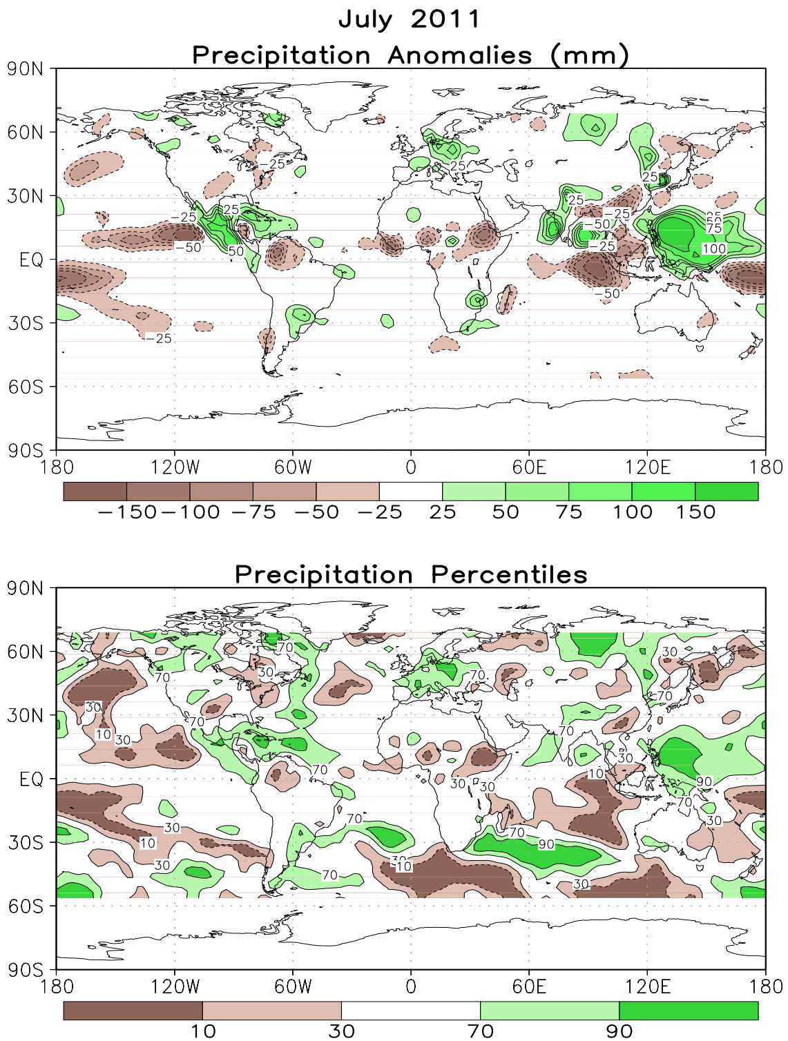
FIGURE E3. Anomalous precipitation (mm, top) and precipitation percentiles based on a Gamma distribution fit to the 1981–2010 base period data (bottom) for JUL 2011. Data are obtained from a merge of raingauge observations and satellite-derived precipitation estimates (Janowiak and Xie 1999, J. Climate , 12 , 3335–3342). Contours are drawn at 200, 100, 50, 25, -25, -50, -100, and -200 mm in top panel. Percentiles are not plotted in regions where mean monthly precipitation is <5mm/month.
