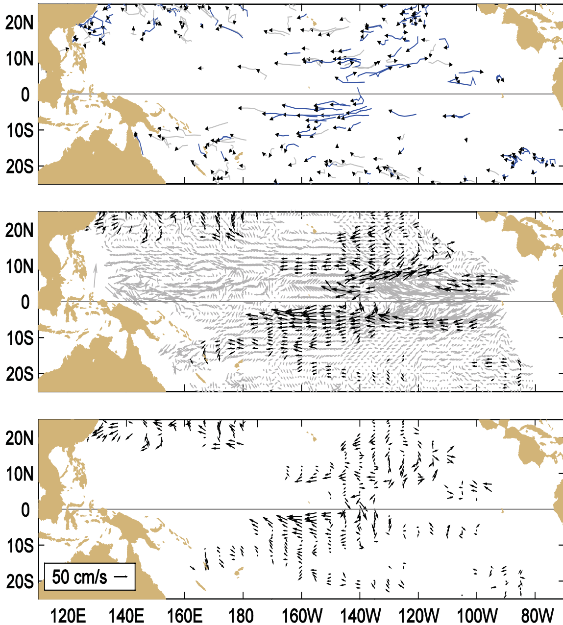
Figure A1.1 Top: Movements of drifting buoys in the tropical Pacific Ocean during July 2011. The linear segments of each trajectory represent a one week displacement. Trajectories of buoys which have lost their subsurface drogues are gray; those with drogues are black.
