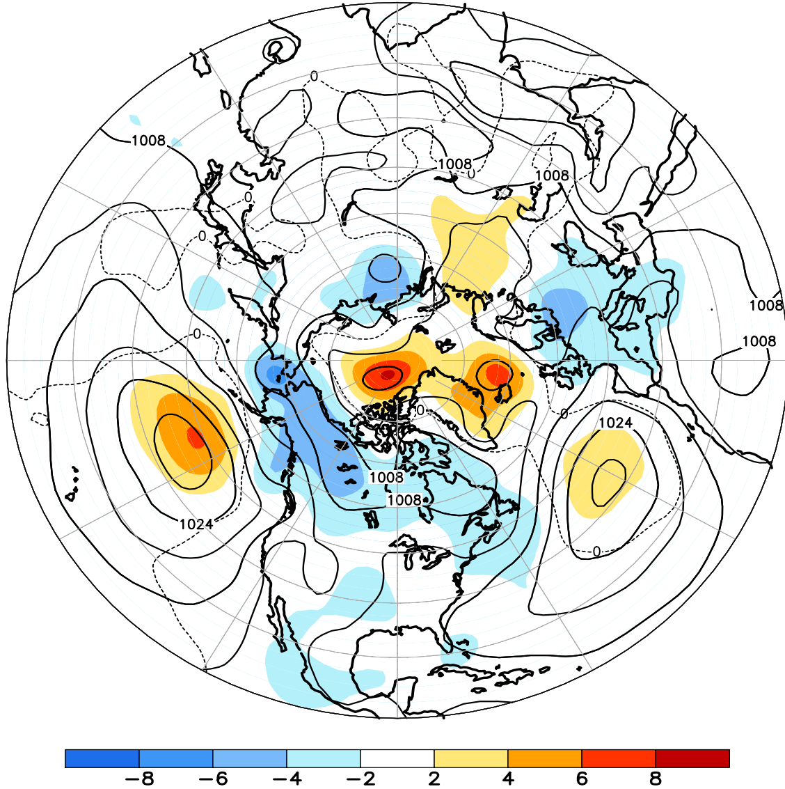
FIGURE E8. Northern Hemisphere mean and anomalous sea level pressure (CDAS/Reanalysis) for JUL 2011. Mean values are denoted by solid contours drawn at an interval of 4 hPa. Anomaly contour interval is 2 hPa with values less (greater) than -2 hPa (2 hPa) indicated by dark (light) shading. Anomalies are calculated as departures from the 1981-2010 base period monthly means.
