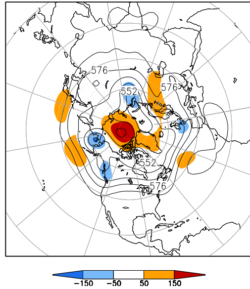
500-hPa Height (dm) & Anomalies (m) (Jul 1–15, 2011)
