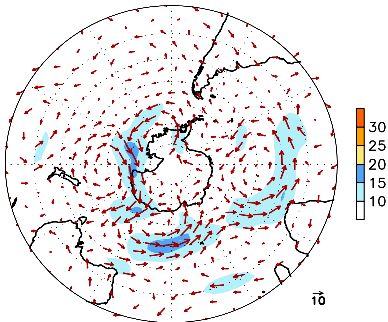
FIGURE E16. Southern Hemisphere mean (left) and anomalous (right) 300-hPa vector wind (CDAS/Reanalysis) for JUL 2011. Mean (anomaly) isotach contour interval is 10 (5) \text{ms}^{-1} . Values greater than 30 \text{ms}^{-1} (left) and 10 \text{ms}^{-1} (rights) are shaded. Anomalies are departures from the 1981-2010 base period monthly means.
