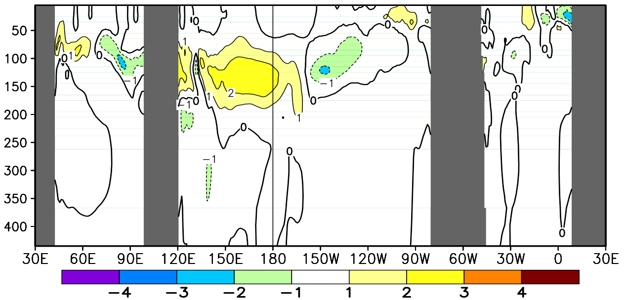
FIGURE T17. Equatorial depth–longitude section of ocean temperature (top) and ocean temperature anomalies (bottom) for JUL 2011. Contour interval is 1°C. Dashed contours in bottom panel indicate negative anomalies. Data are derived from the NCEP’s global ocean data assimilation system version 2 which assimilates oceanic observations into an oceanic GCM (Xue, Y. and Behringer, D.W., 2006: Operational global ocean data assimilation system at NCEP, to be submitted to BAMS). Anomalies are departures from the 1981–2010 base period means.
