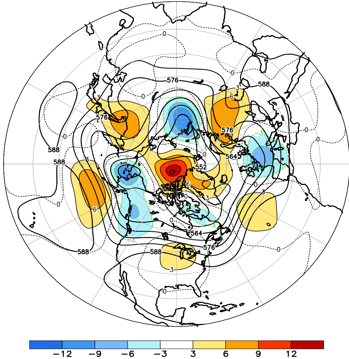
FIGURE E9. Northern Hemisphere mean and anomalous 500-hPa geopotential height (CDAS/Reanalysis) for JUL 2011. Mean heights are denoted by solid contours drawn at an interval of 6 dam. Anomaly contour interval is 3 dam with values less (greater) than -3 dam (3 dam) indicated by dark (light) shading. Anomalies are calculated as departures from the 1981-2010 base period monthly means.
