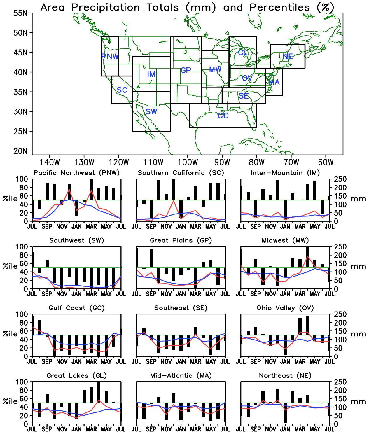
FIGURE E5. Areal estimates of monthly mean precipitation amounts (mm, solid lines) and precipitation percentiles (% , bars) for the most recent 13 months obtained from a merge of raingauge observations and satellite-derived precipitation estimates (Janowiak and Xie 1999, J. Climate , 12 , 3335–3342). The monthly precipitation climatology (mm, dashed lines) is from the 1981–2010 base period monthly means. Monthly percentiles are not shown if the monthly mean is less than 5 mm.
