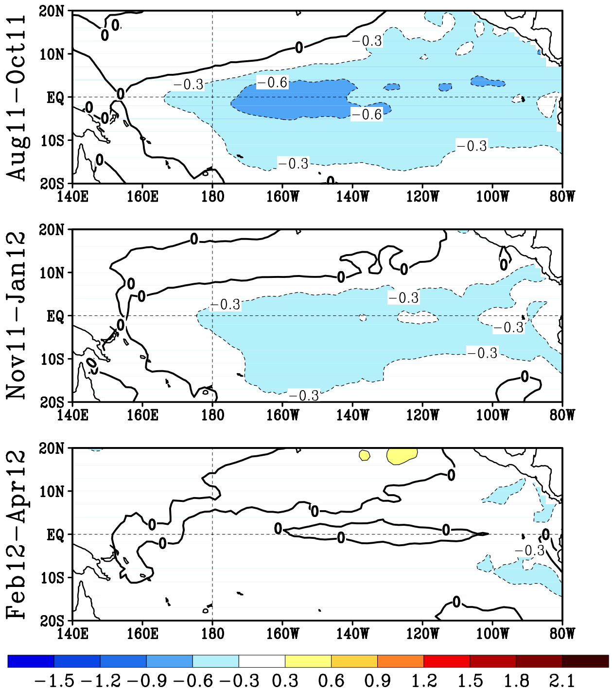
FIGURE F5. Predicted 3-month average sea surface temperature anomalies from the NCEP/CPC Markov model (Xue et al. 2000, J. Climate , 13 , 849-871). The forecast is initiated in JUL 2011 . Contour interval is 0.3C and negative anomalies are indicated by dashed contours. Anomalies are calculated relative to the 1971-2000 climatology.
