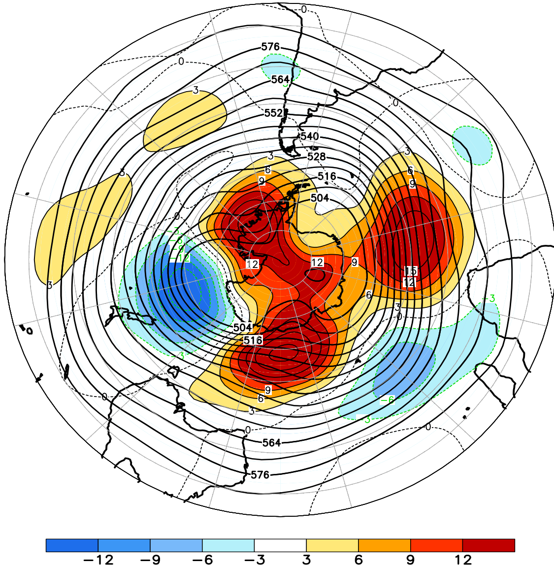
FIGURE E15. Southern Hemisphere mean and anomalous 500-hPa geopotential height (CDAS/Reanalysis) for JUL 2011. Mean heights are denoted by solid contours drawn at an interval of 6 dam. Anomaly contour interval is 3 dam with values less (greater) than -3 dam (3 dam) indicated by dark (light) shading. Anomalies are calculated as departures from the 1981-2010 base period monthly means.
