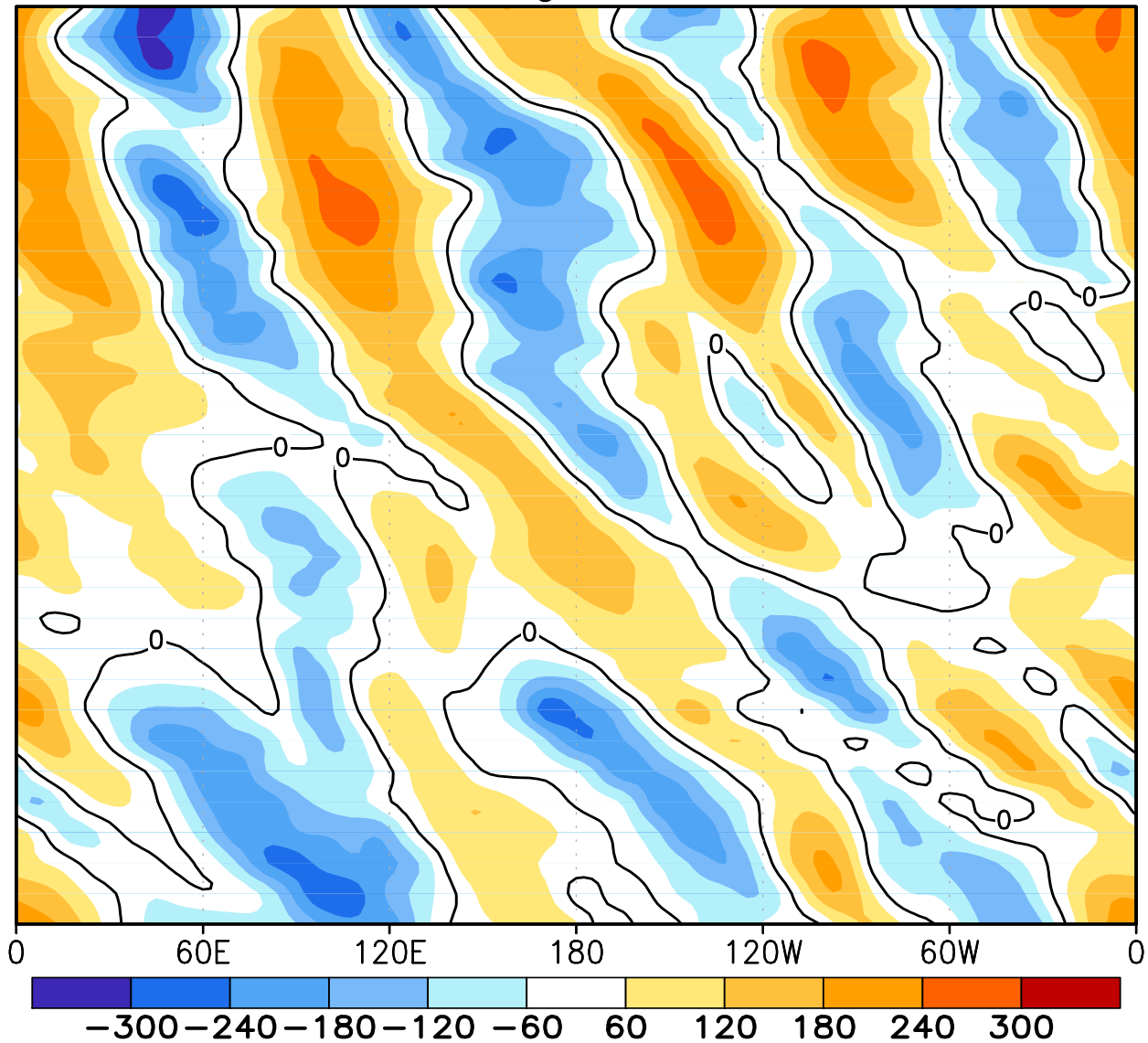
FIGURE E18. Southern Hemisphere: Daily 500-hPa height anomalies for JUL 2011 averaged over the 5° latitude band centered on 40°S. Positive values are indicated by solid contours and dark shading. Negative values are indicated by dashed contours and light shading. Contour interval is 60 m. Anomalies are departures from the 1981-2010 base period daily means.
