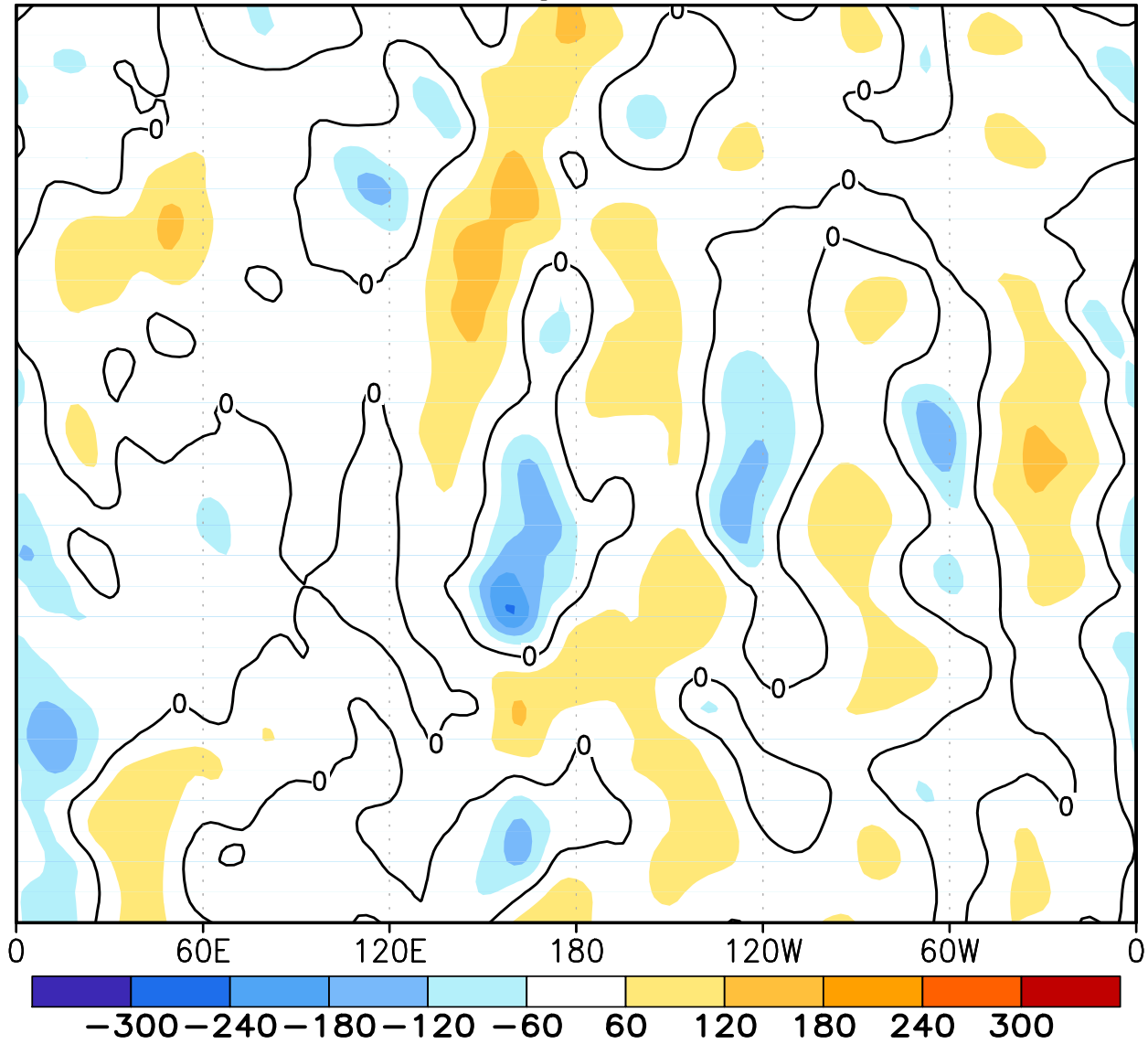
FIGURE E12. Northern Hemisphere: Daily 500-hPa height anomalies for JUL 2011 averaged over the 5° latitude band centered on 40°N. Positive values are indicated by solid contours and dark shading. Negative values are indicated by dashed contours and light shading. Contour interval is 60 m. Anomalies are departures from the 1981-2010 base period daily means.
