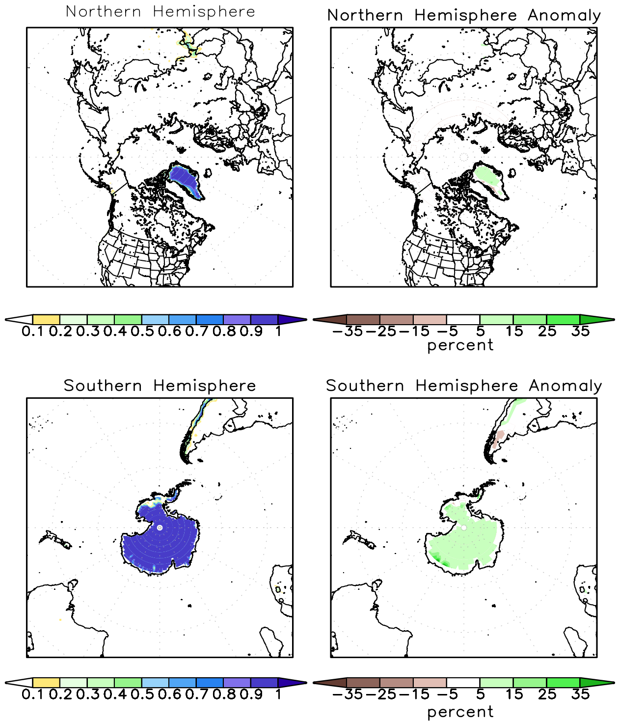
FIGURE A2.2. SSM/I derived snow cover frequency (%) (left) and snow cover anomaly (%) (right) for the month of JUL 2011 based on 1987 - 2010 base period for the Northern Hemisphere (top) and Southern Hemisphere (bottom). It is generated using the algorithm described by Ferraro et. al, 1996, Bull. Amer. Meteor. Soc., vol 77, 891-905.
