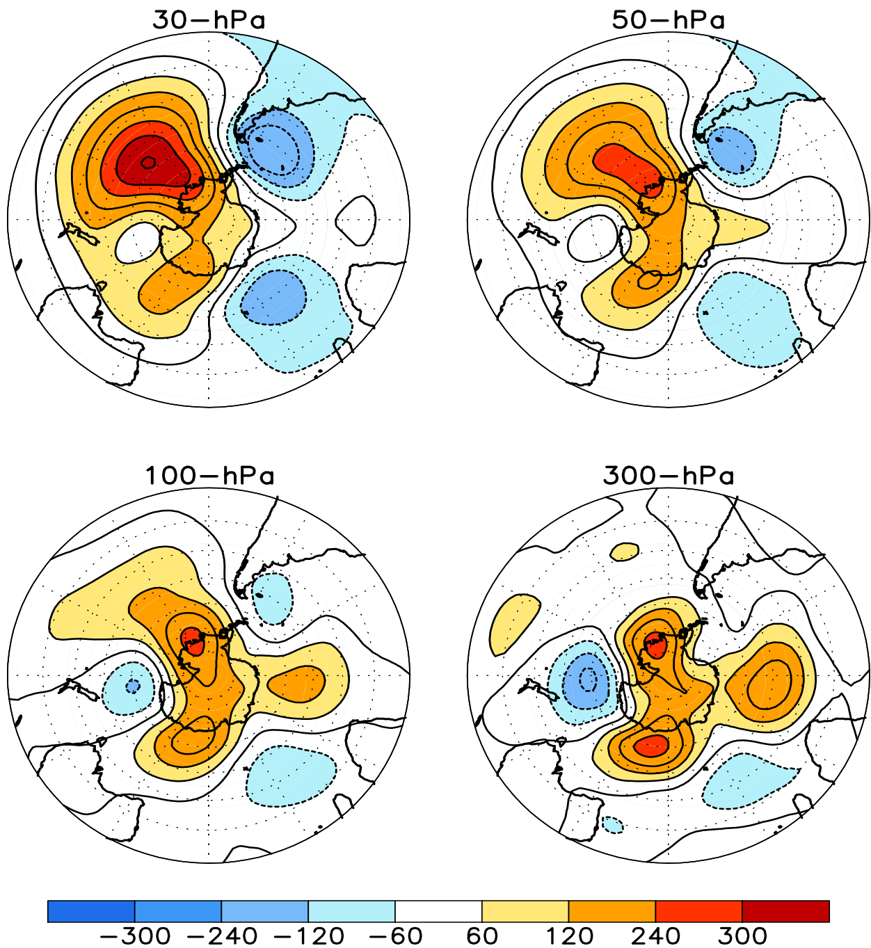
FIGURE S1. Stratospheric height anomalies (m) at selected levels for JUL 2011. Positive values are indicated by solid contours and dark shading. Negative values are indicated by dashed contours and light shading. Contour interval is 60 m. Anomalies are calculated from the 1981-2010 base period means. Winter Hemisphere is shown.
