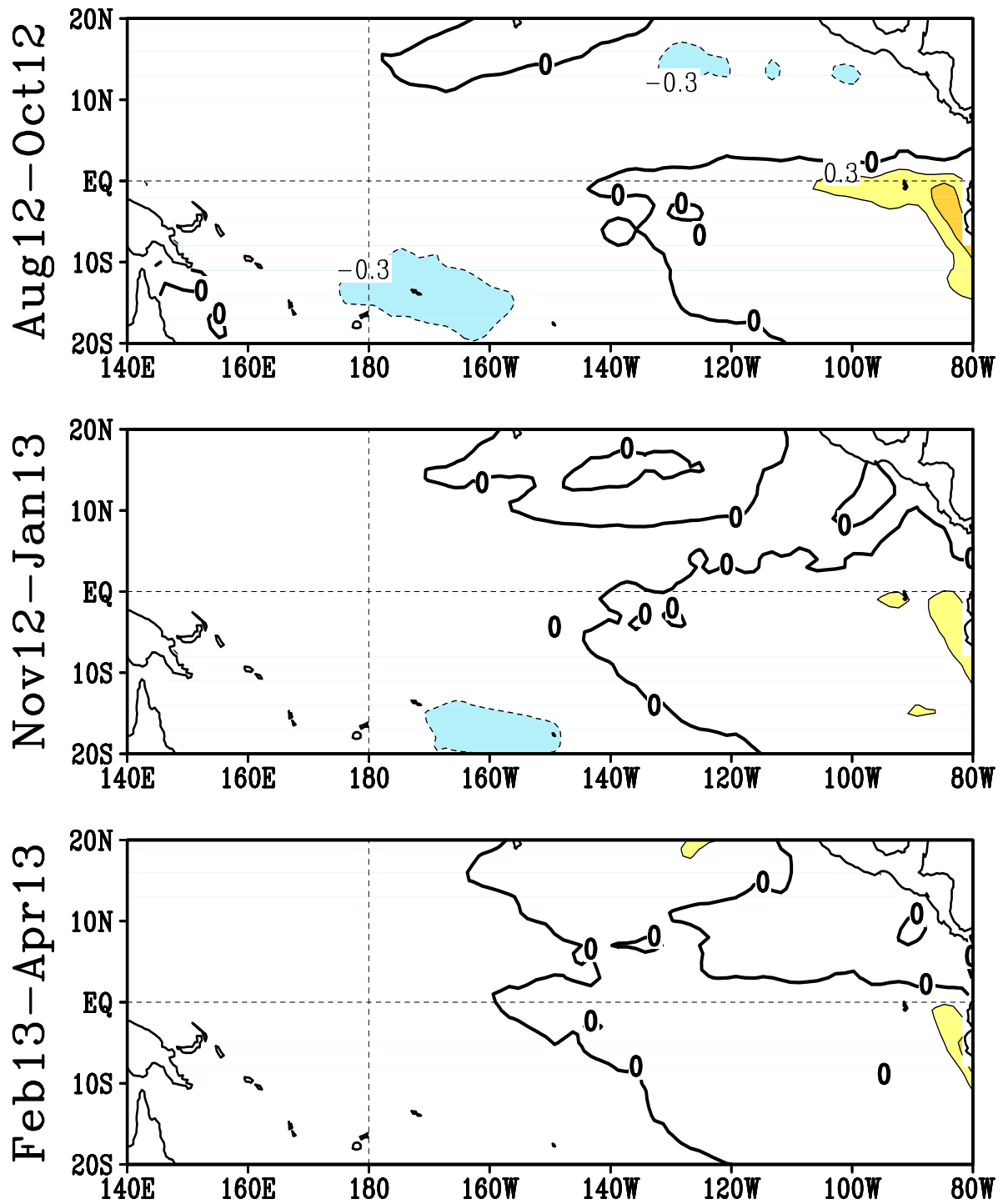
FIGURE F5. Predicted 3-month average sea surface temperature anomalies from the NCEP/CPC Markov model (Xue et al. 2000, J. Climate , 13 , 849-871). The forecast is initiated in JUL 2012 . Contour interval is 0.3C and negative anomalies are indicated by dashed contours. Anomalies are calculated relative to the 1971-2000 climatology.
