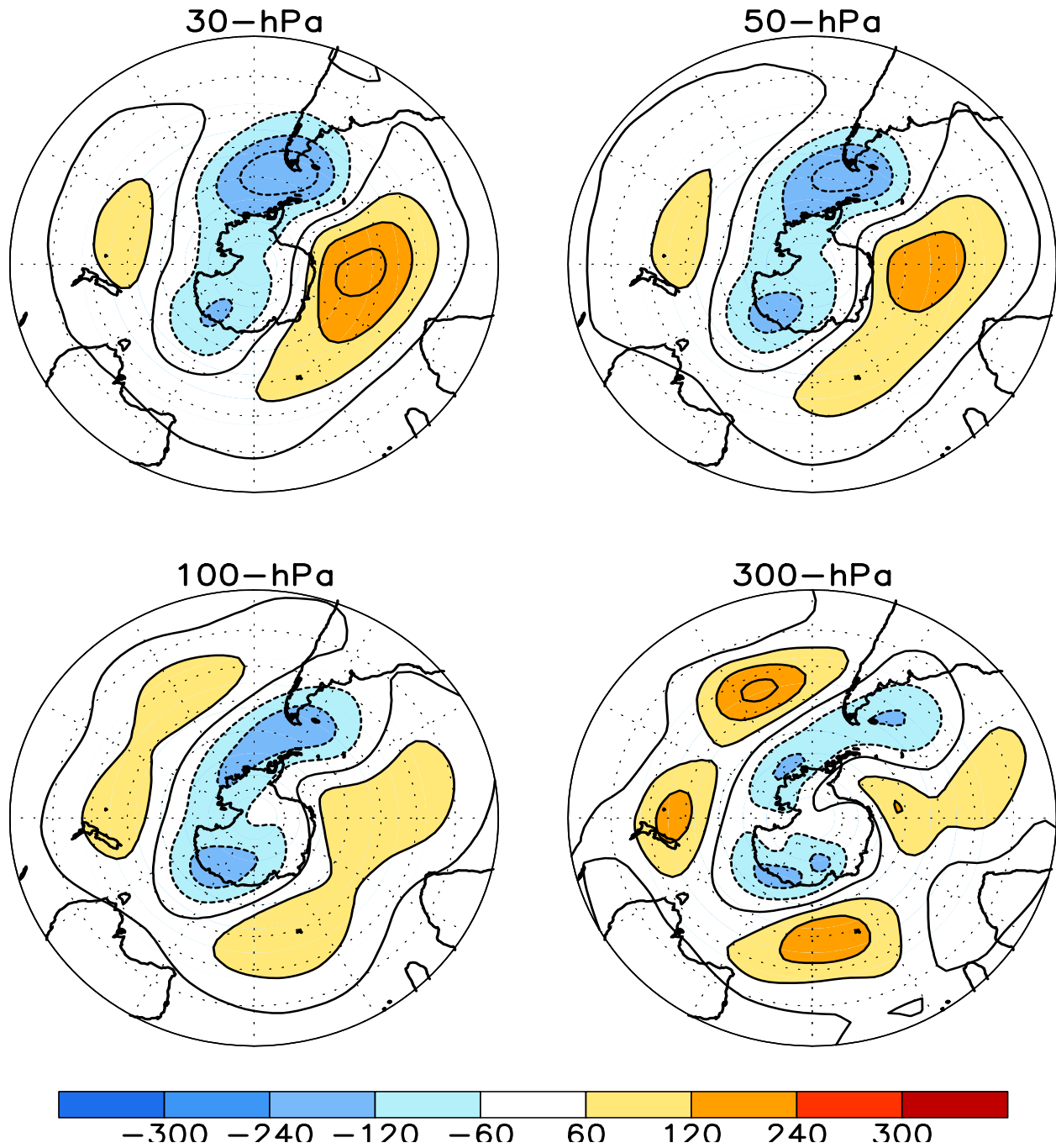
FIGURE S1. Stratospheric height anomalies (m) at selected levels for JUL 2012. Positive values are indicated by solid contours and dark shading. Negative values are indicated by dashed contours and light shading. Contour interval is 60 m. Anomalies are calculated from the 1981-2010 base period means. Winter Hemisphere is shown.
