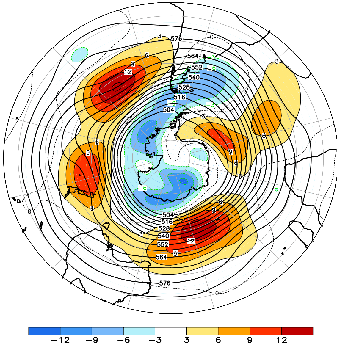
FIGURE E15. Southern Hemisphere mean and anomalous 500-hPa geopotential height (CDAS/Reanalysis) for JUL 2012. Mean heights are denoted by solid contours drawn at an interval of 6 dam. Anomaly contour interval is 3 dam with values less (greater) than -3 dam (3 dam) indicated by dark (light) shading. Anomalies are calculated as departures from the 1981-2010 base period monthly means.
