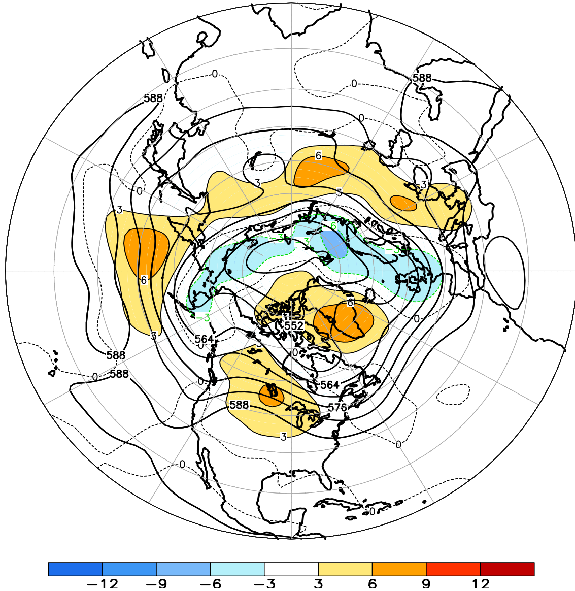
FIGURE E9. Northern Hemisphere mean and anomalous 500-hPa geopotential height (CDAS/Reanalysis) for JUL 2012. Mean heights are denoted by solid contours drawn at an interval of 6 dam. Anomaly contour interval is 3 dam with values less (greater) than -3 dam (3 dam) indicated by dark (light) shading. Anomalies are calculated as departures from the 1981-2010 base period monthly means.
