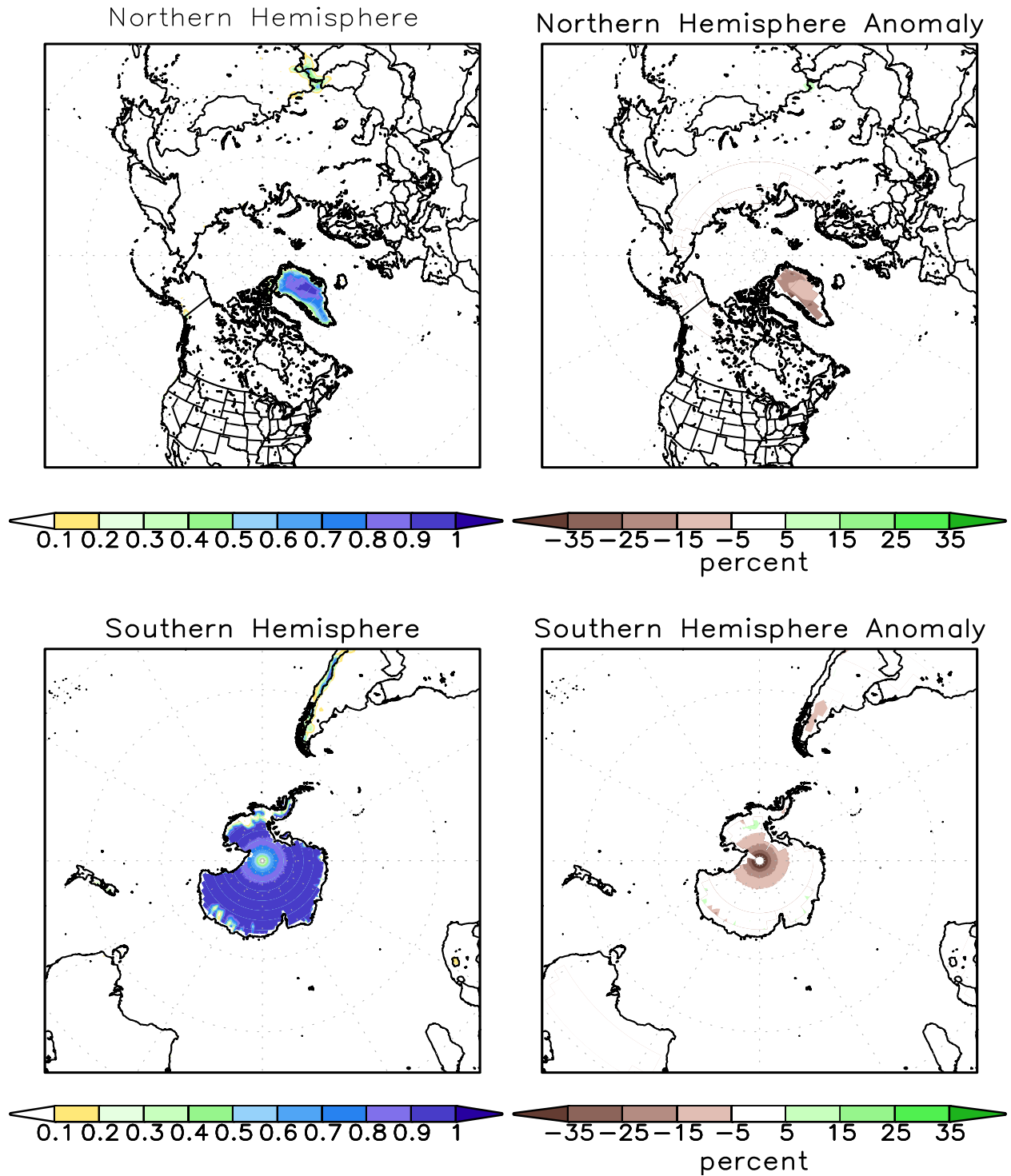
FIGURE A2.2. SSM/I derived snow cover frequency (%) (left) and snow cover anomaly (%) (right) for the month of JUL 2012 based on 1987 - 2010 base period for the Northern Hemisphere (top) and Southern Hemisphere (bottom). It is generated using the algorithm described by Ferraro et. al, 1996, Bull. Amer. Meteor. Soc., vol 77, 891-905.
