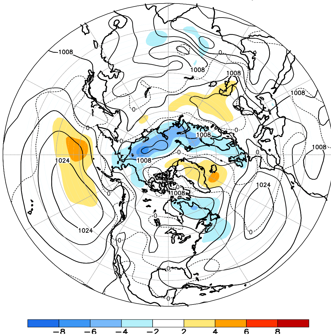
FIGURE E8. Northern Hemisphere mean and anomalous sea level pressure (CDAS/Reanalysis) for JUL 2012. Mean values are denoted by solid contours drawn at an interval of 4 hPa. Anomaly contour interval is 2 hPa with values less (greater) than -2 hPa (2 hPa) indicated by dark (light) shading. Anomalies are calculated as departures from the 1981-2010 base period monthly means.
