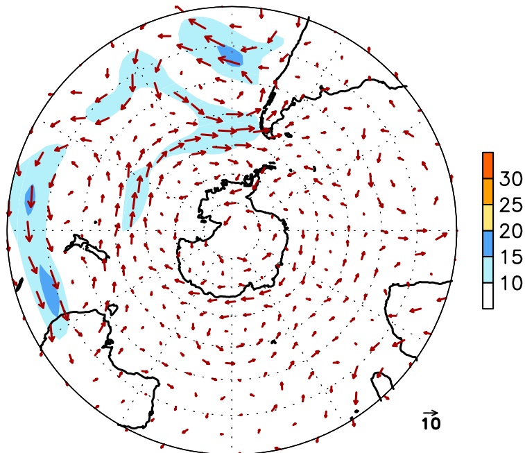
FIGURE E16. Southern Hemisphere mean (left) and anomalous (right) 300-hPa vector wind (CDAS/Reanalysis) for JUL 2013. Mean (anomaly) isotach contour interval is 10 (5) \text{ms}^{-1} . Values greater than 30 \text{ms}^{-1} (left) and 10 \text{ms}^{-1} (rights) are shaded. Anomalies are departures from the 1981-2010 base period monthly means.
