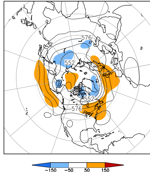
500-hPa Height (dm) & Anomalies (m) (Jul 1–15, 2013)
