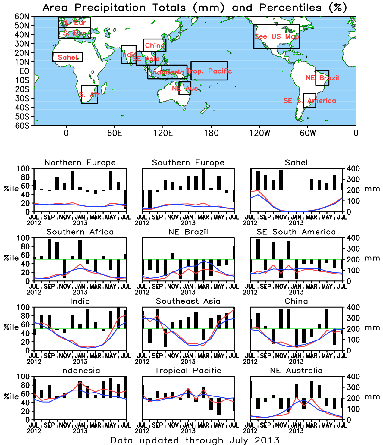
FIGURE E4. Areal estimates of monthly mean precipitation amounts (mm, solid lines) and precipitation percentiles (%ile, bars) for the most recent 13 months obtained from a merge of raingauge observations and satellite-derived precipitation estimates (Janowiak and Xie 1999, J. Climate , 12, 3335–3342). The monthly precipitation climatology (mm, dashed lines) is from the 1981–2010 base period monthly means. Monthly percentiles are not shown if the monthly mean is less than 5 mm.
