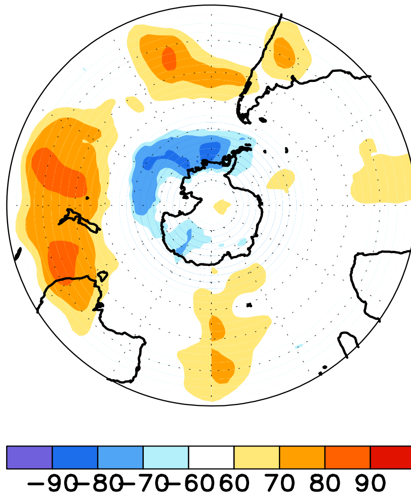
FIGURE E17. Southern Hemisphere percentage of days during JUL 2013 in which 500-hPa height anomalies greater than 15 m (red) and less than -15 m (blue) were observed. Values greater than 70% are shaded and contour in-
