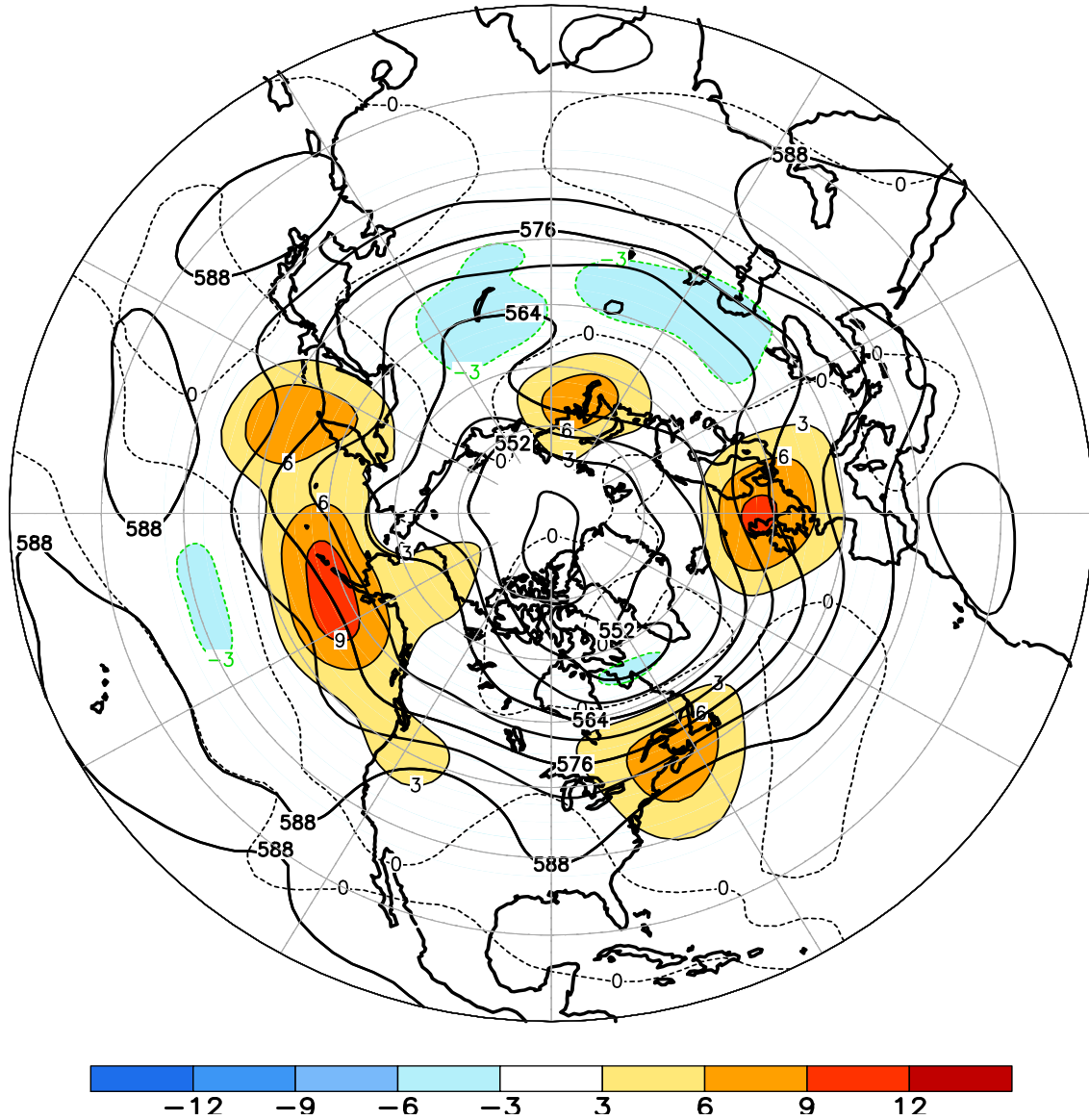
FIGURE E9. Northern Hemisphere mean and anomalous 500-hPa geopotential height (CDAS/Reanalysis) for JUL 2013. Mean heights are denoted by solid contours drawn at an interval of 6 dam. Anomaly contour interval is 3 dam with values less (greater) than -3 dam (3 dam) indicated by dark (light) shading. Anomalies are calculated as departures from the 1981-2010 base period monthly means.
