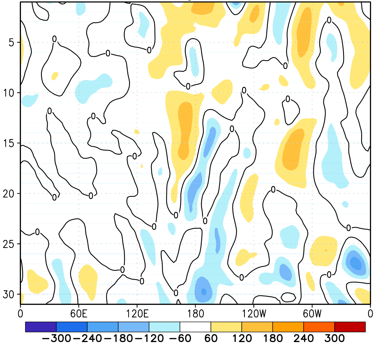
FIGURE E12. Northern Hemisphere: Daily 500-hPa height anomalies for JUL 2013 averaged over the 5° latitude band centered on 40°N. Positive values are indicated by solid contours and dark shading. Negative values are indicated by dashed contours and light shading. Contour interval is 60 m. Anomalies are departures from the 1981-2010 base period daily means.
