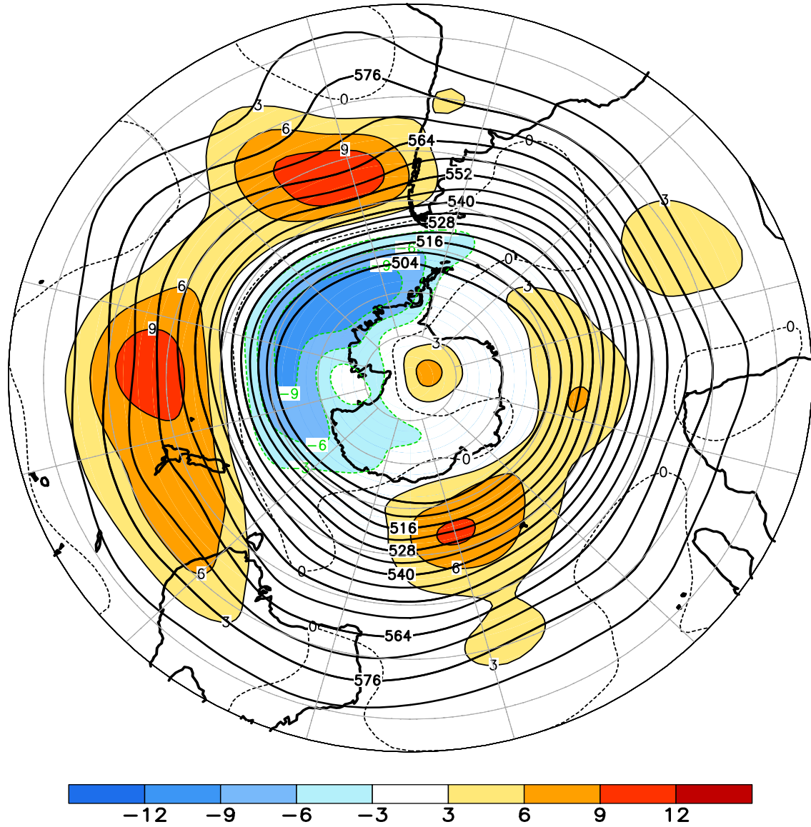
FIGURE E15. Southern Hemisphere mean and anomalous 500-hPa geopotential height (CDAS/Reanalysis) for JUL 2013. Mean heights are denoted by solid contours drawn at an interval of 6 dam. Anomaly contour interval is 3 dam with values less (greater) than -3 dam (3 dam) indicated by dark (light) shading. Anomalies are calculated as departures from the 1981-2010 base period monthly means.
