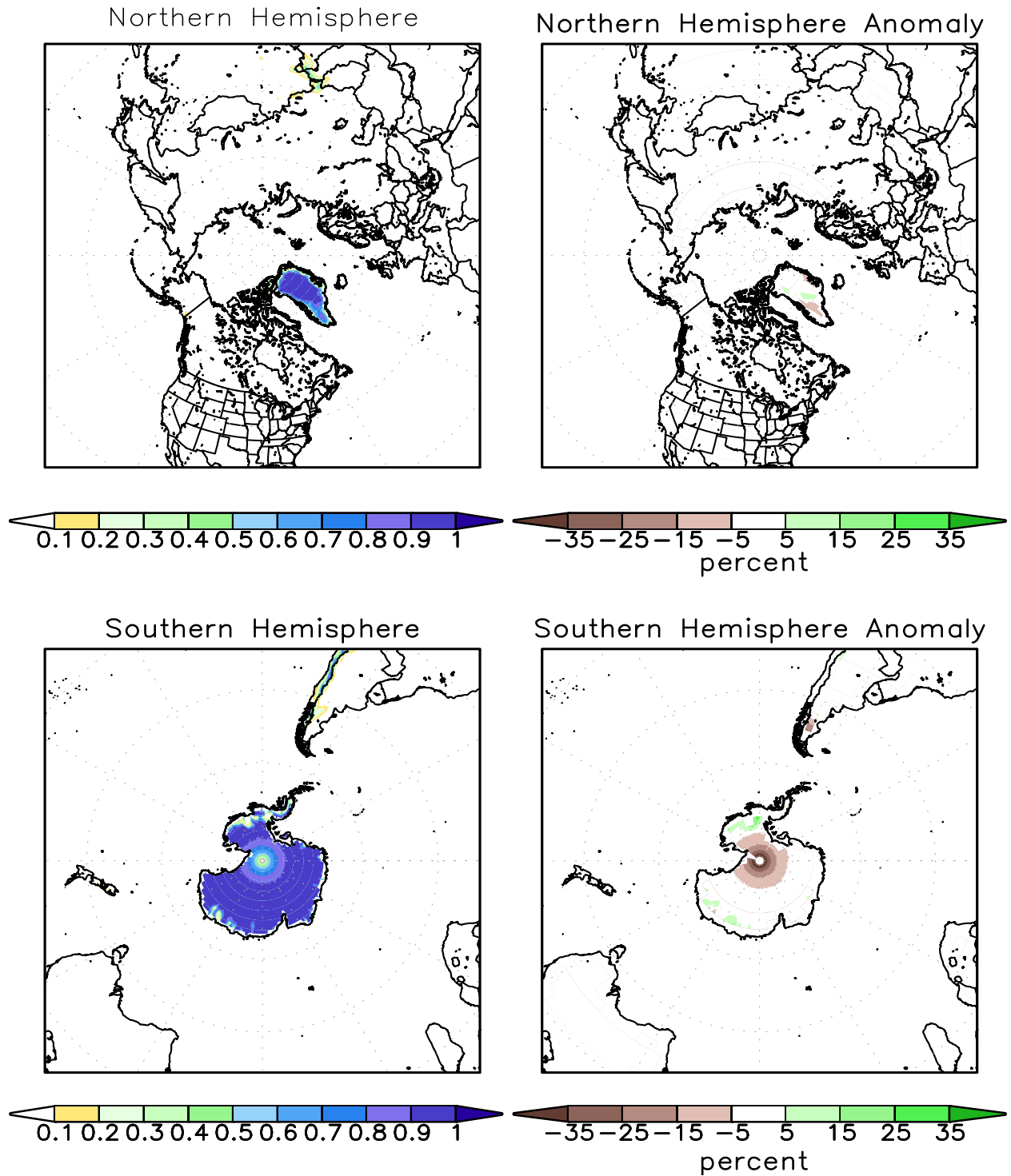
FIGURE A2.2. SSM/I derived snow cover frequency (%) (left) and snow cover anomaly (%) (right) for the month of JUL 2013 based on 1987 - 2010 base period for the Northern Hemisphere (top) and Southern Hemisphere (bottom). It is generated using the algorithm described by Ferraro et. al, 1996, Bull. Amer. Meteor. Soc., vol 77, 891-905.
