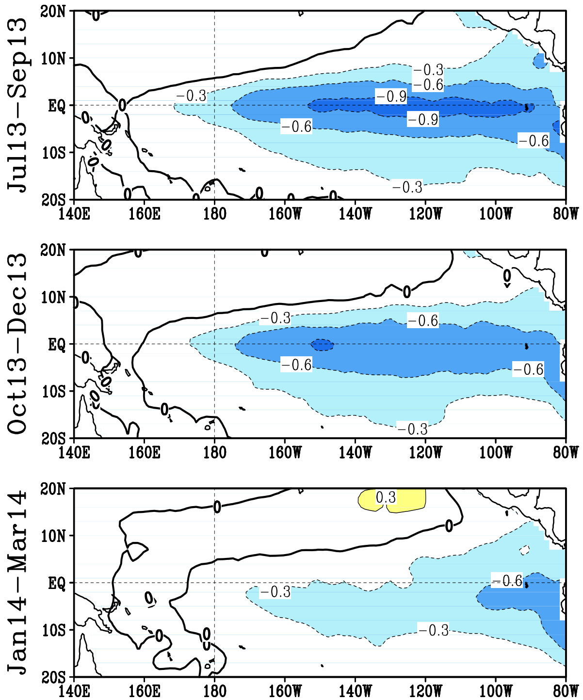
FIGURE F5. Predicted 3-month average sea surface temperature anomalies from the NCEP/CPC Markov model (Xue et al. 2000, J. Climate , 13 , 849-871). The forecast is initiated in JUL 2013 . Contour interval is 0.3C and negative anomalies are indicated by dashed contours. Anomalies are calculated relative to the 1971-2000 climatology.
