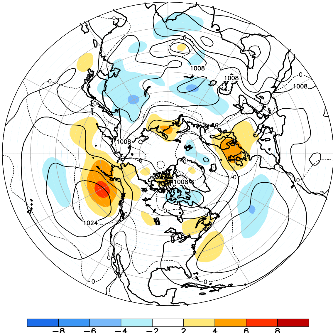
FIGURE E8. Northern Hemisphere mean and anomalous sea level pressure (CDAS/Reanalysis) for JUL 2013. Mean values are denoted by solid contours drawn at an interval of 4 hPa. Anomaly contour interval is 2 hPa with values less (greater) than -2 hPa (2 hPa) indicated by dark (light) shading. Anomalies are calculated as departures from the 1981-2010 base period monthly means.
