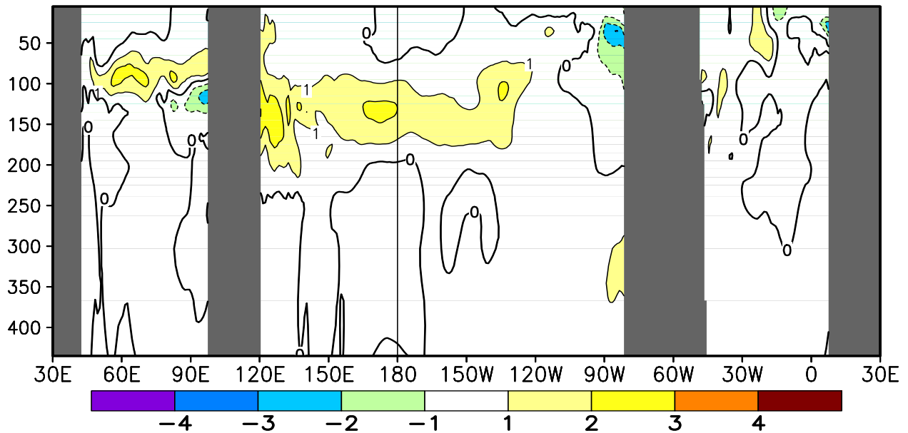
FIGURE T17. Equatorial depth–longitude section of ocean temperature (top) and ocean temperature anomalies (bottom) for JUL 2013. Contour interval is 1°C. Dashed contours in bottom panel indicate negative anomalies. Data are derived from the NCEP’s global ocean data assimilation system version 2 which assimilates oceanic observations into an oceanic GCM (Xue, Y. and Behringer, D.W., 2006: Operational global ocean data assimilation system at NCEP, to be submitted to BAMS). Anomalies are departures from the 1981–2010 base period means.
