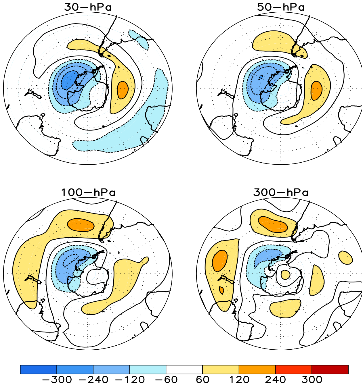
FIGURE S1. Stratospheric height anomalies (m) at selected levels for JUL 2013. Positive values are indicated by solid contours and dark shading. Negative values are indicated by dashed contours and light shading. Contour interval is 60 m. Anomalies are calculated from the 1981-2010 base period means. Winter Hemisphere is shown.
