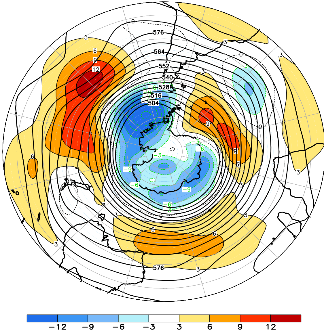
FIGURE E15. Southern Hemisphere mean and anomalous 500-hPa geopotential height (CDAS/Reanalysis) for JUN 2010. Mean heights are denoted by solid contours drawn at an interval of 6 dam. Anomaly contour interval is 3 dam with values less (greater) than -3 dam (3 dam) indicated by dark (light) shading. Anomalies are calculated as departures from the 1979-95 base period monthly means.
