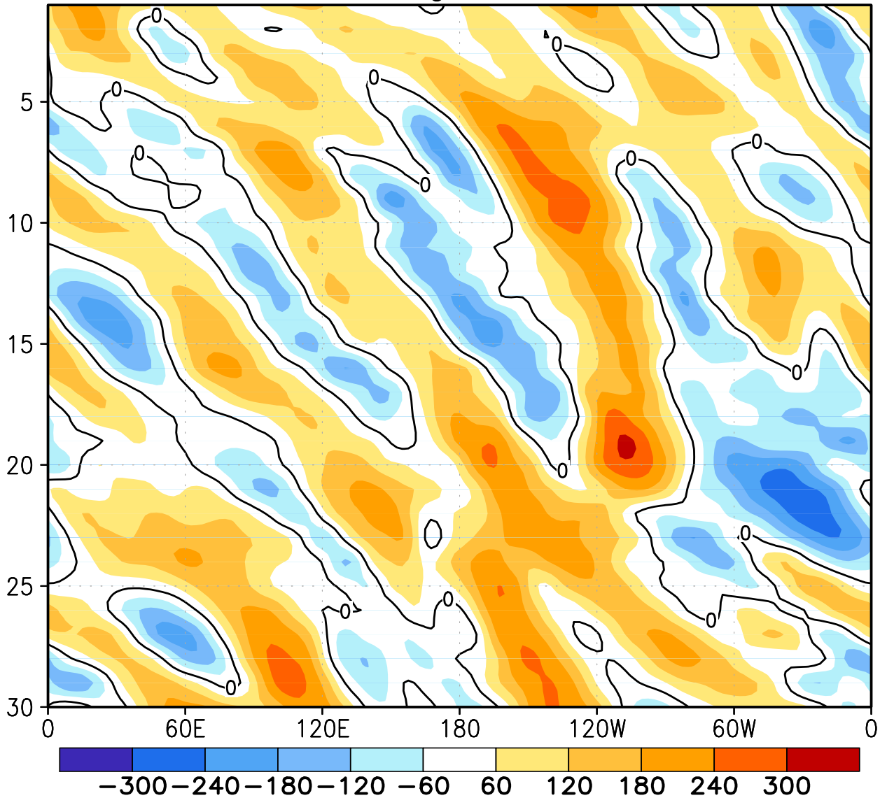
FIGURE E18. Southern Hemisphere: Daily 500-hPa height anomalies for JUN 2010 averaged over the 5° latitude band centered on 40°S. Positive values are indicated by solid contours and dark shading. Negative values are indicated by dashed contours and light shading. Contour interval is 60 m. Anomalies are departures from the 1979-95 base period daily means.
