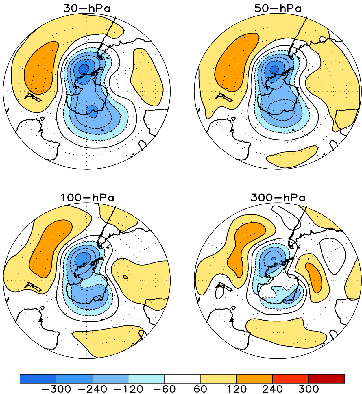
FIGURE S1. Stratospheric height anomalies (m) at selected levels for JUN 2010. Positive values are indicated by solid contours and dark shading. Negative values are indicated by dashed contours and light shading. Contour interval is 60 m. Anomalies are calculated from the 1979–95 base period means. Winter Hemisphere is shown.
