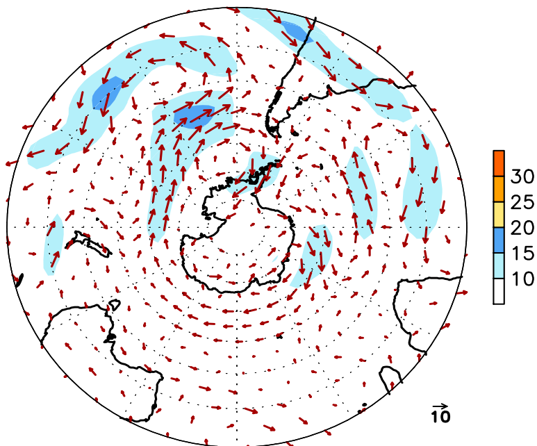
FIGURE E16. Southern Hemisphere mean (left) and anomalous (right) 300-hPa vector wind (CDAS/Reanalysis) for JUN 2010. Mean (anomaly) isotach contour interval is 10 (5) \text{ms}^{-1} . Values greater than 30 \text{ms}^{-1} (left) and 10 \text{ms}^{-1} (rights) are shaded. Anomalies are departures from the 1979-95 base period monthly means.
