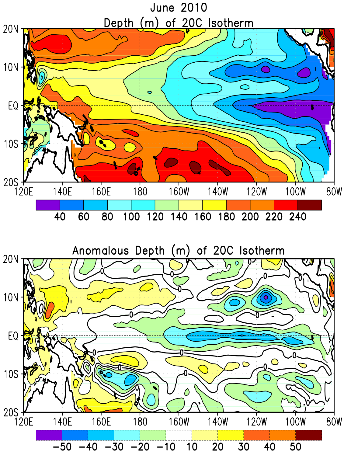
FIGURE T16. Mean (top) and anomalous (bottom) depth of the 20°C isotherm for JUN 2010. Contour interval is 40 m (top) and 10 m (bottom). Dashed contours in bottom panel indicate negative anomalies. Data are derived from the NCEP’s global ocean data assimilation system version 2 which assimilates oceanic observations into an oceanic GCM (Xue, Y. and Behringer, D.W., 2006: Operational global ocean data assimilation system at NCEP, to be submitted to BAMS). Anomalies are departures from the 1982–2004 base period means.
