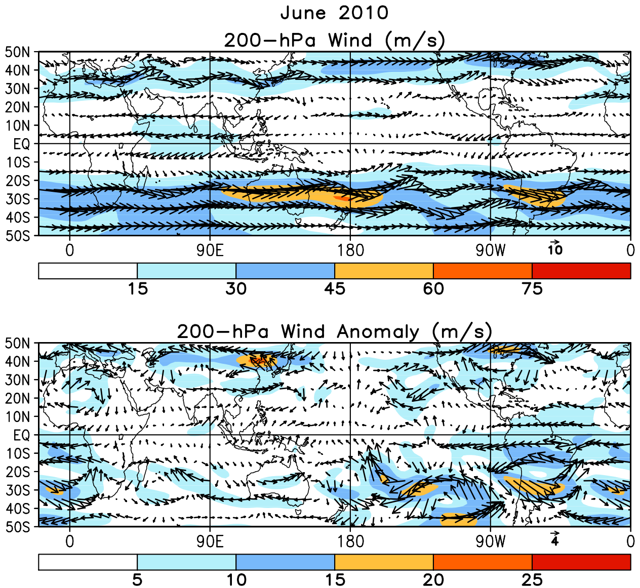
FIGURE T21. Mean (top) and anomalous (bottom) 200-hPa vector wind (CDAS/Reanalysis) for JUN 2010. Contour interval for isotachs is 15 \text{ ms}^{-1} (top) and 5 \text{ ms}^{-1} (bottom). Anomalies are departures from 1979–95 base period monthly means.
