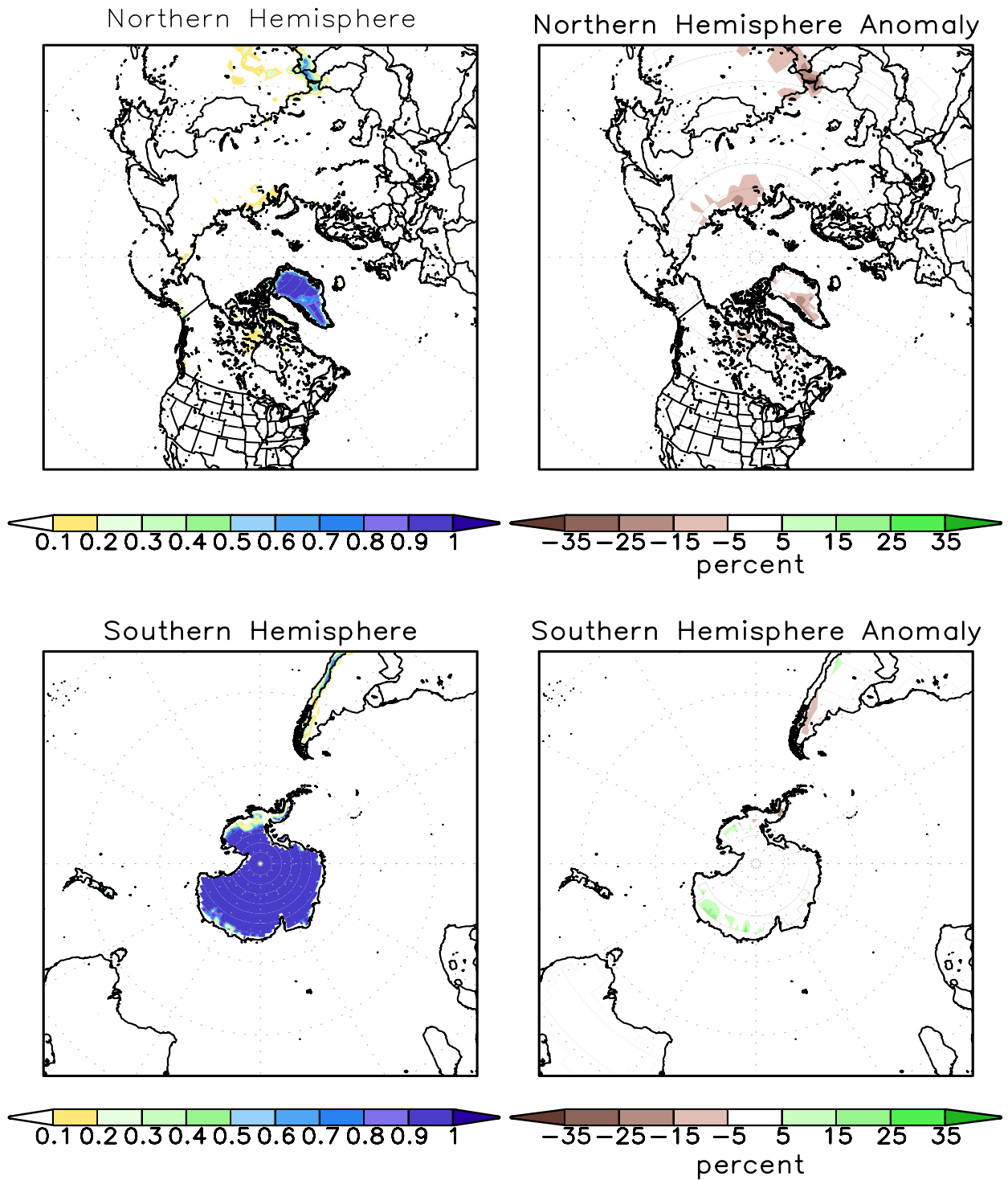
FIGURE A2.2. SSM/I derived snow cover frequency (%) (left) and snow cover anomaly (%) (right) for the month of JUN 2010 based on 1987 - 2006 base period for the Northern Hemisphere (top) and Southern Hemisphere (bottom). It is generated using the algorithm described by Ferraro et. al, 1996, Bull. Amer. Meteor. Soc., vol 77, 891-905.
