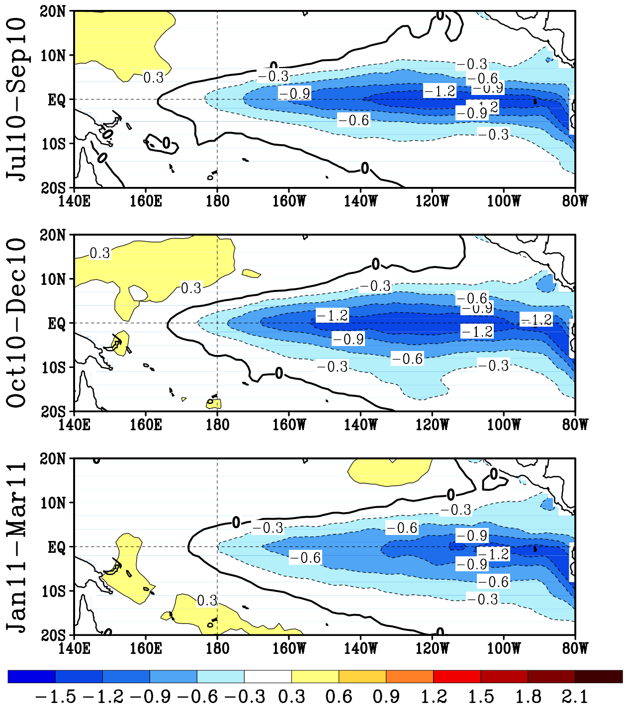
FIGURE F5. Predicted 3-month average sea surface temperature anomalies from the NCEP/CPC Markov model (Xue et al. 2000, J. Climate , 13 , 849-871). The forecast is initiated in JUN 2010 . Contour interval is 0.3C and negative anomalies are indicated by dashed contours. Anomalies are calculated relative to the 1971-2000 climatology.
