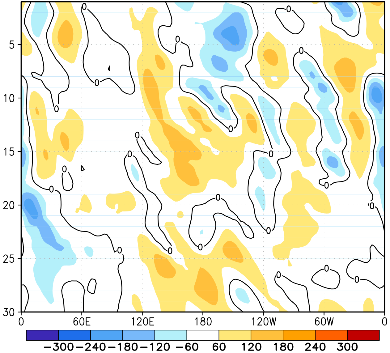
FIGURE E12. Northern Hemisphere: Daily 500-hPa height anomalies for JUN 2010 averaged over the 5° latitude band centered on 40°N. Positive values are indicated by solid contours and dark shading. Negative values are indicated by dashed contours and light shading. Contour interval is 60 m. Anomalies are departures from the 1979-95 base period daily means.
