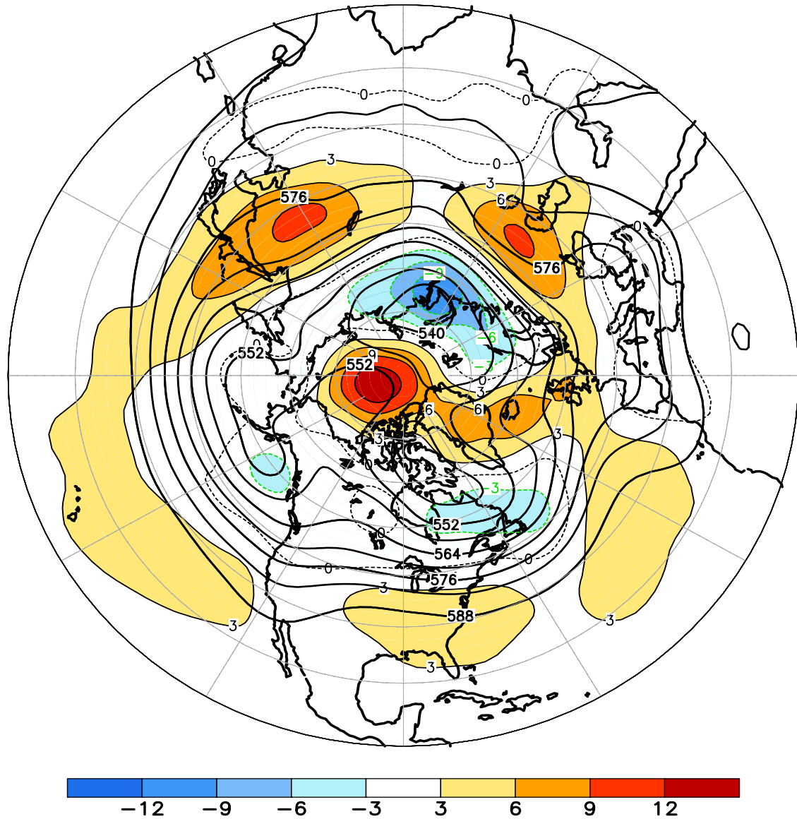
FIGURE E9. Northern Hemisphere mean and anomalous 500-hPa geopotential height (CDAS/Reanalysis) for JUN 2010. Mean heights are denoted by solid contours drawn at an interval of 6 dam. Anomaly contour interval is 3 dam with values less (greater) than -3 dam (3 dam) indicated by dark (light) shading. Anomalies are calculated as departures from the 1979-95 base period monthly means.
