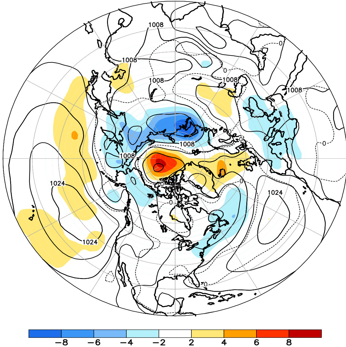
FIGURE E8. Northern Hemisphere mean and anomalous sea level pressure (CDAS/Reanalysis) for JUN 2010. Mean values are denoted by solid contours drawn at an interval of 4 hPa. Anomaly contour interval is 2 hPa with values less (greater) than -2 hPa (2 hPa) indicated by dark (light) shading. Anomalies are calculated as departures from the 1979-95 base period monthly means.
