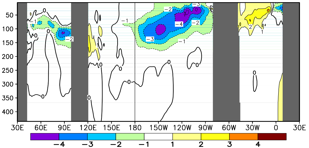
FIGURE T17. Equatorial depth–longitude section of ocean temperature (top) and ocean temperature anomalies (bottom) for JUN 2010. Contour interval is 1°C. Dashed contours in bottom panel indicate negative anomalies. Data are derived from the NCEP’s global ocean data assimilation system version 2 which assimilates oceanic observations into an oceanic GCM (Xue, Y. and Behringer, D.W., 2006: Operational global ocean data assimilation system at NCEP, to be submitted to BAMS). Anomalies are departures from the 1982–2004 base period means.
