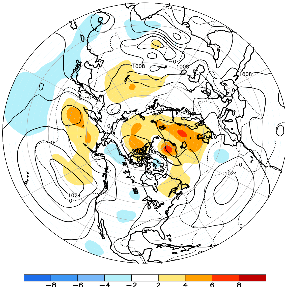
FIGURE E8. Northern Hemisphere mean and anomalous sea level pressure (CDAS/Reanalysis) for JUN 2014. Mean values are denoted by solid contours drawn at an interval of 4 hPa. Anomaly contour interval is 2 hPa with values less (greater) than -2 hPa (2 hPa) indicated by dark (light) shading. Anomalies are calculated as departures from the 1981-2010 base period monthly means.
