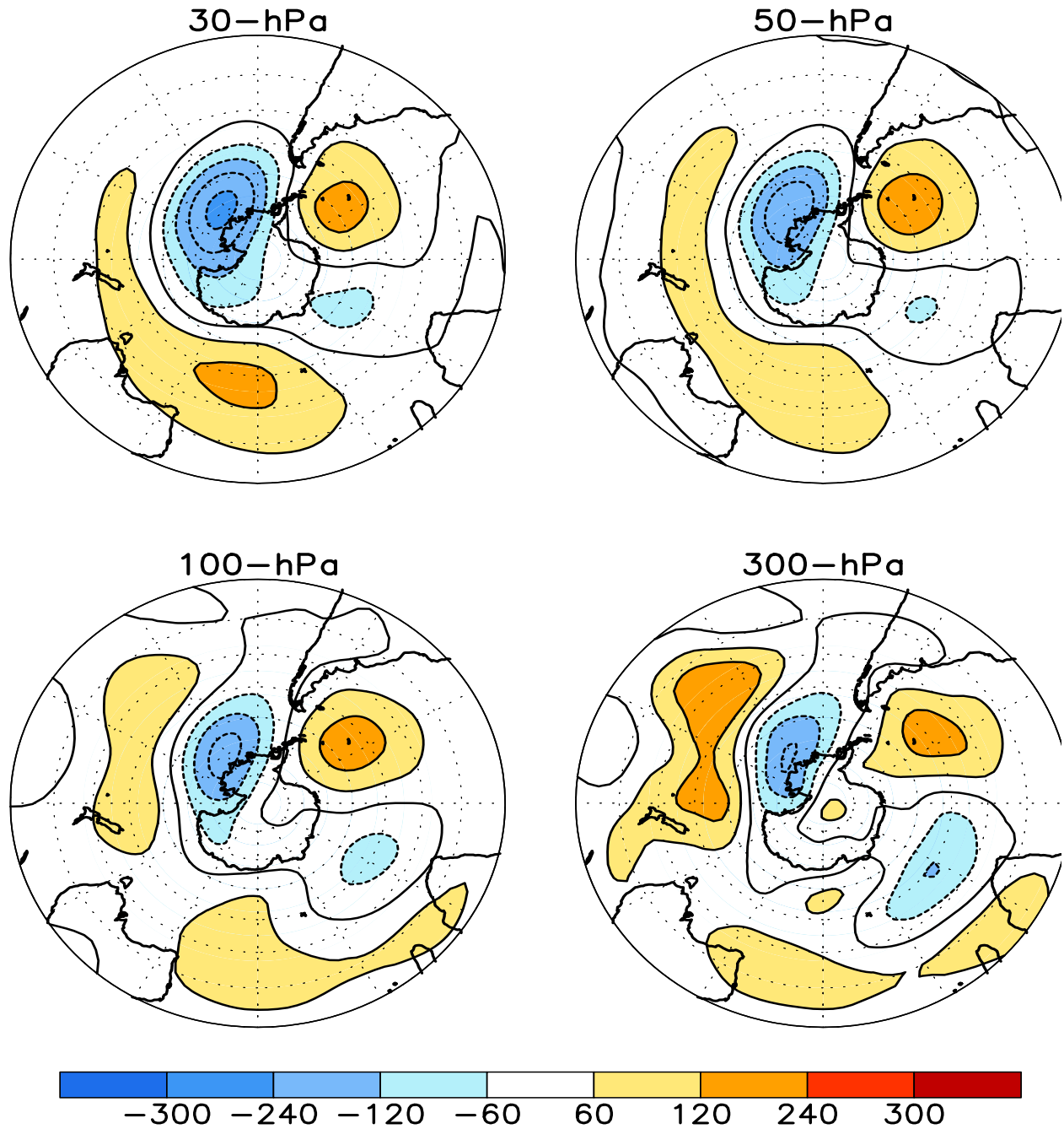
FIGURE S1. Stratospheric height anomalies (m) at selected levels for JUN 2014. Positive values are indicated by solid contours and dark shading. Negative values are indicated by dashed contours and light shading. Contour interval is 60 m. Anomalies are calculated from the 1981-2010 base period means. Winter Hemisphere is shown.
