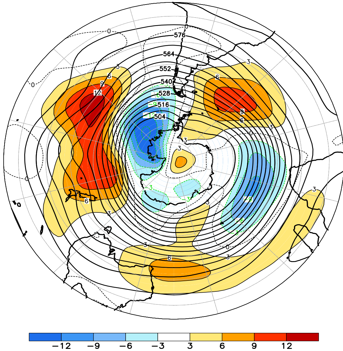
FIGURE E15. Southern Hemisphere mean and anomalous 500-hPa geopotential height (CDAS/Reanalysis) for JUN 2014. Mean heights are denoted by solid contours drawn at an interval of 6 dam. Anomaly contour interval is 3 dam with values less (greater) than -3 dam (3 dam) indicated by dark (light) shading. Anomalies are calculated as departures from the 1981-2010 base period monthly means.
