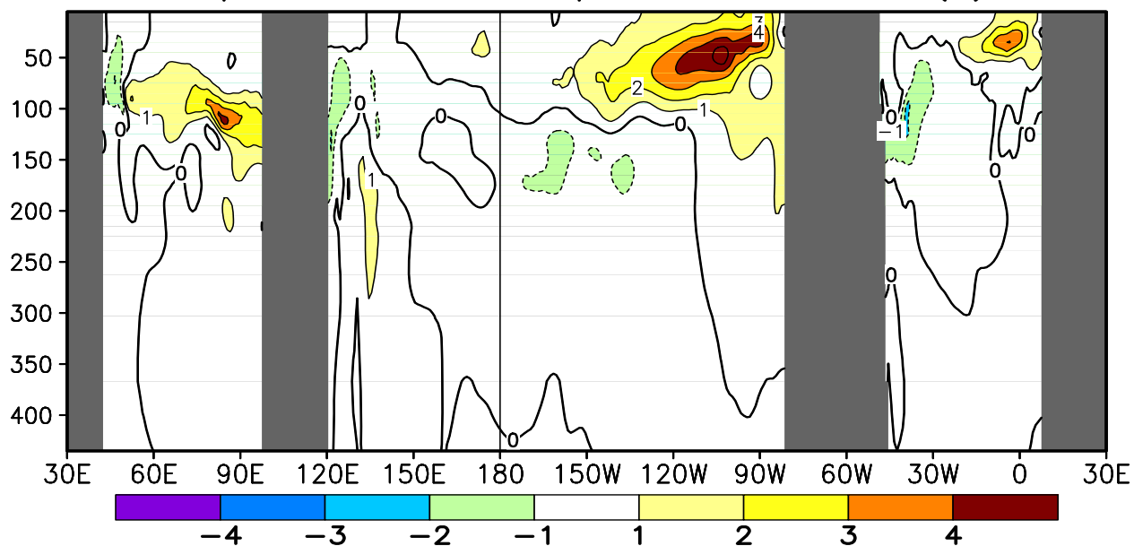
FIGURE T17. Equatorial depth–longitude section of ocean temperature (top) and ocean temperature anomalies (bottom) for JUN 2014. Contour interval is 1°C. Dashed contours in bottom panel indicate negative anomalies. Data are derived from the NCEP’s global ocean data assimilation system version 2 which assimilates oceanic observations into an oceanic GCM (Xue, Y. and Behringer, D.W., 2006: Operational global ocean data assimilation system at NCEP, to be submitted to BAMS). Anomalies are departures from the 1981–2010 base period means.
