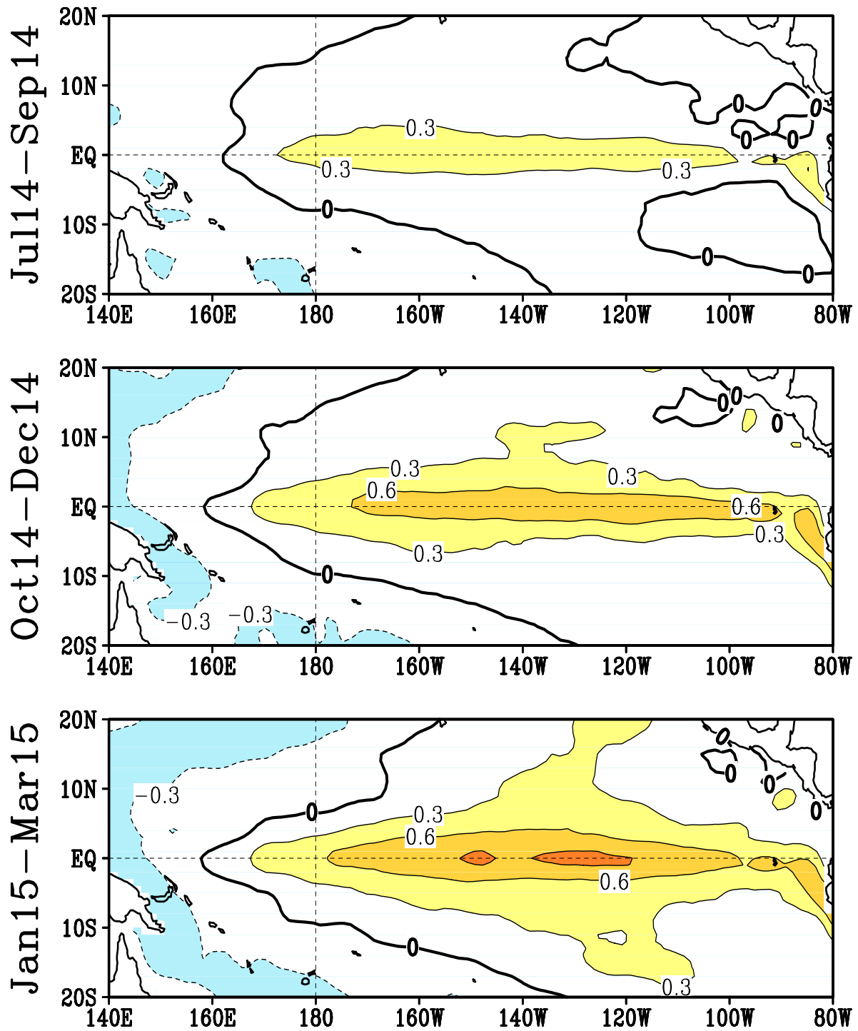
FIGURE F5. Predicted 3-month average sea surface temperature anomalies from the NCEP/CPC Markov model (Xue et al. 2000, J. Climate , 13 , 849-871). The forecast is initiated in JUN 2014 . Contour interval is 0.3C and negative anomalies are indicated by dashed contours. Anomalies are calculated relative to the 1971-2000 climatology.
