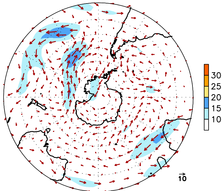
FIGURE E16. Southern Hemisphere mean (left) and anomalous (right) 300-hPa vector wind (CDAS/Reanalysis) for JUN 2014. Mean (anomaly) isotach contour interval is 10 (5) \text{ms}^{-1} . Values greater than 30 \text{ms}^{-1} (left) and 10 \text{ms}^{-1} (rights) are shaded. Anomalies are departures from the 1981-2010 base period monthly means.
