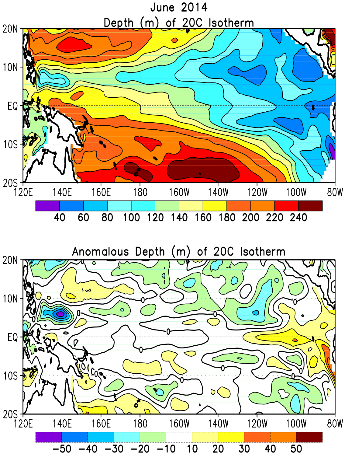
FIGURE T16. Mean (top) and anomalous (bottom) depth of the 20°C isotherm for JUN 2014. Contour interval is 40 m (top) and 10 m (bottom). Dashed contours in bottom panel indicate negative anomalies. Data are derived from the NCEP’s global ocean data assimilation system version 2 which assimilates oceanic observations into an oceanic GCM (Xue, Y. and Behringer, D.W., 2006: Operational global ocean data assimilation system at NCEP, to be submitted to BAMS). Anomalies are departures from the 1981–2010 base period means.
