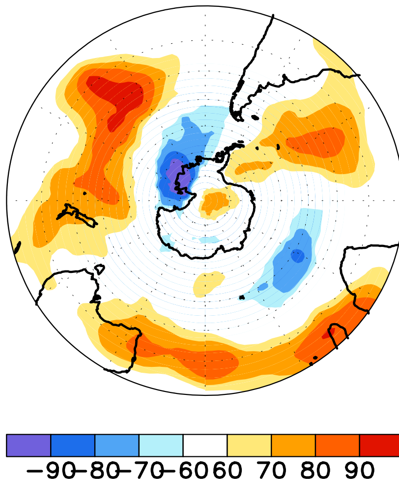
FIGURE E17. Southern Hemisphere percentage of days during JUN 2014 in which 500-hPa height anomalies greater than 15 m (red) and less than -15 m (blue) were observed. Values greater than 70% are shaded and contour in-
