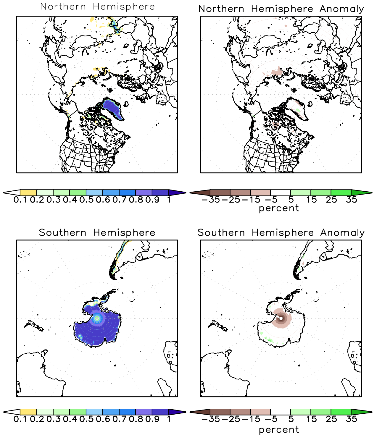
FIGURE A2.2. SSM/I derived snow cover frequency (%) (left) and snow cover anomaly (%) (right) for the month of JUN 2014 based on 1987 - 2010 base period for the Northern Hemisphere (top) and Southern Hemisphere (bottom). It is generated using the algorithm described by Ferraro et. al, 1996, Bull. Amer. Meteor. Soc., vol 77, 891-905.
