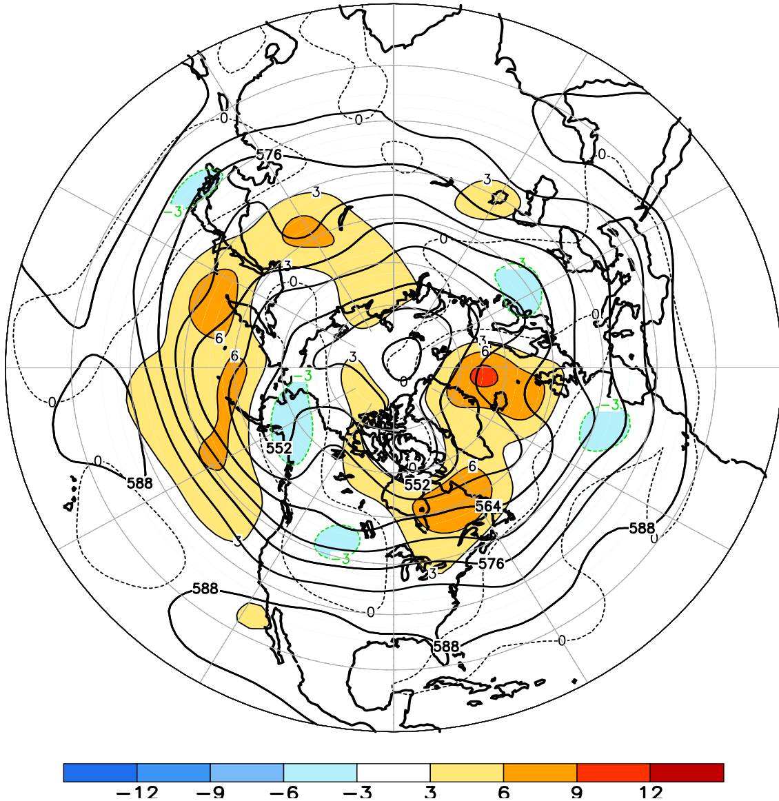
FIGURE E9. Northern Hemisphere mean and anomalous 500-hPa geopotential height (CDAS/Reanalysis) for JUN 2014. Mean heights are denoted by solid contours drawn at an interval of 6 dam. Anomaly contour interval is 3 dam with values less (greater) than -3 dam (3 dam) indicated by dark (light) shading. Anomalies are calculated as departures from the 1981-2010 base period monthly means.
