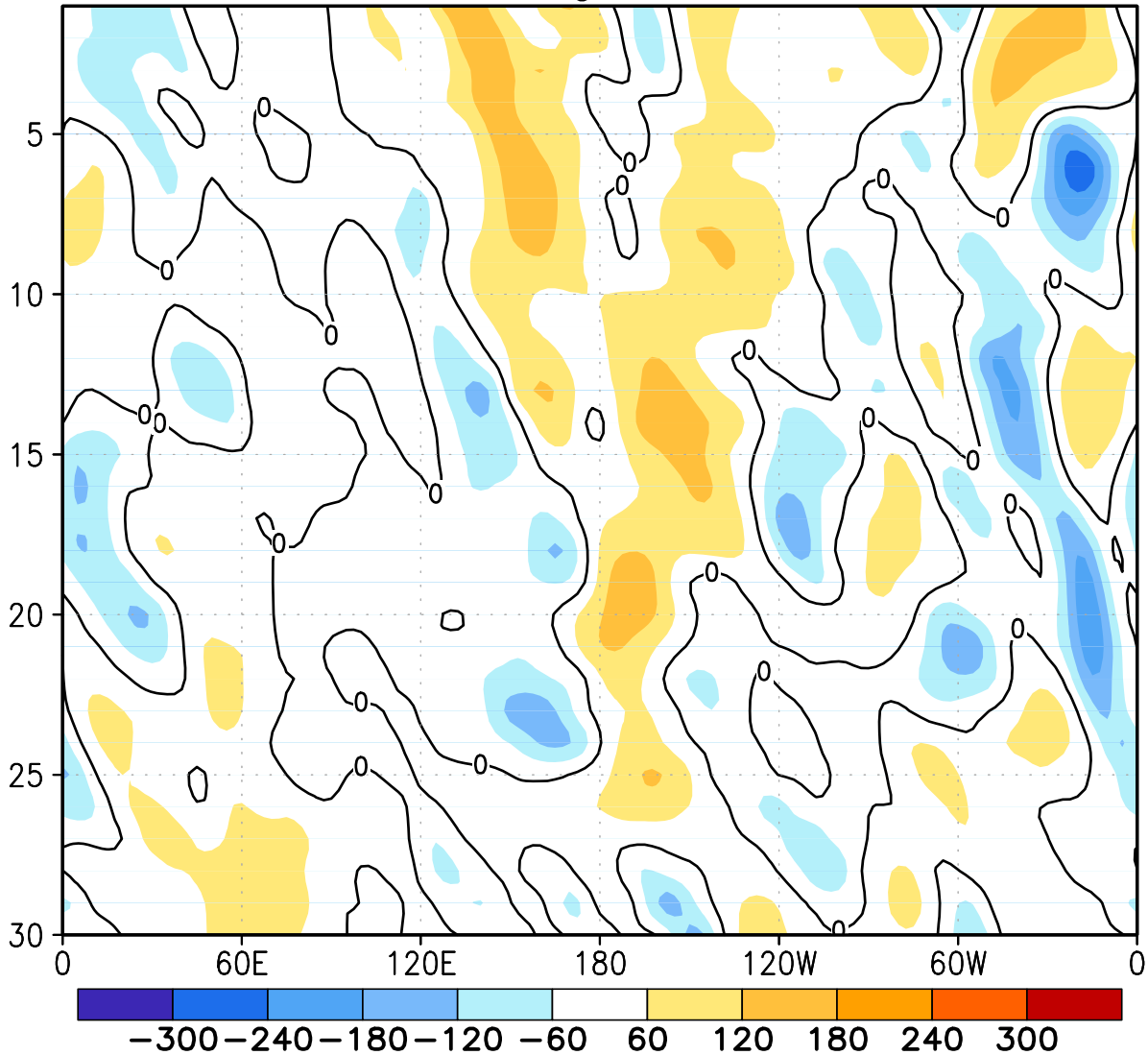
FIGURE E12. Northern Hemisphere: Daily 500-hPa height anomalies for JUN 2014 averaged over the 5° latitude band centered on 40°N. Positive values are indicated by solid contours and dark shading. Negative values are indicated by dashed contours and light shading. Contour interval is 60 m. Anomalies are departures from the 1981-2010 base period daily means.
