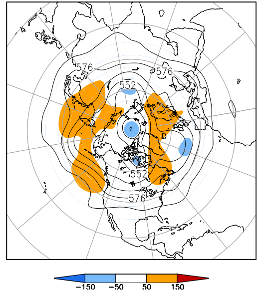
500-hPa Height (dm) & Anomalies (m) (Jun 1–15, 2014)
