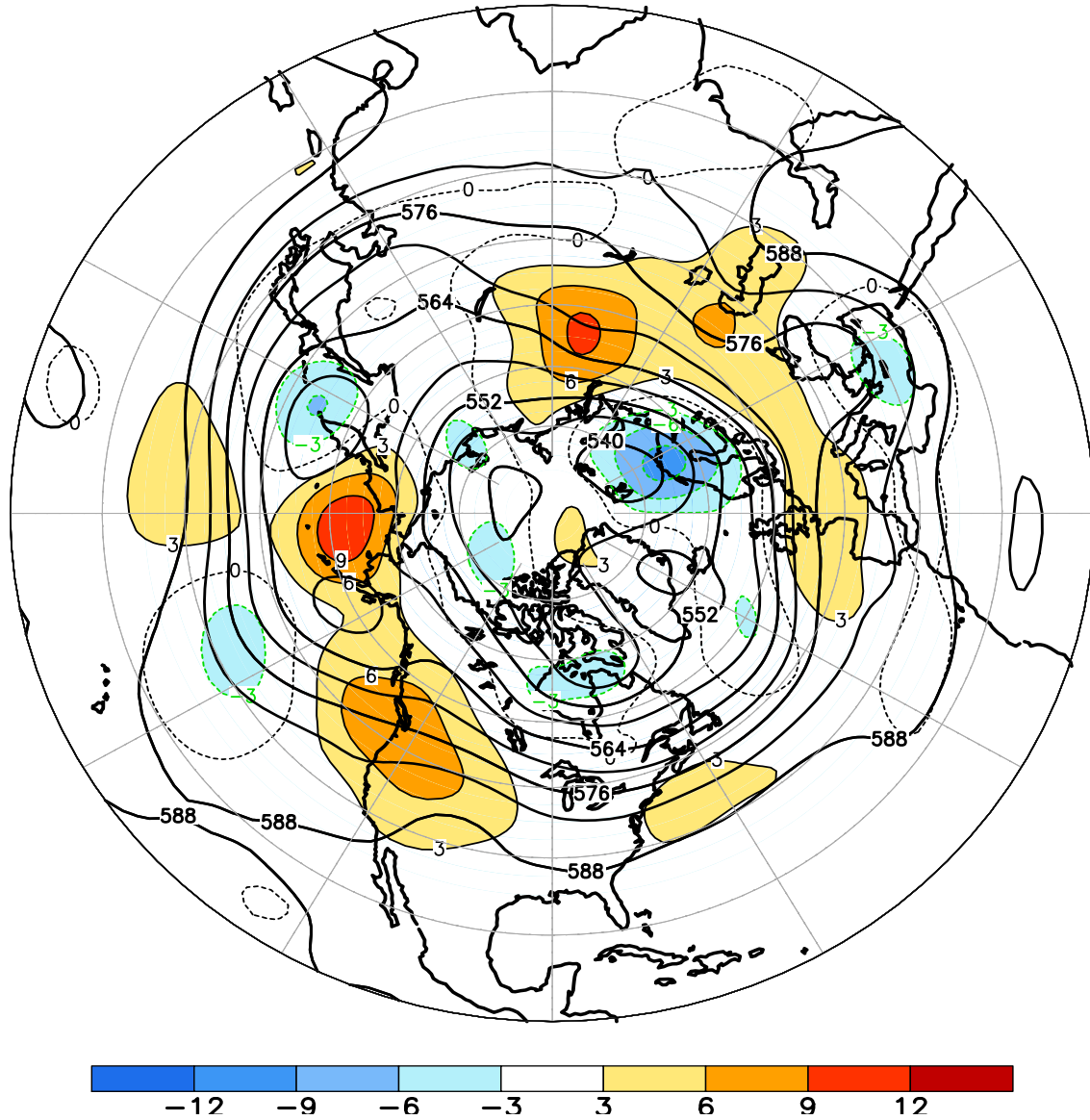
FIGURE E9. Northern Hemisphere mean and anomalous 500-hPa geopotential height (CDAS/Reanalysis) for JUN 2015. Mean heights are denoted by solid contours drawn at an interval of 6 dam. Anomaly contour interval is 3 dam with values less (greater) than -3 dam (3 dam) indicated by dark (light) shading. Anomalies are calculated as departures from the 1981-2010 base period monthly means.
