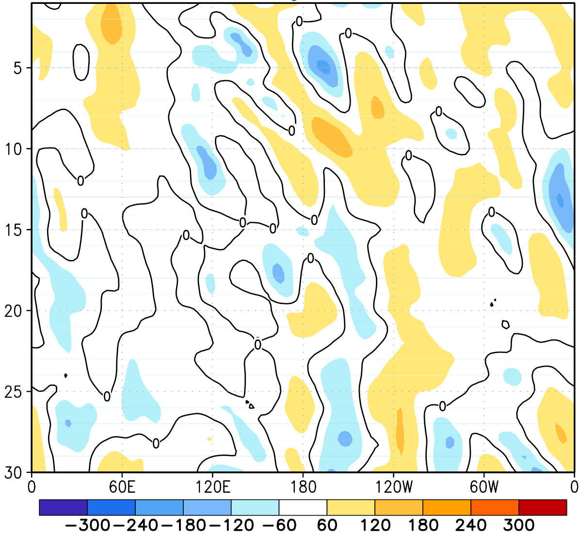
FIGURE E12. Northern Hemisphere: Daily 500-hPa height anomalies for JUN 2015 averaged over the 5° latitude band centered on 40°N. Positive values are indicated by solid contours and dark shading. Negative values are indicated by dashed contours and light shading. Contour interval is 60 m. Anomalies are departures from the 1981-2010 base period daily means.
