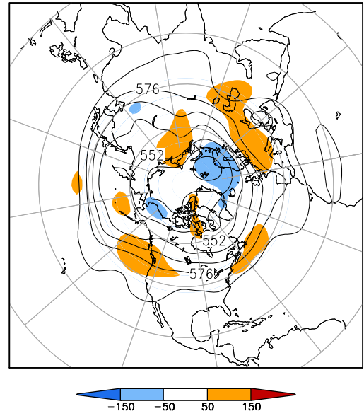
500-hPa Height (dm) & Anomalies (m) (Jun 1–15, 2015)
