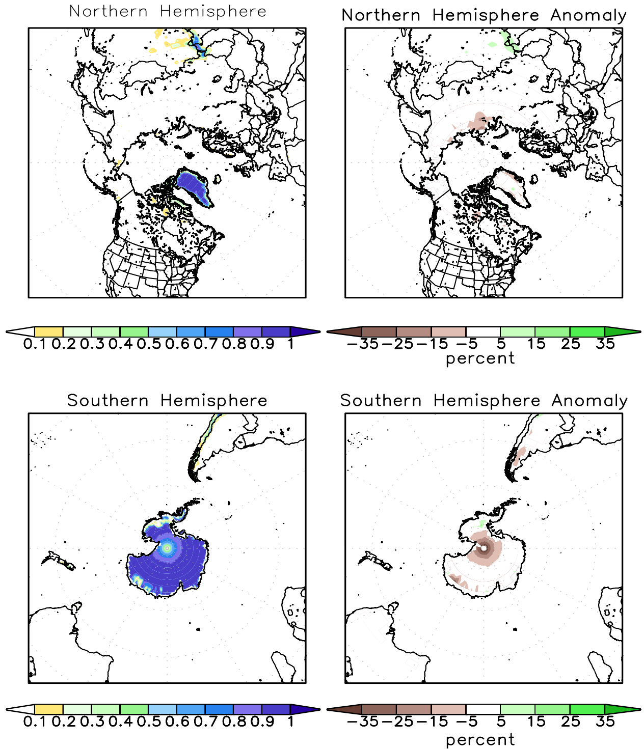
FIGURE A2.2. SSM/I derived snow cover frequency (%) (left) and snow cover anomaly (%) (right) for the month of JUN 2015 based on 1987 - 2010 base period for the Northern Hemisphere (top) and Southern Hemisphere (bottom). It is generated using the algorithm described by Ferraro et. al, 1996, Bull. Amer. Meteor. Soc., vol 77, 891-905.
