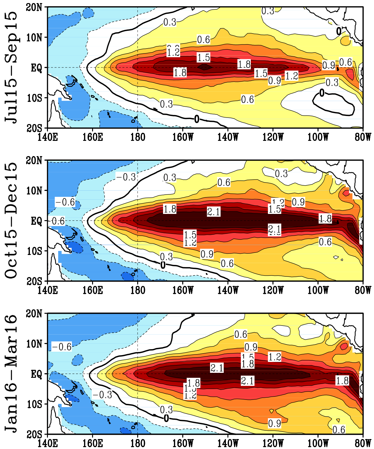
FIGURE F5. Predicted 3-month average sea surface temperature anomalies from the NCEP/CPC Markov model (Xue et al. 2000, J. Climate , 13 , 849-871). The forecast is initiated in JUN 2015 . Contour interval is 0.3C and negative anomalies are indicated by dashed contours. Anomalies are calculated relative to the 1971-2000 climatology.
