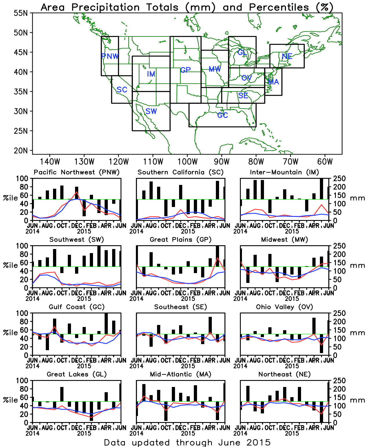
FIGURE E5. Areal estimates of monthly mean precipitation amounts (mm, solid lines) and precipitation percentiles (%ile, bars) for the most recent 13 months obtained from a merge of raingauge observations and satellite-derived precipitation estimates (Janowiak and Xie 1999, J. Climate , 12, 3335–3342). The monthly precipitation climatology (mm, dashed lines) is from the 1981–2010 base period monthly means. Monthly percentiles are not shown if the monthly mean is less than 5 mm.
