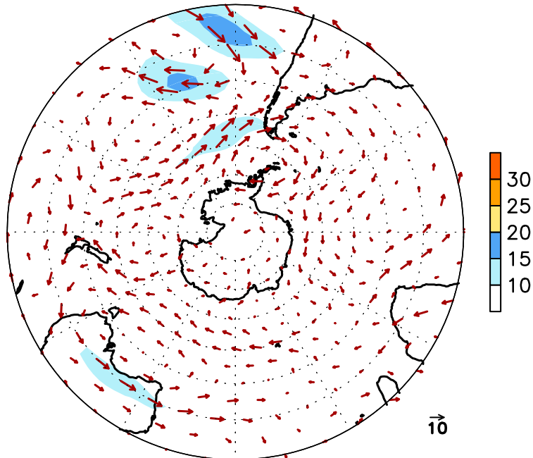
FIGURE E16. Southern Hemisphere mean (left) and anomalous (right) 300-hPa vector wind (CDAS/Reanalysis) for JUN 2015. Mean (anomaly) isotach contour interval is 10 (5) \text{ms}^{-1} . Values greater than 30 \text{ms}^{-1} (left) and 10 \text{ms}^{-1} (rights) are shaded. Anomalies are departures from the 1981-2010 base period monthly means.
