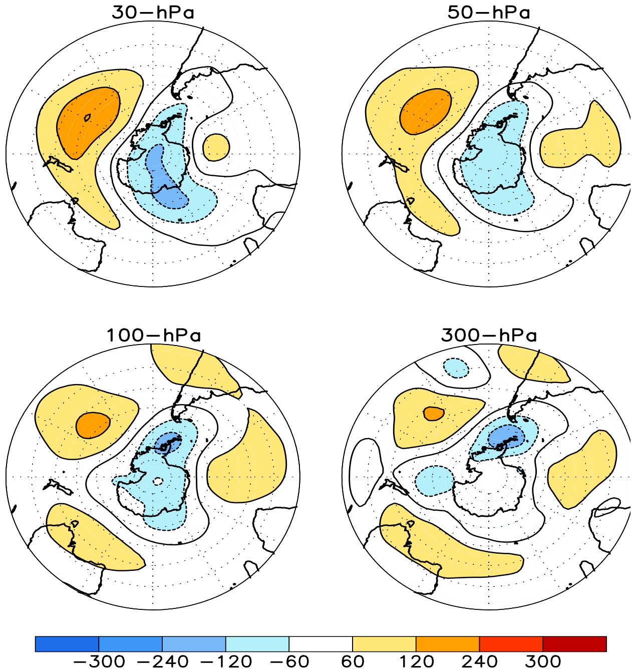
FIGURE S1. Stratospheric height anomalies (m) at selected levels for JUN 2015. Positive values are indicated by solid contours and dark shading. Negative values are indicated by dashed contours and light shading. Contour interval is 60 m. Anomalies are calculated from the 1981-2010 base period means. Winter Hemisphere is shown.
