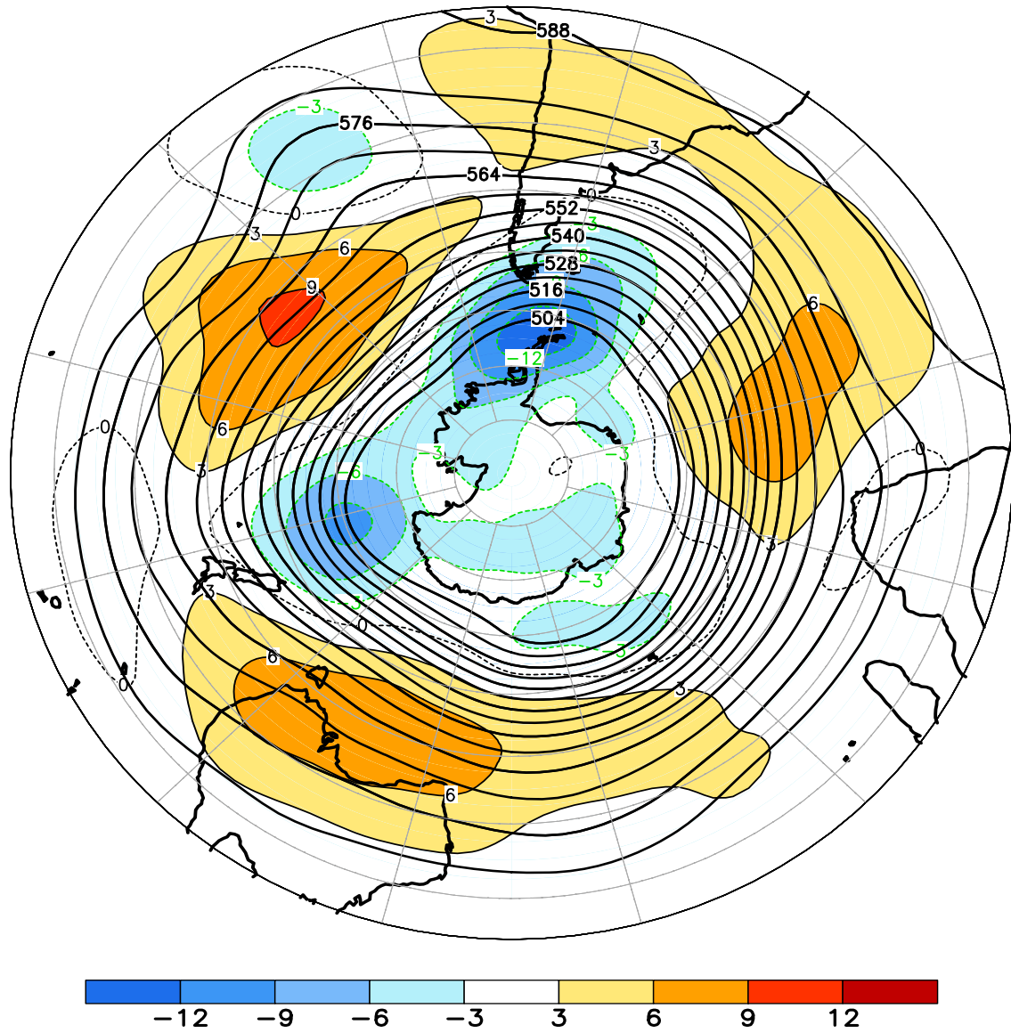
FIGURE E15. Southern Hemisphere mean and anomalous 500-hPa geopotential height (CDAS/Reanalysis) for JUN 2015. Mean heights are denoted by solid contours drawn at an interval of 6 dam. Anomaly contour interval is 3 dam with values less (greater) than -3 dam (3 dam) indicated by dark (light) shading. Anomalies are calculated as departures from the 1981-2010 base period monthly means.
