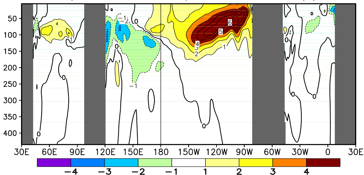
FIGURE T17. Equatorial depth–longitude section of ocean temperature (top) and ocean temperature anomalies (bottom) for JUN 2015. Contour interval is 1°C. Dashed contours in bottom panel indicate negative anomalies. Data are derived from the NCEP’s global ocean data assimilation system version 2 which assimilates oceanic observations into an oceanic GCM (Xue, Y. and Behringer, D.W., 2006: Operational global ocean data assimilation system at NCEP, to be submitted to BAMS). Anomalies are departures from the 1981–2010 base period means.
