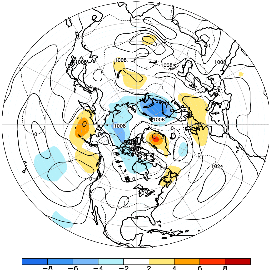
FIGURE E8. Northern Hemisphere mean and anomalous sea level pressure (CDAS/Reanalysis) for JUN 2015. Mean values are denoted by solid contours drawn at an interval of 4 hPa. Anomaly contour interval is 2 hPa with values less (greater) than -2 hPa (2 hPa) indicated by dark (light) shading. Anomalies are calculated as departures from the 1981-2010 base period monthly means.
