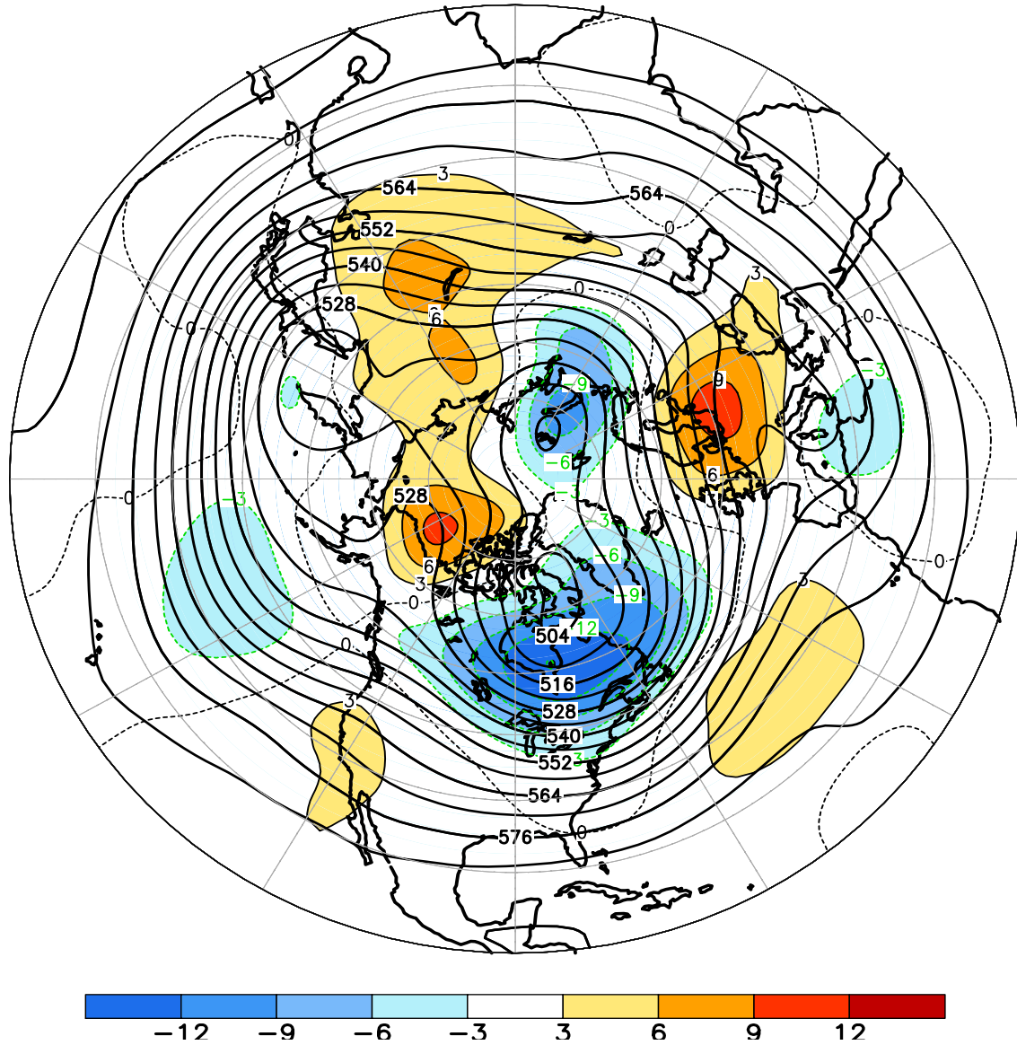
FIGURE E9. Northern Hemisphere mean and anomalous 500-hPa geopotential height (CDAS/Reanalysis) for MAR 2014. Mean heights are denoted by solid contours drawn at an interval of 6 dam. Anomaly contour interval is 3 dam with values less (greater) than -3 dam (3 dam) indicated by dark (light) shading. Anomalies are calculated as departures from the 1981-2010 base period monthly means.
