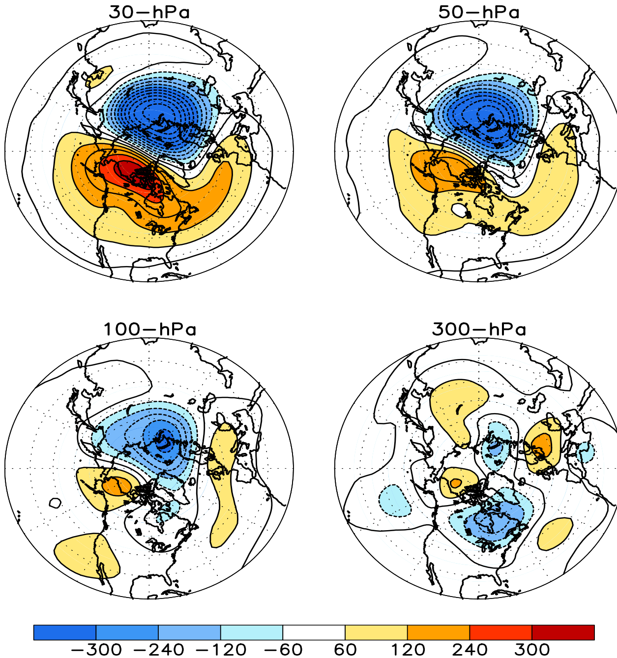
FIGURE S1. Stratospheric height anomalies (m) at selected levels for MAR 2014. Positive values are indicated by solid contours and dark shading. Negative values are indicated by dashed contours and light shading. Contour interval is 60 m. Anomalies are calculated from the 1981-2010 base period means. Winter Hemisphere is shown.
