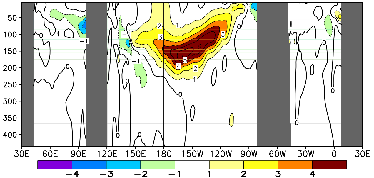
FIGURE T17. Equatorial depth-longitude section of ocean temperature (top) and ocean temperature anomalies (bottom) for MAR 2014. Contour interval is 1°C. Dashed contours in bottom panel indicate negative anomalies. Data are derived from the NCEP's global ocean data assimilation system version 2 which assimilates oceanic observations into an oceanic GCM (Xue, Y. and Behringer, D.W., 2006: Operational global ocean data assimilation system at NCEP, to be submitted to BAMS). Anomalies are departures from the 1981–2010 base period means.
