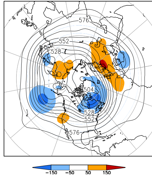
500-hPa Height (dm) & Anomalies (m) (Mar 1–15, 2014)
