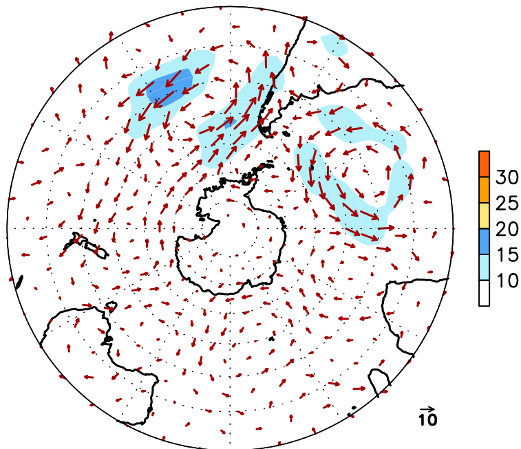
FIGURE E16. Southern Hemisphere mean (left) and anomalous (right) 300-hPa vector wind (CDAS/Reanalysis) for MAR 2014. Mean (anomaly) isotach contour interval is 10 (5) \text{ms}^{-1} . Values greater than 30 \text{ms}^{-1} (left) and 10 \text{ms}^{-1} (rights) are shaded. Anomalies are departures from the 1981-2010 base period monthly means.
