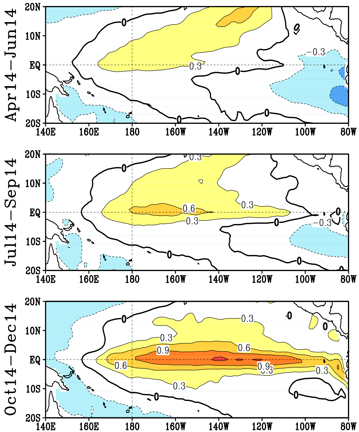
FIGURE F5. Predicted 3-month average sea surface temperature anomalies from the NCEP/CPC Markov model (Xue et al. 2000, J. Climate , 13 , 849-871). The forecast is initiated in MAR 2014 . Contour interval is 0.3C and negative anomalies are indicated by dashed contours. Anomalies are calculated relative to the 1971-2000 climatology.
