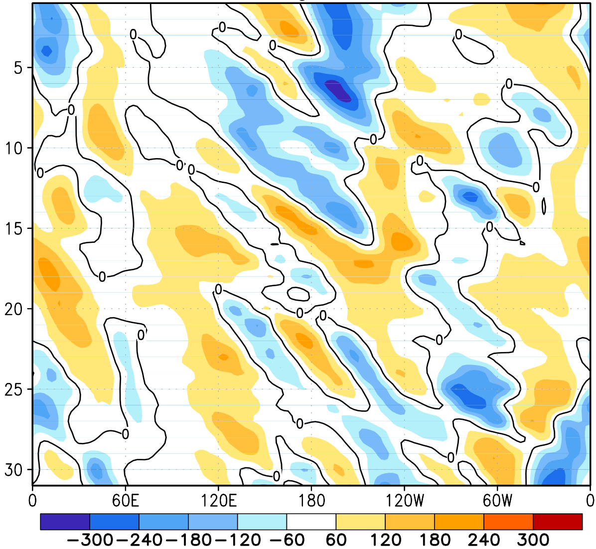
FIGURE E12. Northern Hemisphere: Daily 500-hPa height anomalies for MAR 2014 averaged over the 5° latitude band centered on 40°N. Positive values are indicated by solid contours and dark shading. Negative values are indicated by dashed contours and light shading. Contour interval is 60 m. Anomalies are departures from the 1981-2010 base period daily means.
