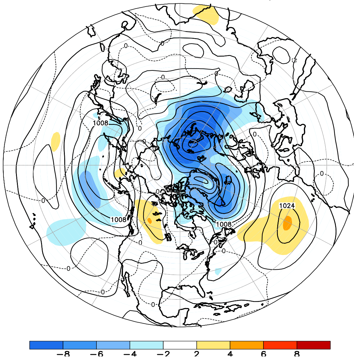
FIGURE E8. Northern Hemisphere mean and anomalous sea level pressure (CDAS/Reanalysis) for MAR 2014. Mean values are denoted by solid contours drawn at an interval of 4 hPa. Anomaly contour interval is 2 hPa with values less (greater) than -2 hPa (2 hPa) indicated by dark (light) shading. Anomalies are calculated as departures from the 1981-2010 base period monthly means.
