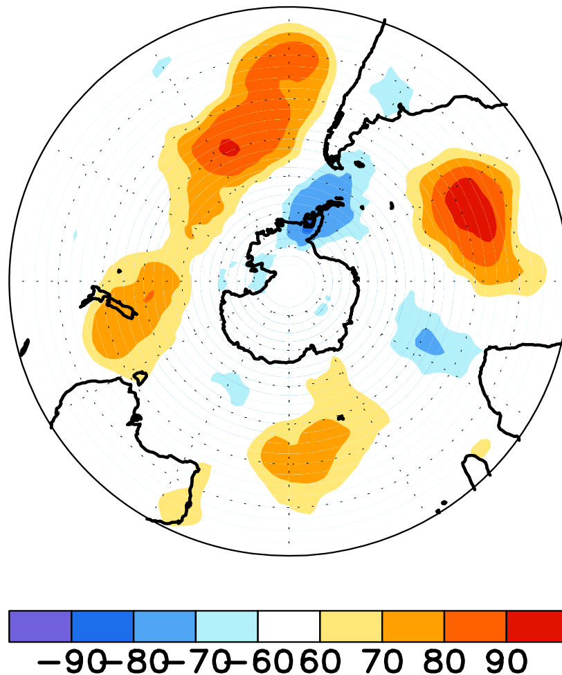
FIGURE E17. Southern Hemisphere percentage of days during MAR 2014 in which 500-hPa height anomalies greater than 15 m (red) and less than -15 m (blue) were observed. Values greater than 70% are shaded and contour interval
