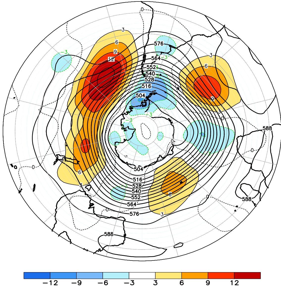
FIGURE E15. Southern Hemisphere mean and anomalous 500-hPa geopotential height (CDAS/Reanalysis) for MAR 2014. Mean heights are denoted by solid contours drawn at an interval of 6 dam. Anomaly contour interval is 3 dam with values less (greater) than -3 dam (3 dam) indicated by dark (light) shading. Anomalies are calculated as departures from the 1981-2010 base period monthly means.
