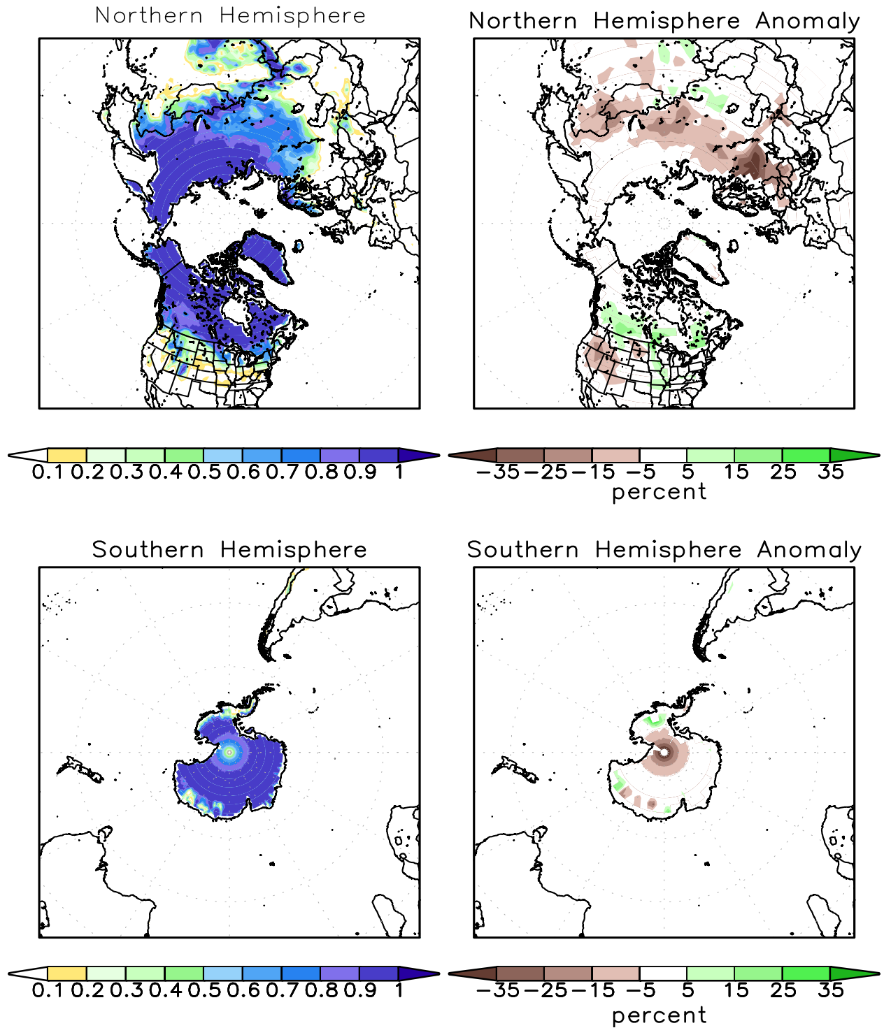
FIGURE A2.2. SSM/I derived snow cover frequency (%) (left) and snow cover anomaly (%) (right) for the month of MAR 2014 based on 1987 - 2010 base period for the Northern Hemisphere (top) and Southern Hemisphere (bottom). It is generated using the algorithm described by Ferraro et. al, 1996, Bull. Amer. Meteor. Soc., vol 77, 891-905.
