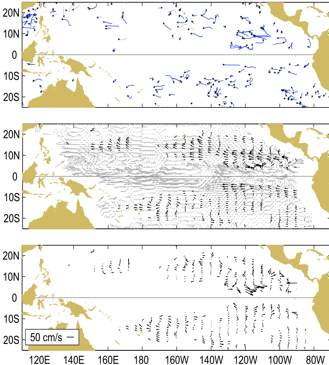
Figure A1.1 Top: Movements of drifting buoys in the tropical Pacific Ocean during March 2014. The linear segments of each trajectory represent a one week displacement. Trajectories of buoys which have lost their subsurface drogues are gray; those with drogues are black.
