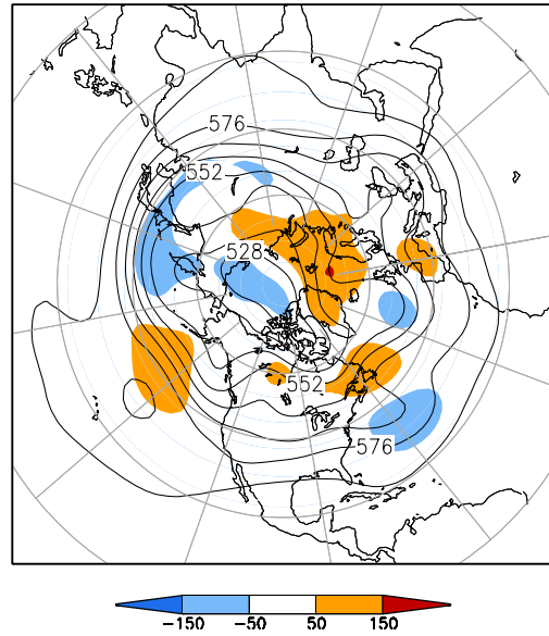
500-hPa Height (dm) & Anomalies (m) (May 1–15, 2011)
