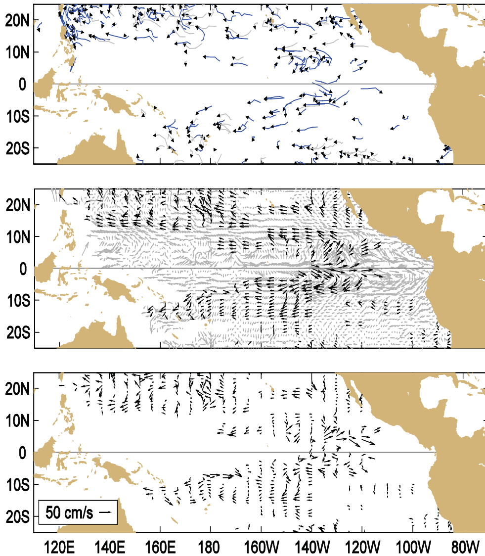
Figure A1.1 Top: Movements of drifting buoys in the tropical Pacific Ocean during May 2011. The linear segments of each trajectory represent a one week displacement. Trajectories of buoys which have lost their subsurface drogues are gray; those with drogues are black.
