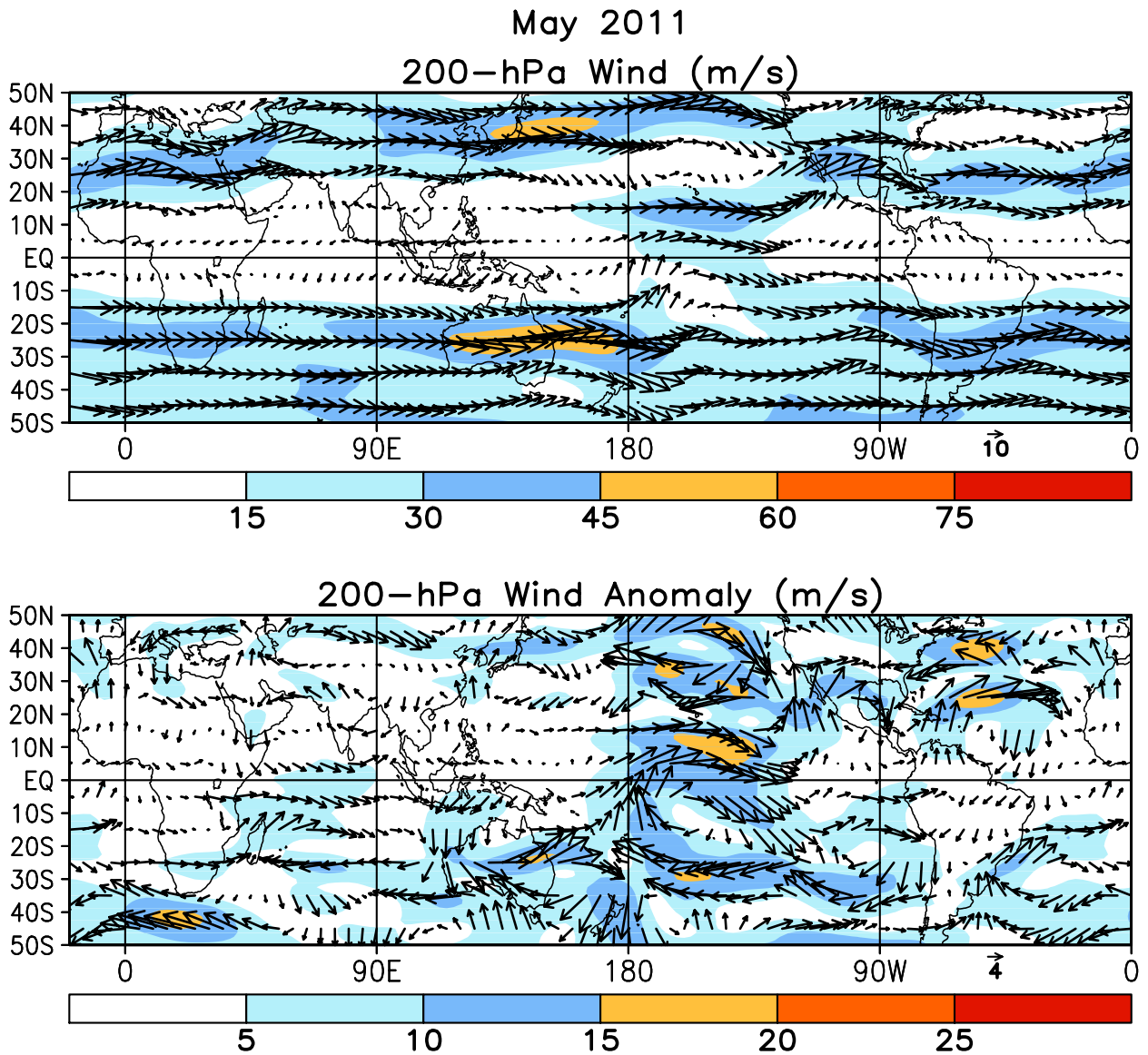
FIGURE T21. Mean (top) and anomalous (bottom) 200-hPa vector wind (CDAS/Reanalysis) for MAY 2011. Contour interval for isotachs is 15 \text{ ms}^{-1} (top) and 5 \text{ ms}^{-1} (bottom). Anomalies are departures from 1981-2010 base period monthly means.
