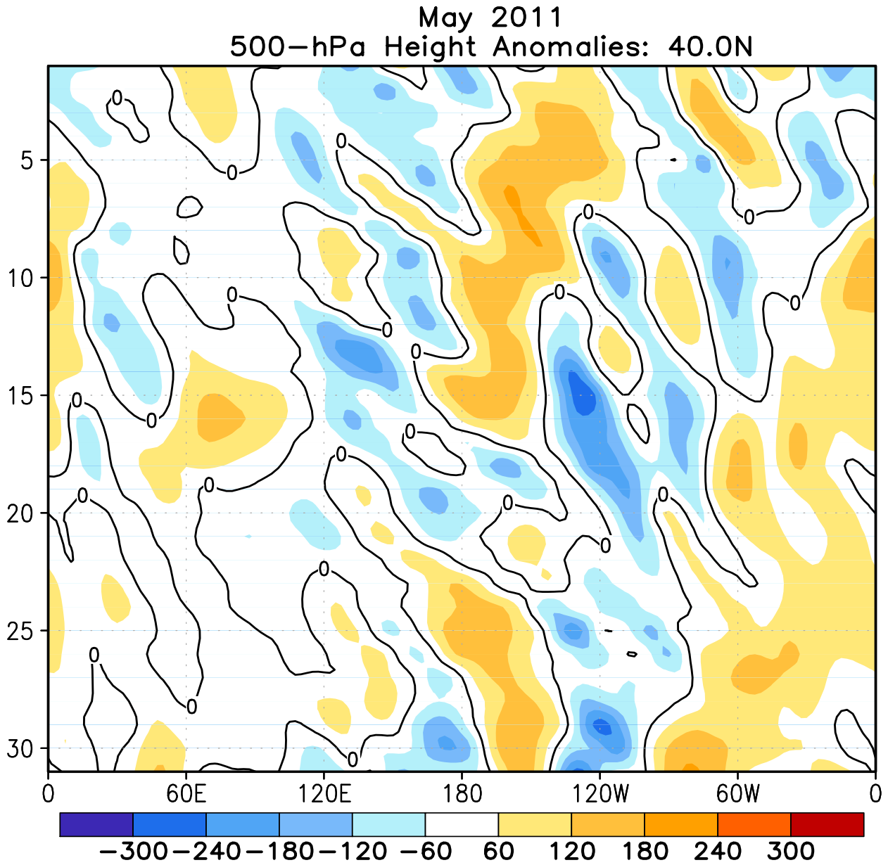
FIGURE E12. Northern Hemisphere: Daily 500-hPa height anomalies for MAY 2011 averaged over the 5° latitude band centered on 40°N. Positive values are indicated by solid contours and dark shading. Negative values are indicated by dashed contours and light shading. Contour interval is 60 m. Anomalies are departures from the 1981-2010 base period daily means.
