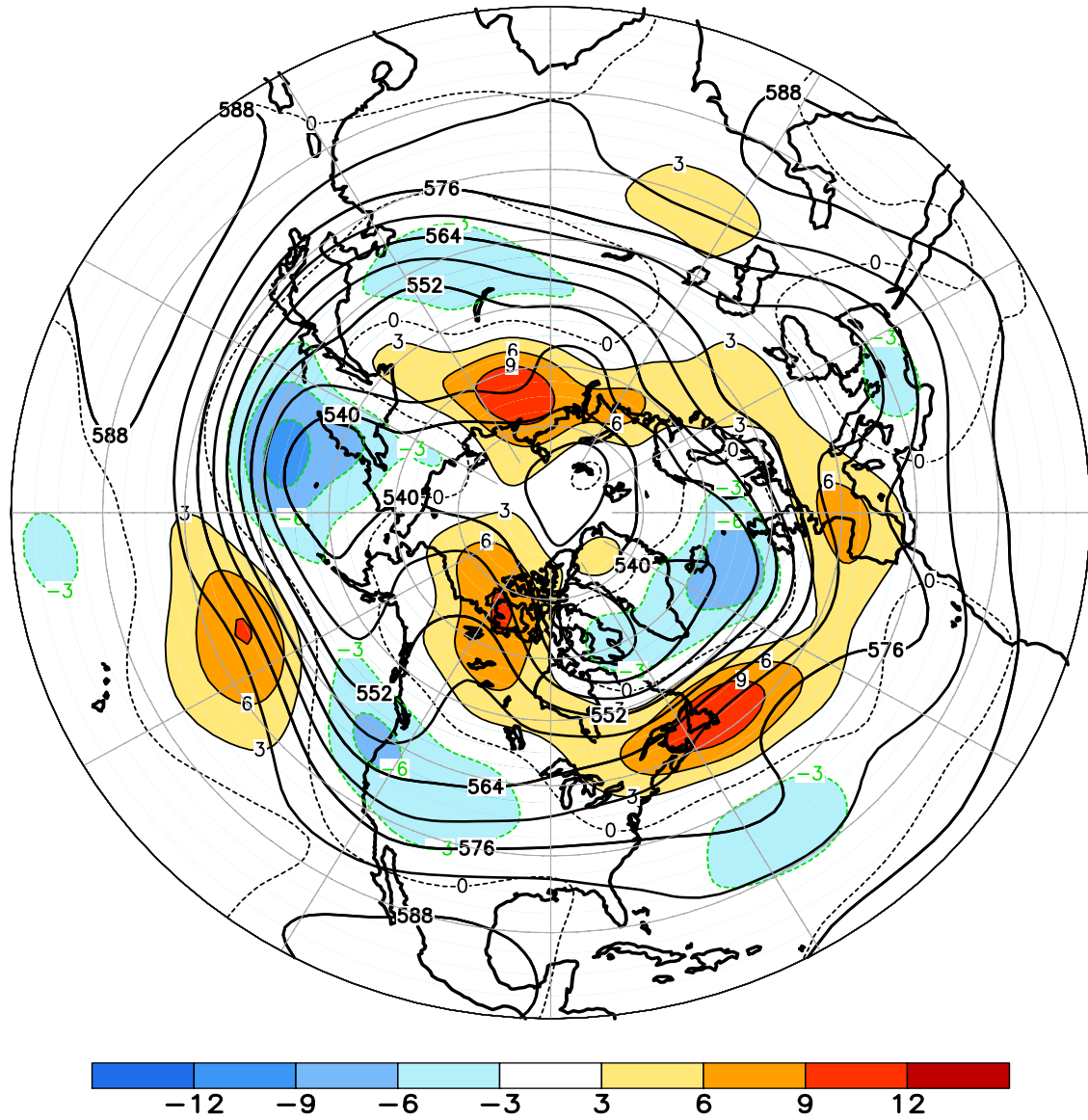
FIGURE E9. Northern Hemisphere mean and anomalous 500-hPa geopotential height (CDAS/Reanalysis) for MAY 2011. Mean heights are denoted by solid contours drawn at an interval of 6 dam. Anomaly contour interval is 3 dam with values less (greater) than -3 dam (3 dam) indicated by dark (light) shading. Anomalies are calculated as departures from the 1981-2010 base period monthly means.
