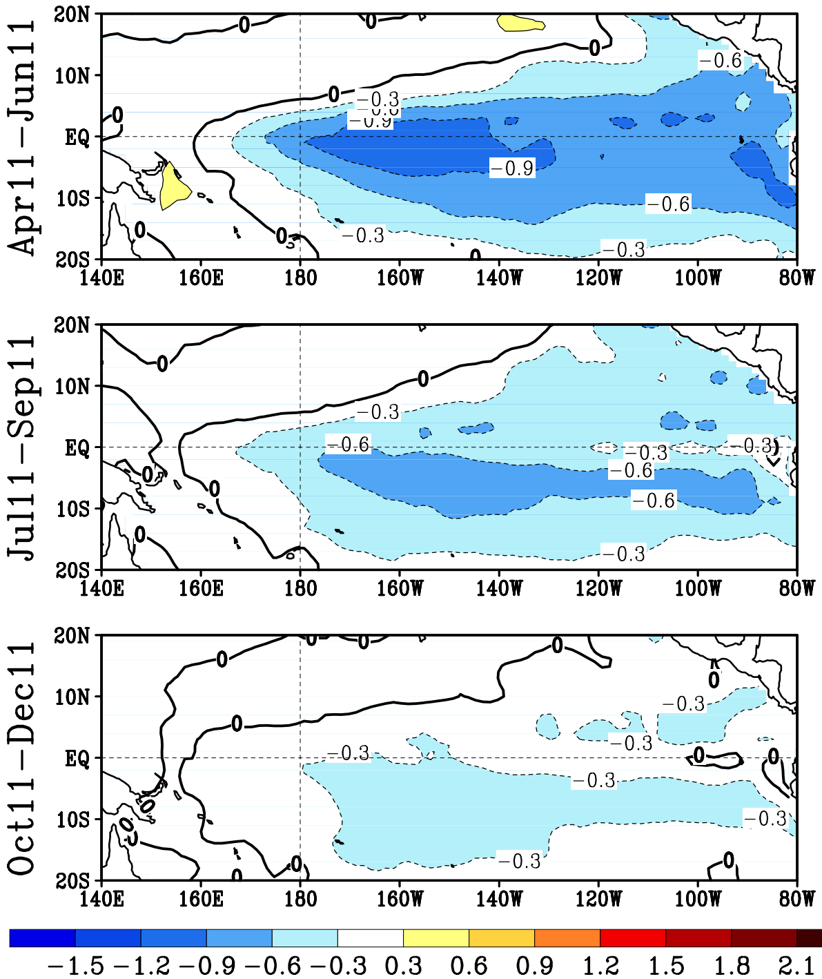
FIGURE F5. Predicted 3-month average sea surface temperature anomalies from the NCEP/CPC Markov model (Xue et al. 2000, J. Climate , 13 , 849-871). The forecast is initiated in MAY 2011 . Contour interval is 0.3C and negative anomalies are indicated by dashed contours. Anomalies are calculated relative to the 1971-2000 climatology.
