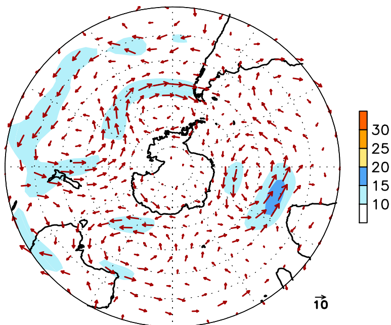
FIGURE E16. Southern Hemisphere mean (left) and anomalous (right) 300-hPa vector wind (CDAS/Reanalysis) for MAY 2011. Mean (anomaly) isotach contour interval is 10 (5) \text{ms}^{-1} . Values greater than 30 \text{ms}^{-1} (left) and 10 \text{ms}^{-1} (rights) are shaded. Anomalies are departures from the 1981-2010 base period monthly means.
