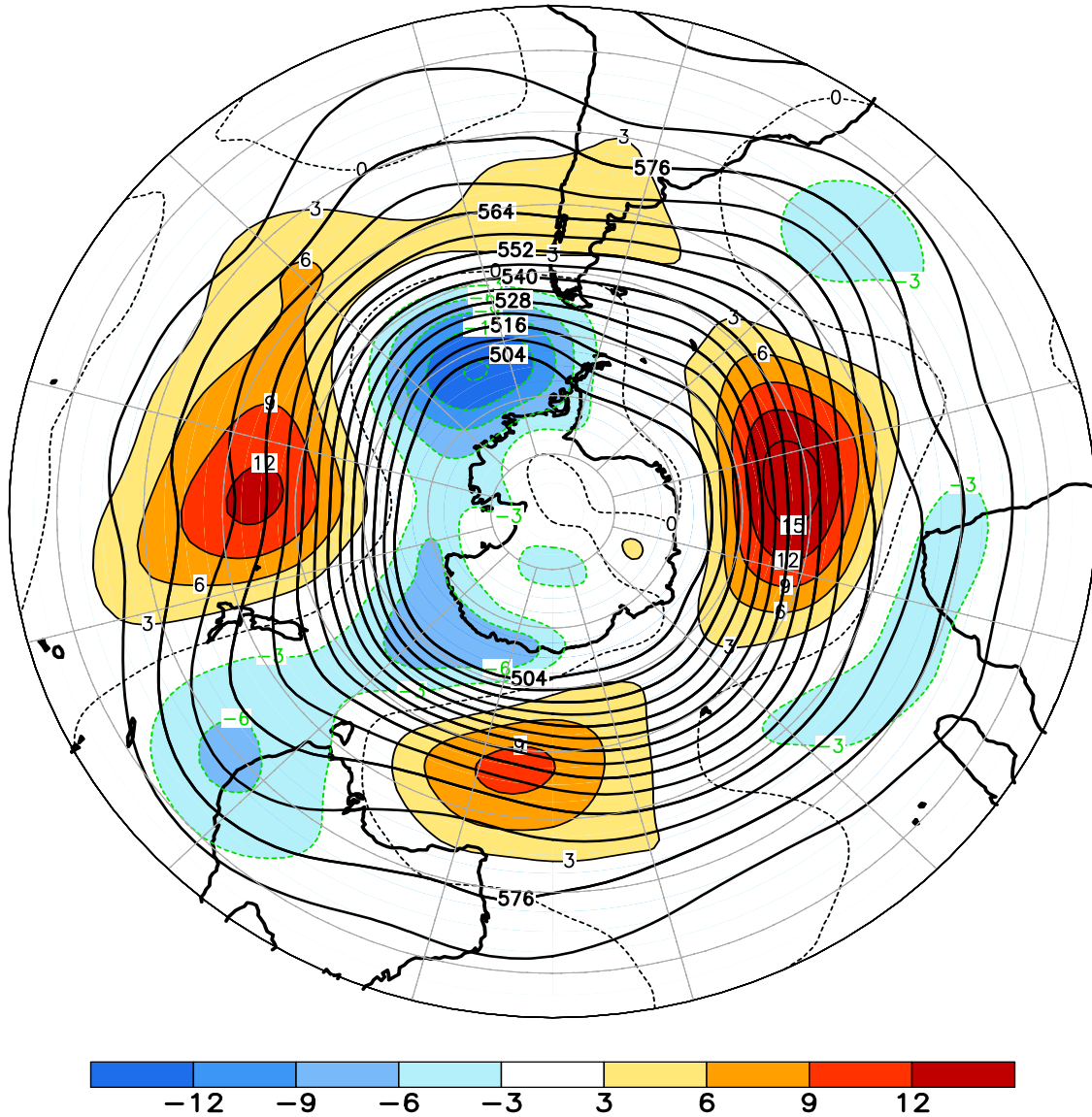
FIGURE E15. Southern Hemisphere mean and anomalous 500-hPa geopotential height (CDAS/Reanalysis) for MAY 2011. Mean heights are denoted by solid contours drawn at an interval of 6 dam. Anomaly contour interval is 3 dam with values less (greater) than -3 dam (3 dam) indicated by dark (light) shading. Anomalies are calculated as departures from the 1981-2010 base period monthly means.
