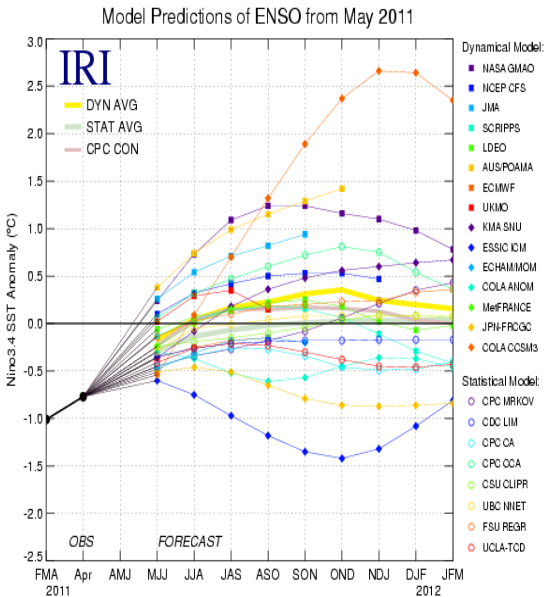
FIGURE F13. Time series of predicted sea surface temperature anomalies for the Nino 3.4 region (deg. C) from various dynamical and statistical models for nine overlapping 3-month periods. The Nino 3.4 region spans the east-central equatorial Pacific between 5N-5S, 170W-120W. Figure provided by the International Research Institute (IRI).
