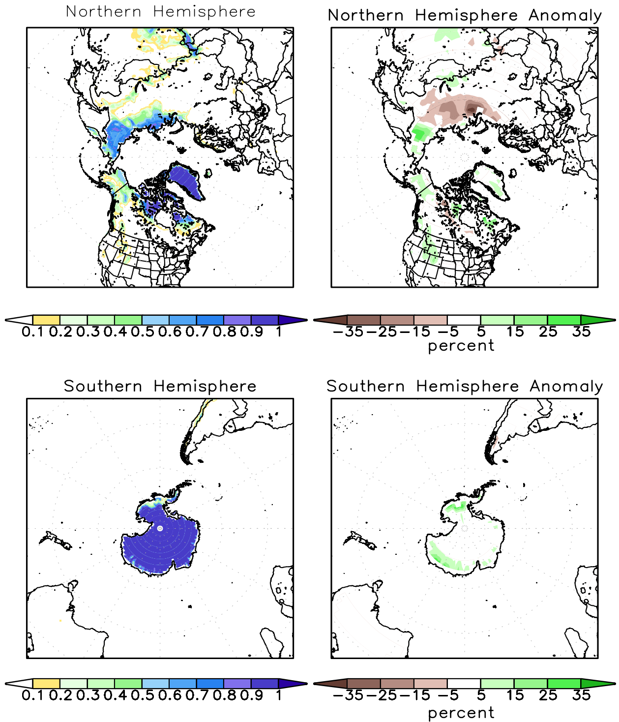
FIGURE A2.2. SSM/I derived snow cover frequency (%) (left) and snow cover anomaly (%) (right) for the month of MAY 2011 based on 1987 - 2010 base period for the Northern Hemisphere (top) and Southern Hemisphere (bottom). It is generated using the algorithm described by Ferraro et. al, 1996, Bull. Amer. Meteor. Soc., vol 77, 891-905.
