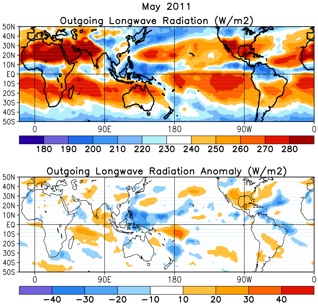
FIGURE T25. Mean (top) and anomalous (bottom) outgoing longwave radiation for MAY 2011 (NOAA 18 AVHRR IR window channel measurements by NESDIS/ORA). OLR contour interval is 20 Wm -2 with values greater than 280 Wm -2 indicated by dashed contours. Anomaly contour interval is 15 Wm -2 with positive values indicated by dashed contours and light shading. Anomalies are departures from the 1981-2010 base period monthly means.
