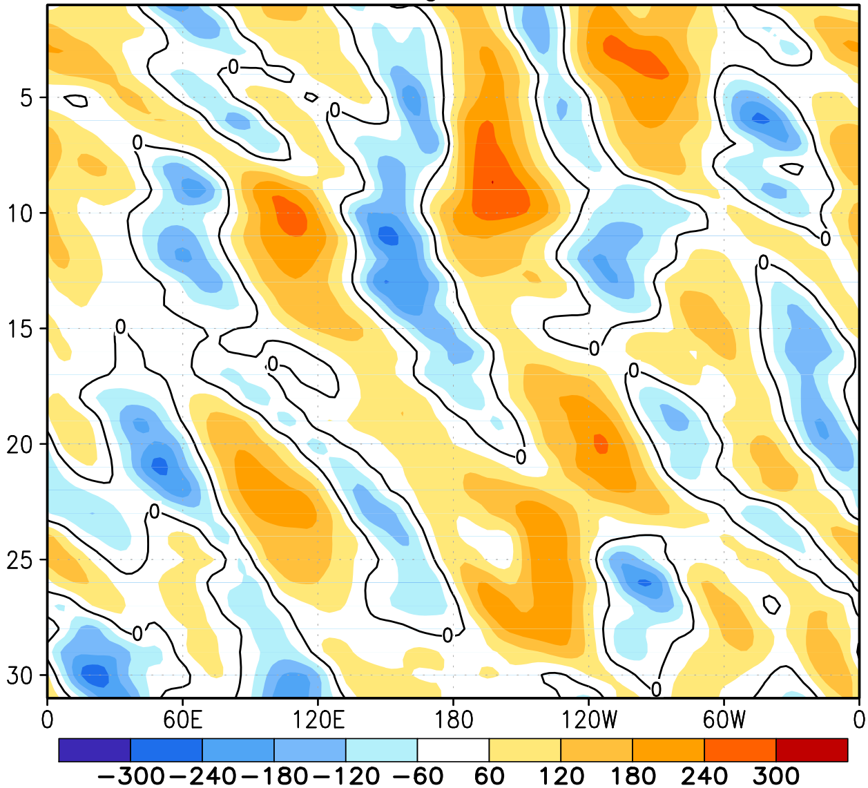
FIGURE E18. Southern Hemisphere: Daily 500-hPa height anomalies for MAY 2011 averaged over the 5° latitude band centered on 40°S. Positive values are indicated by solid contours and dark shading. Negative values are indicated by dashed contours and light shading. Contour interval is 60 m. Anomalies are departures from the 1981-2010 base period daily means.
