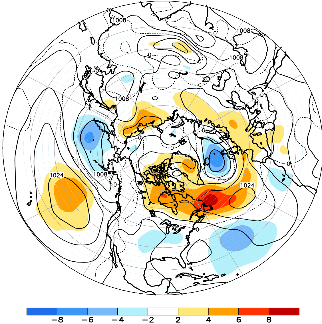
FIGURE E8. Northern Hemisphere mean and anomalous sea level pressure (CDAS/Reanalysis) for MAY 2011. Mean values are denoted by solid contours drawn at an interval of 4 hPa. Anomaly contour interval is 2 hPa with values less (greater) than -2 hPa (2 hPa) indicated by dark (light) shading. Anomalies are calculated as departures from the 1981-2010 base period monthly means.
