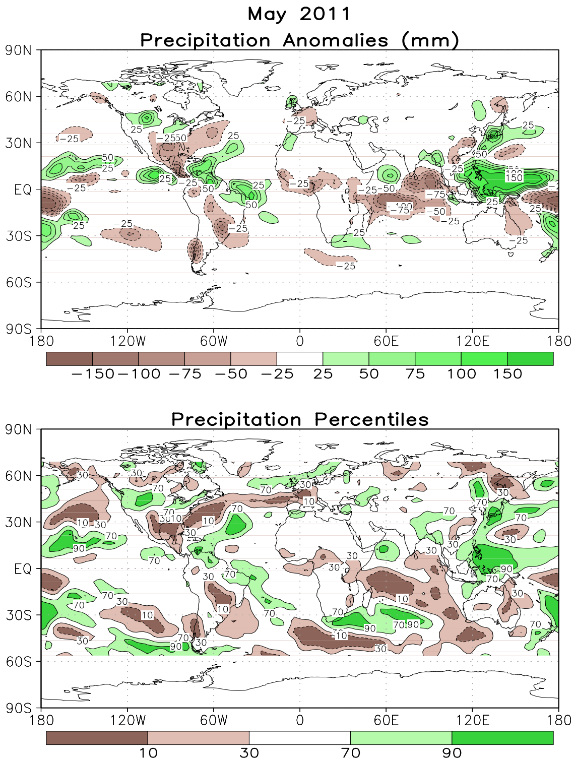
FIGURE E3. Anomalous precipitation (mm, top) and precipitation percentiles based on a Gamma distribution fit to the 1981–2010 base period data (bottom) for MAY 2011. Data are obtained from a merge of raingauge observations and satellite-derived precipitation estimates (Janowiak and Xie 1999, J. Climate , 12 , 3335–3342). Contours are drawn at 200, 100, 50, 25, -25, -50, -100, and -200 mm in top panel. Percentiles are not plotted in regions where mean monthly precipitation is <5mm/month.
