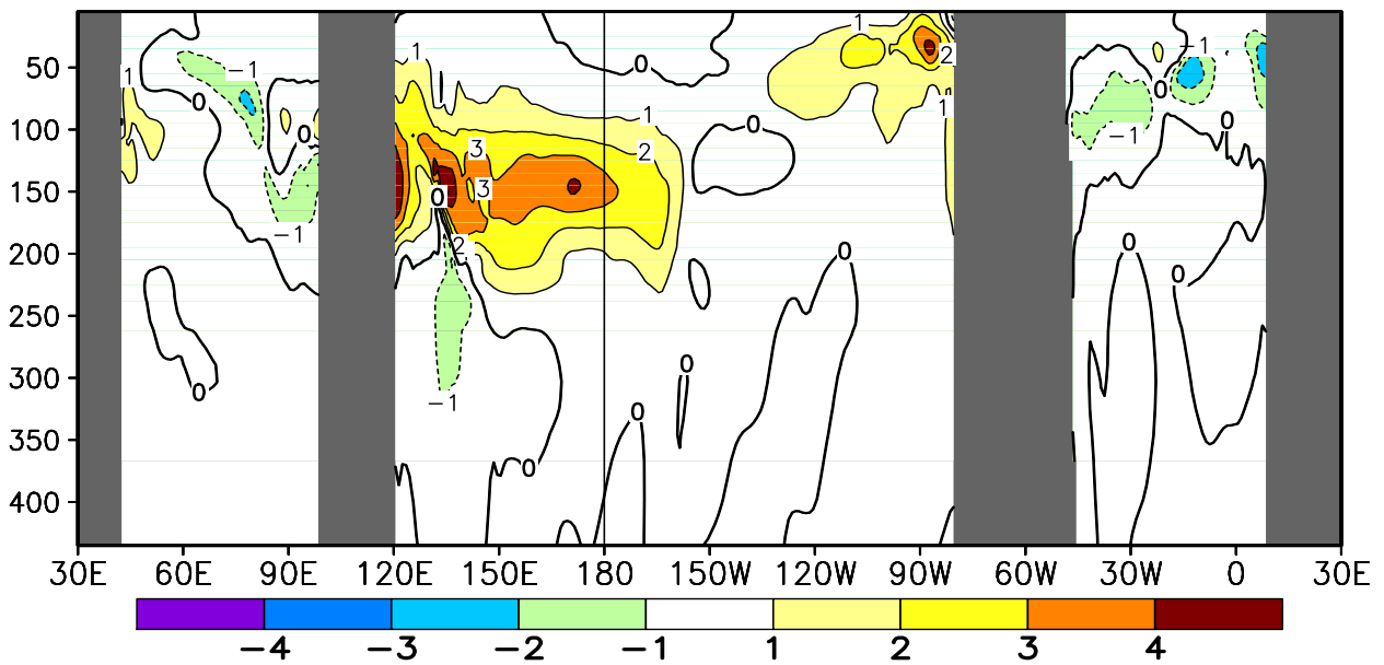
FIGURE T17. Equatorial depth–longitude section of ocean temperature (top) and ocean temperature anomalies (bottom) for MAY 2011. Contour interval is 1°C. Dashed contours in bottom panel indicate negative anomalies. Data are derived from the NCEP’s global ocean data assimilation system version 2 which assimilates oceanic observations into an oceanic GCM (Xue, Y. and Behringer, D.W., 2006: Operational global ocean data assimilation system at NCEP, to be submitted to BAMS). Anomalies are departures from the 1981–2010 base period means.
