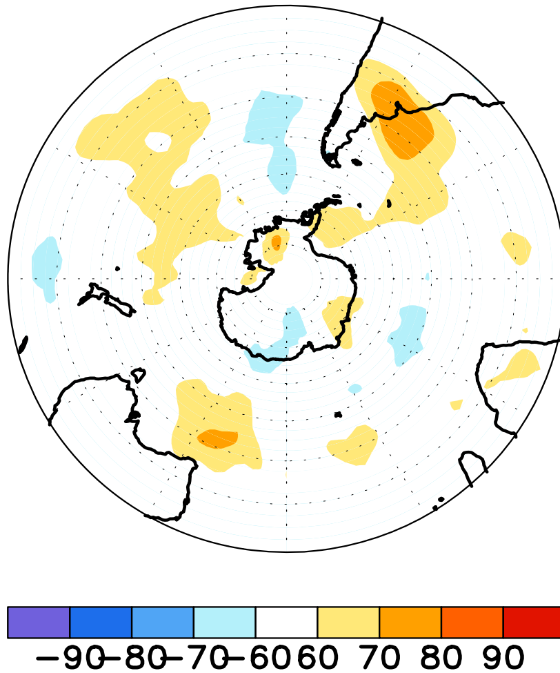
FIGURE E17. Southern Hemisphere percentage of days during MAY 2012 in which 500-hPa height anomalies greater than 15 m (red) and less than -15 m (blue) were observed. Values greater than 70% are shaded and contour in-
