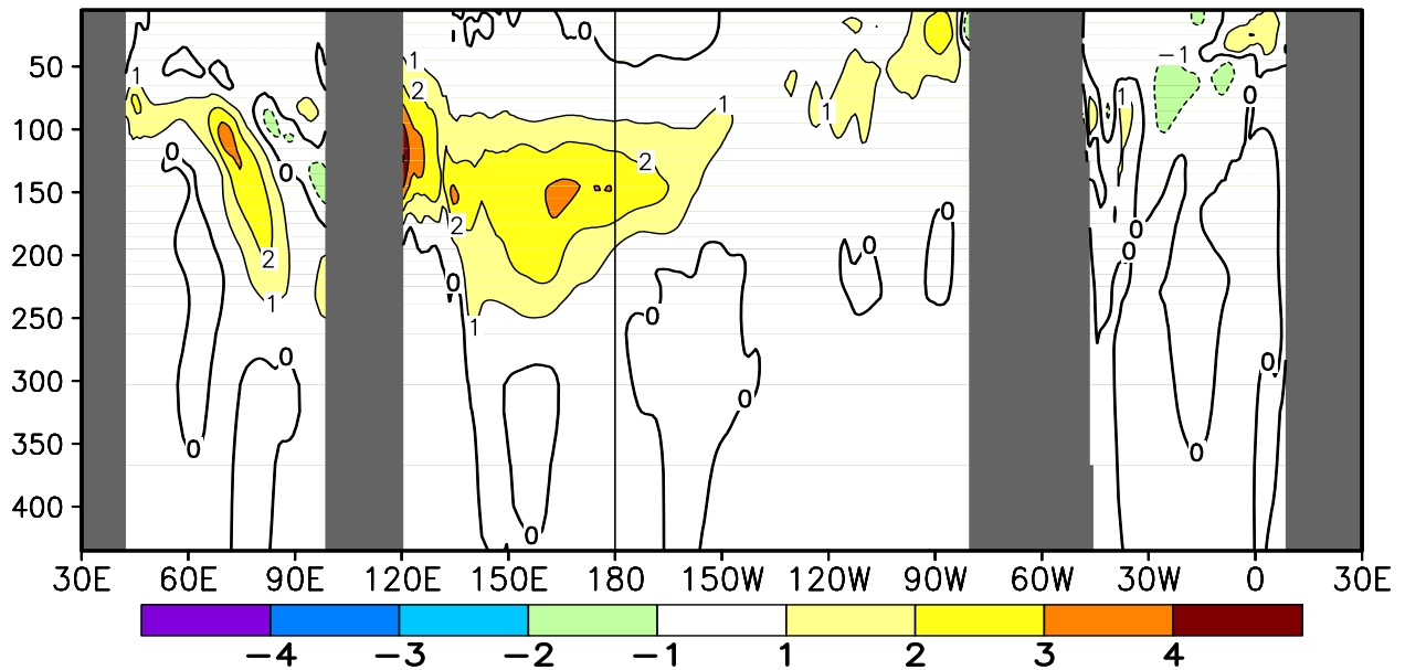
FIGURE T17. Equatorial depth–longitude section of ocean temperature (top) and ocean temperature anomalies (bottom) for MAY 2012. Contour interval is 1°C. Dashed contours in bottom panel indicate negative anomalies. Data are derived from the NCEP’s global ocean data assimilation system version 2 which assimilates oceanic observations into an oceanic GCM (Xue, Y. and Behringer, D.W., 2006: Operational global ocean data assimilation system at NCEP, to be submitted to BAMS). Anomalies are departures from the 1981–2010 base period means.
