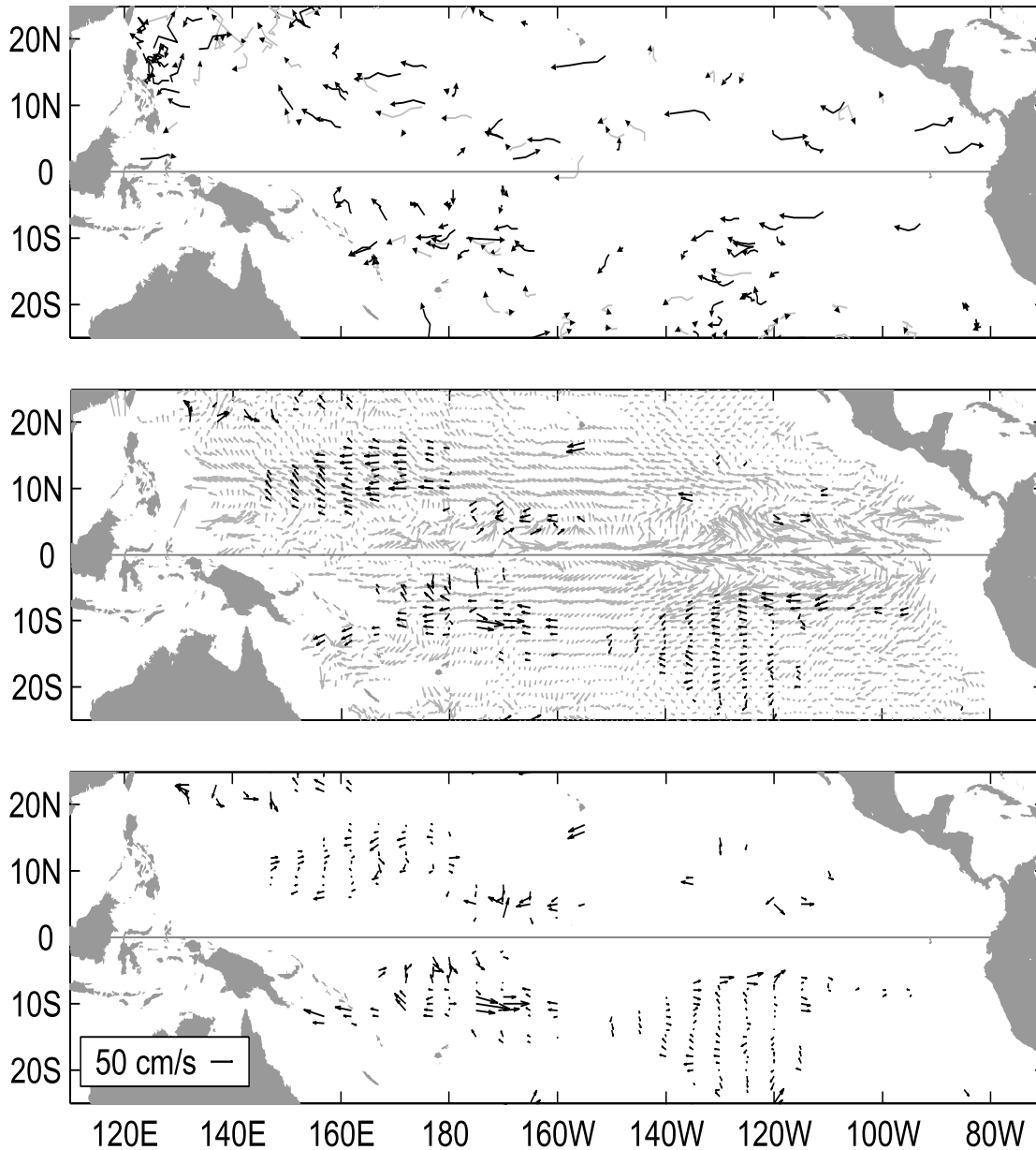
Figure A1.1 Top: Movements of drifting buoys in the tropical Pacific Ocean during May 2012. The linear segments of each trajectory represent a one week displacement. Trajectories of buoys which have lost their subsurface drogues are gray; those with drogues are black.
