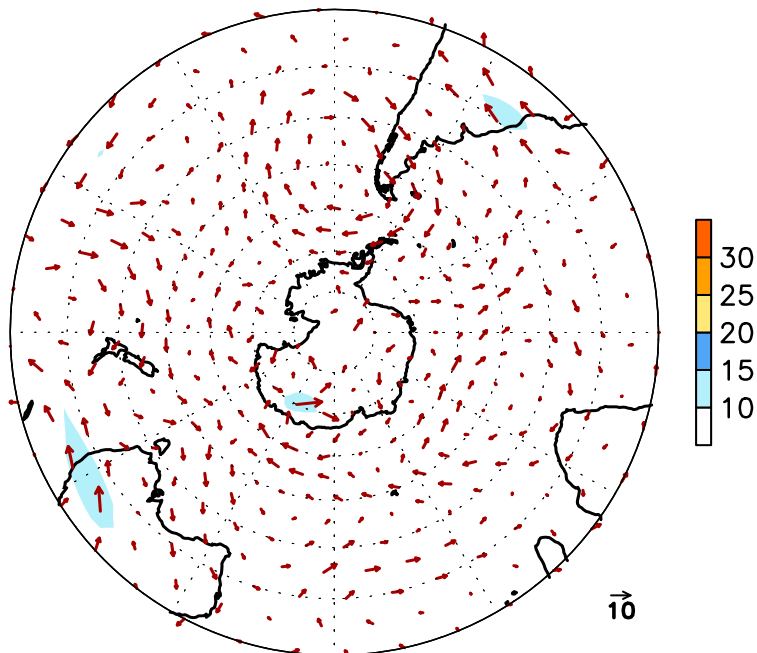
FIGURE E16. Southern Hemisphere mean (left) and anomalous (right) 300-hPa vector wind (CDAS/Reanalysis) for MAY 2012. Mean (anomaly) isotach contour interval is 10 (5) \text{ms}^{-1} . Values greater than 30 \text{ms}^{-1} (left) and 10 \text{ms}^{-1} (rights) are shaded. Anomalies are departures from the 1981-2010 base period monthly means.
