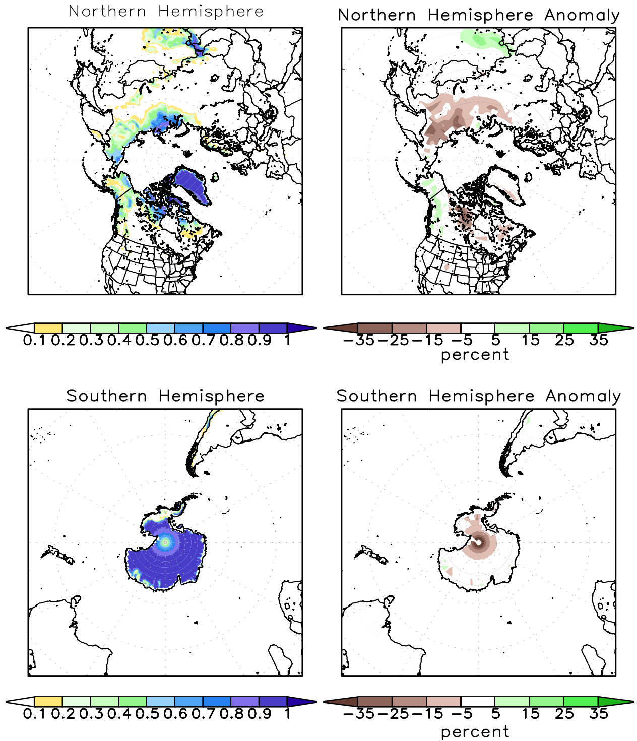
FIGURE A2.2. SSM/I derived snow cover frequency (%) (left) and snow cover anomaly (%) (right) for the month of MAY 2012 based on 1987 - 2010 base period for the Northern Hemisphere (top) and Southern Hemisphere (bottom). It is generated using the algorithm described by Ferraro et. al, 1996, Bull. Amer. Meteor. Soc., vol 77, 891-905.
