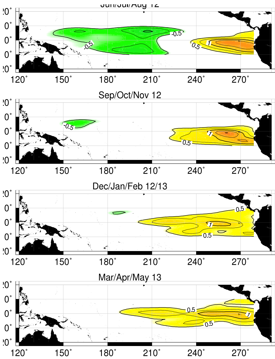
FIGURE F11. SST anomaly forecast for the equatorial Pacific from the Hybrid Coupled Model (HCM) developed by the Scripps Institution of Oceanography and the Max-Planck Institut fuer Meteorologie.
