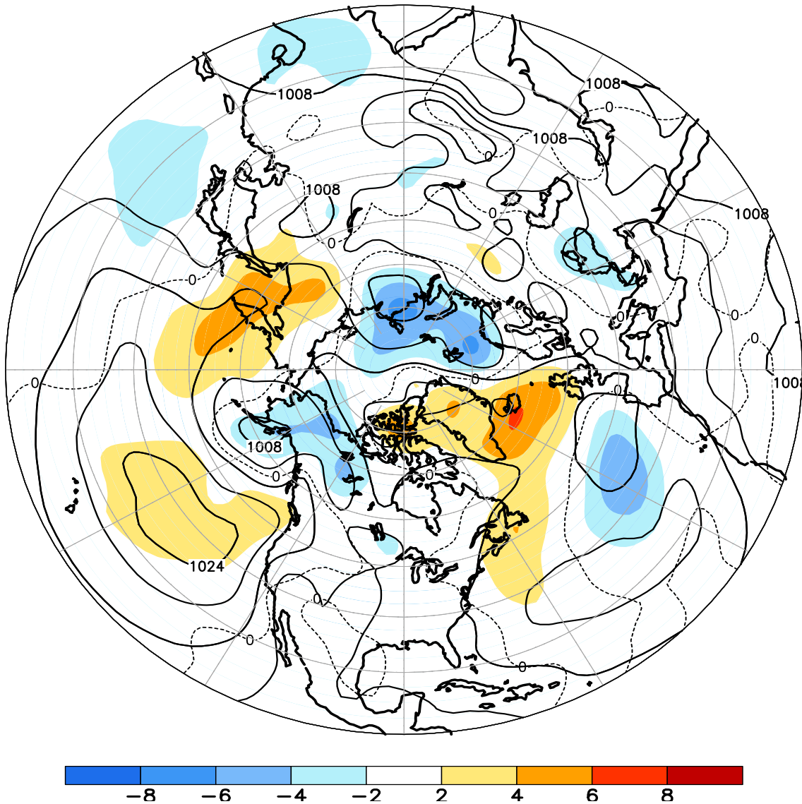
FIGURE E8. Northern Hemisphere mean and anomalous sea level pressure (CDAS/Reanalysis) for MAY 2012. Mean values are denoted by solid contours drawn at an interval of 4 hPa. Anomaly contour interval is 2 hPa with values less (greater) than -2 hPa (2 hPa) indicated by dark (light) shading. Anomalies are calculated as departures from the 1981-2010 base period monthly means.
