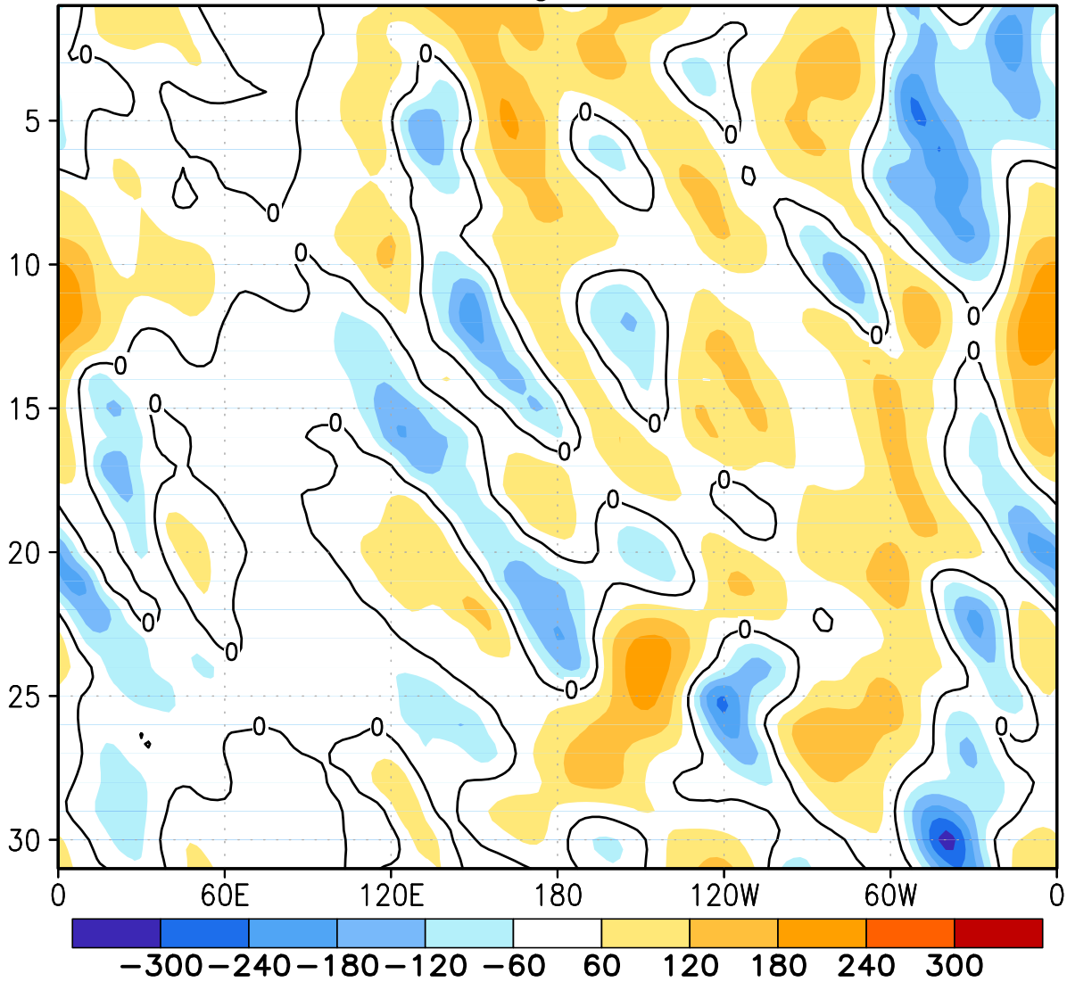
FIGURE E12. Northern Hemisphere: Daily 500-hPa height anomalies for MAY 2012 averaged over the 5° latitude band centered on 40°N. Positive values are indicated by solid contours and dark shading. Negative values are indicated by dashed contours and light shading. Contour interval is 60 m. Anomalies are departures from the 1981-2010 base period daily means.
