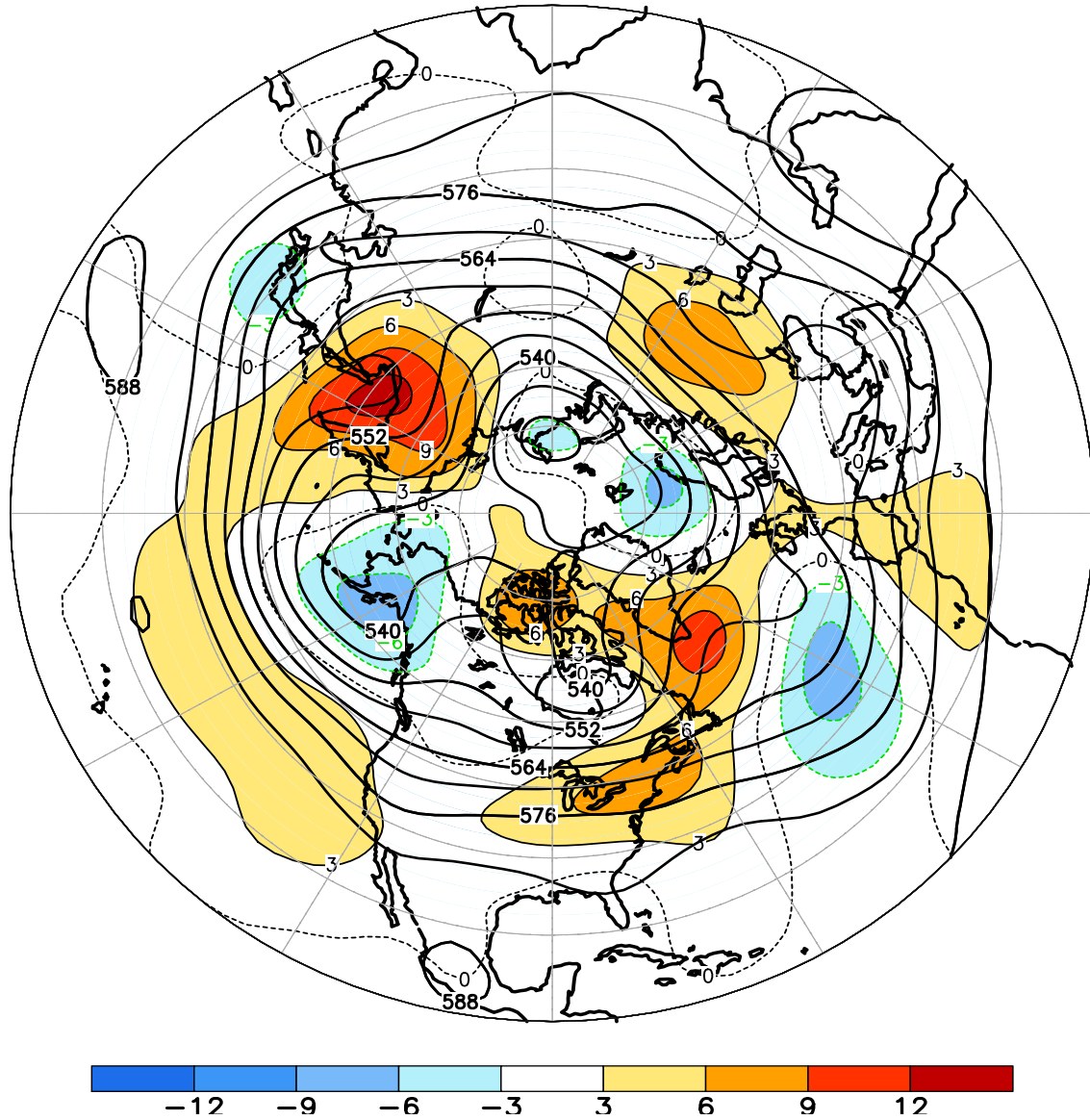
FIGURE E9. Northern Hemisphere mean and anomalous 500-hPa geopotential height (CDAS/Reanalysis) for MAY 2012. Mean heights are denoted by solid contours drawn at an interval of 6 dam. Anomaly contour interval is 3 dam with values less (greater) than -3 dam (3 dam) indicated by dark (light) shading. Anomalies are calculated as departures from the 1981-2010 base period monthly means.
