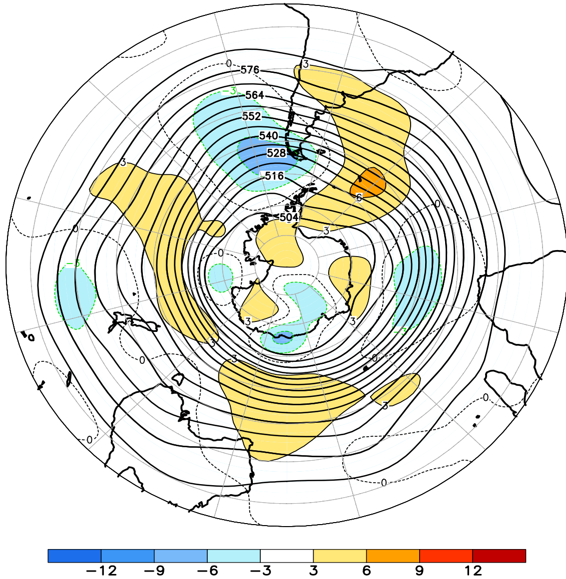
FIGURE E15. Southern Hemisphere mean and anomalous 500-hPa geopotential height (CDAS/Reanalysis) for MAY 2012. Mean heights are denoted by solid contours drawn at an interval of 6 dam. Anomaly contour interval is 3 dam with values less (greater) than -3 dam (3 dam) indicated by dark (light) shading. Anomalies are calculated as departures from the 1981-2010 base period monthly means.
