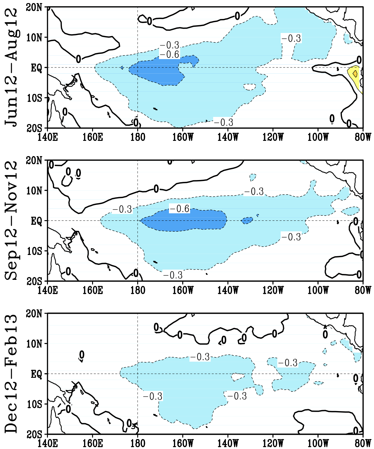
FIGURE F5. Predicted 3-month average sea surface temperature anomalies from the NCEP/CPC Markov model (Xue et al. 2000, J. Climate , 13 , 849-871). The forecast is initiated in MAY 2012. Contour interval is 0.3C and negative anomalies are indicated by dashed contours. Anomalies are calculated relative to the 1971-2000 climatology.
