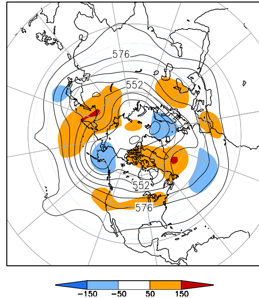
500-hPa Height (dm) & Anomalies (m) (May 1–15, 2012)
