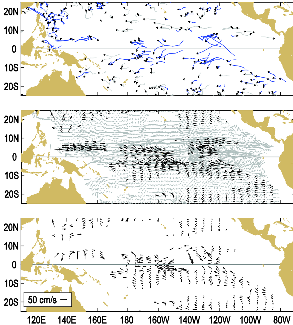
Figure A1.1 Top: Movements of drifting buoys in the tropical Pacific Ocean during October 2011. The linear segments of each trajectory represent a one week displacement. Trajectories of buoys which have lost their subsurface drogues are gray; those with drogues are black.
