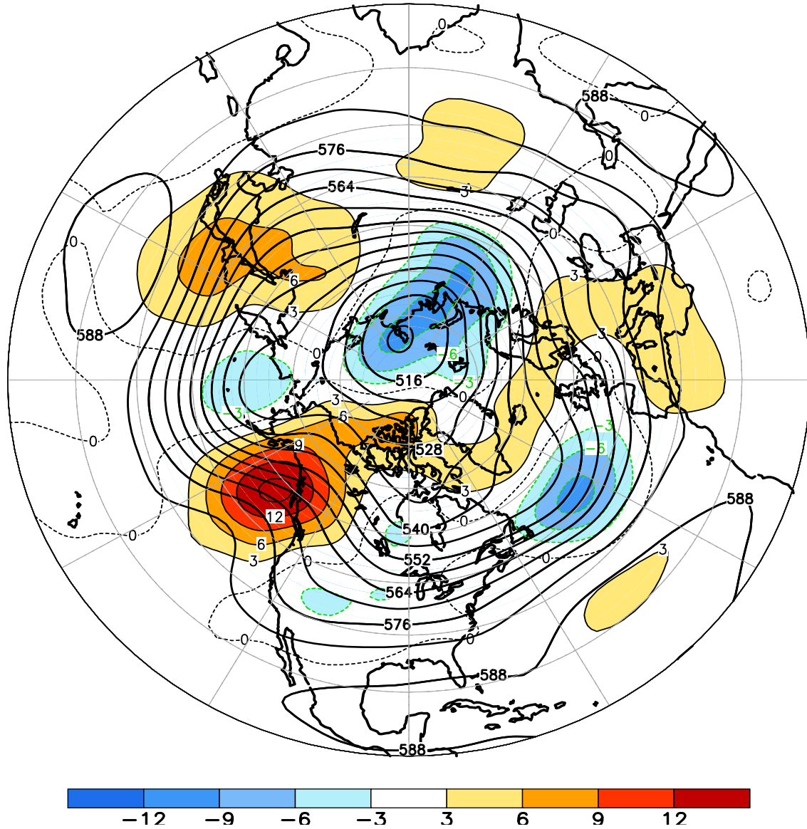
FIGURE E9. Northern Hemisphere mean and anomalous 500-hPa geopotential height (CDAS/Reanalysis) for OCT 2013. Mean heights are denoted by solid contours drawn at an interval of 6 dam. Anomaly contour interval is 3 dam with values less (greater) than -3 dam (3 dam) indicated by dark (light) shading. Anomalies are calculated as departures from the 1981-2010 base period monthly means.
