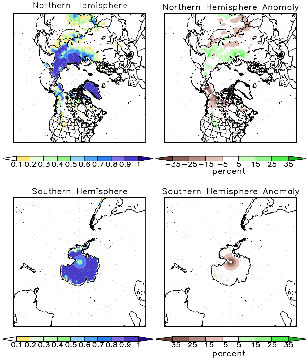
FIGURE A2.2. SSM/I derived snow cover frequency (%) (left) and snow cover anomaly (%) (right) for the month of OCT 2013 based on 1987 - 2010 base period for the Northern Hemisphere (top) and Southern Hemisphere (bottom). It is generated using the algorithm described by Ferraro et. al, 1996, Bull. Amer. Meteor. Soc., vol 77, 891-905.
