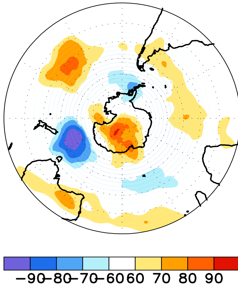
FIGURE E17. Southern Hemisphere percentage of days during OCT 2013 in which 500-hPa height anomalies greater than 15 m (red) and less than -15 m (blue) were observed. Values greater than 70% are shaded and contour in-
