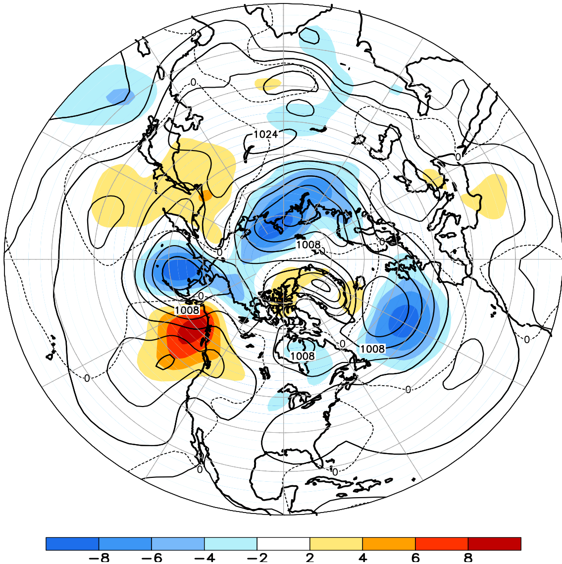
FIGURE E8. Northern Hemisphere mean and anomalous sea level pressure (CDAS/Reanalysis) for OCT 2013. Mean values are denoted by solid contours drawn at an interval of 4 hPa. Anomaly contour interval is 2 hPa with values less (greater) than -2 hPa (2 hPa) indicated by dark (light) shading. Anomalies are calculated as departures from the 1981-2010 base period monthly means.
