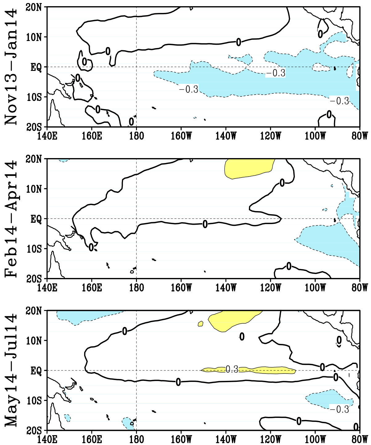
FIGURE F5. Predicted 3-month average sea surface temperature anomalies from the NCEP/CPC Markov model (Xue et al. 2000, J. Climate , 13 , 849-871). The forecast is initiated in OCT 2013 . Contour interval is 0.3C and negative anomalies are indicated by dashed contours. Anomalies are calculated relative to the 1971-2000 climatology.
