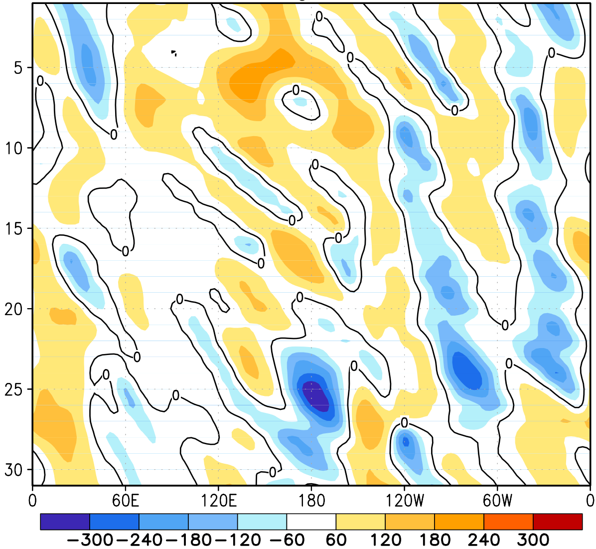
FIGURE E12. Northern Hemisphere: Daily 500-hPa height anomalies for OCT 2013 averaged over the 5° latitude band centered on 40°N. Positive values are indicated by solid contours and dark shading. Negative values are indicated by dashed contours and light shading. Contour interval is 60 m. Anomalies are departures from the 1981-2010 base period daily means.
