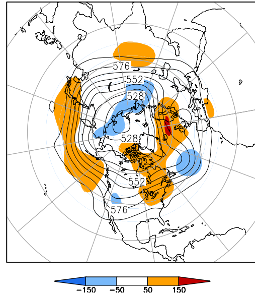
500-hPa Height (dm) & Anomalies (m) (Oct 1–15, 2013)
