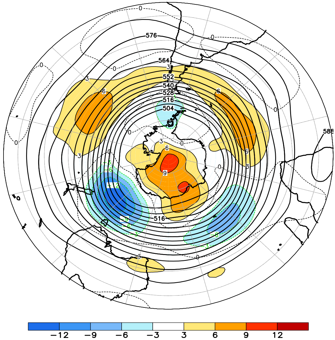
FIGURE E15. Southern Hemisphere mean and anomalous 500-hPa geopotential height (CDAS/Reanalysis) for OCT 2013. Mean heights are denoted by solid contours drawn at an interval of 6 dam. Anomaly contour interval is 3 dam with values less (greater) than -3 dam (3 dam) indicated by dark (light) shading. Anomalies are calculated as departures from the 1981-2010 base period monthly means.
