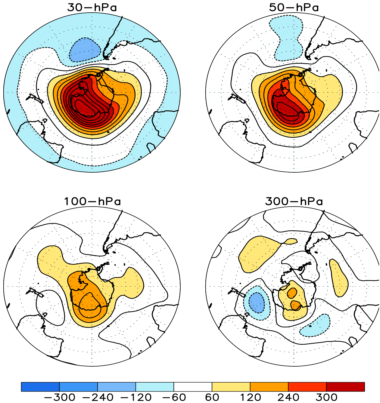
FIGURE S1. Stratospheric height anomalies (m) at selected levels for OCT 2013. Positive values are indicated by solid contours and dark shading. Negative values are indicated by dashed contours and light shading. Contour interval is 60 m. Anomalies are calculated from the 1981-2010 base period means. Winter Hemisphere is shown.
