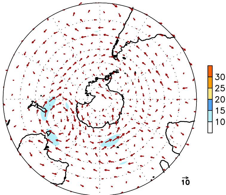
FIGURE E16. Southern Hemisphere mean (left) and anomalous (right) 300-hPa vector wind (CDAS/Reanalysis) for OCT 2013. Mean (anomaly) isotach contour interval is 10 (5) \text{ms}^{-1} . Values greater than 30 \text{ms}^{-1} (left) and 10 \text{ms}^{-1} (rights) are shaded. Anomalies are departures from the 1981-2010 base period monthly means.
