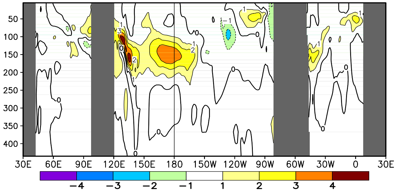
FIGURE T17. Equatorial depth–longitude section of ocean temperature (top) and ocean temperature anomalies (bottom) for OCT 2013. Contour interval is 1°C. Dashed contours in bottom panel indicate negative anomalies. Data are derived from the NCEP’s global ocean data assimilation system version 2 which assimilates oceanic observations into an oceanic GCM (Xue, Y. and Behringer, D.W., 2006: Operational global ocean data assimilation system at NCEP, to be submitted to BAMS). Anomalies are departures from the 1981–2010 base period means.
