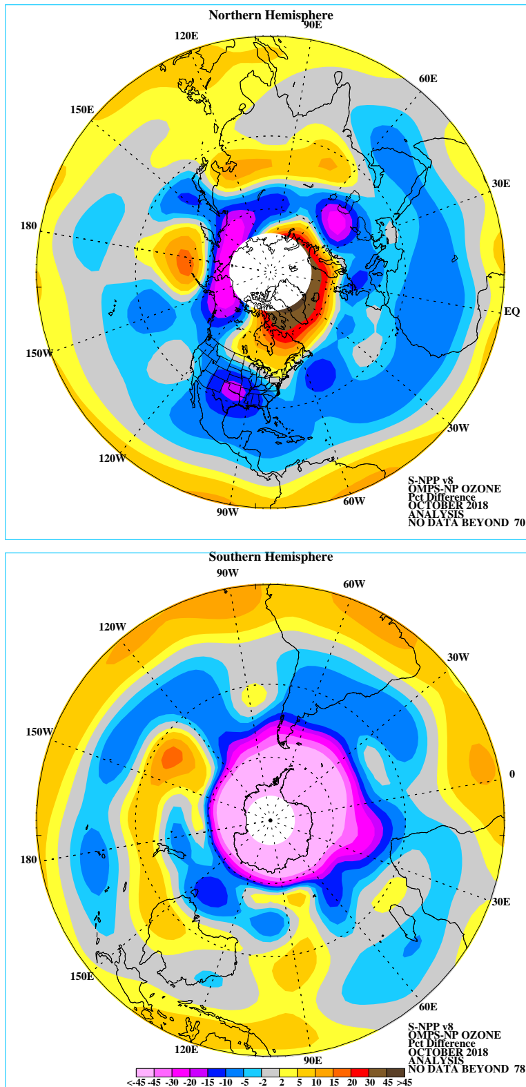
FIGURE S6. Northern (top) and Southern (bottom) Hemisphere total ozone anomaly (percent difference from monthly mean for the period 1979-1986). The region near the winter pole has no SBUV/2 data.
