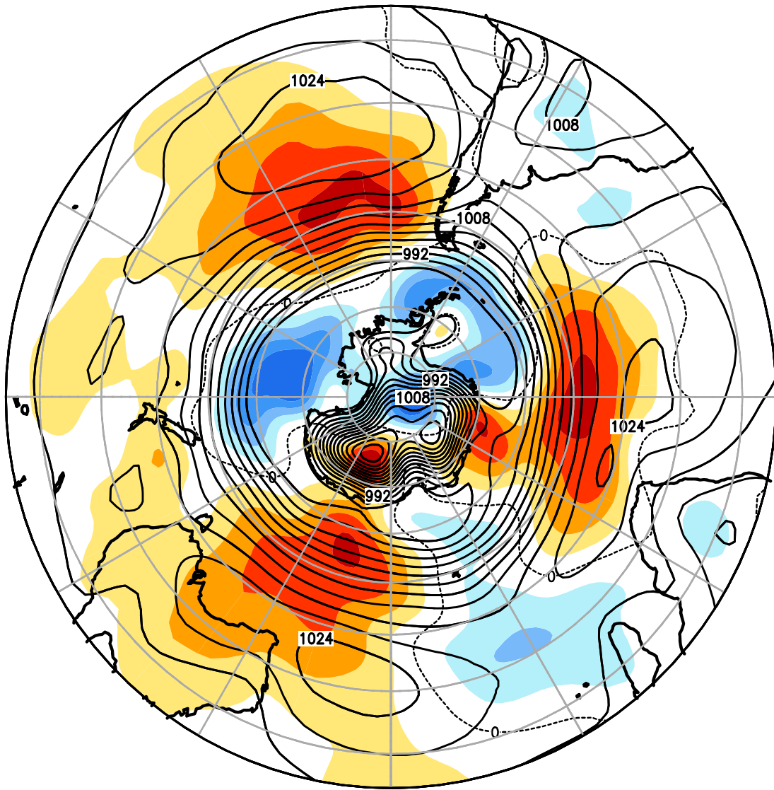
FIGURE E14. Southern Hemisphere mean and anomalous sea level pressure(CDAS/Reanalysis) for OCT 2023. Mean values are denoted by solid contours drawn at an interval of 4 hPa. Anomaly contour interval is 2 hPa with values less (greater) than -2 hPa (2 hPa) indicated by dark (light) shading. Anomalies are calculated as departures from the 1991-2020 base period monthly means.
