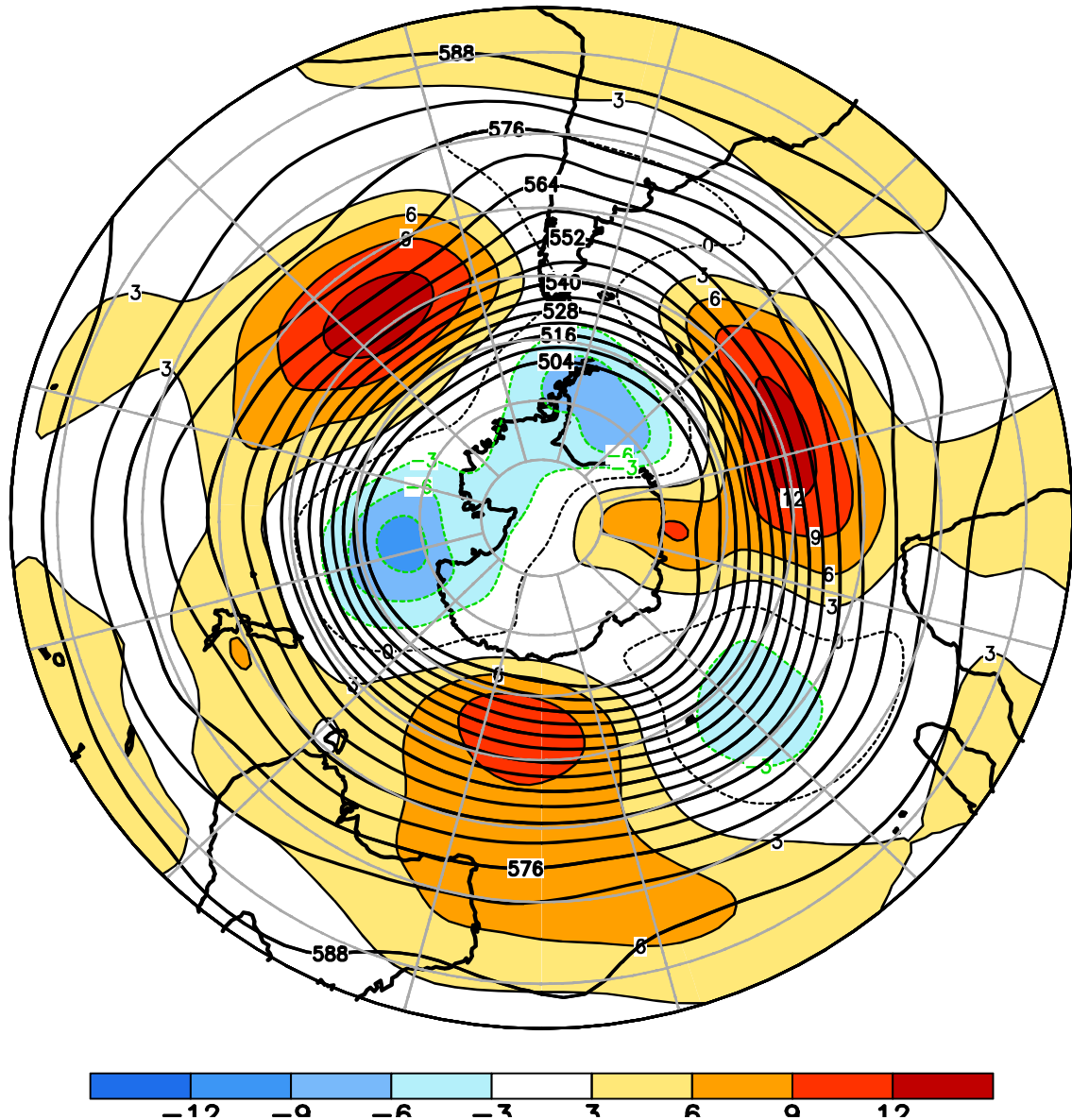
FIGURE E15. Southern Hemisphere mean and anomalous 500-hPa geopotential height (CDAS/Reanalysis) for OCT 2023. Mean heights are denoted by solid contours drawn at an interval of 6 dam. Anomaly contour interval is 3 dam with values less (greater) than -3 dam (3 dam) indicated by dark (light) shading. Anomalies are calculated as departures from the 1991-2020 base period monthly means.
