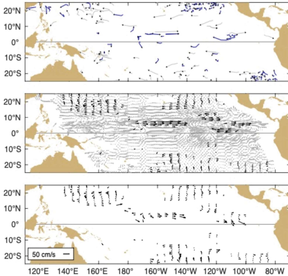
Figure A1.1 Top: Movements of drifting buoys in the tropical Pacific Ocean during October 2023. The linear segments of each trajectory represent a one week displacement. Trajectories of buoys which have lost their subsurface drogues are gray; those with drogues are black.
