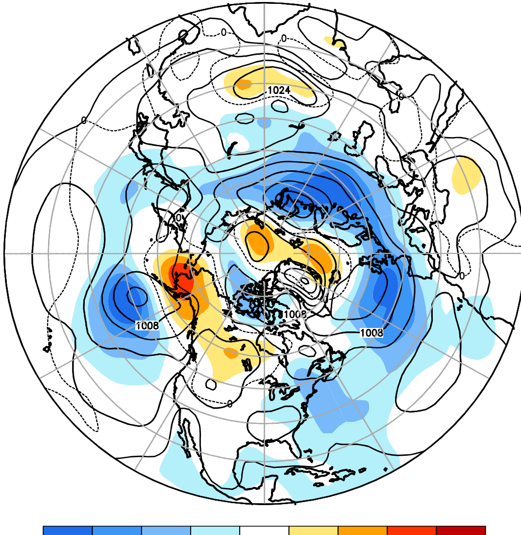
FIGURE E8. Northern Hemisphere mean and anomalous sea level pressure (CDAS/Reanalysis) for OCT 2023. Mean values are denoted by solid contours drawn at an interval of 4 hPa. Anomaly contour interval is 2 hPa with values less (greater) than -2 hPa (2 hPa) indicated by dark (light) shading. Anomalies are calculated as departures from the 1991-2020 base period monthly means.
