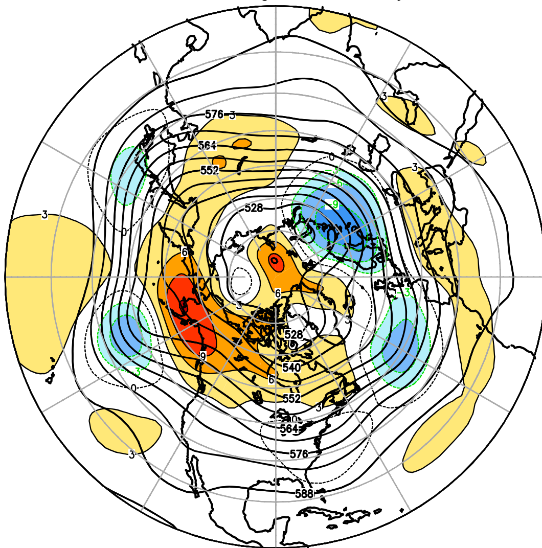
FIGURE E9. Northern Hemisphere mean and anomalous 500-hPa geopotential height (CDAS/Reanalysis) for OCT 2023. Mean heights are denoted by solid contours drawn at an interval of 6 dam. Anomaly contour interval is 3 dam with values less (greater) than -3 dam (3 dam) indicated by dark (light) shading. Anomalies are calculated as departures from the 1991-2020 base period monthly means.
