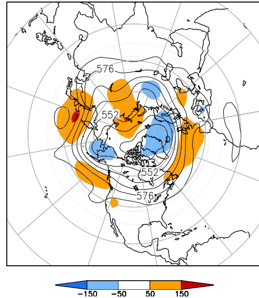
500-hPa Height (dm) & Anomalies (m) (Sep 1–15, 2012)
