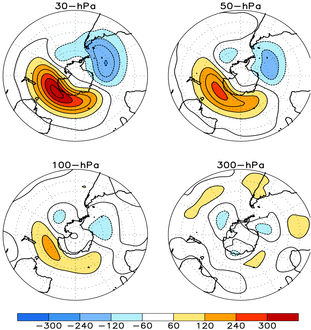
FIGURE S1. Stratospheric height anomalies (m) at selected levels for SEP 2012. Positive values are indicated by solid contours and dark shading. Negative values are indicated by dashed contours and light shading. Contour interval is 60 m. Anomalies are calculated from the 1981-2010 base period means. Winter Hemisphere is shown.
