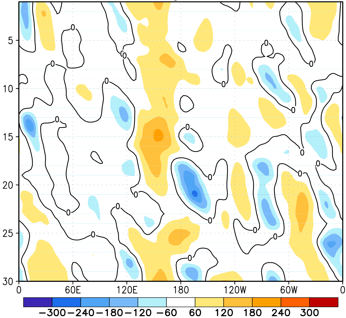
FIGURE E12. Northern Hemisphere: Daily 500-hPa height anomalies for SEP 2012 averaged over the 5° latitude band centered on 40°N. Positive values are indicated by solid contours and dark shading. Negative values are indicated by dashed contours and light shading. Contour interval is 60 m. Anomalies are departures from the 1981-2010 base period daily means.
