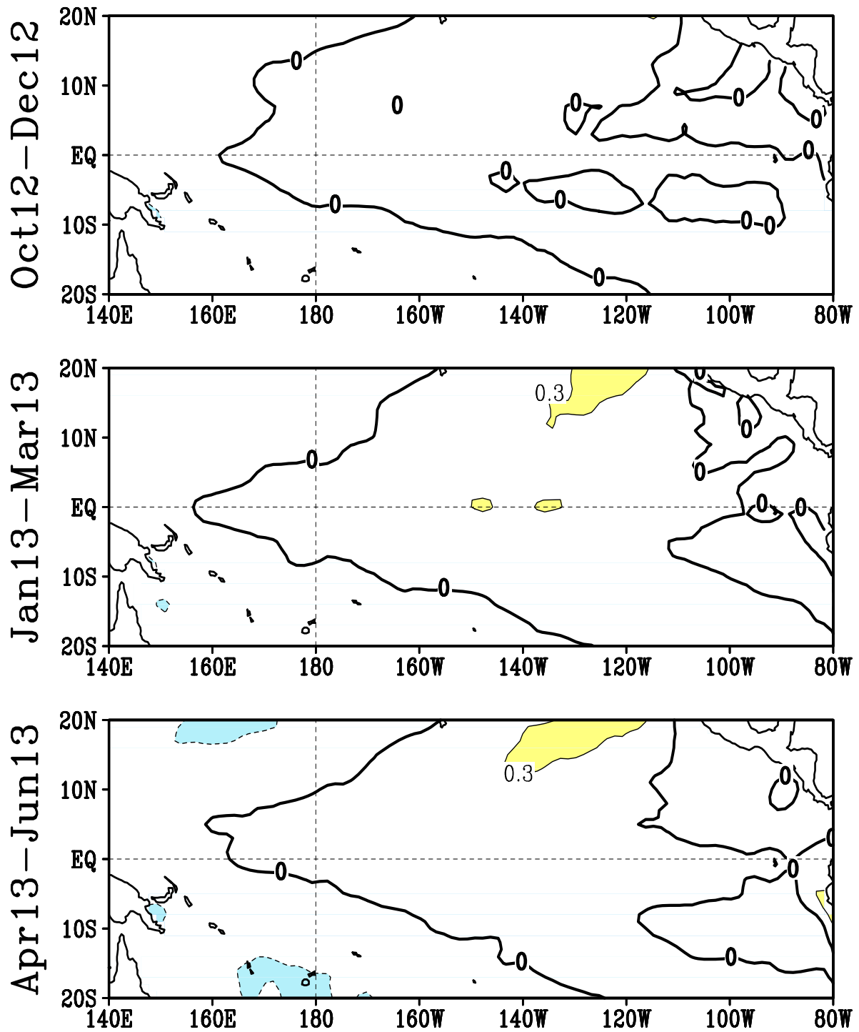
FIGURE F5. Predicted 3-month average sea surface temperature anomalies from the NCEP/CPC Markov model (Xue et al. 2000, J. Climate , 13 , 849-871). The forecast is initiated in SEP 2012. Contour interval is 0.3C and negative anomalies are indicated by dashed contours. Anomalies are calculated relative to the 1971-2000 climatology.
