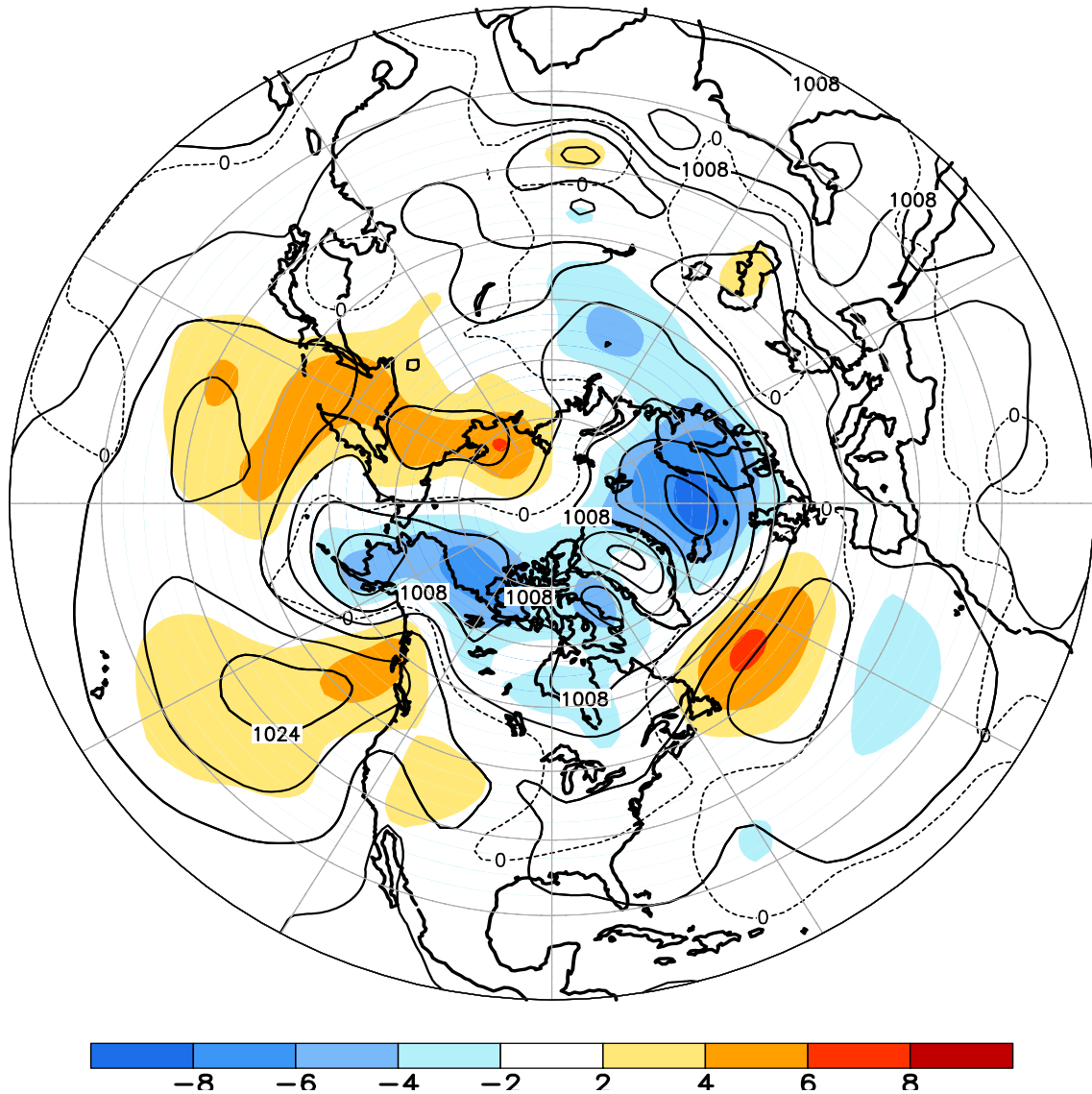
FIGURE E8. Northern Hemisphere mean and anomalous sea level pressure (CDAS/Reanalysis) for SEP 2012. Mean values are denoted by solid contours drawn at an interval of 4 hPa. Anomaly contour interval is 2 hPa with values less (greater) than -2 hPa (2 hPa) indicated by dark (light) shading. Anomalies are calculated as departures from the 1981-2010 base period monthly means.
