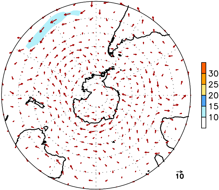
FIGURE E16. Southern Hemisphere mean (left) and anomalous (right) 300-hPa vector wind (CDAS/Reanalysis) for SEP 2012. Mean (anomaly) isotach contour interval is 10 (5) ms -1 . Values greater than 30 ms -1 (left) and 10 ms -1 (rights) are shaded. Anomalies are departures from the 1981-2010 base period monthly means.
