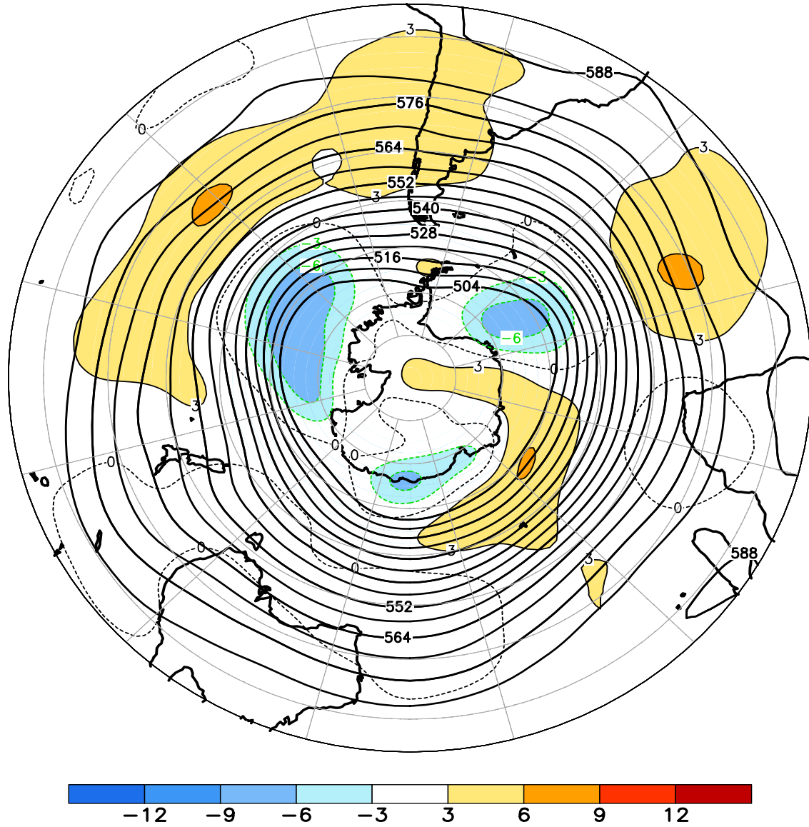
FIGURE E15. Southern Hemisphere mean and anomalous 500-hPa geopotential height (CDAS/Reanalysis) for SEP 2012. Mean heights are denoted by solid contours drawn at an interval of 6 dam. Anomaly contour interval is 3 dam with values less (greater) than -3 dam (3 dam) indicated by dark (light) shading. Anomalies are calculated as departures from the 1981-2010 base period monthly means.
