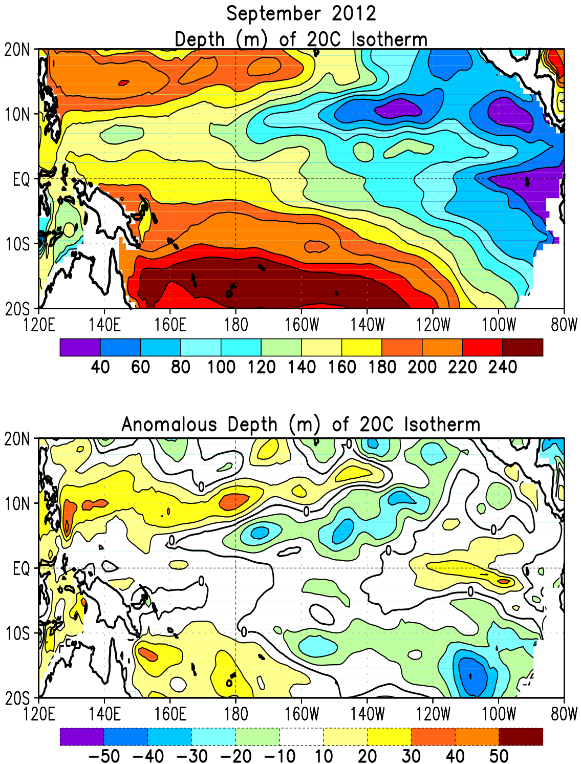
FIGURE T16. Mean (top) and anomalous (bottom) depth of the 20°C isotherm for SEP 2012. Contour interval is 40 m (top) and 10 m (bottom). Dashed contours in bottom panel indicate negative anomalies. Data are derived from the NCEP’s global ocean data assimilation system version 2 which assimilates oceanic observations into an oceanic GCM (Xue, Y. and Behringer, D.W., 2006: Operational global ocean data assimilation system at NCEP, to be submitted to BAMS). Anomalies are departures from the 1981–2010 base period means.
