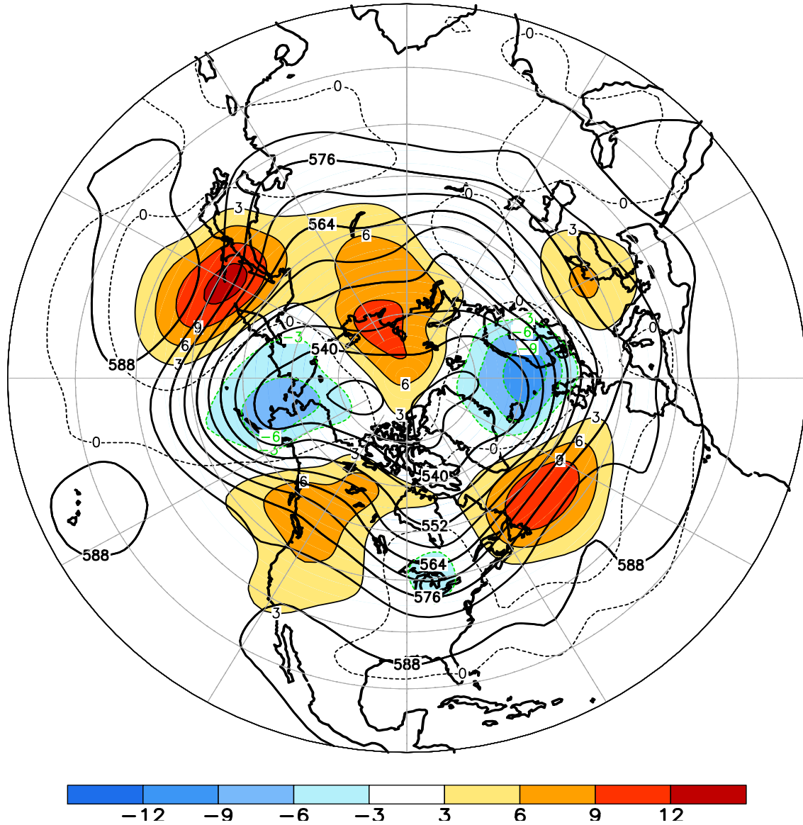
FIGURE E9. Northern Hemisphere mean and anomalous 500-hPa geopotential height (CDAS/Reanalysis) for SEP 2012. Mean heights are denoted by solid contours drawn at an interval of 6 dam. Anomaly contour interval is 3 dam with values less (greater) than -3 dam (3 dam) indicated by dark (light) shading. Anomalies are calculated as departures from the 1981-2010 base period monthly means.
