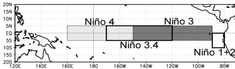
FIGURE T5. Niño region indices, calculated as the area-averaged sea surface temperature anomalies (C) for the specified region. The Niño 1+2 region (top) covers the extreme eastern equatorial Pacific between 0-10S, 90W-80W. The Niño-3 region (2nd from top) spans the eastern equatorial Pacific between 5N-5S, 150W-90W. The Niño 3.4 region (3rd from top) spans the east-central equatorial Pacific between 5N-5S, 170W-120W. The Niño 4 region (bottom) spans the date line and covers the area 5N-5S, 160E-150W. Anomalies are departures from the 1981-2010 base period monthly means ( Smith and Reynolds 1998, J. Climate, 11, 3320-3323 ). Monthly values of each index are also displayed in Table 2 .
