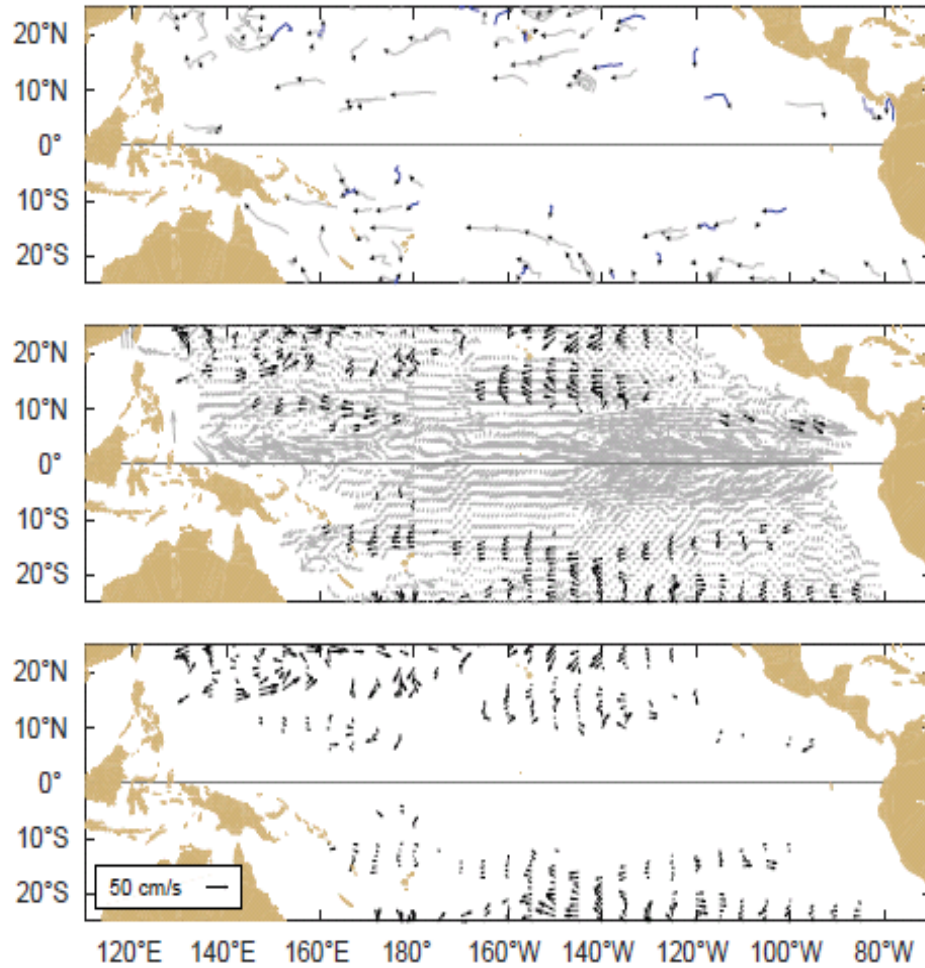
Figure A1.1 Top: Movements of drifting buoys in the tropical Pacific Ocean during September 2017. The linear segments of each trajectory represent a one week displacement. Trajectories of buoys which have lost their subsurface drogues are gray; those with drogues are black.
