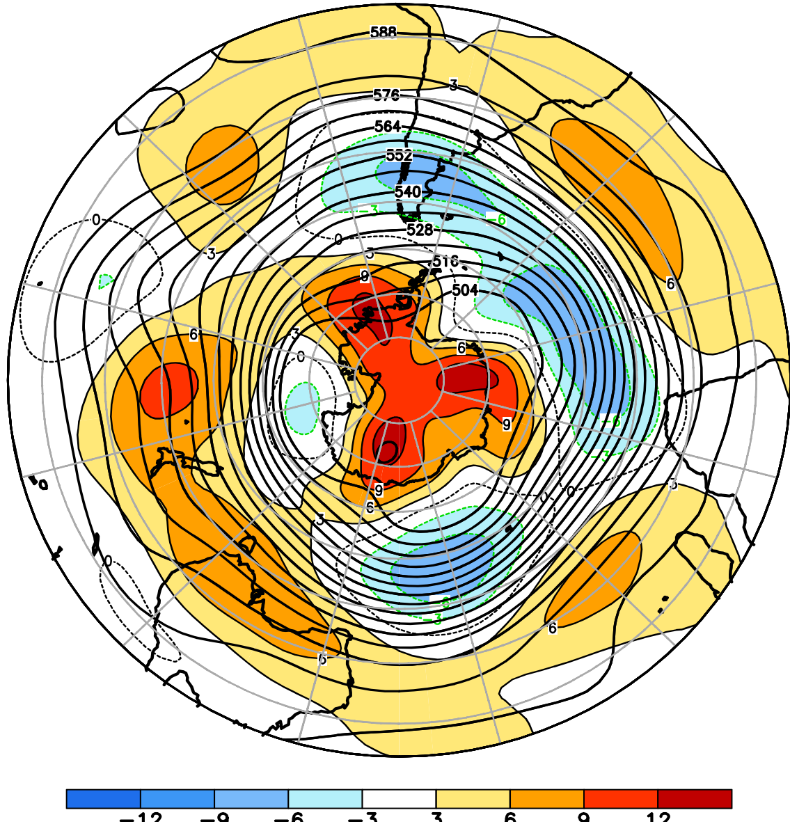
FIGURE E15. Southern Hemisphere mean and anomalous 500-hPa geopotential height (CDAS/Reanalysis) for SEP 2023. Mean heights are denoted by solid contours drawn at an interval of 6 dam. Anomaly contour interval is 3 dam with values less (greater) than -3 dam (3 dam) indicated by dark (light) shading. Anomalies are calculated as departures from the 1991-2020 base period monthly means.
