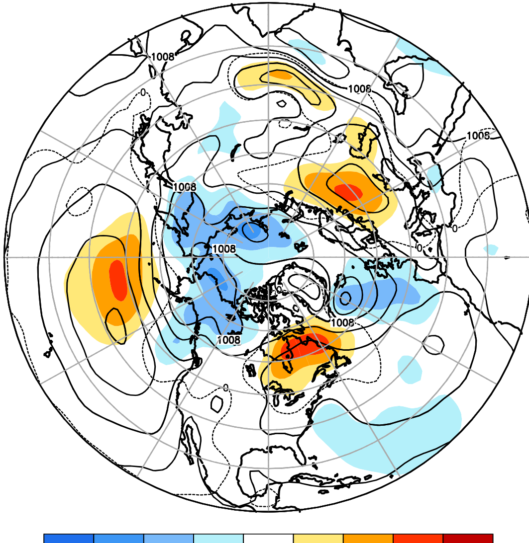
FIGURE E8. Northern Hemisphere mean and anomalous sea level pressure (CDAS/Reanalysis) for SEP 2023. Mean values are denoted by solid contours drawn at an interval of 4 hPa. Anomaly contour interval is 2 hPa with values less (greater) than -2 hPa (2 hPa) indicated by dark (light) shading. Anomalies are calculated as departures from the 1991-2020 base period monthly means.
