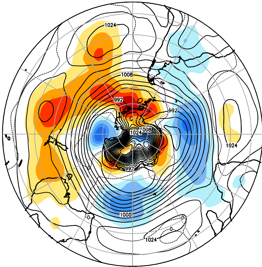
FIGURE E14. Southern Hemisphere mean and anomalous sea level pressure(CDAS/Reanalysis) for SEP 2023. Mean values are denoted by solid contours drawn at an interval of 4 hPa. Anomaly contour interval is 2 hPa with values less (greater) than -2 hPa (2 hPa) indicated by dark (light) shading. Anomalies are calculated as departures from the 1991-2020 base period monthly means.
