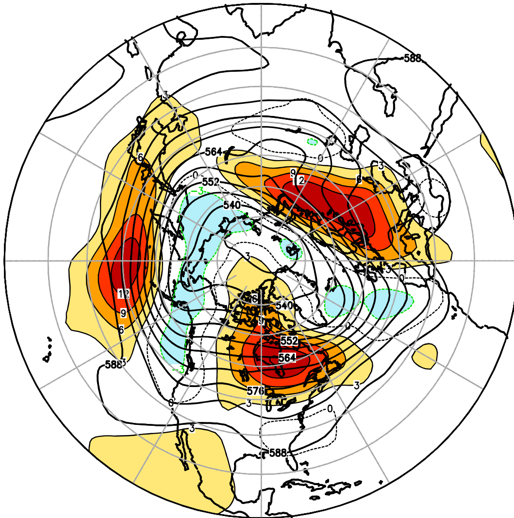
FIGURE E9. Northern Hemisphere mean and anomalous 500-hPa geopotential height (CDAS/Reanalysis) for SEP 2023. Mean heights are denoted by solid contours drawn at an interval of 6 dam. Anomaly contour interval is 3 dam with values less (greater) than -3 dam (3 dam) indicated by dark (light) shading. Anomalies are calculated as departures from the 1991-2020 base period monthly means.
