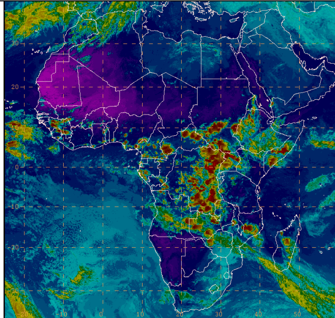
IR Satellite Image (valid 16220Z of 23 October 2013)
