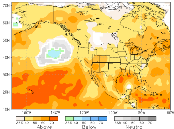
NMME prob fcst TMP2m IC=201704 for lead 1 2017 MJJ
