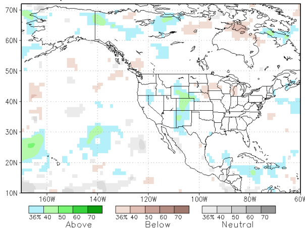
NMME prob fcst Prate IC=201704 for lead 1 2017 MJJ
