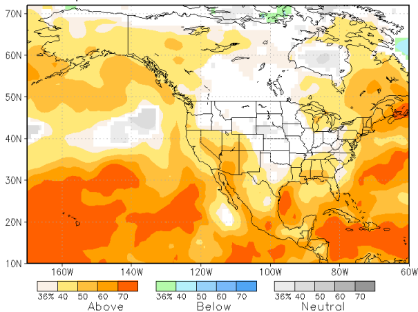
NMME prob fcast TMP2m IC=201705 for lead 1 2017 JJA
