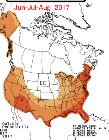
NMME prob fcast TMP2m IC=201705 for lead 1 2017 JJA
