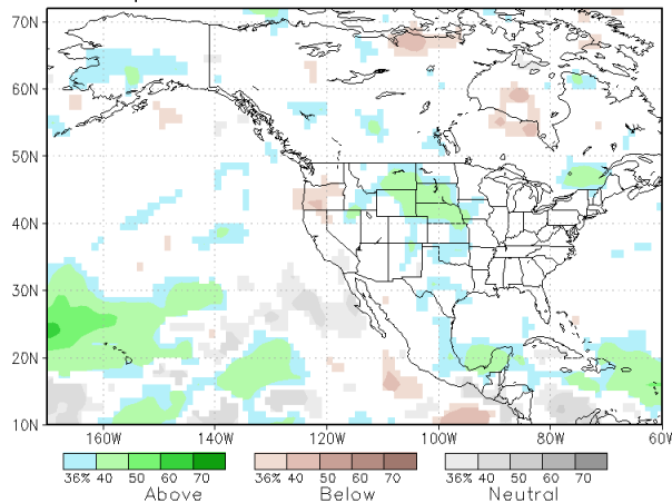
NMME prob fcast Prate IC=201705 for lead 1 2017 JJA
