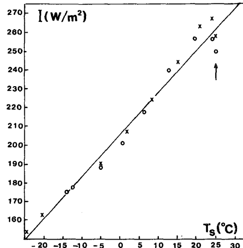
FIG. 1b. As in Fig. 1a except for the surface temperature. The straight line shows the parameterization used in the model. The arrow indicates the dip in I in the equatorial region.
