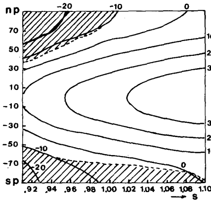
FIG. 9. Sea level temperature distribution in the warm branch for a range of solar constants. Isotherms are drawn every 10^{\circ}\text{C} ; hatched areas indicate an ice cover of 50% or more.
