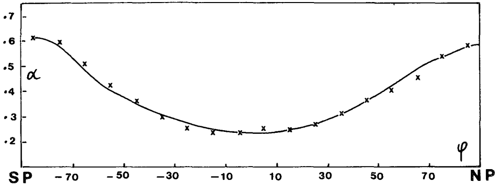
FIG. 4. Computed albedo (solid line) compared with observed values given by Ellis and Vonder Haar (1976).
