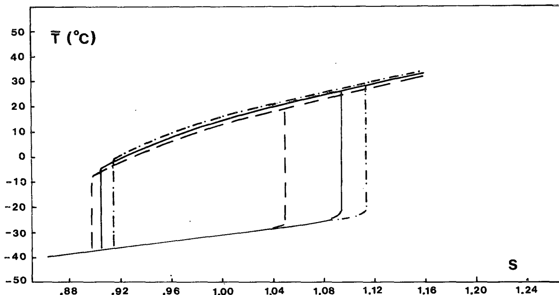
FIG. 11. Solution diagram for three diffusivities: D=0.4 (dashed line), D=0.7 (solid line), D=1.0 (dot-dashed line) W (m^2 ^\circ C)^{-1} . The solid line corresponds to the standard case.
