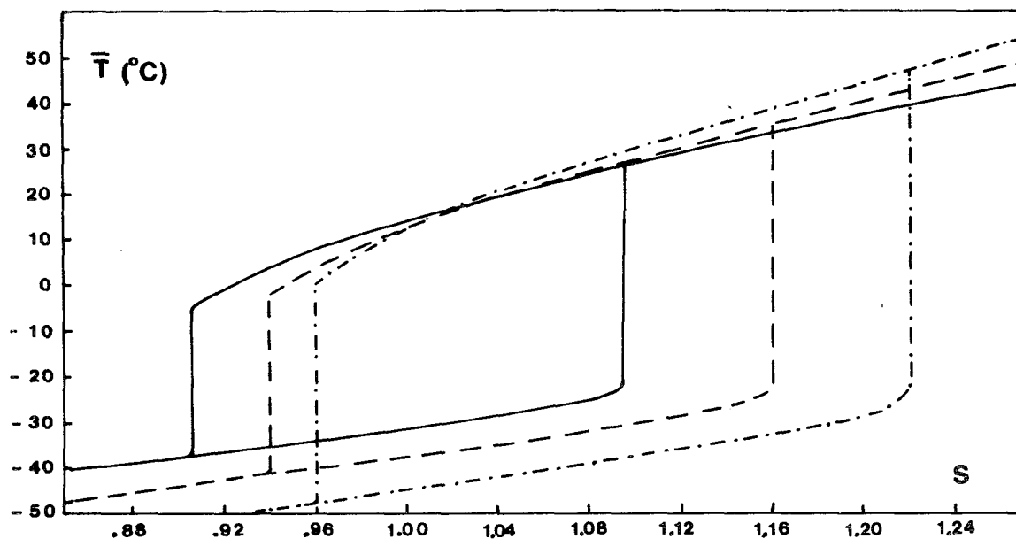
FIG. 10. Solution diagrams for three parameterizations of the outgoing radiation: 205+2.23 T_s (solid line), 210+2.00 T_s (dashed line), 213+1.75 T_s (dot-dashed line) W m^{-2} . The solid line corresponds to the standard case.
