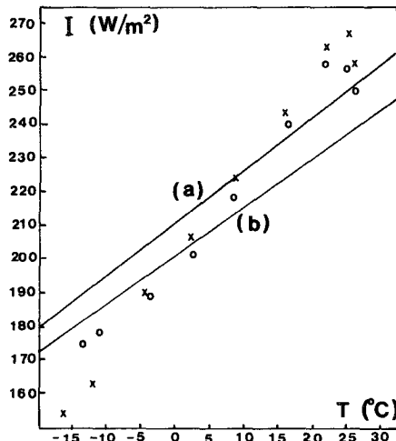
FIG. 1a. The annual infrared emission as a function of the mean sea level temperature for belts of 10° latitude. Circles refer to the Northern Hemisphere, crosses to the Southern. Lines (a) and (b) indicate relations used by earlier workers.
