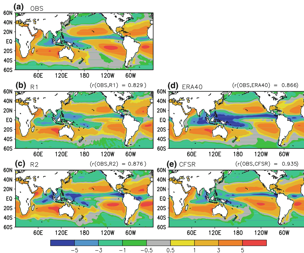
Fig. 2 1988–2000 average of E - P . a Observation, b R1, c R2, d ERA40, and e CFSR. Unit is mm/day and values are shaded at -5 , -3 , -1 , -0.5 , 0.5 , 1 , 3 , and 5
