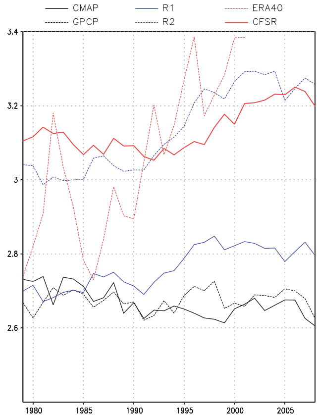
Fig. 10 Annual mean of global average precipitation (mm/day) for CMAP (solid black), GPCP (dashed black), R1 (solid blue), R2 (dashed blue), ERA40 (dashed red), and CFSR (solid red)
