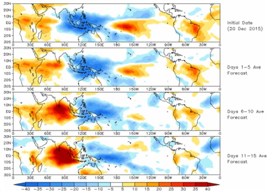
OLR prediction of MJO-related anomalies using CA model reconstruction by RMM1 & RMM2 (20 Dec 2015)
