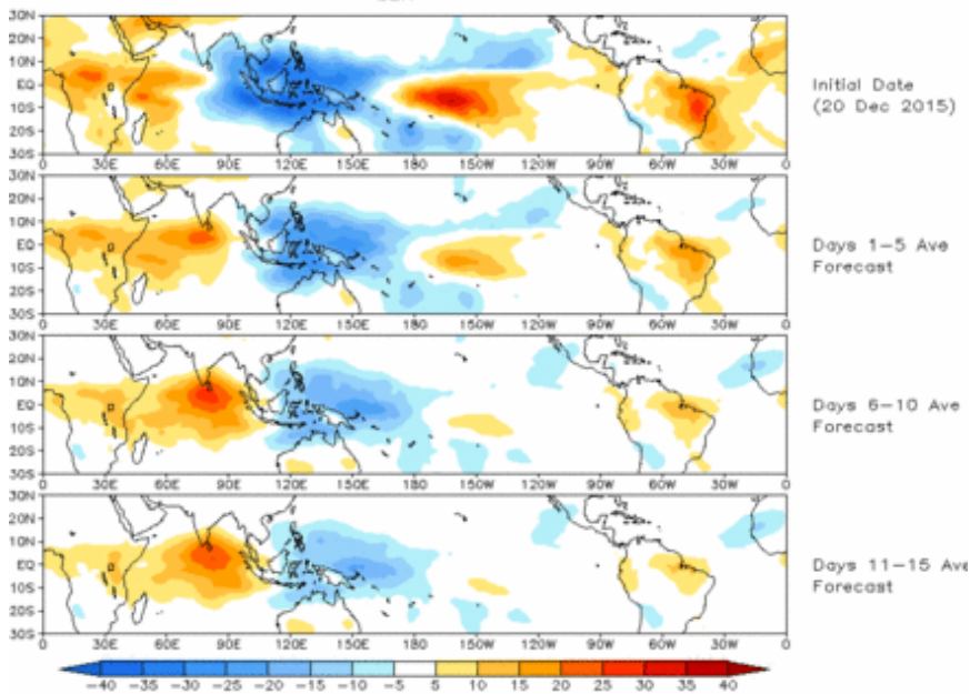
Prediction of MJO-related anomalies using GEFS operational forecast Initial date: 20 Dec 2015 OLR
