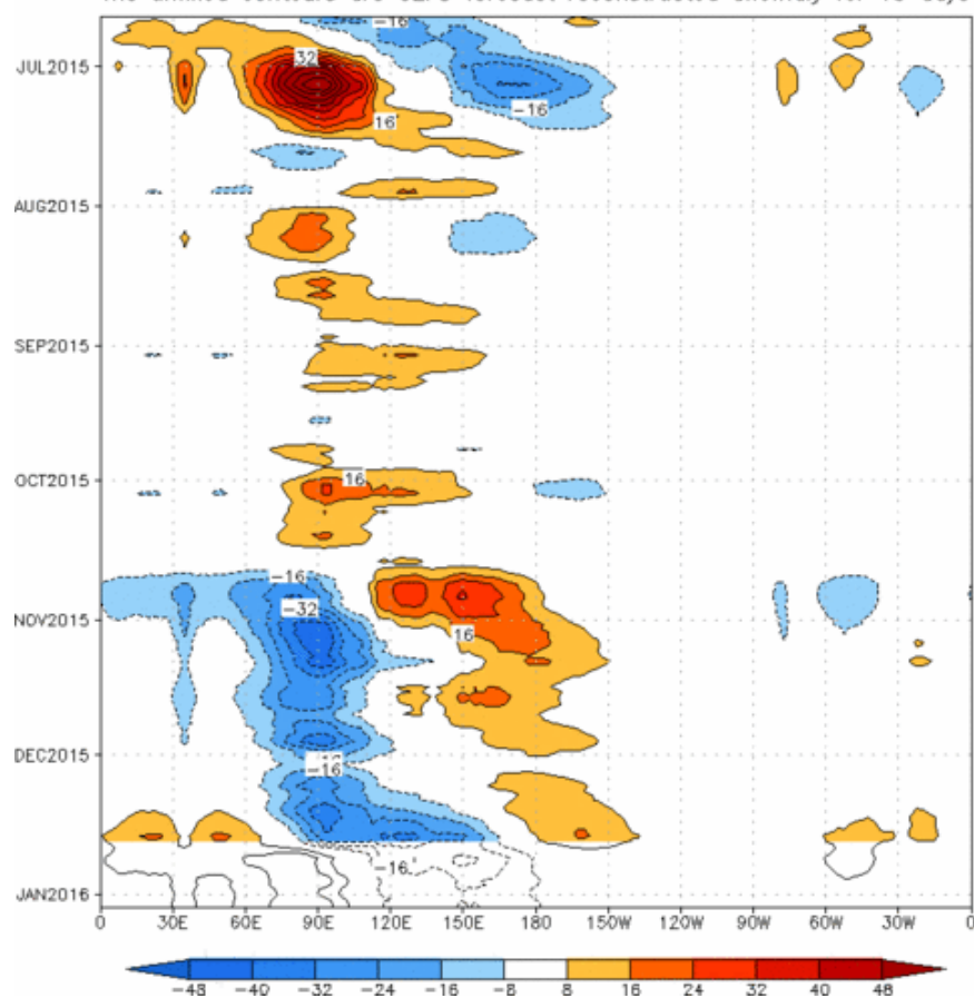
Reconstructed anomaly field associated with the MJO using RMM1 & RMM2 OLR [7.5°S,7.5°N] (cont:4Wm -2 ) Period:20-Jun-2015 to 20-Dec-2015 The unfilled contours are GEFS forecast reconstructed anomaly for 15 days
