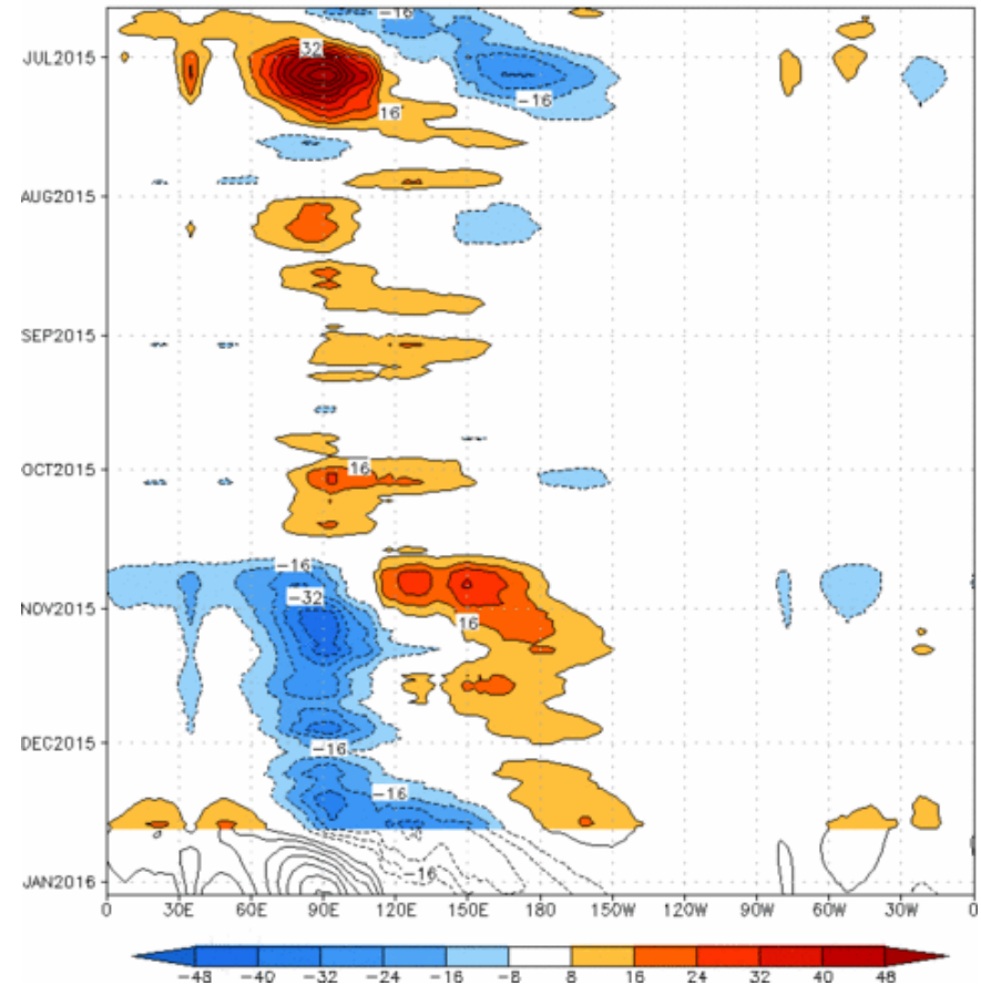
Reconstructed anomaly field associated with the MJO using RMM1 & RMM2 OLR [7.5°S,7.5°N] (cont:4Wm -2 ) Period:20-Jun-2015 to 20-Dec-2015 The unfilled contours are CA forecast reconstructed anomaly for 15 days
