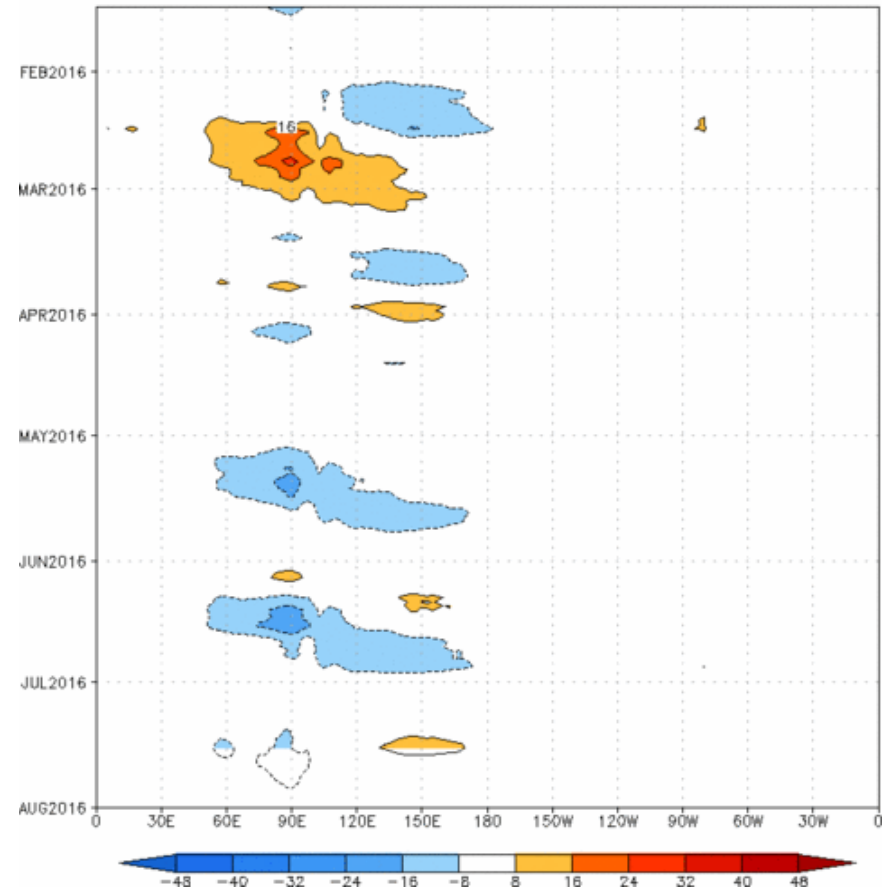
Reconstructed anomaly field associated with the MJO using RMM1 & RMM2 OLR [ 7.5^\circ S, 7.5^\circ N] ( \text{cint}: 4\text{Wm}^{-2} ) Period: 16-Jan-2016 to 17-Jul-2016 The unfilled contours are CA forecast reconstructed anomaly for 15 days
