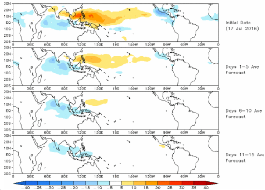
OLR prediction of MJO-related anomalies using CA model reconstruction by RMM1 & RMM2 (17 Jul 2016)
