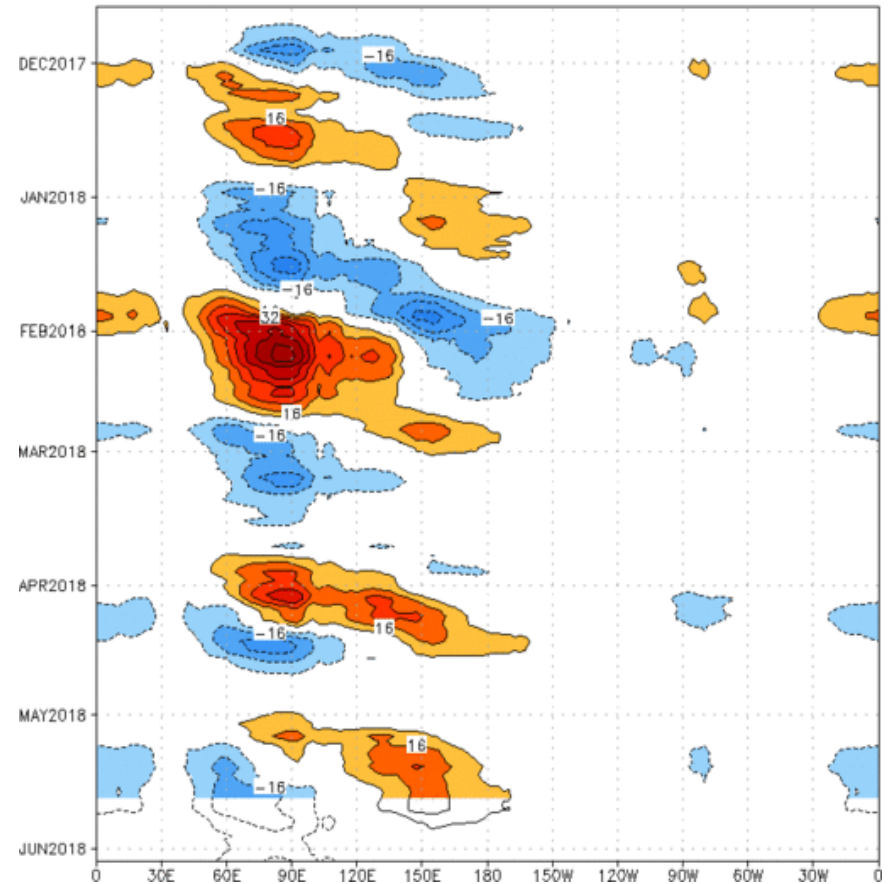
Reconstructed anomaly field associated with the MJO using RMM1 & RMM2 OLR [ 7.5^{\circ} S, 7.5^{\circ} N] (cont: 4\text{Wm}^{-2} ) Period: 18–Nov–2017 to 20–May–2018 The unfilled contours are GEFS forecast reconstructed anomaly for 15 days
