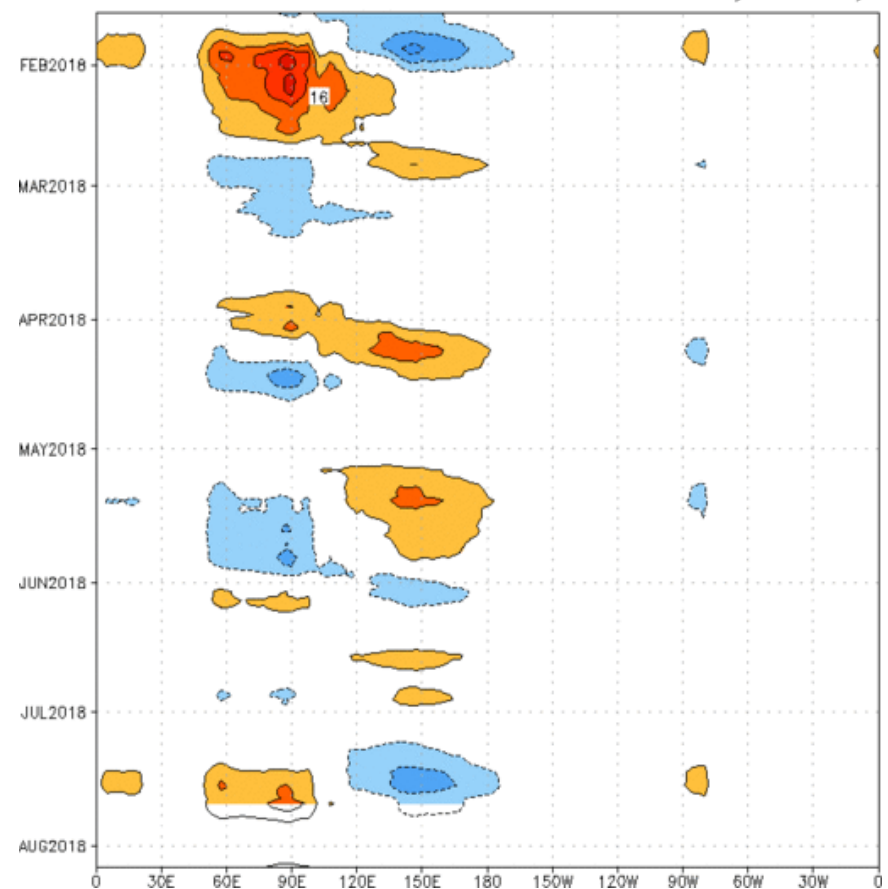
Reconstructed anomaly field associated with the MJO using RMM1 & RMM2 OLR [ 7.5^{\circ} S, 7.5^{\circ} N] (cont: 4\text{Wm}^{-2} ) Period: 20-Jan-2018 to 22-Jul-2018 The unfilled contours are GEFS forecast reconstructed anomaly for 15 days
