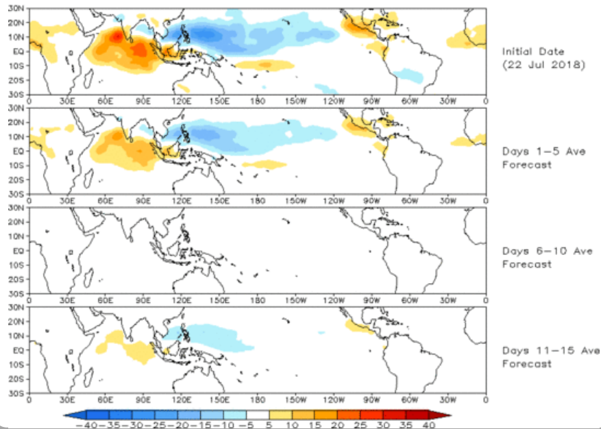
Prediction of MJO-related anomalies using GEFS operational forecast Initial date: 22 Jul 2018 OLR
