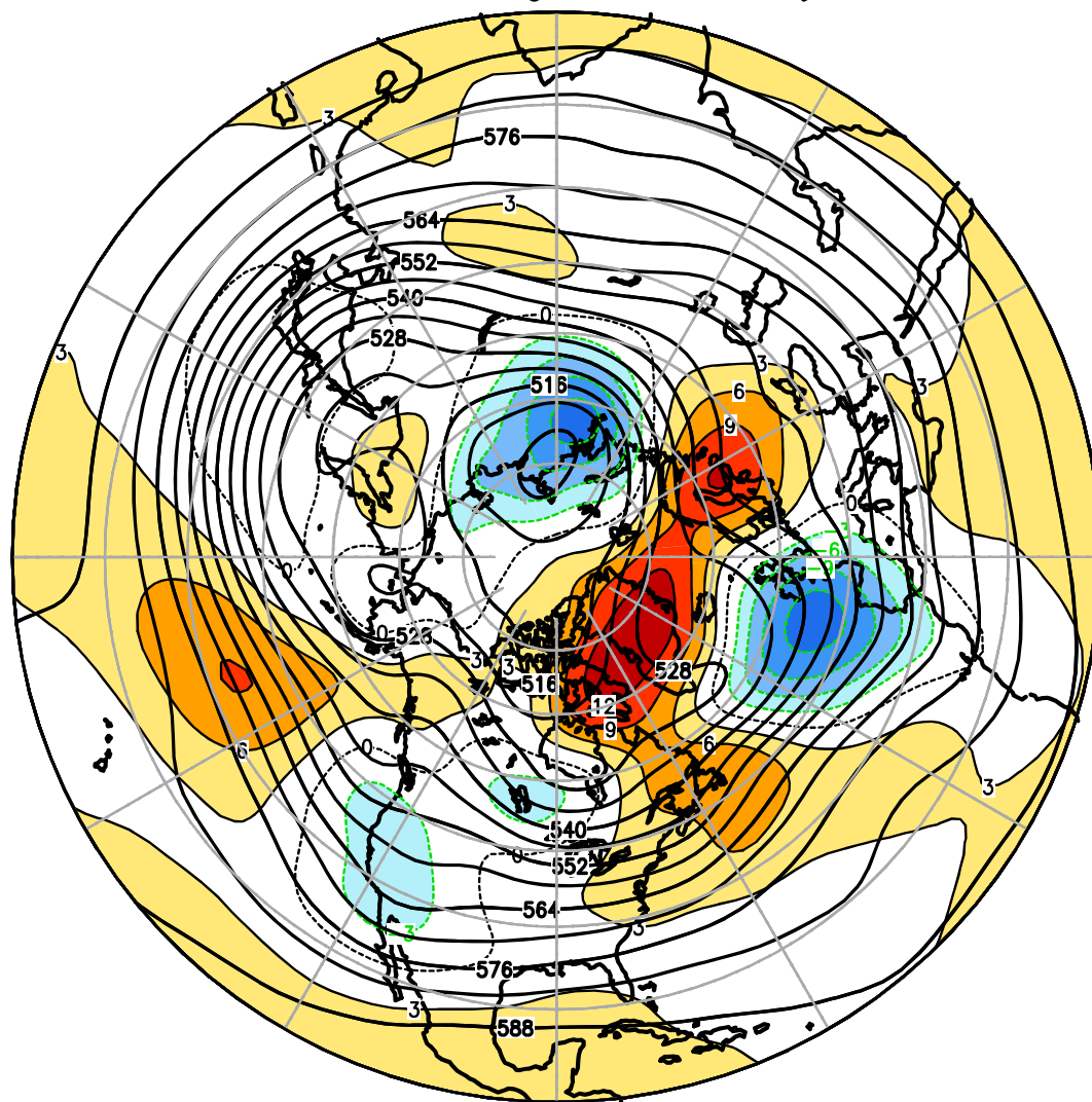
FIGURE E9. Northern Hemisphere mean and anomalous 500-hPa geopotential height (CDAS/Reanalysis) for MAR 2024. Mean heights are denoted by solid contours drawn at an interval of 6 dam. Anomaly contour interval is 3 dam with values less (greater) than -3 dam (3 dam) indicated by dark (light) shading. Anomalies are calculated as departures from the 1991-2020 base period monthly means.
