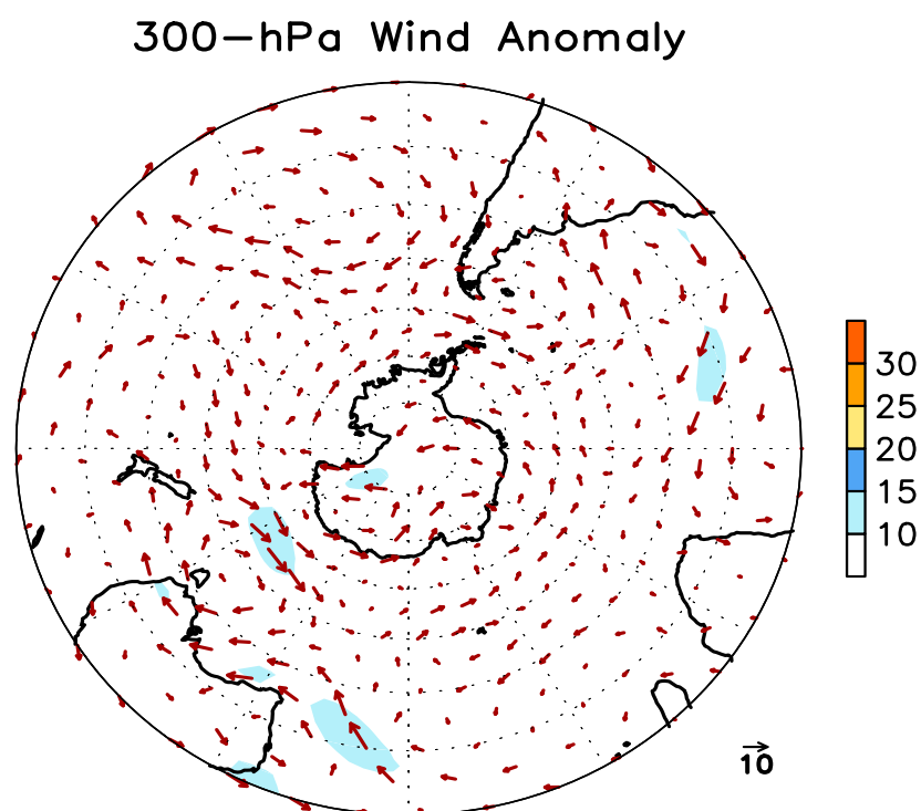
FIGURE E16. Southern Hemisphere mean (left) and anomalous (right) 300-hPa vector wind (CDAS/Reanalysis) for APR 2020. Mean (anomaly) isotach contour interval is 10 (5) \text{ms}^{-1} . Values greater than 30 \text{ms}^{-1} (left) and 10 \text{ms}^{-1} (rights) are shaded. Anomalies are departures from the 1981-2010 base period monthly means.
