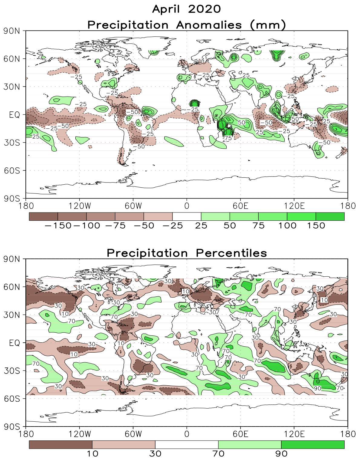
FIGURE E3. Anomalous precipitation (mm, top) and precipitation percentiles based on a Gamma distribution fit to the 1981–2010 base period data (bottom) for APR 2020. Data are obtained from a merge of raingauge observations and satellite-derived precipitation estimates (Janowiak and Xie 1999, J. Climate , 12 , 3335–3342). Contours are drawn at 200, 100, 50, 25, -25, -50, -100, and -200 mm in top panel. Percentiles are not plotted in regions where mean monthly precipitation is <5mm/month.
