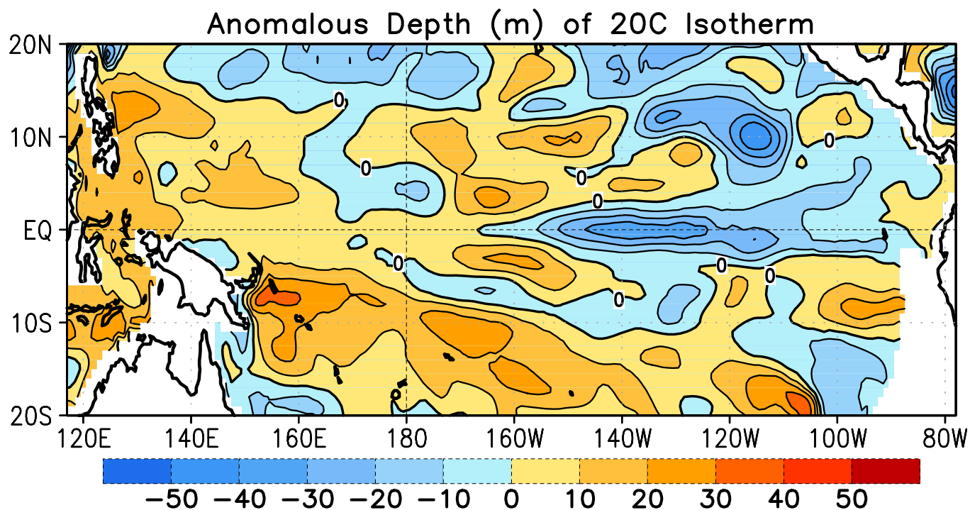
FIGURE T16. Mean (top) and anomalous (bottom) depth of the 20°C isotherm for AUG 2021. Contour interval is 40 m (top) and 10 m (bottom). Dashed contours in bottom panel indicate negative anomalies. Data are derived from the NCEP's global ocean data assimilation system version 2 which assimilates oceanic observations into an oceanic GCM (Xue, Y. and Behringer, D.W., 2006: Operational global ocean data assimilation system at NCEP, to be submitted to BAMS). Anomalies are departures from the 1991-2020 base period means.
