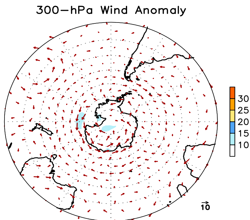
FIGURE E16. Southern Hemisphere mean (left) and anomalous (right) 300-hPa vector wind (CDAS/Reanalysis) for AUG 2021. Mean (anomaly) isotach contour interval is 10 (5) \text{ms}^{-1} . Values greater than 30 \text{ms}^{-1} (left) and 10 \text{ms}^{-1} (rights) are shaded. Anomalies are departures from the 1991-2020 base period monthly means.
