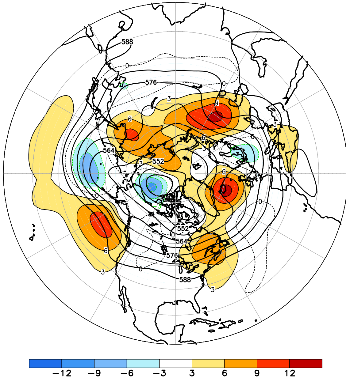
FIGURE E9. Northern Hemisphere mean and anomalous 500-hPa geopotential height (CDAS/Reanalysis) for AUG 2021. Mean heights are denoted by solid contours drawn at an interval of 6 dam. Anomaly contour interval is 3 dam with values less (greater) than -3 dam (3 dam) indicated by dark (light) shading. Anomalies are calculated as departures from the 1991-2020 base period monthly means.
