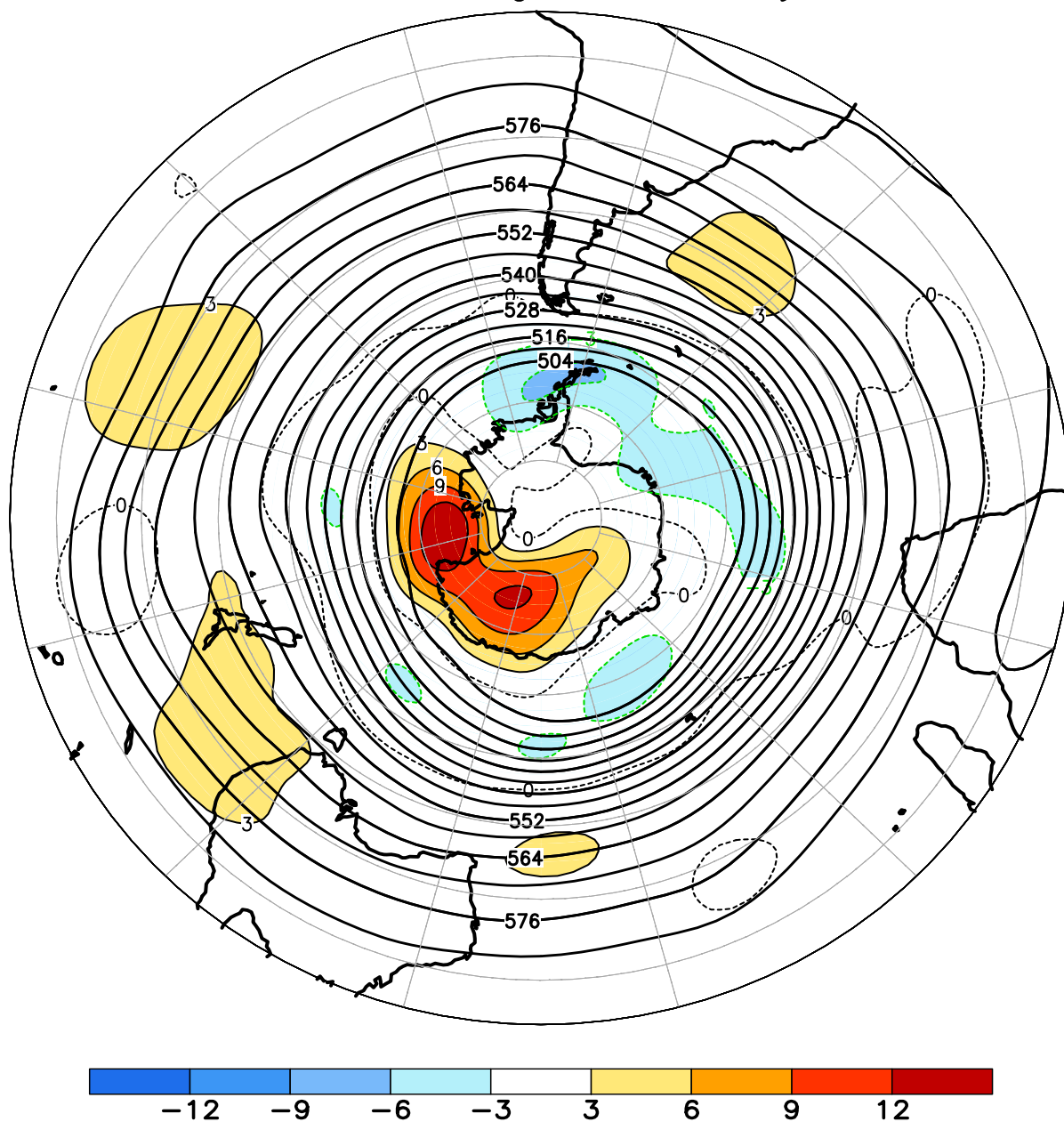
FIGURE E15. Southern Hemisphere mean and anomalous 500-hPa geopotential height (CDAS/Reanalysis) for AUG 2021. Mean heights are denoted by solid contours drawn at an interval of 6 dam. Anomaly contour interval is 3 dam with values less (greater) than -3 dam (3 dam) indicated by dark (light) shading. Anomalies are calculated as departures from the 1991-2020 base period monthly means.
