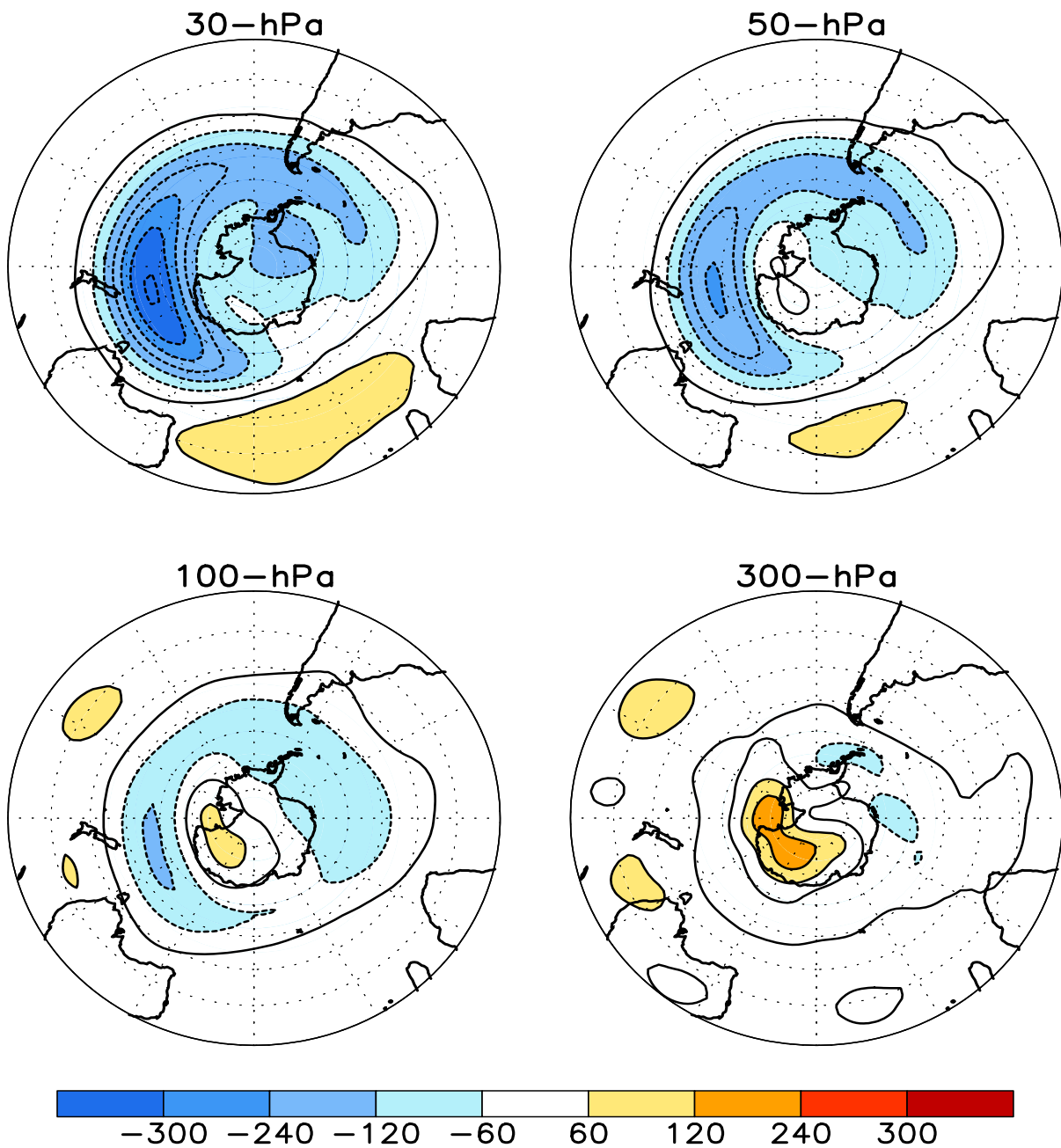
FIGURE S1. Stratospheric height anomalies (m) at selected levels for AUG 2021. Positive values are indicated by solid contours and dark shading. Negative values are indicated by dashed contours and light shading. Contour interval is 60 m. Anomalies are calculated from the 1991-2020 base period means. Winter Hemisphere is shown.
