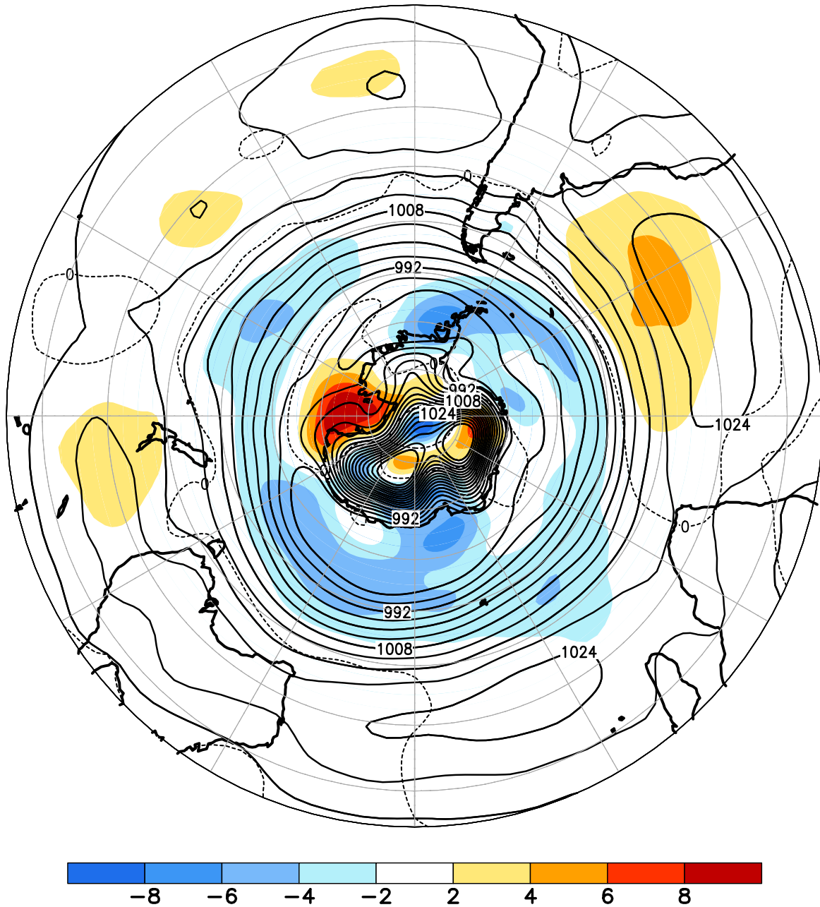
FIGURE E14. Southern Hemisphere mean and anomalous sea level pressure(CDAS/Reanalysis) for AUG 2021. Mean values are denoted by solid contours drawn at an interval of 4 hPa. Anomaly contour interval is 2 hPa with values less (greater) than -2 hPa (2 hPa) indicated by dark (light) shading. Anomalies are calculated as departures from the 1991-2020 base period monthly means.
