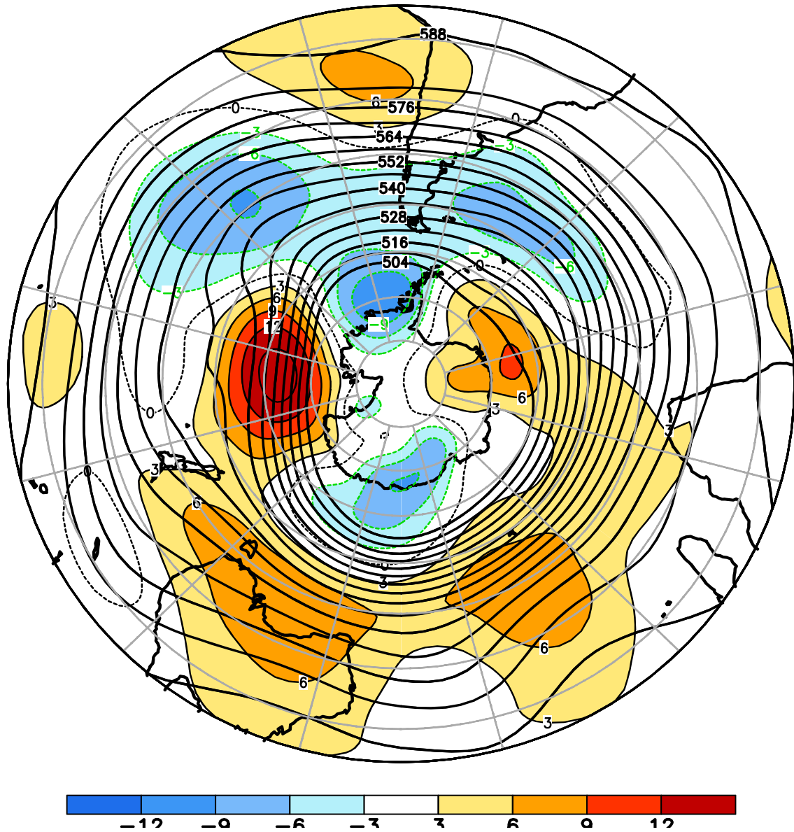
FIGURE E15. Southern Hemisphere mean and anomalous 500-hPa geopotential height (CDAS/Reanalysis) for AUG 2023. Mean heights are denoted by solid contours drawn at an interval of 6 dam. Anomaly contour interval is 3 dam with values less (greater) than -3 dam (3 dam) indicated by dark (light) shading. Anomalies are calculated as departures from the 1991-2020 base period monthly means.
