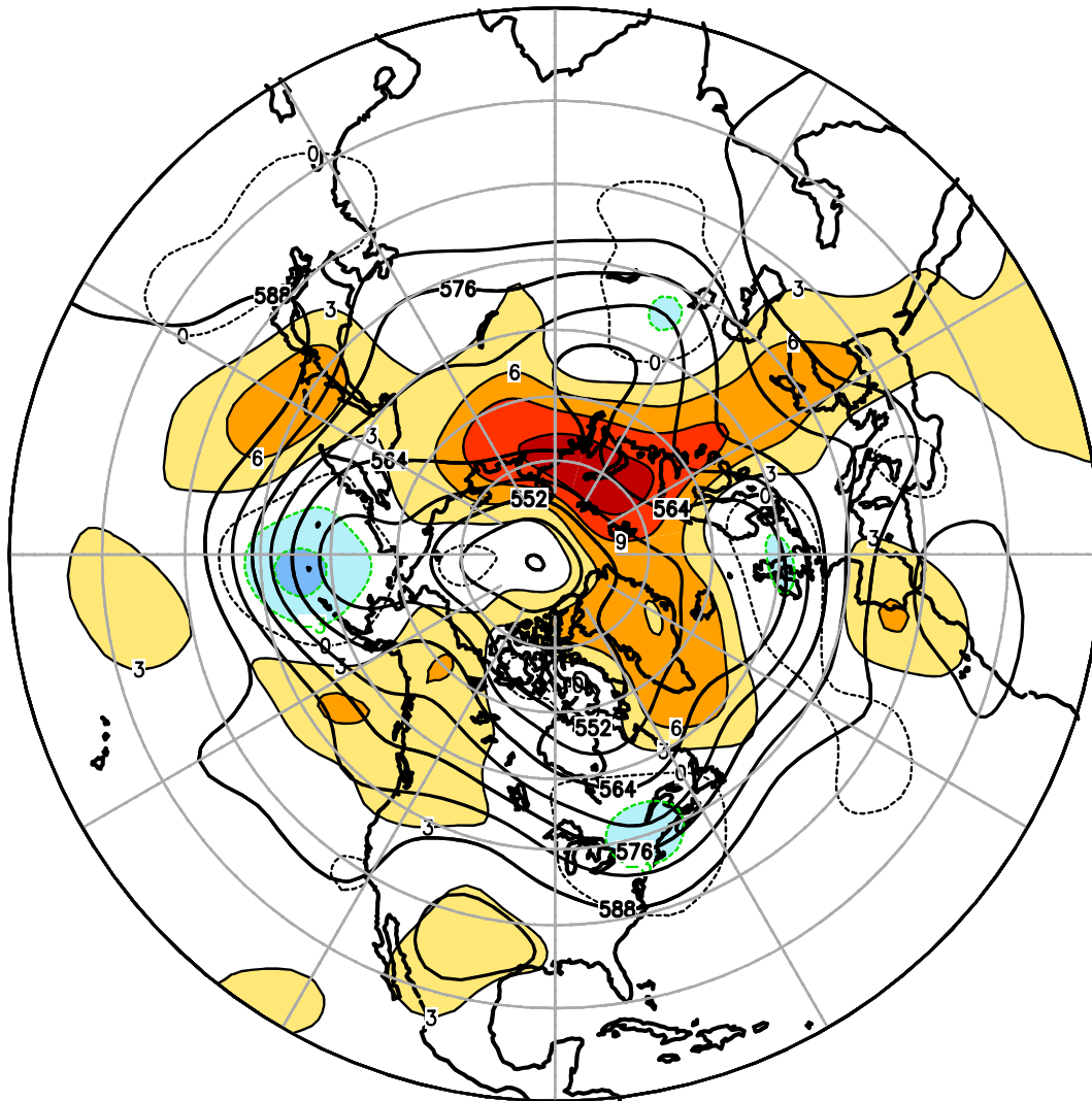
FIGURE E9. Northern Hemisphere mean and anomalous 500-hPa geopotential height (CDAS/Reanalysis) for AUG 2023. Mean heights are denoted by solid contours drawn at an interval of 6 dam. Anomaly contour interval is 3 dam with values less (greater) than -3 dam (3 dam) indicated by dark (light) shading. Anomalies are calculated as departures from the 1991-2020 base period monthly means.
