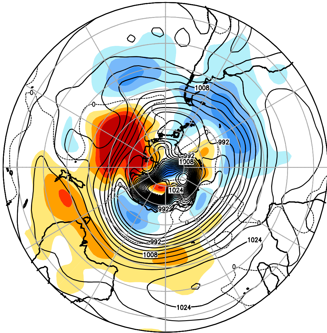
FIGURE E14. Southern Hemisphere mean and anomalous sea level pressure(CDAS/Reanalysis) for AUG 2023. Mean values are denoted by solid contours drawn at an interval of 4 hPa. Anomaly contour interval is 2 hPa with values less (greater) than -2 hPa (2 hPa) indicated by dark (light) shading. Anomalies are calculated as departures from the 1991-2020 base period monthly means.
