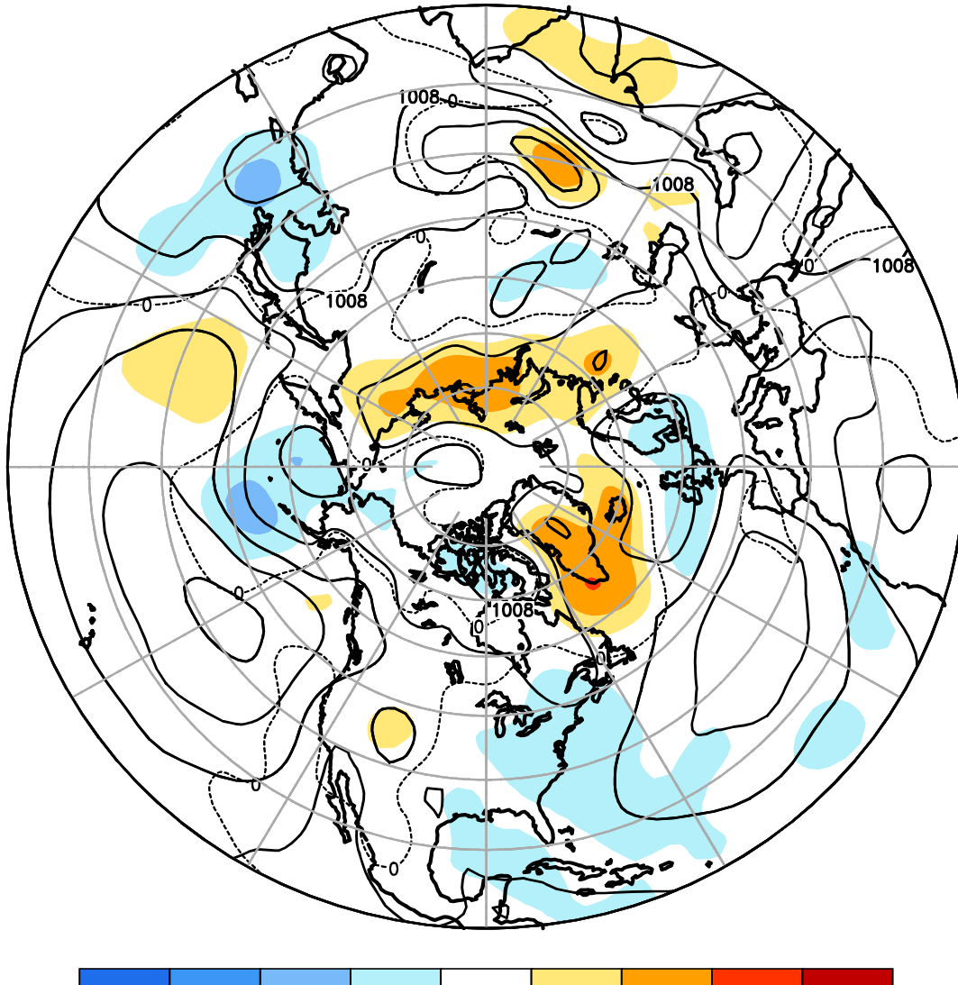
FIGURE E8. Northern Hemisphere mean and anomalous sea level pressure (CDAS/Reanalysis) for AUG 2023. Mean values are denoted by solid contours drawn at an interval of 4 hPa. Anomaly contour interval is 2 hPa with values less (greater) than -2 hPa (2 hPa) indicated by dark (light) shading. Anomalies are calculated as departures from the 1991-2020 base period monthly means.
