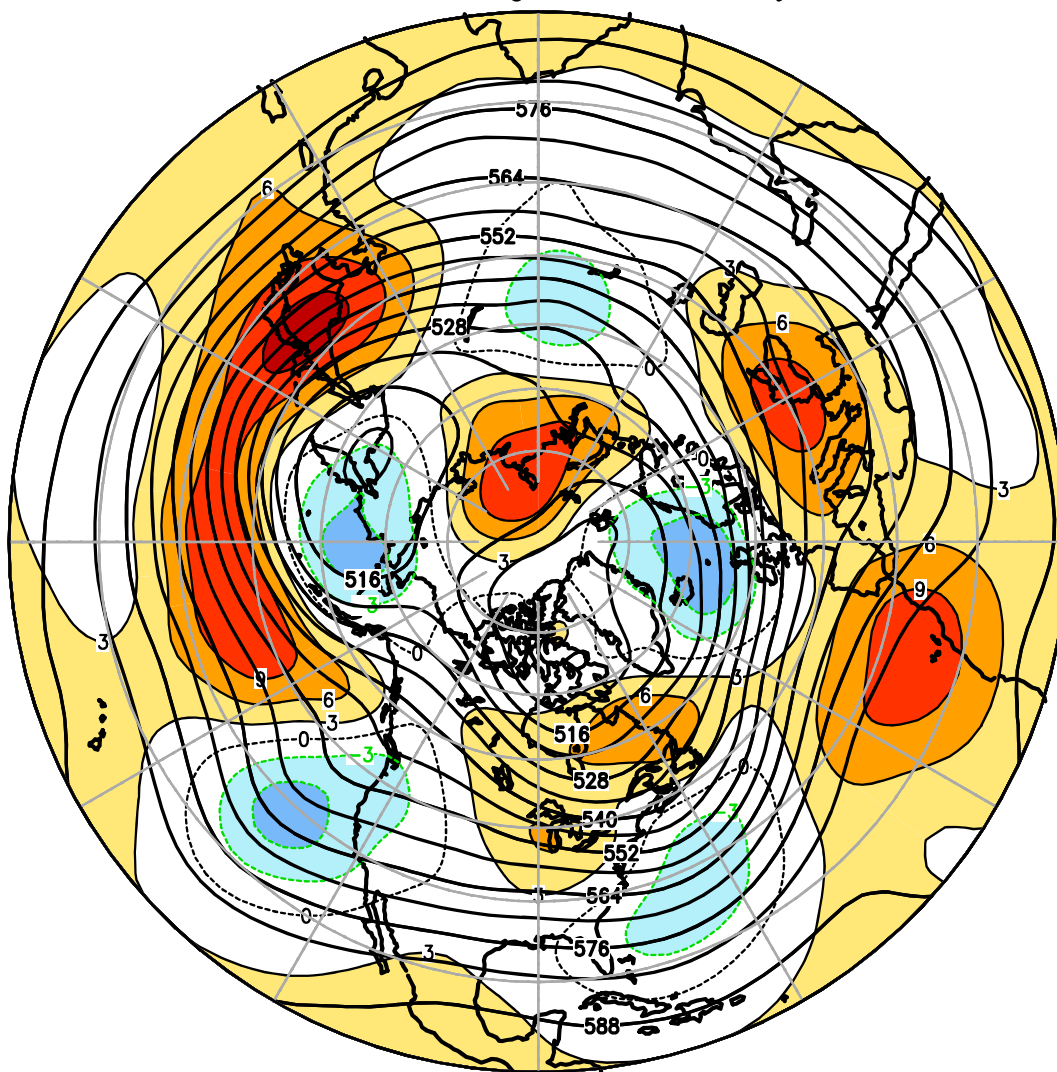
FIGURE E9. Northern Hemisphere mean and anomalous 500-hPa geopotential height (CDAS/Reanalysis) for FEB 2024. Mean heights are denoted by solid contours drawn at an interval of 6 dam. Anomaly contour interval is 3 dam with values less (greater) than -3 dam (3 dam) indicated by dark (light) shading. Anomalies are calculated as departures from the 1991-2020 base period monthly means.
