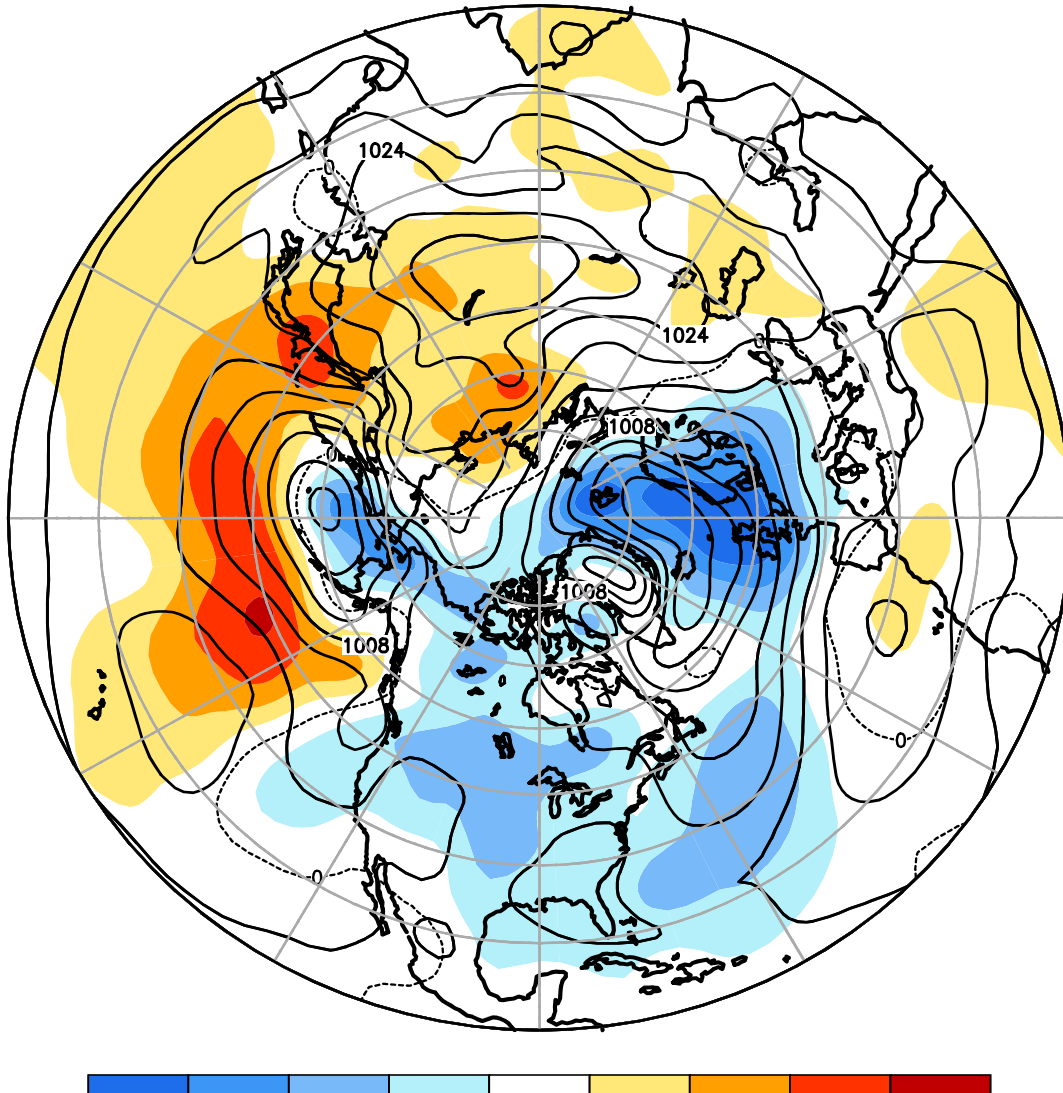
FIGURE E8. Northern Hemisphere mean and anomalous sea level pressure (CDAS/Reanalysis) for FEB 2024. Mean values are denoted by solid contours drawn at an interval of 4 hPa. Anomaly contour interval is 2 hPa with values less (greater) than -2 hPa (2 hPa) indicated by dark (light) shading. Anomalies are calculated as departures from the 1991-2020 base period monthly means.
