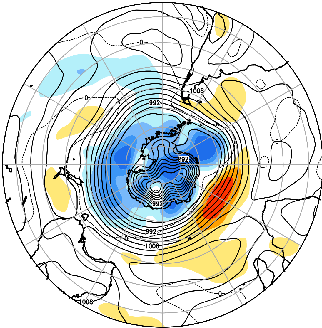
FIGURE E14. Southern Hemisphere mean and anomalous sea level pressure(CDAS/Reanalysis) for FEB 2024. Mean values are denoted by solid contours drawn at an interval of 4 hPa. Anomaly contour interval is 2 hPa with values less (greater) than -2 hPa (2 hPa) indicated by dark (light) shading. Anomalies are calculated as departures from the 1991-2020 base period monthly means.
