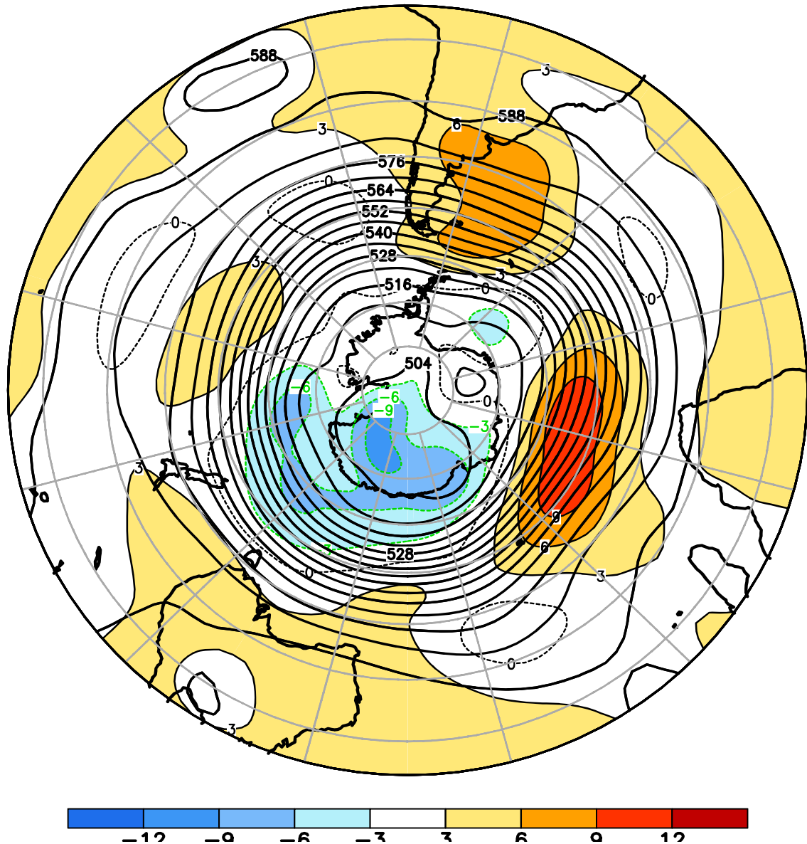
FIGURE E15. Southern Hemisphere mean and anomalous 500-hPa geopotential height (CDAS/Reanalysis) for FEB 2024. Mean heights are denoted by solid contours drawn at an interval of 6 dam. Anomaly contour interval is 3 dam with values less (greater) than -3 dam (3 dam) indicated by dark (light) shading. Anomalies are calculated as departures from the 1991-2020 base period monthly means.
