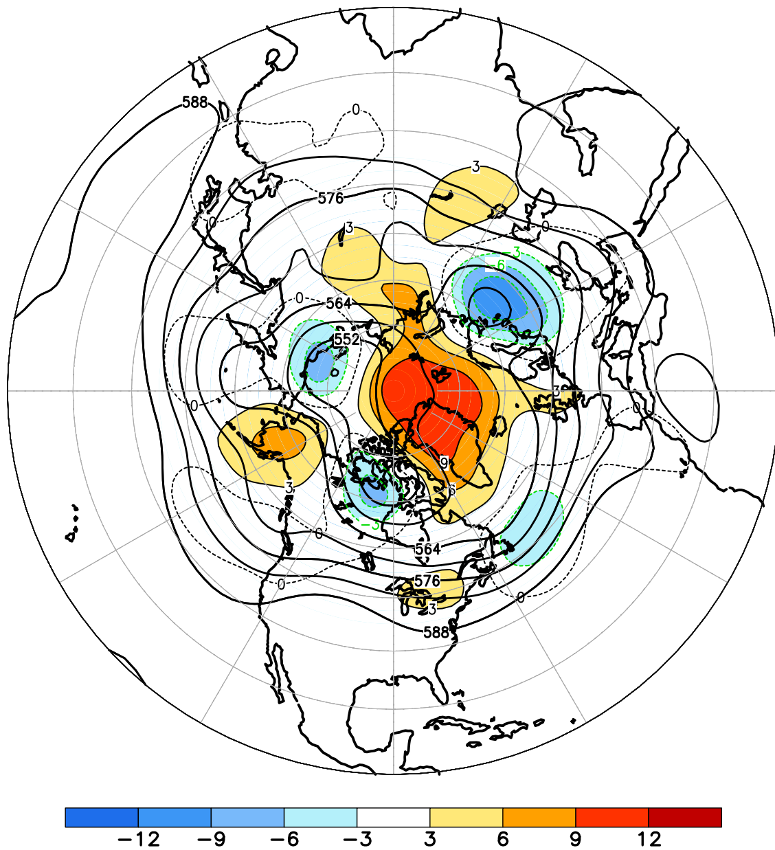
FIGURE E9. Northern Hemisphere mean and anomalous 500-hPa geopotential height (CDAS/Reanalysis) for JUL 2019. Mean heights are denoted by solid contours drawn at an interval of 6 dam. Anomaly contour interval is 3 dam with values less (greater) than -3 dam (3 dam) indicated by dark (light) shading. Anomalies are calculated as departures from the 1981-2010 base period monthly means.
