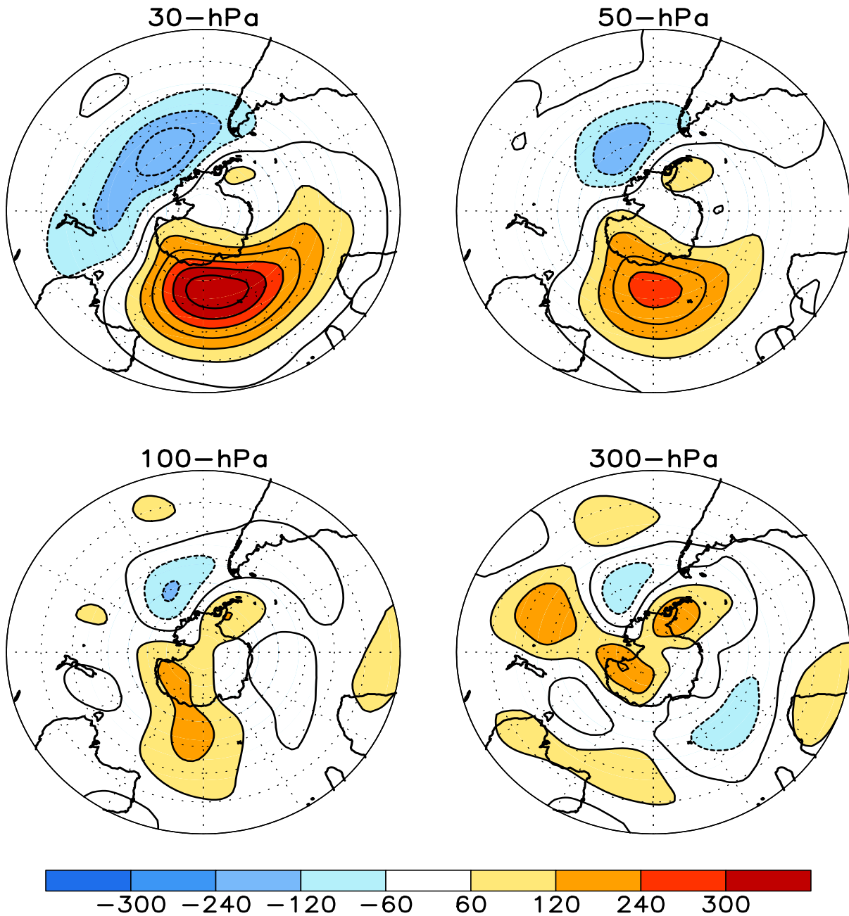
FIGURE S1. Stratospheric height anomalies (m) at selected levels for JUL 2019. Positive values are indicated by solid contours and dark shading. Negative values are indicated by dashed contours and light shading. Contour interval is 60 m. Anomalies are calculated from the 1981-2010 base period means. Winter Hemisphere is shown.
