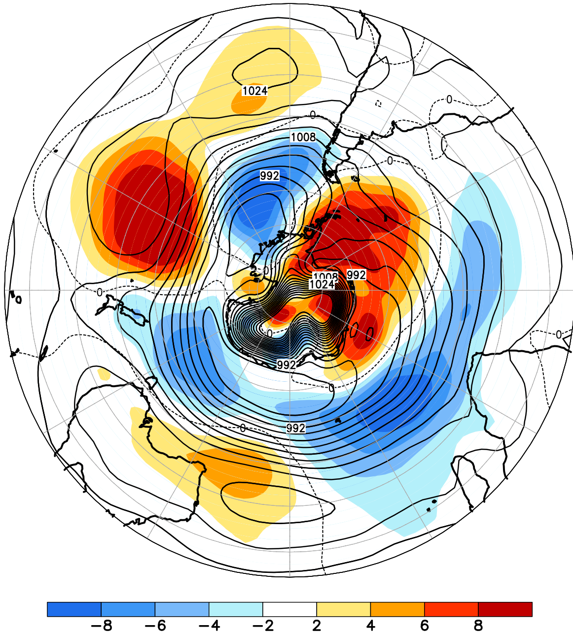
FIGURE E14. Southern Hemisphere mean and anomalous sea level pressure(CDAS/Reanalysis) for JUL 2019. Mean values are denoted by solid contours drawn at an interval of 4 hPa. Anomaly contour interval is 2 hPa with values less (greater) than -2 hPa (2 hPa) indicated by dark (light) shading. Anomalies are calculated as departures from the 1981-2010 base period monthly means.
