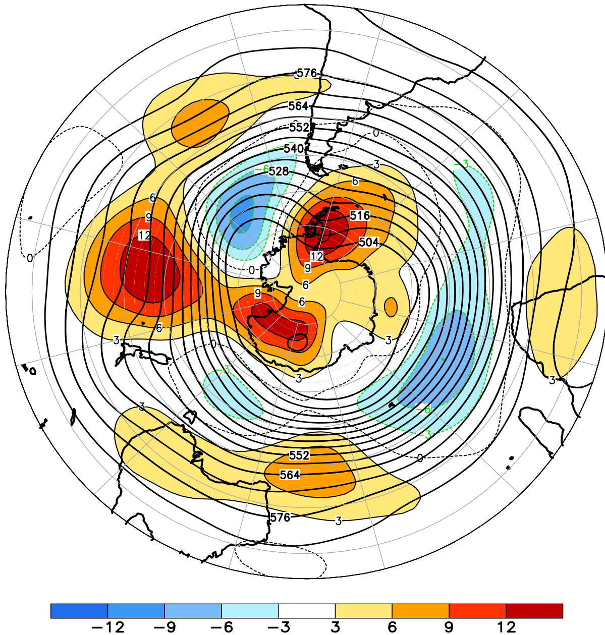
FIGURE E15. Southern Hemisphere mean and anomalous 500-hPa geopotential height (CDAS/Reanalysis) for JUL 2019. Mean heights are denoted by solid contours drawn at an interval of 6 dam. Anomaly contour interval is 3 dam with values less (greater) than -3 dam (3 dam) indicated by dark (light) shading. Anomalies are calculated as departures from the 1981-2010 base period monthly means.
