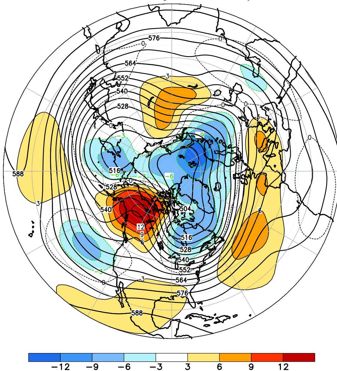
FIGURE E9. Northern Hemisphere mean and anomalous 500-hPa geopotential height (CDAS/Reanalysis) for MAR 2019. Mean heights are denoted by solid contours drawn at an interval of 6 dam. Anomaly contour interval is 3 dam with values less (greater) than -3 dam (3 dam) indicated by dark (light) shading. Anomalies are calculated as departures from the 1981-2010 base period monthly means.
