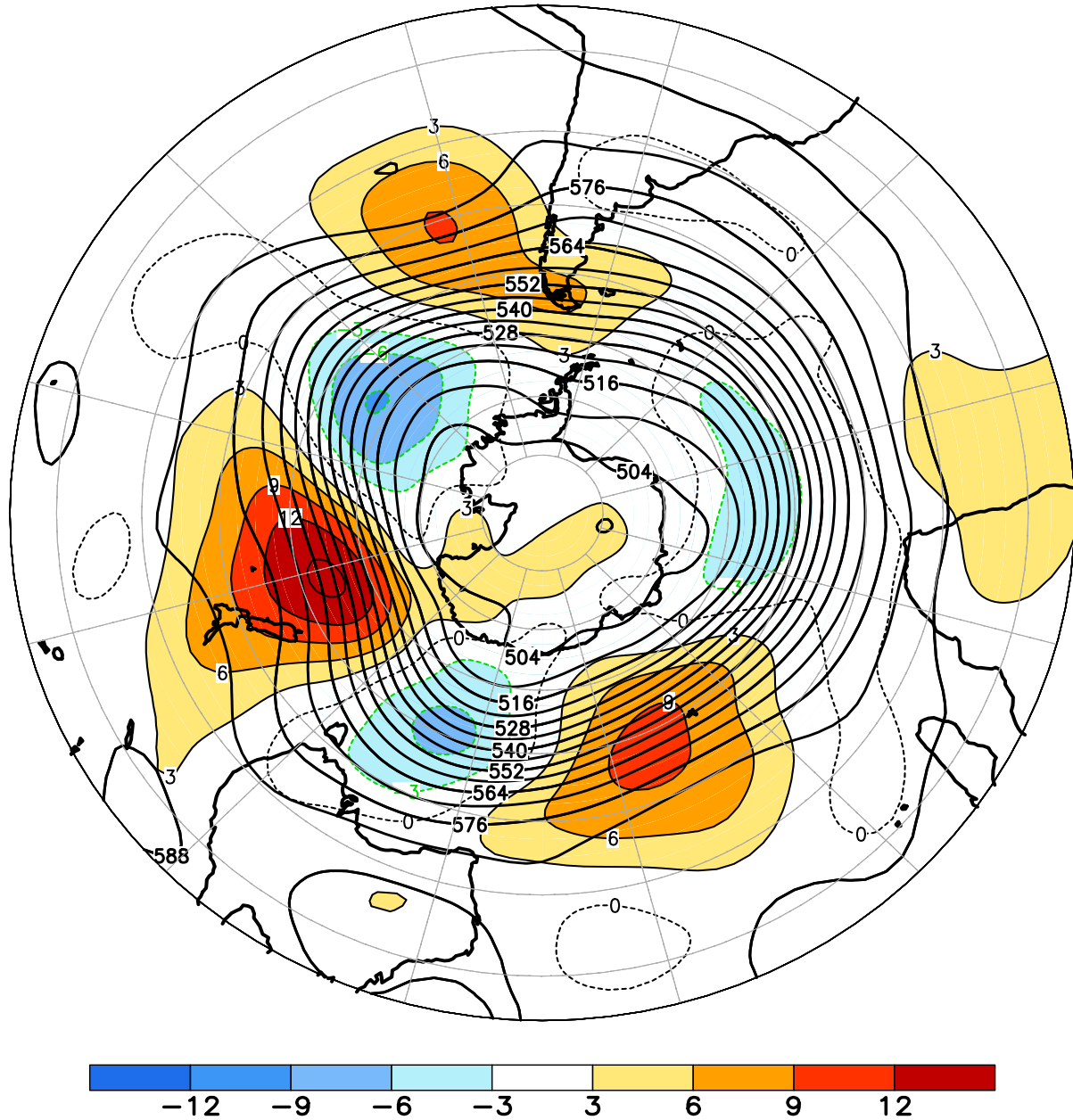
FIGURE E15. Southern Hemisphere mean and anomalous 500-hPa geopotential height (CDAS/Reanalysis) for MAR 2019. Mean heights are denoted by solid contours drawn at an interval of 6 dam. Anomaly contour interval is 3 dam with values less (greater) than -3 dam (3 dam) indicated by dark (light) shading. Anomalies are calculated as departures from the 1981-2010 base period monthly means.
