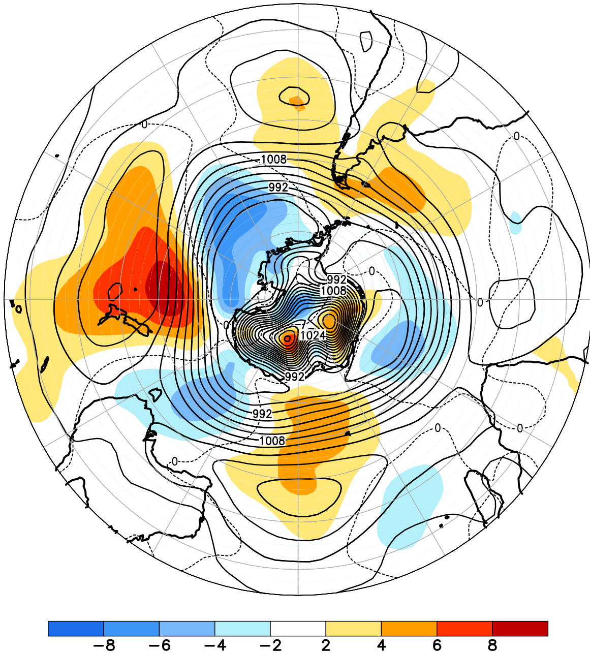
FIGURE E14. Southern Hemisphere mean and anomalous sea level pressure(CDAS/Reanalysis) for MAR 2019. Mean values are denoted by solid contours drawn at an interval of 4 hPa. Anomaly contour interval is 2 hPa with values less (greater) than -2 hPa (2 hPa) indicated by dark (light) shading. Anomalies are calculated as departures from the 1981-2010 base period monthly means.
