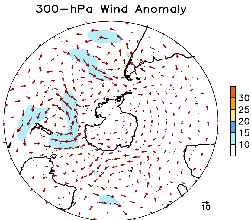
FIGURE E16. Southern Hemisphere mean (left) and anomalous (right) 300-hPa vector wind (CDAS/Reanalysis) for MAR 2019. Mean (anomaly) isotach contour interval is 10 (5) \text{ms}^{-1} . Values greater than 30 \text{ms}^{-1} (left) and 10 \text{ms}^{-1} (rights) are shaded. Anomalies are departures from the 1981-2010 base period monthly means.
