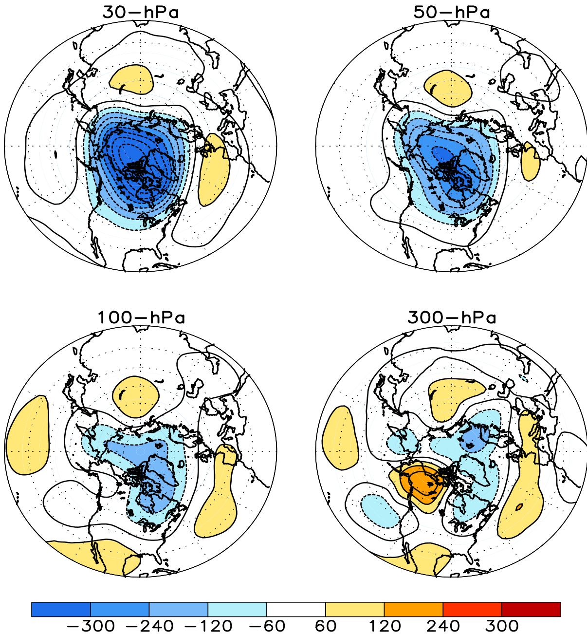
FIGURE S1. Stratospheric height anomalies (m) at selected levels for MAR 2019. Positive values are indicated by solid contours and dark shading. Negative values are indicated by dashed contours and light shading. Contour interval is 60 m. Anomalies are calculated from the 1981-2010 base period means. Winter Hemisphere is shown.
