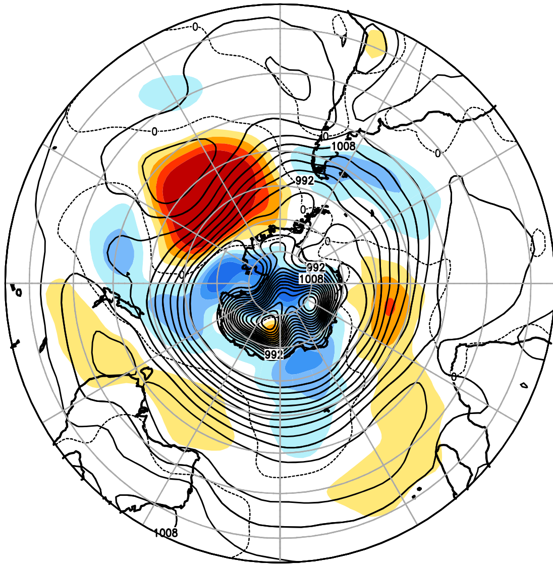
FIGURE E14. Southern Hemisphere mean and anomalous sea level pressure(CDAS/Reanalysis) for MAR 2024. Mean values are denoted by solid contours drawn at an interval of 4 hPa. Anomaly contour interval is 2 hPa with values less (greater) than -2 hPa (2 hPa) indicated by dark (light) shading. Anomalies are calculated as departures from the 1991-2020 base period monthly means.
