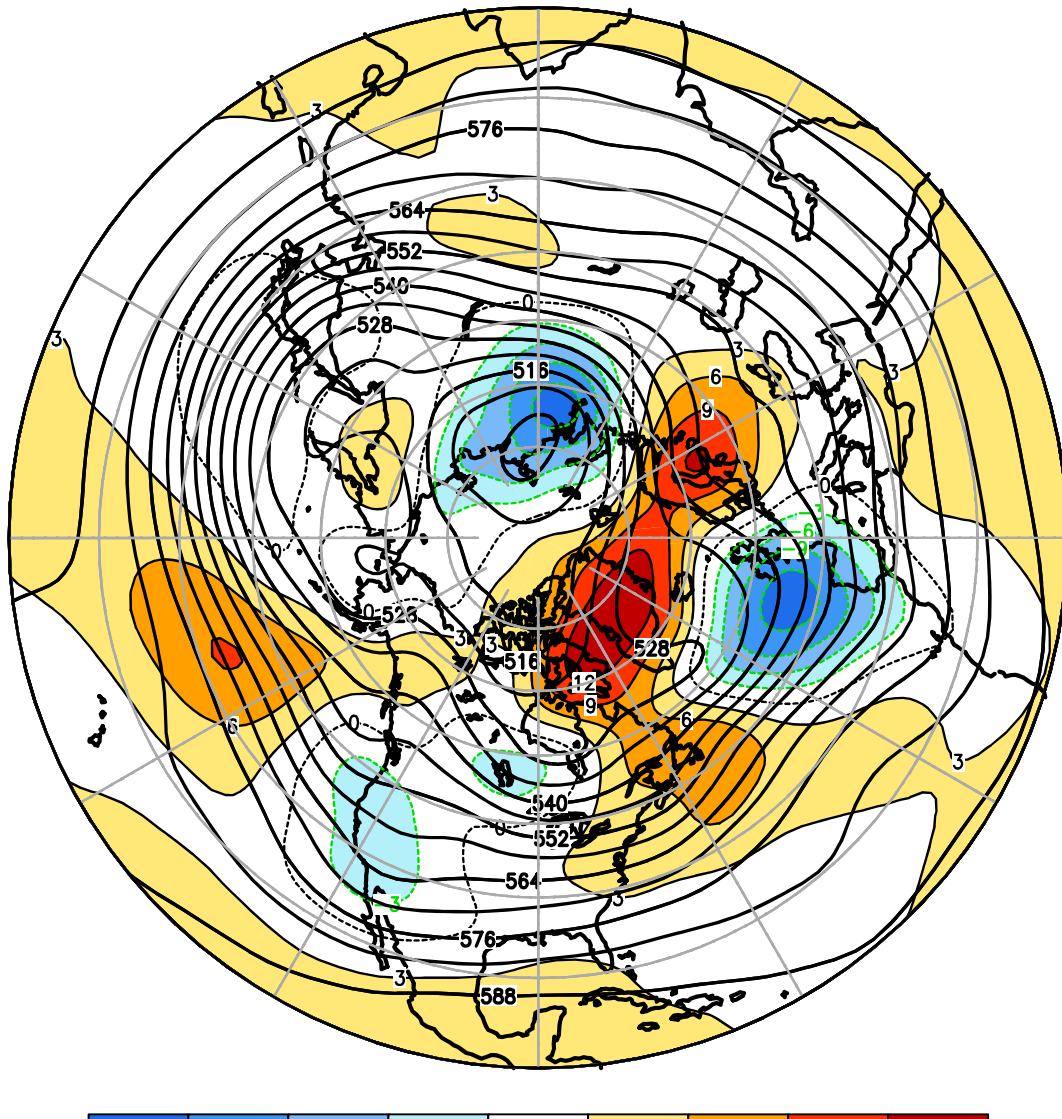
FIGURE E9. Northern Hemisphere mean and anomalous 500-hPa geopotential height (CDAS/Reanalysis) for MAR 2024. Mean heights are denoted by solid contours drawn at an interval of 6 dam. Anomaly contour interval is 3 dam with values less (greater) than -3 dam (3 dam) indicated by dark (light) shading. Anomalies are calculated as departures from the 1991-2020 base period monthly means.
