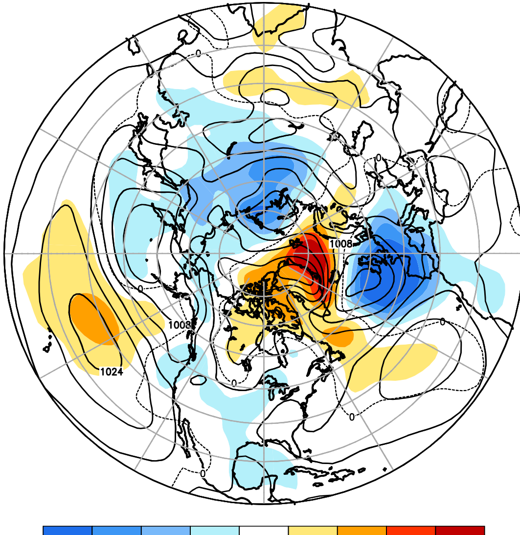
FIGURE E8. Northern Hemisphere mean and anomalous sea level pressure (CDAS/Reanalysis) for MAR 2024. Mean values are denoted by solid contours drawn at an interval of 4 hPa. Anomaly contour interval is 2 hPa with values less (greater) than -2 hPa (2 hPa) indicated by dark (light) shading. Anomalies are calculated as departures from the 1991-2020 base period monthly means.
