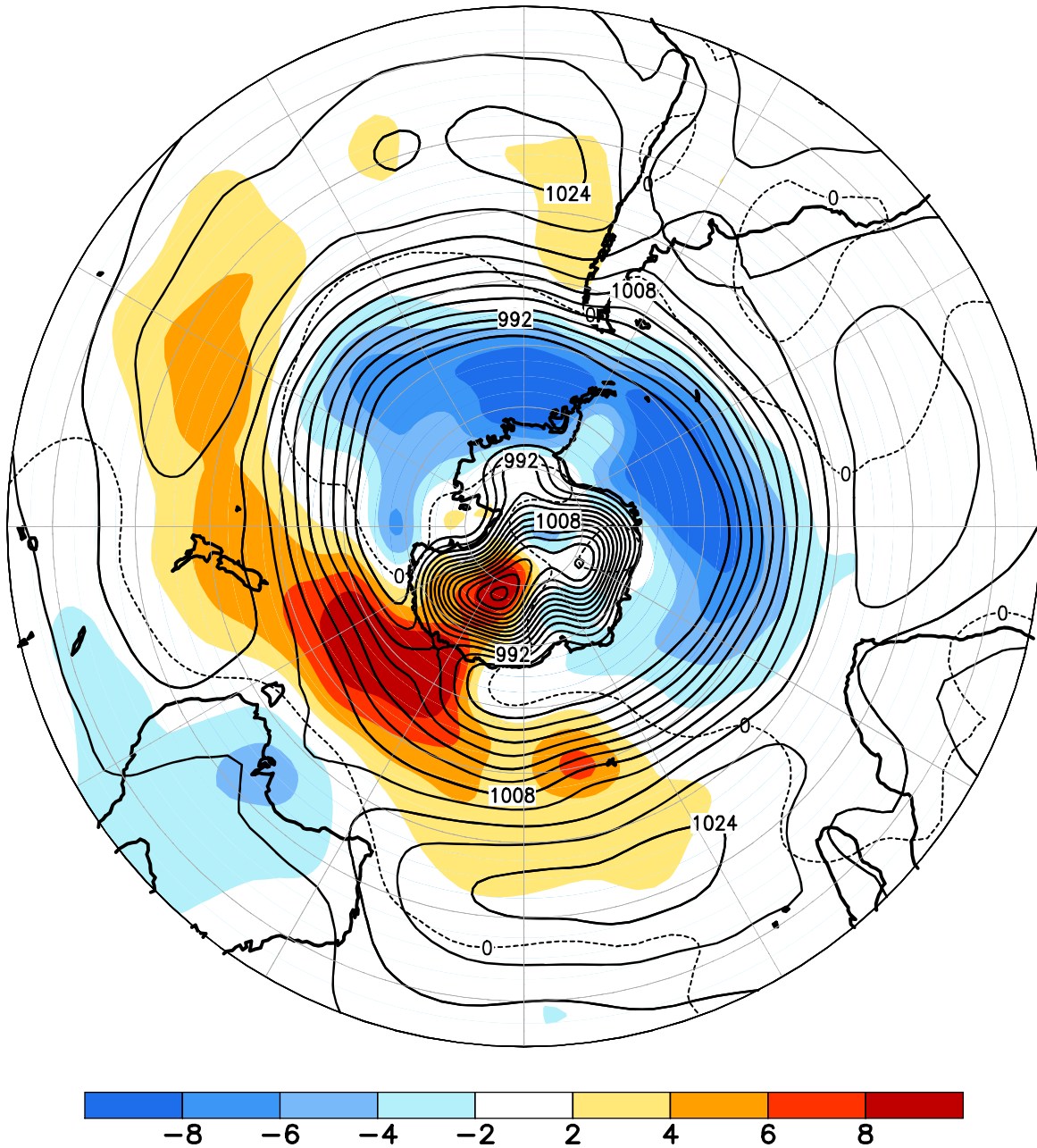
FIGURE E14. Southern Hemisphere mean and anomalous sea level pressure(CDAS/Reanalysis) for OCT 2022. Mean values are denoted by solid contours drawn at an interval of 4 hPa. Anomaly contour interval is 2 hPa with values less (greater) than -2 hPa (2 hPa) indicated by dark (light) shading. Anomalies are calculated as departures from the 1991-2020 base period monthly means.
