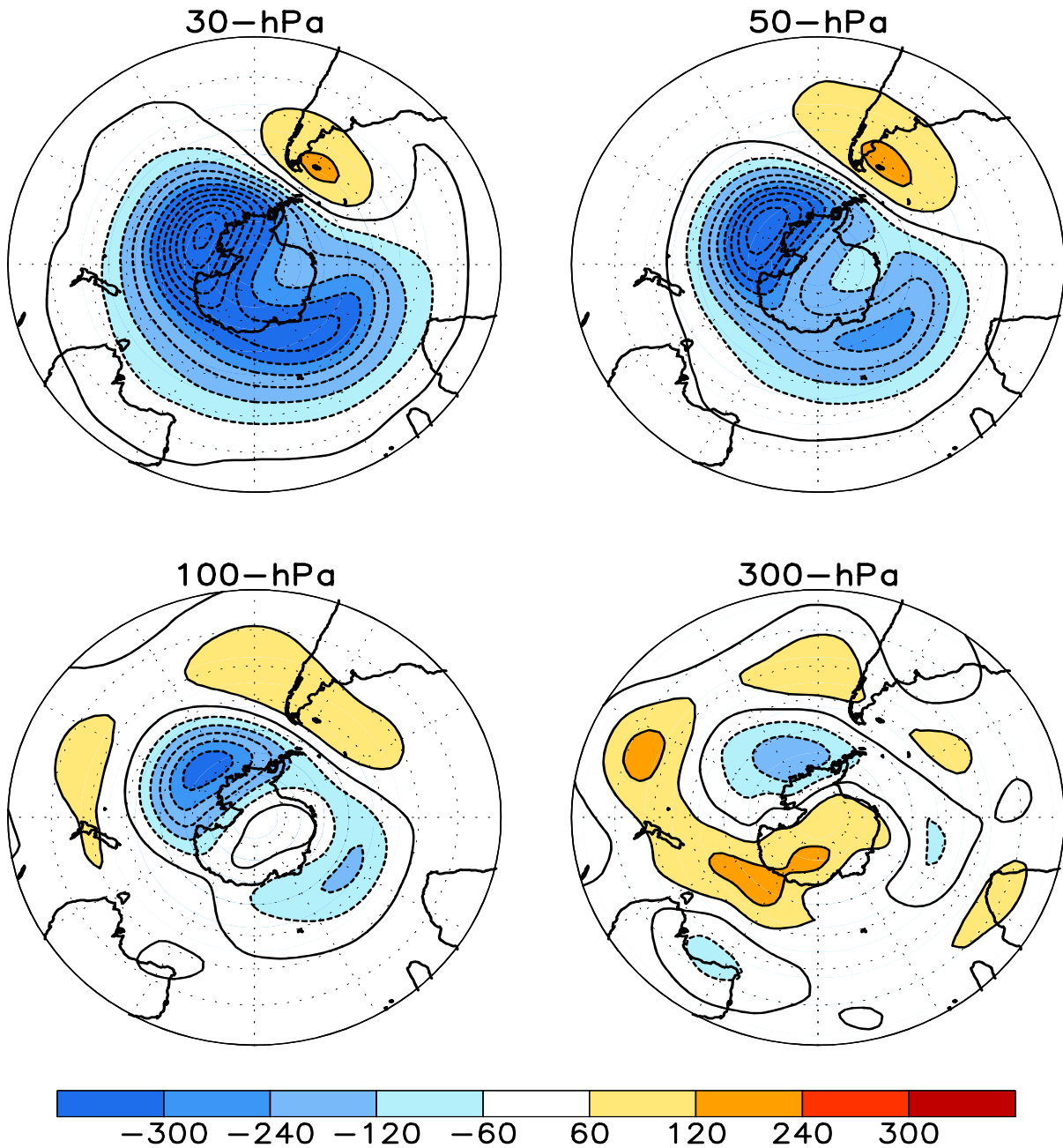
FIGURE S1. Stratospheric height anomalies (m) at selected levels for OCT 2022. Positive values are indicated by solid contours and dark shading. Negative values are indicated by dashed contours and light shading. Contour interval is 60 m. Anomalies are calculated from the 1991-2020 base period means. Winter Hemisphere is shown.
