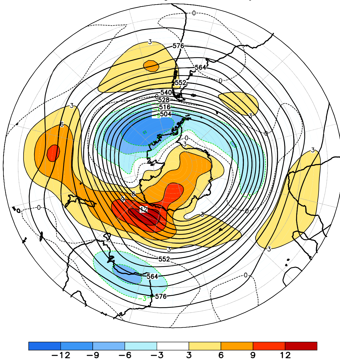
FIGURE E15. Southern Hemisphere mean and anomalous 500-hPa geopotential height (CDAS/Reanalysis) for OCT 2022. Mean heights are denoted by solid contours drawn at an interval of 6 dam. Anomaly contour interval is 3 dam with values less (greater) than -3 dam (3 dam) indicated by dark (light) shading. Anomalies are calculated as departures from the 1991-2020 base period monthly means.
