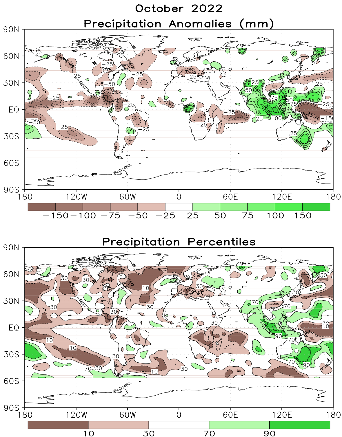
FIGURE E3. Anomalous precipitation (mm, top) and precipitation percentiles based on a Gamma distribution fit to the 1981-2010 base period data (bottom) for OCT 2022. Data are obtained from a merge of raingauge observations and satellite-derived precipitation estimates (Janowiak and Xie 1999, J. Climate , 12 , 3335–3342). Contours are drawn at 200, 100, 50, 25, -25, -50, -100, and -200 mm in top panel. Percentiles are not plotted in regions where mean monthly precipitation is <5mm/month.
