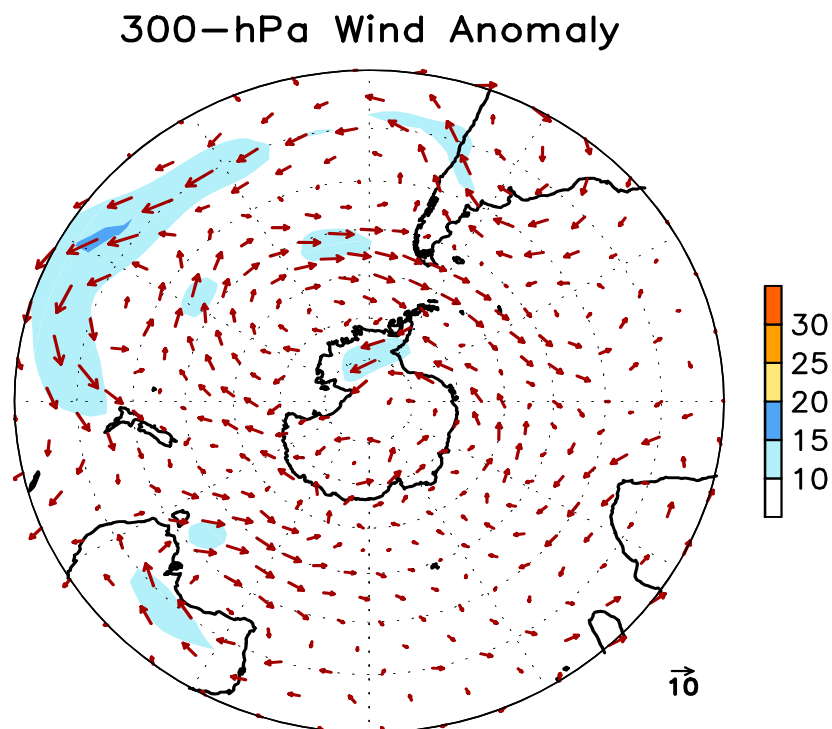
FIGURE E16. Southern Hemisphere mean (left) and anomalous (right) 300-hPa vector wind (CDAS/Reanalysis) for OCT 2022. Mean (anomaly) isotach contour interval is 10 (5) \text{ms}^{-1} . Values greater than 30 \text{ms}^{-1} (left) and 10 \text{ms}^{-1} (rights) are shaded. Anomalies are departures from the 1991-2020 base period monthly means.
