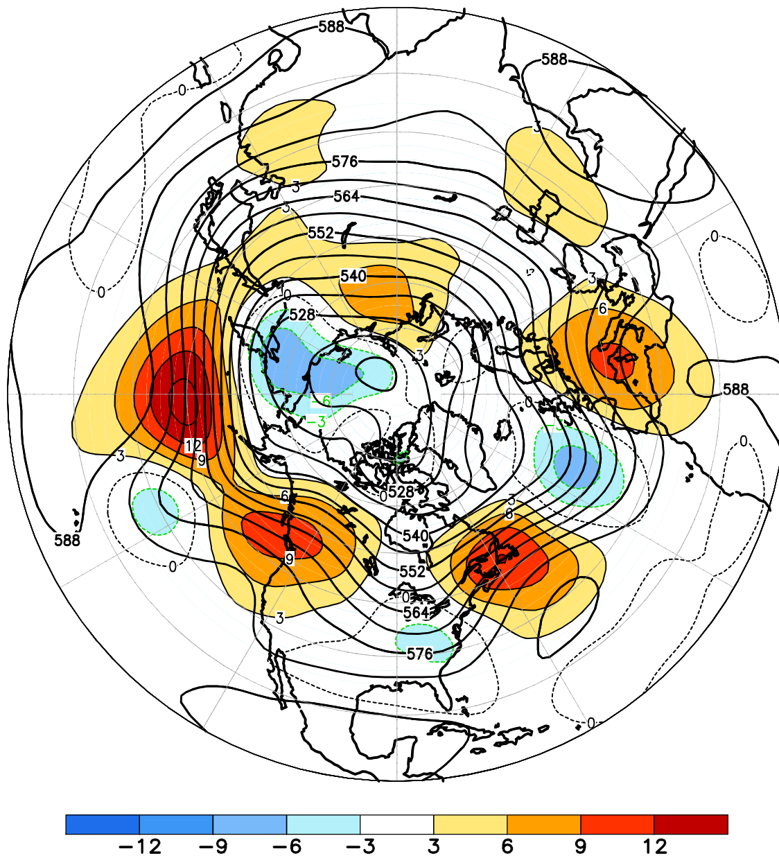
FIGURE E9. Northern Hemisphere mean and anomalous 500-hPa geopotential height (CDAS/Reanalysis) for OCT 2022. Mean heights are denoted by solid contours drawn at an interval of 6 dam. Anomaly contour interval is 3 dam with values less (greater) than -3 dam (3 dam) indicated by dark (light) shading. Anomalies are calculated as departures from the 1991-2020 base period monthly means.
