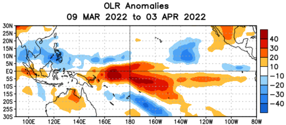
Figure 5. Average outgoing longwave radiation (OLR) anomalies ( W/m^2 ) for the period 9 March – 3 April 2022. OLR anomalies are computed as departures from the 1991-2020 base period pentad means.
