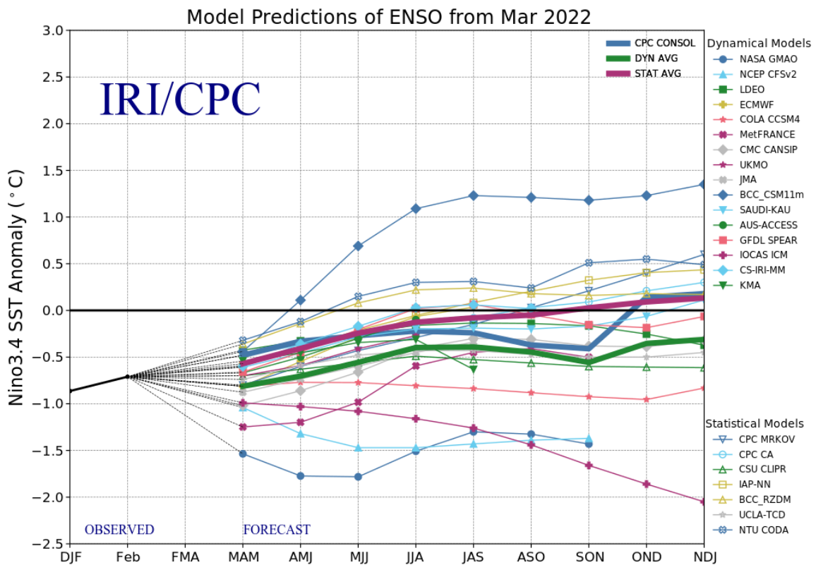
Figure 6. Forecasts of sea surface temperature (SST) anomalies for the Niño 3.4 region ( 5^{\circ}N - 5^{\circ}S , 120^{\circ}W - 170^{\circ}W ). Figure updated 18 March 2022.
