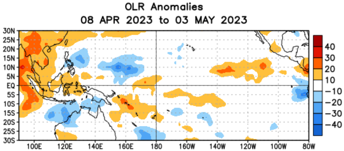
Figure 5. Average outgoing longwave radiation (OLR) anomalies ( W/m^2 ) for the period 8 April – 3 May 2023. OLR anomalies are computed as departures from the 1991-2020 base period pentad means.
