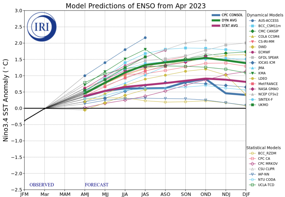
Figure 6. Forecasts of sea surface temperature (SST) anomalies for the Niño 3.4 region ( 5^{\circ}N - 5^{\circ}S , 120^{\circ}W - 170^{\circ}W ). Figure updated 19 April 2023 by the International Research Institute (IRI) for Climate and Society.
